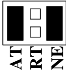
Figure 2 - Headers J1B – J4B, RS-485 'Auto' Enabled, with 'No Echo'
