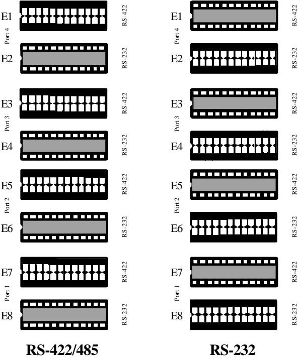
Figure 6 - Headers E1 - E4, Electrical Interface Selection
