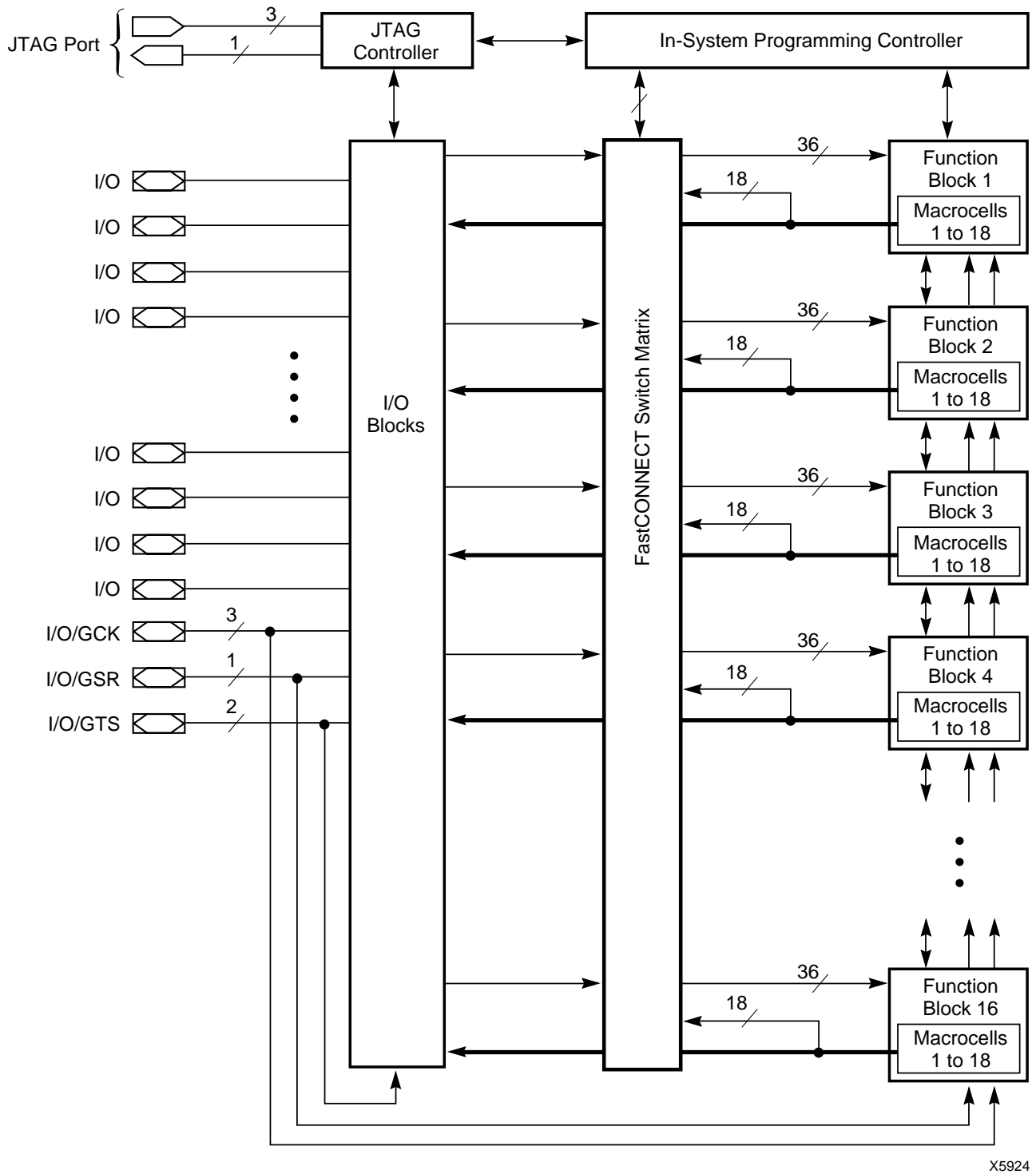
Figure 2: XC95288 Architecture
