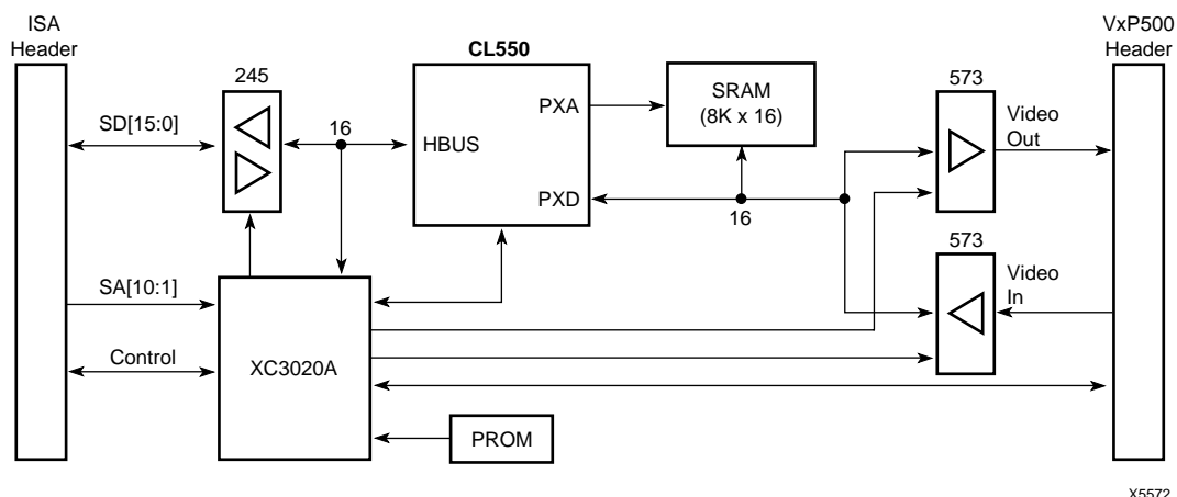
Figure 1. CL550 Motion-JPEG Daughter Card Block Diagram
