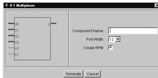
Figure 2: Parameterization Window
