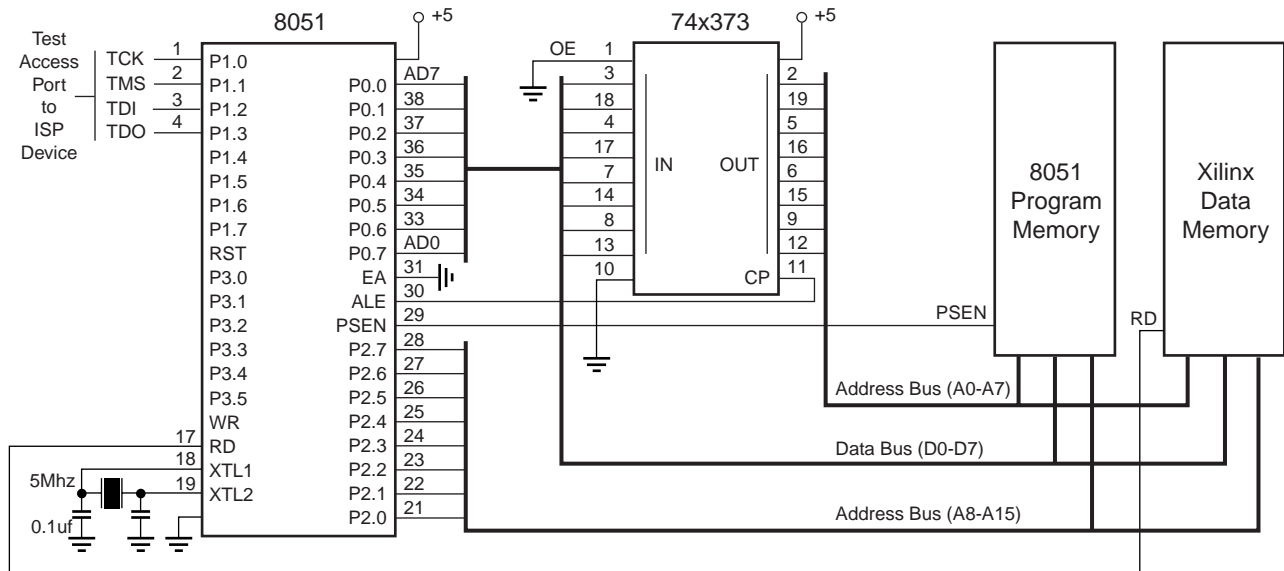
Figure 1: ISP Controller Schematic
