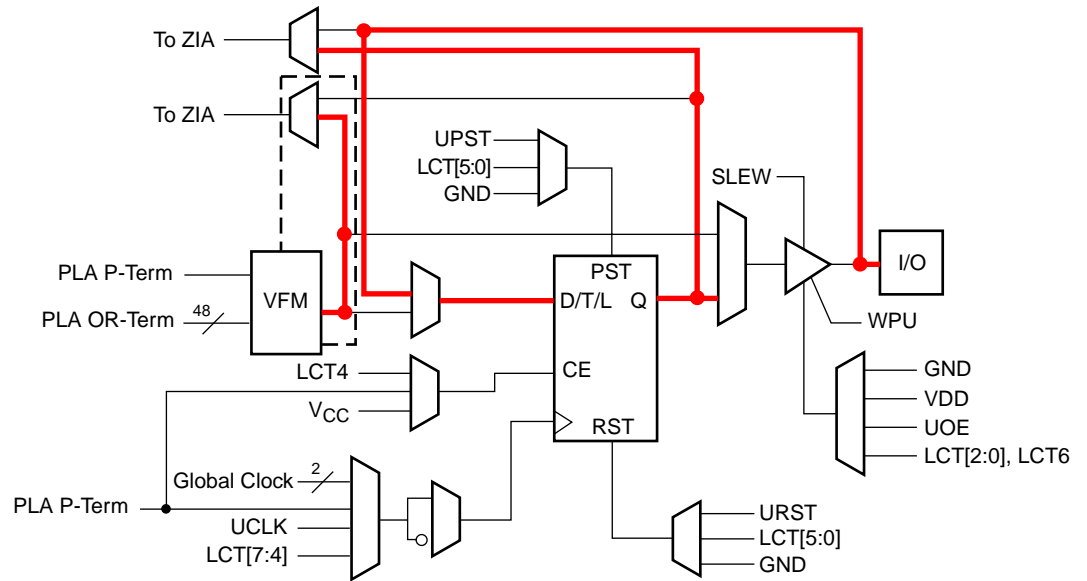
Figure 10: XPLA3 Input Register Path with Buried Combinatorial Node
