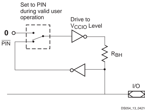
Figure 13: Bus-Hold Logic
