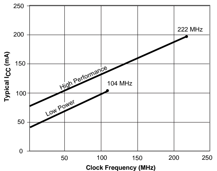
Figure 1: Typical I_{CC} vs. Frequency for XC95144XL
