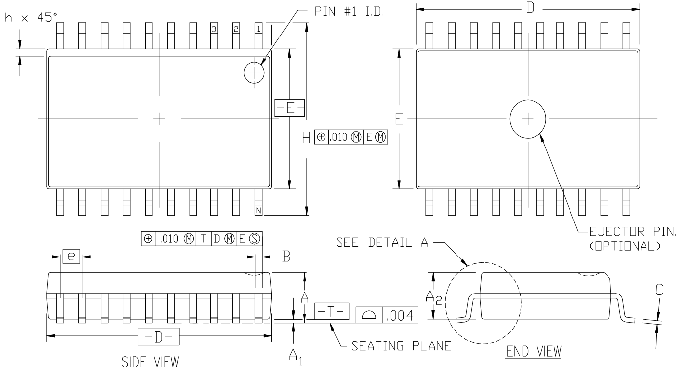
BOTTOM VIEW
