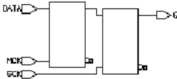
Figure 6-6 Two-Phase Clocks
