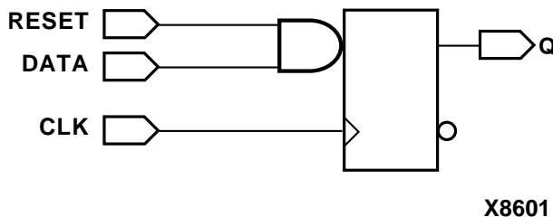
Figure 6-13 D Flip-Flop with Synchronous Reset
