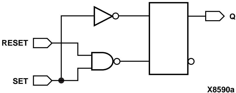
Figure 6-1 SR Latch
