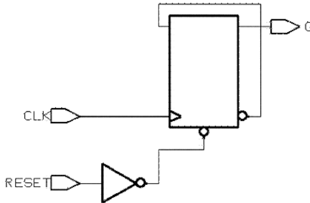
Figure 6-19 Toggle Flip-Flop with Asynchronous Reset
