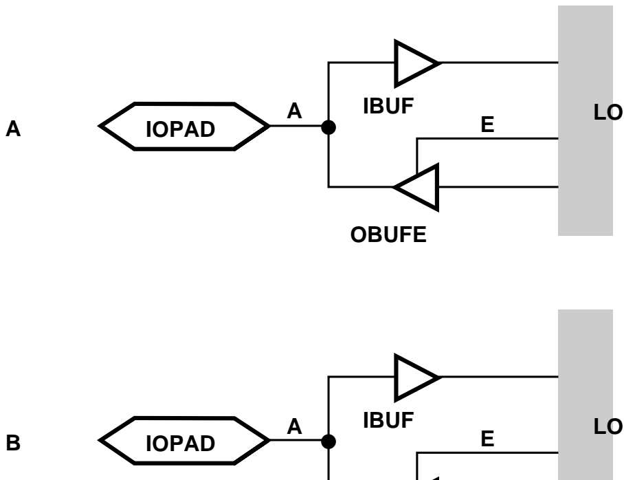
Figure 4-2 Bidirectional Signals and Buses
