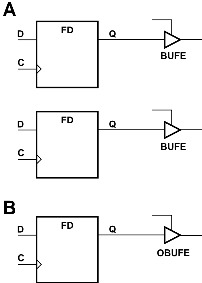
Figure 4-3 Methods of Multiplexing Tristate Signals
