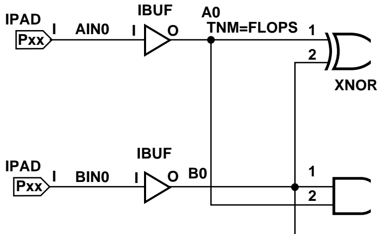
Figure 3-5 TNM on Net Used to Group Flip-Flops
