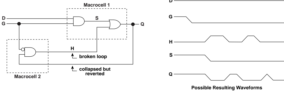
Figure 4-5 Malfunction of Physical Implementation
