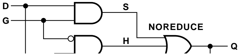
Figure 4-6 D-type Latch Solutions
