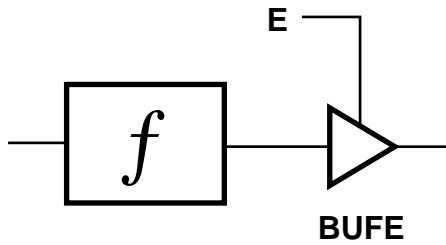
Figure 2-6 Incorrect Tristate Multiplexing of CPLD Outputs
