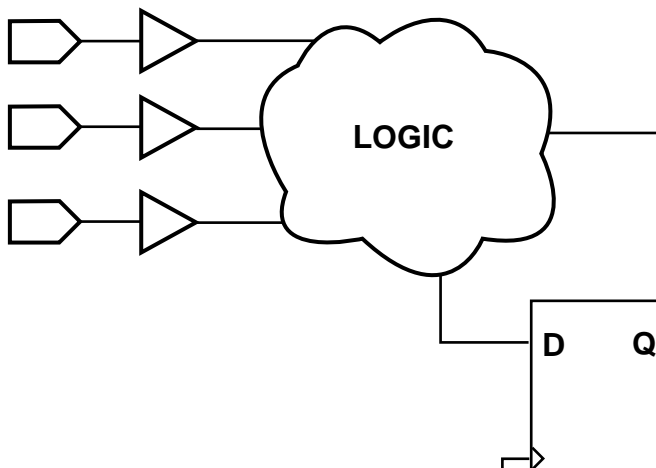
Figure 3-3 TNM on Primitive Symbols
