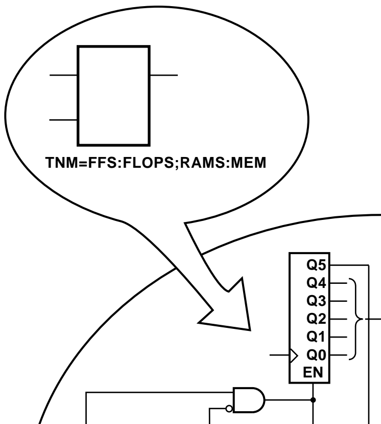
Figure 3-4 TNM on Macro Symbol
