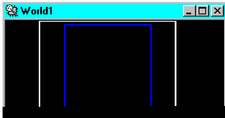
Figure 2-9 World Window
