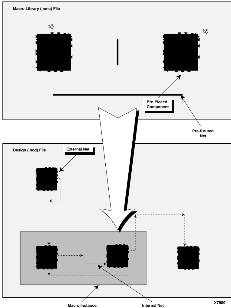
Figure 4-2 Macro Terminology
