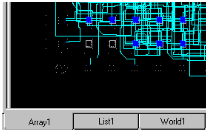
Figure 2-10 Window Tabs
