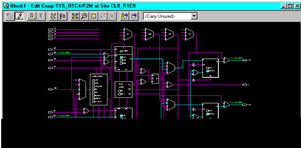
Figure 2-11 Block Window
