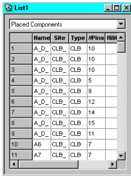
Figure 2-7 List Window
