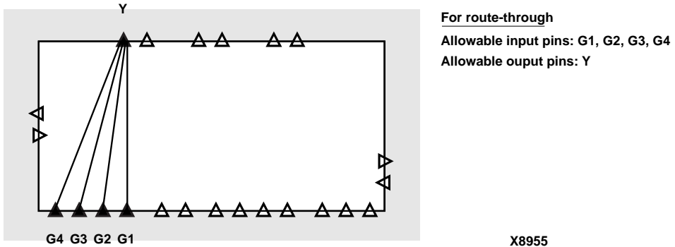
Figure 3-18 Slice Pins for Route-Throughs in Virtex Designs
