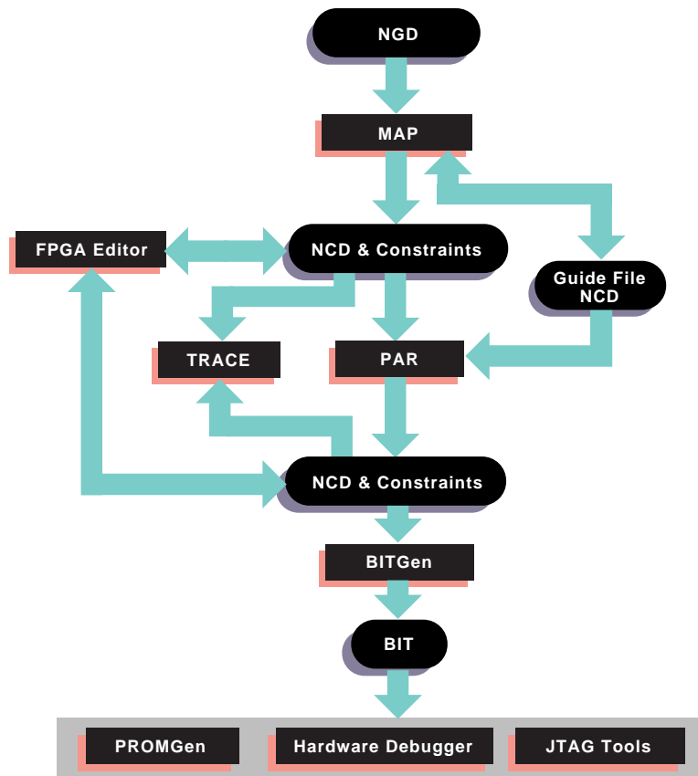
Figure 1-1 Design Flow
