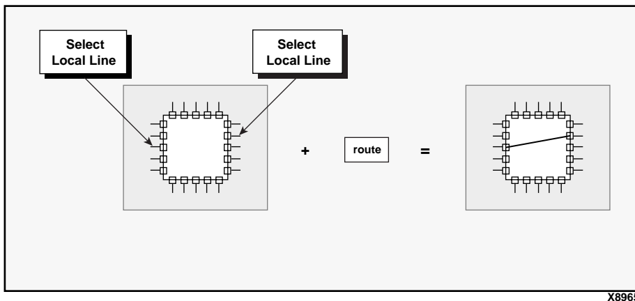
Figure 3-16 Routing Through a Switch Box
