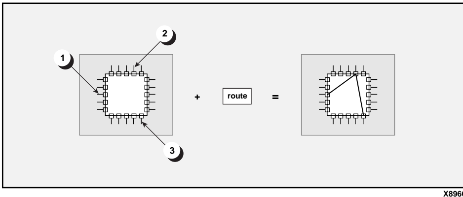
Figure 3-17 Routing a Bank Shot
