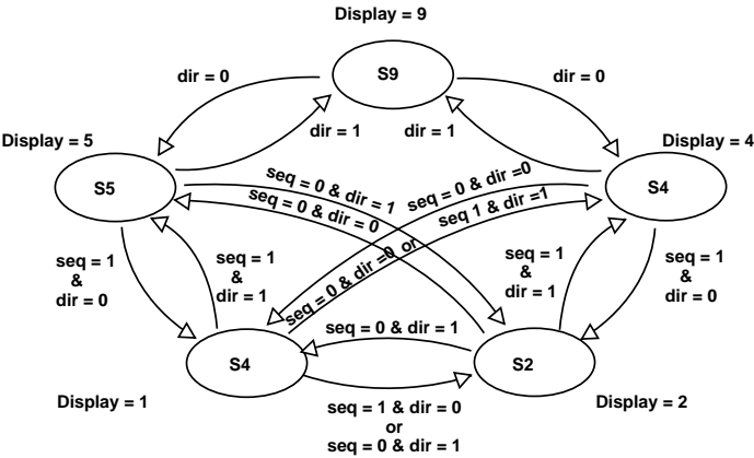
Figure 7-1 State Diagram
