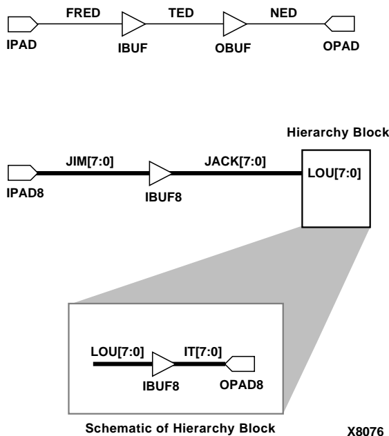
Figure 0-1 Locking I/Os to Pin Locations
