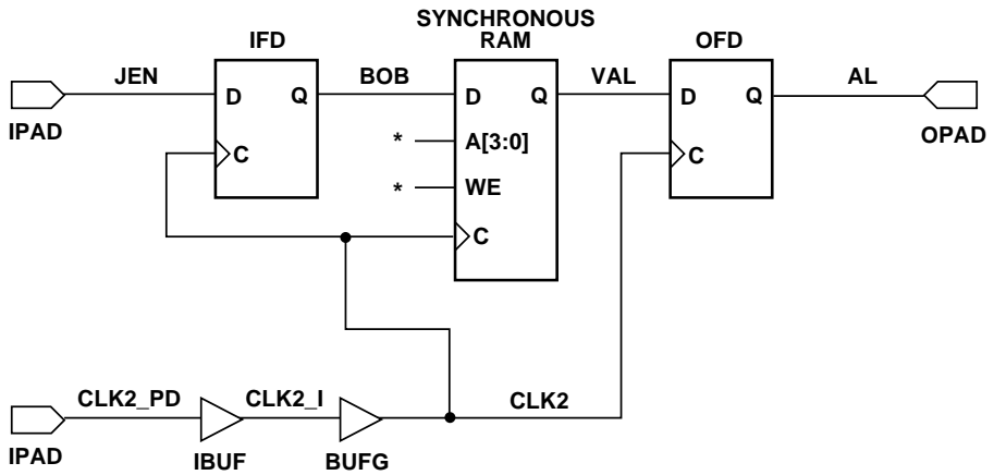
Figure 0-2 Specifying Timing Constraints
