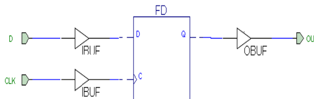
Figure 4-2 MACROS2 Schematic
