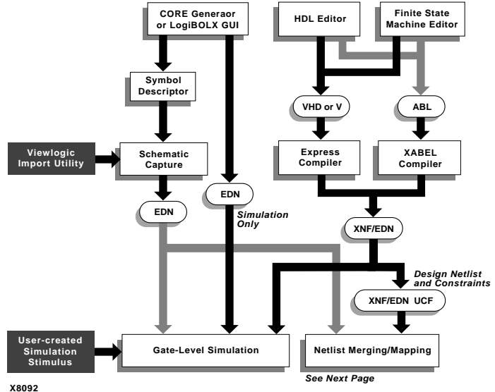
Figure D-1 Manipulation of Netlist and Constraint Files for FPGAs (Part 1)
