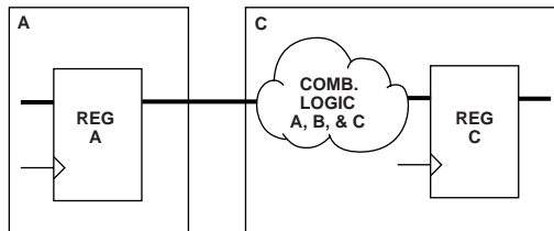
Figure 6-5 Combinatorial Logic Path Grouped Into One Block (Efficient use of Design Resources)
