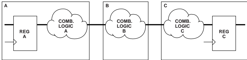
Figure 6-4 Combinatorial Logic Path Split Across Boundaries (Inefficient Use of Design Resources)
