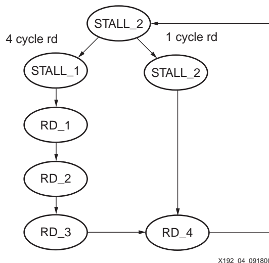
Figure 4: Read Command Finite State Machine
