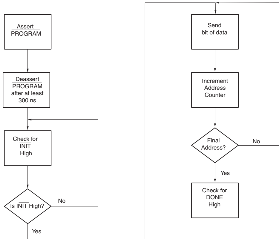
Figure 11: Slave Serial Configuration Flow Diagram
