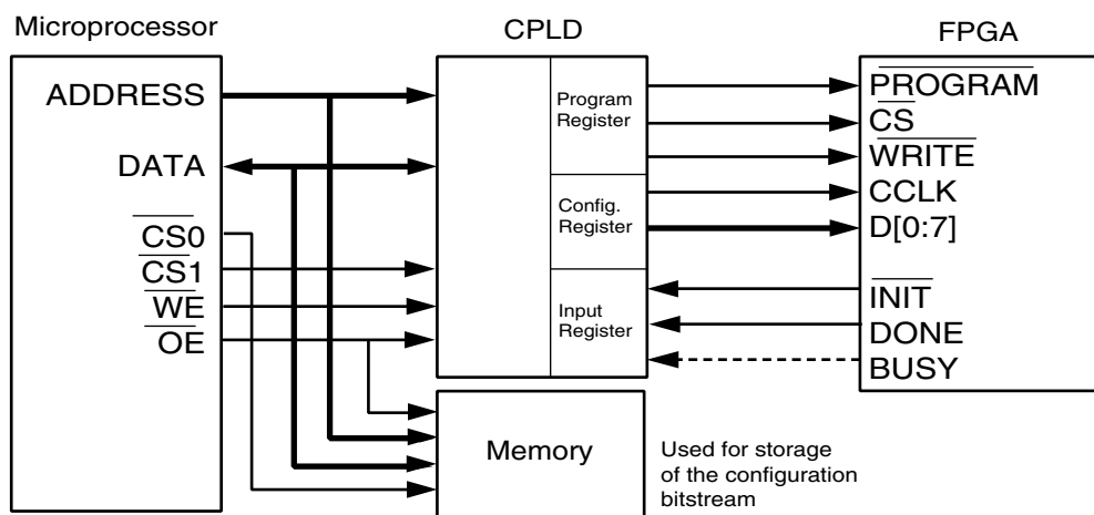
Figure 6: SelectMAP Configuration
