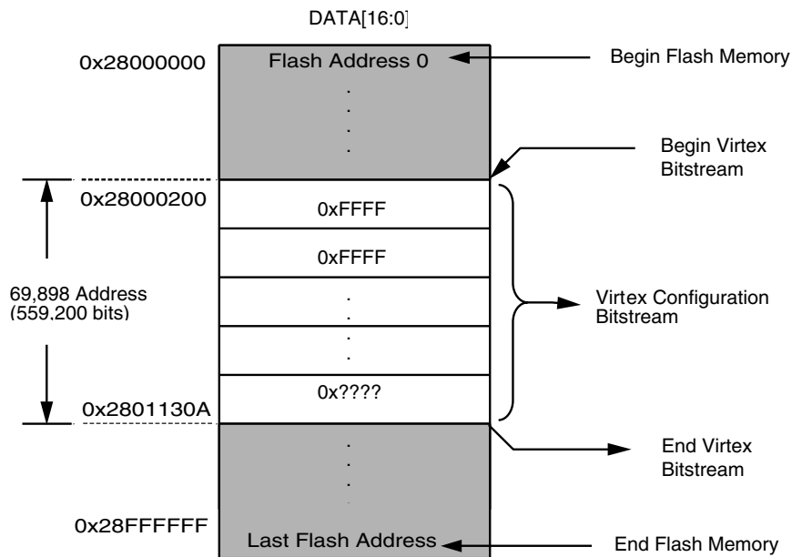
Figure 5: Flash Memory Map
