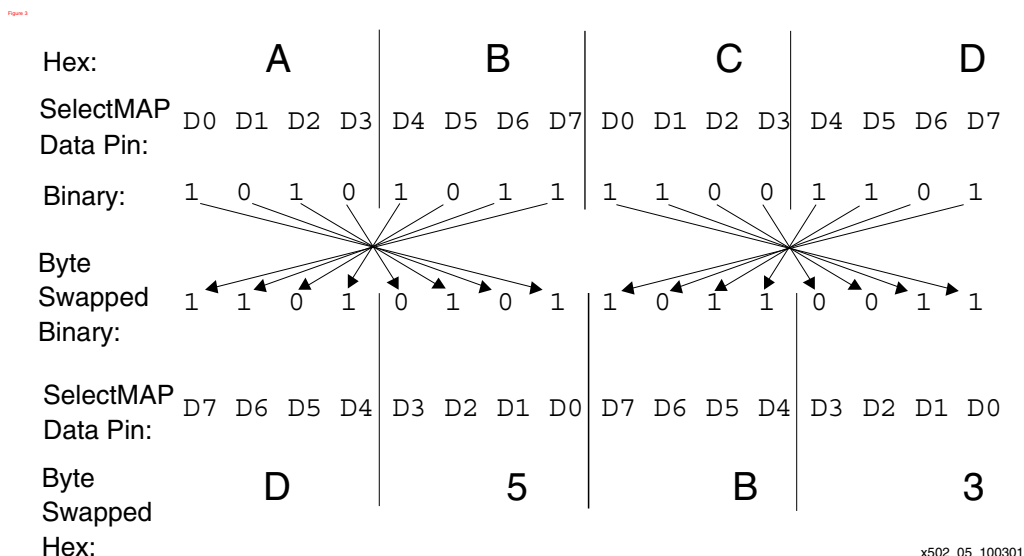
Figure 3: Byte-Swapping Example
