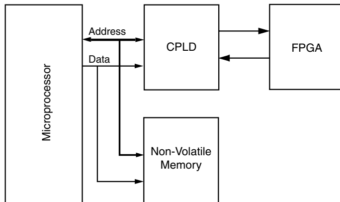
Figure 1: System Diagram
