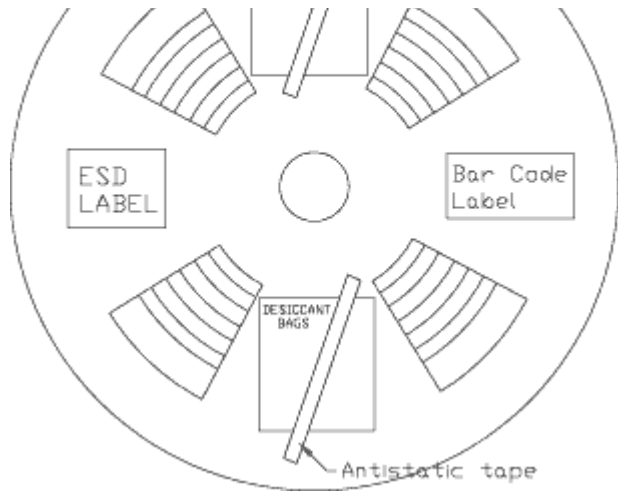
Figure 1: Standard Bar Code Label Locations
