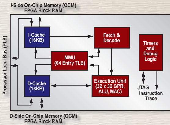
Figure 4 - Inside the PowerPC 405 processor
