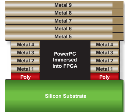
Figure 6 - Hard IP cores are deeply embedded and actively connected within the FPGA fabric
