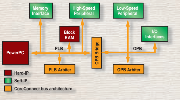
Figure 5 - Hard and soft IP cores
