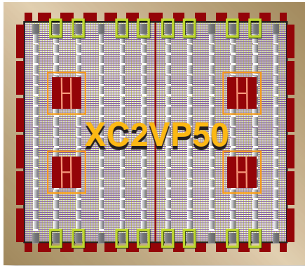
Figure 1 - The Virtex-II Pro XC2VP50 device features four IBM PowerPC 405 processors and 16 Rocket I/O multi-gigabit transceivers embedded in the FPGA fabric
