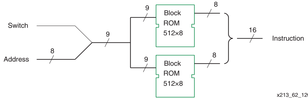
Figure 73: Switching Between Block RAMs (Method 2)
