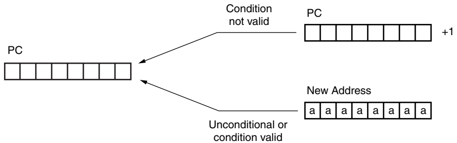
Figure 11: JUMP Instruction
