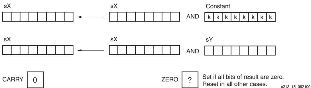
Figure 23: AND Instruction
