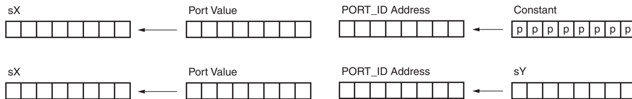
Figure 41: INPUT Instruction
