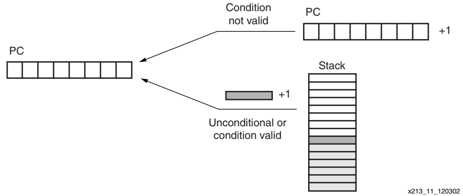
Figure 15: RETURN Instruction
