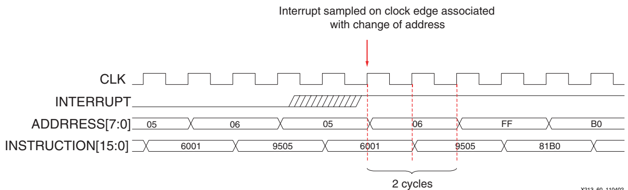
Figure 68: Interrupt Timing
