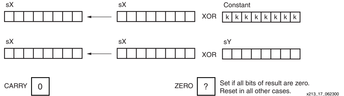
Figure 27: XOR Instruction
