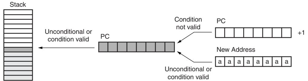
Figure 13: CALL Instruction
