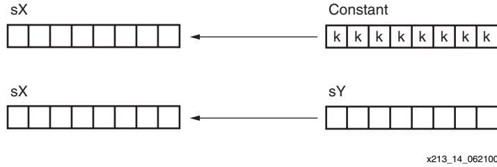
Figure 21: LOAD Instruction
