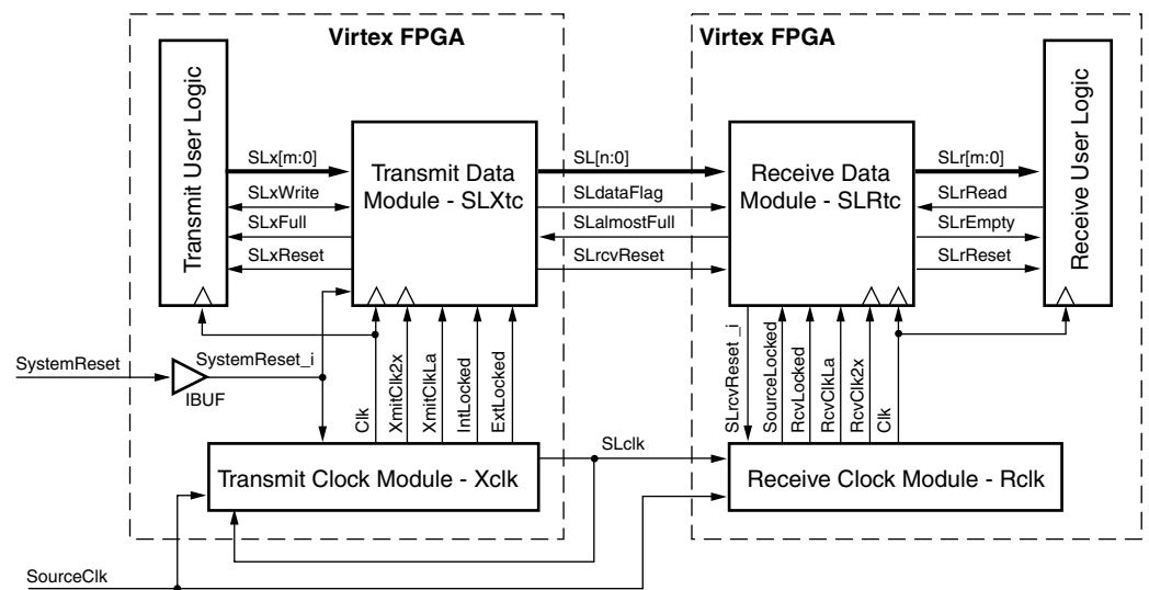
Figure 4: SelectLink Top-Level Modules and Interconnects
