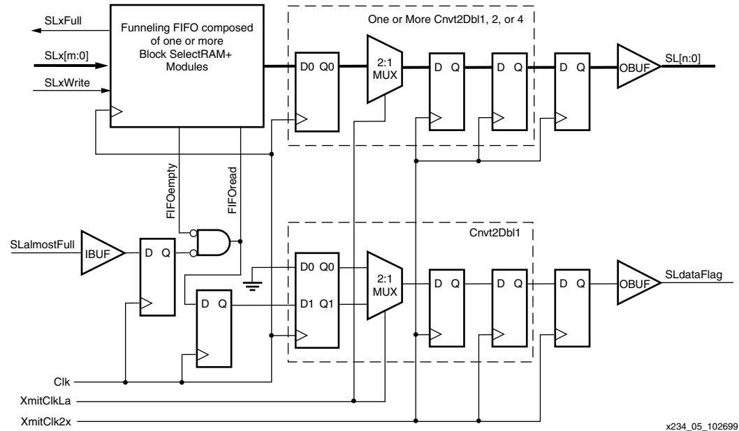
Figure 5: Module SLXtc
