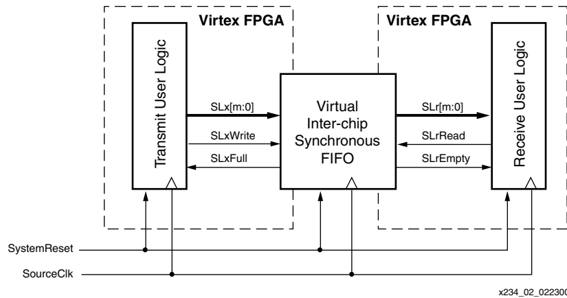
Figure 2: SelectLink Conceptual Diagram
