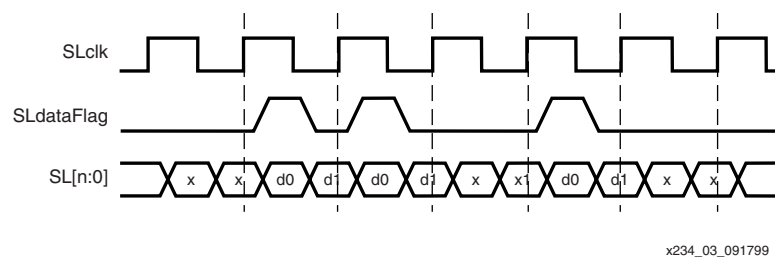
Figure 3: External Timing
