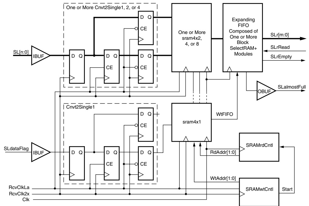
Figure 6: Module SLRtc
