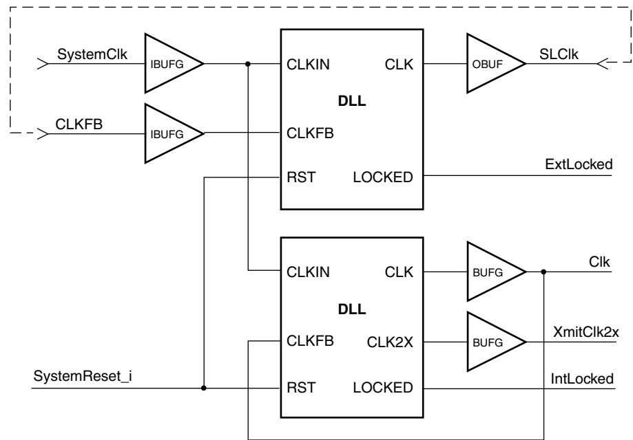
Figure 8: Xclk Detail
