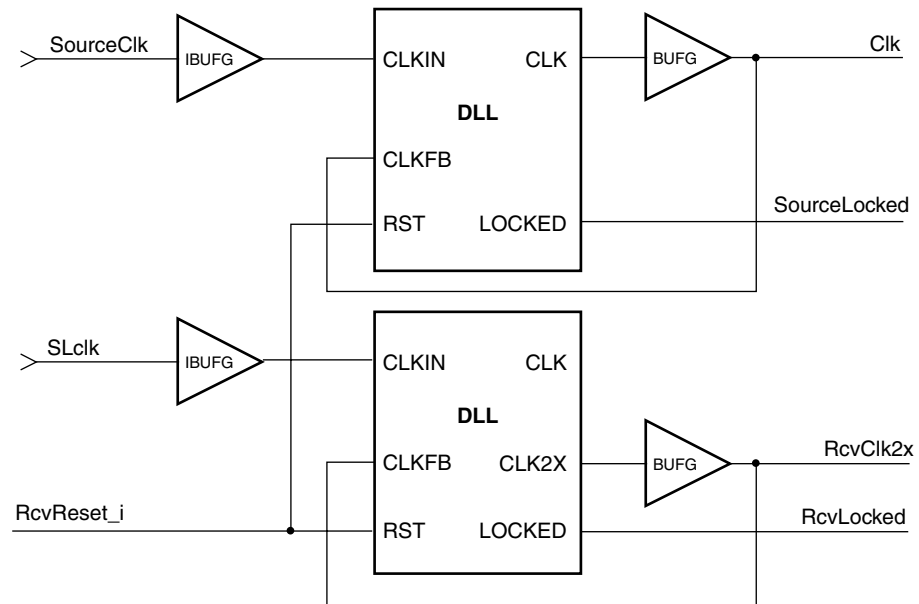
Figure 9: Rclk Detail
