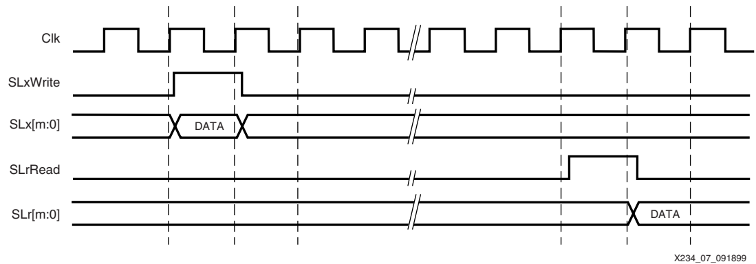
Figure 7: User Interface Write and Read Timing
