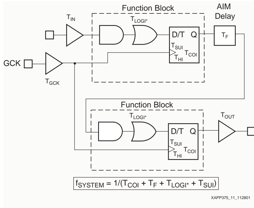
Figure 11: Multiple Logic Levels
