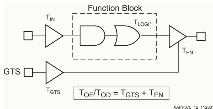
Figure 12: Global Output Enable Timing
