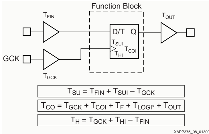
Figure 8: Direct Input Register Path
