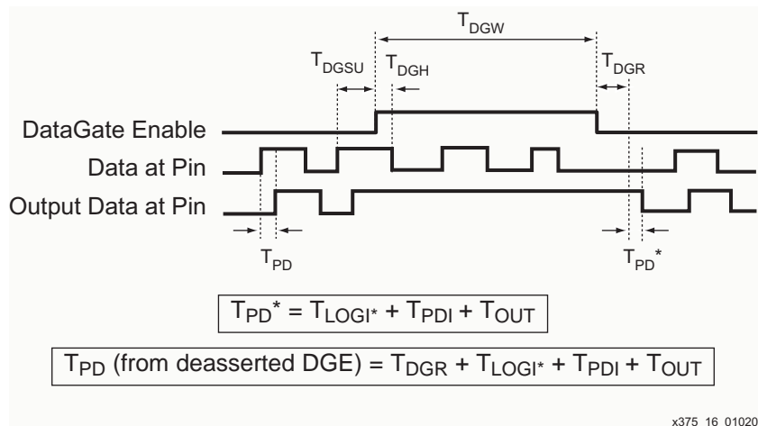
Figure 16: DataGate Timing Requirements
