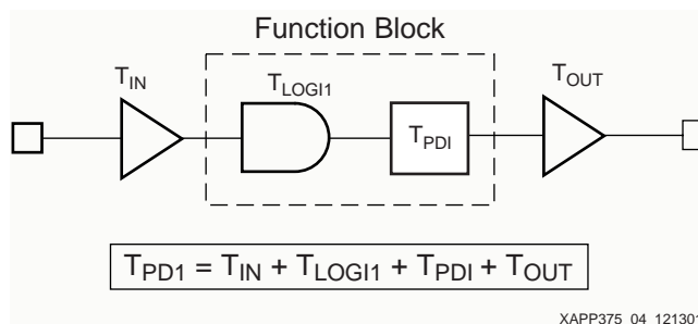
Figure 4: T_{PD1} with a Single Product Term
