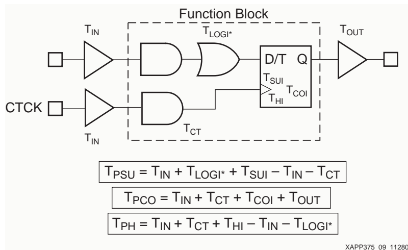
Figure 9: Product Term Clocking
