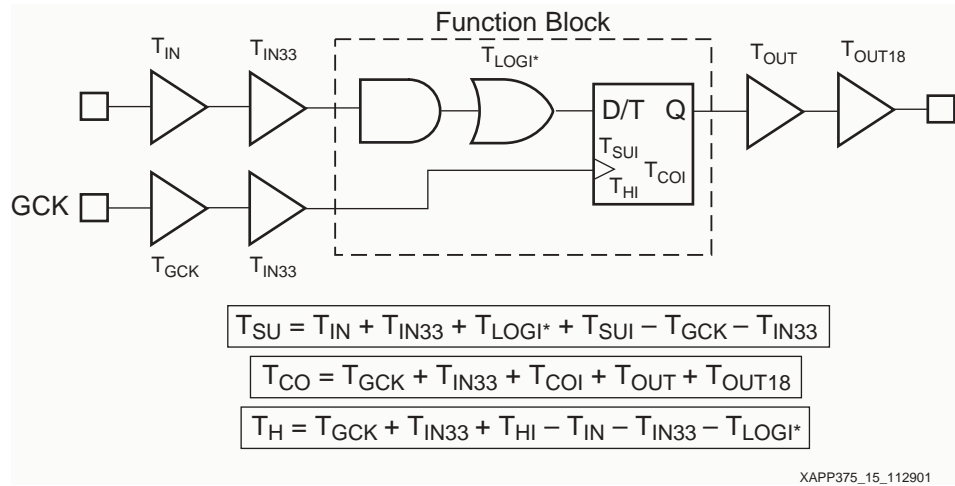
Figure 15: I/O Standard Timing Example
