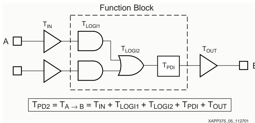
Figure 5: T_{PD2} with 2 to 56 Product Terms
