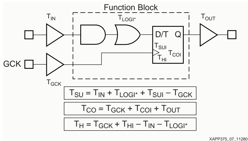
Figure 7: Simple Registered Path
