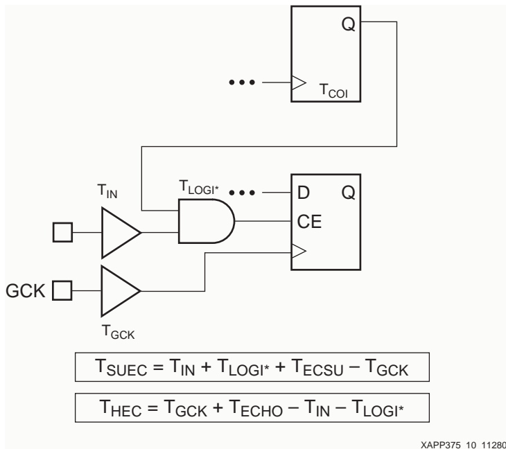
Figure 10: Clock Enable Timing Parameters
