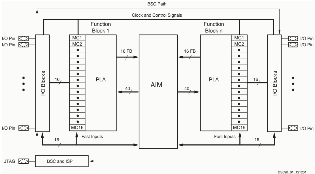
Figure 1: CoolRunner-II Architecture
