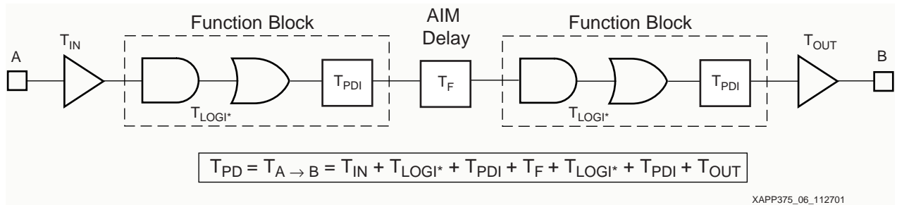
Figure 6: T_{PD} with 2 Levels of Logic
