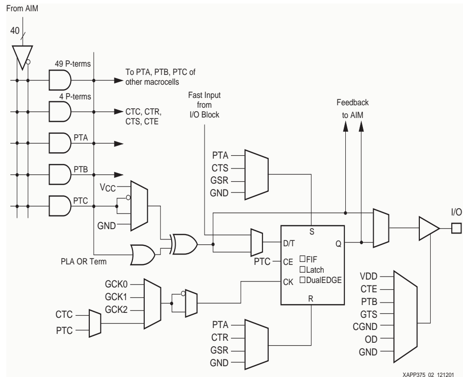
Figure 2: CoolRunner-II Macrocell
