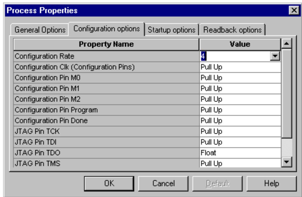
Figure 13: Configuration Options for Virtex or Spartan-II Devices
