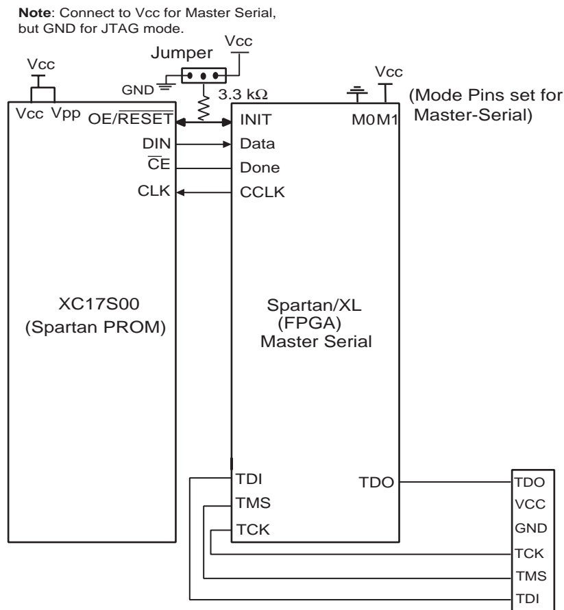
Figure 8: Spartan-XL Master-Serial/JTAG Mode Connections
