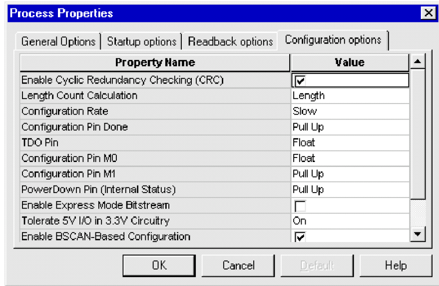
Figure 10: Spartan-XL Configuration Options in the Foundation ISE Software Package
