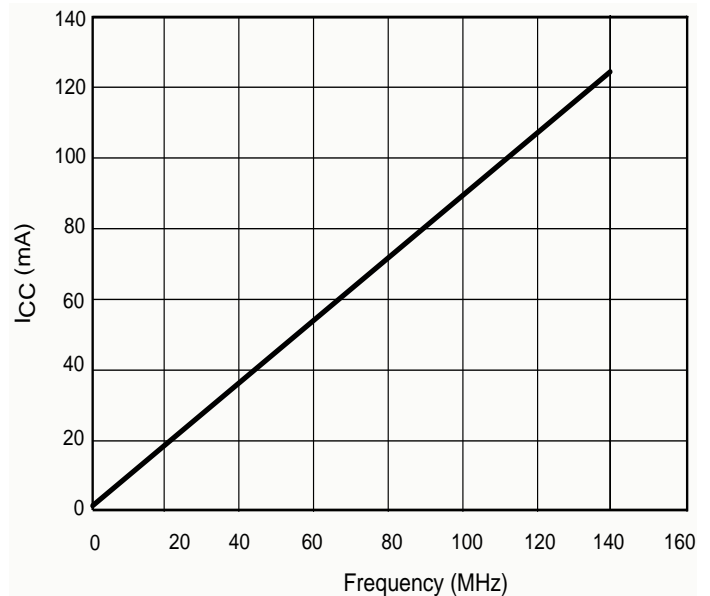
Figure 1: XCR3256XL Typical I_{CC} vs. Frequency at V_{CC} = 3.3V, 25^{\circ}C
