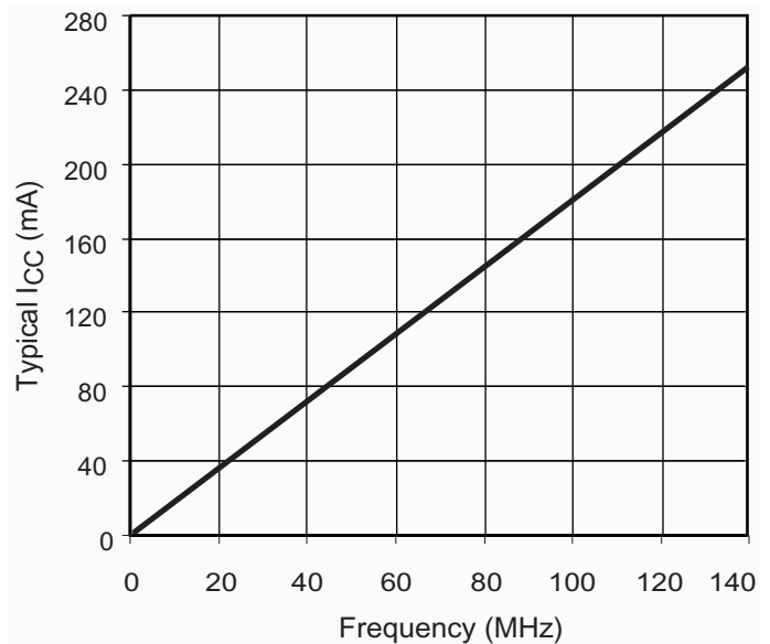
Figure 1: XCR3384XL Typical I_{CC} vs. Frequency at V_{CC} = 3.3V, 25^{\circ}C
