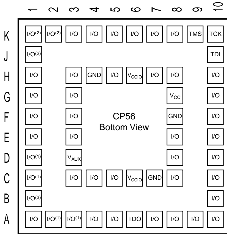
Figure 9: VQ44 Package
