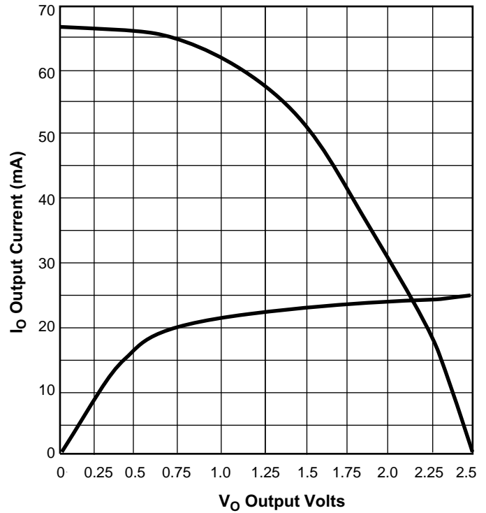
Figure 6: Typical I/O Output for LVC MOS25
