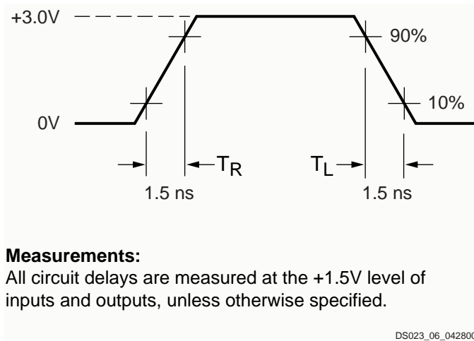
Figure 4: Typical Voltage Waveform
