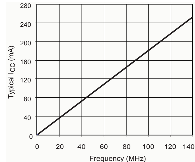
Figure 1: XCR3384XL Typical I CC vs. Frequency at V CC = 3.3V, 25°C
