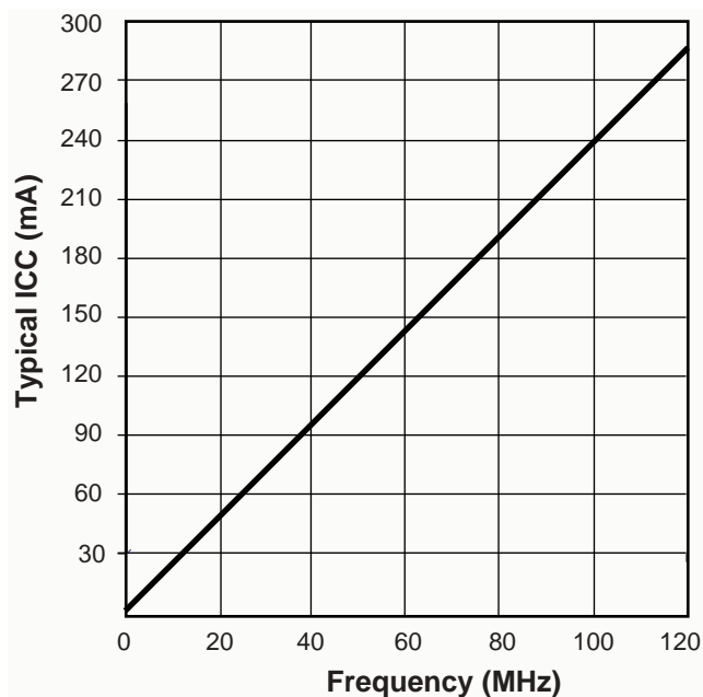
Figure 1: XCR3512XL Typical I_{CC} vs. Frequency at V_{CC} = 3.3\text{V} , 25^\circ\text{C}
