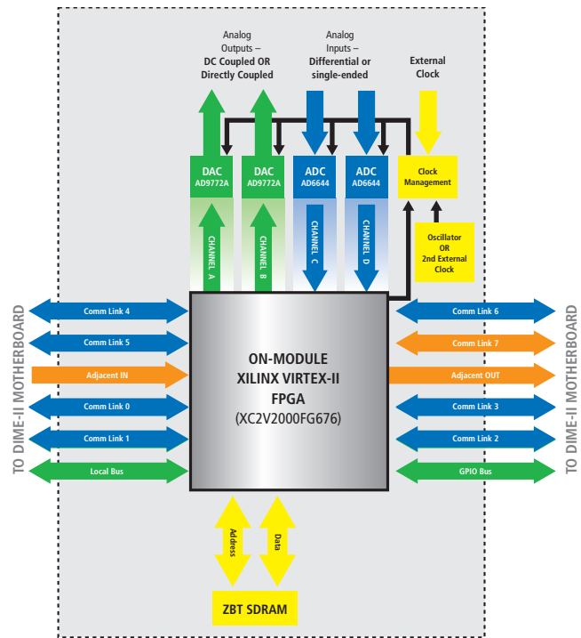
Dime II module functional diagram
