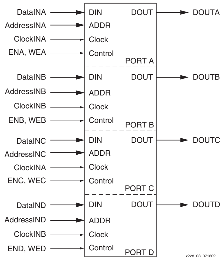
Figure 3: Four-Port Functionality
