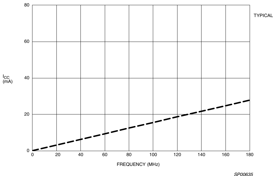
Figure 5: I_{CC} vs. Frequency at V_{CC} = 5V, 25^{\circ}C
