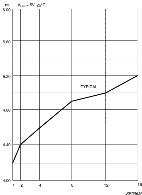
Figure 6: t_{PD\_PAL} vs. # Outputs Switching
