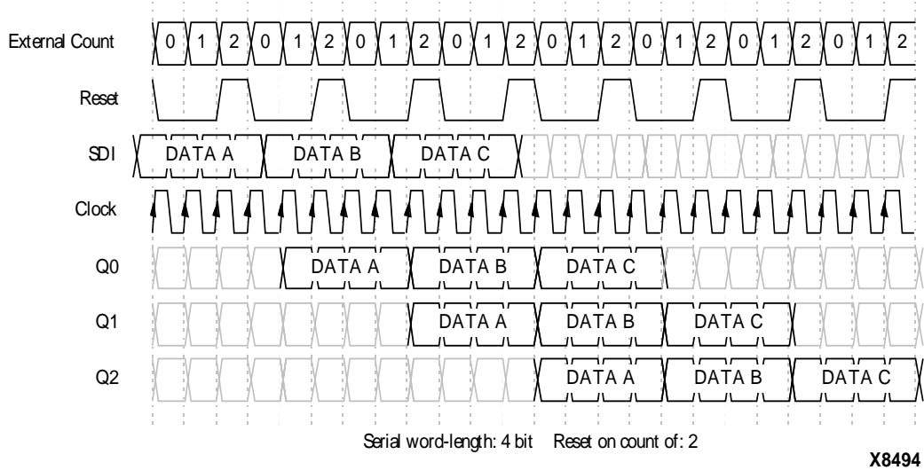
Figure 3: Timing Diagram Example Showing 3 Delay Stages of 4-bit Data
