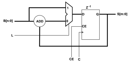
Figure 1: Block Diagram
