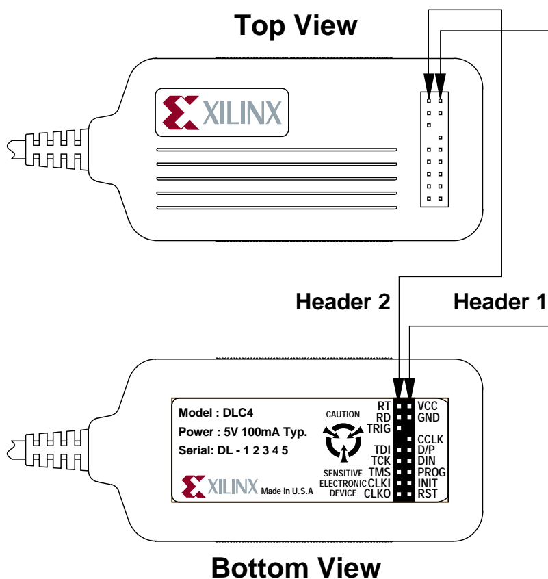
Figure 1-10 XChecker Cable
