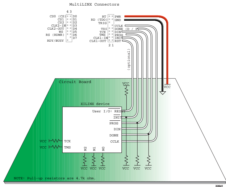
Figure 2-4 Slave Serial Mode (Virtex, Spartan, XC5200, XC4000)
