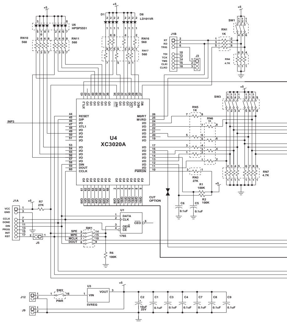
Figure 3-7 XC3020A Schematic
