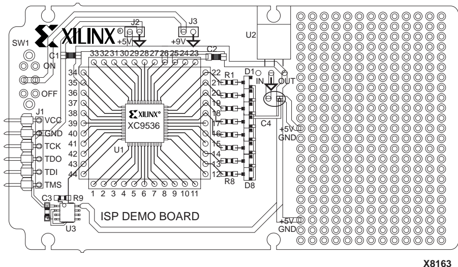
Figure 4-2 CPLD ISP Demonstration Board
