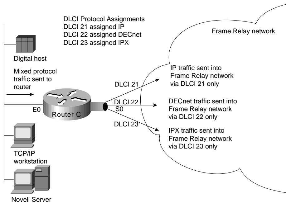
Figure 9-12 Virtual interfaces assigned specific protocols.
