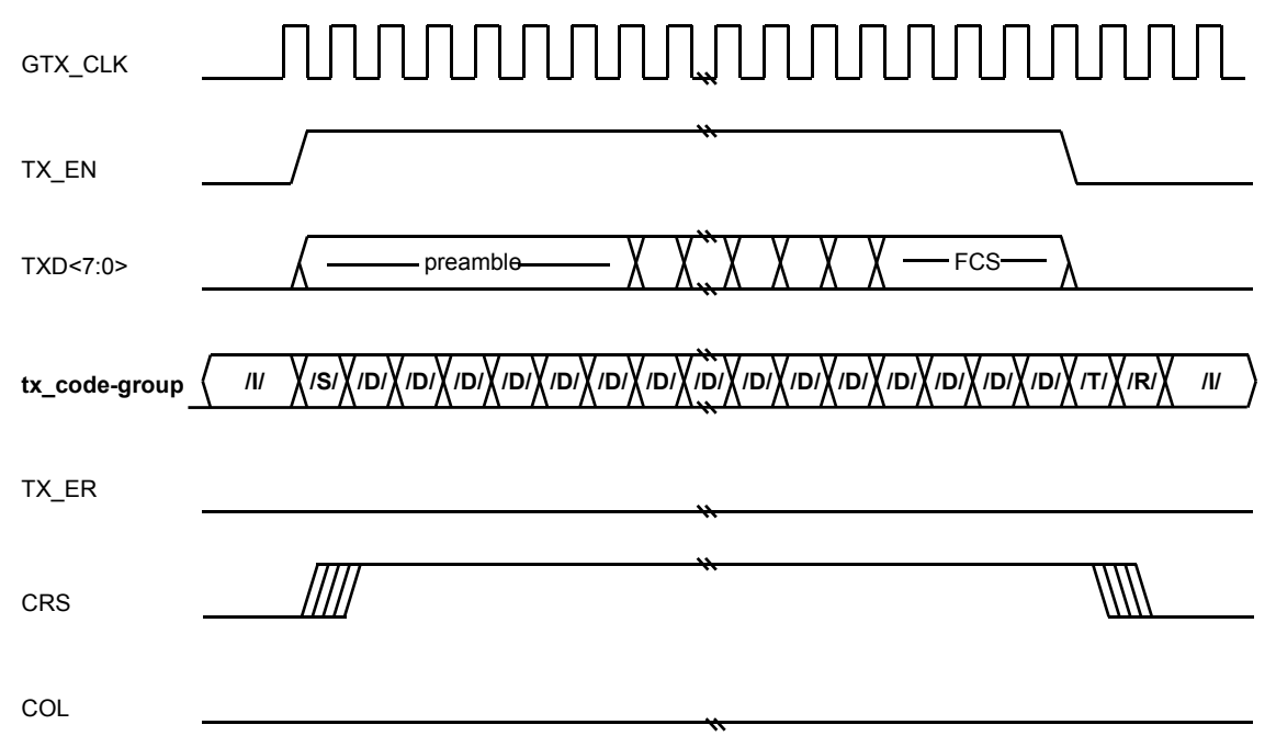
Figure 36–4—PCS encapsulation
