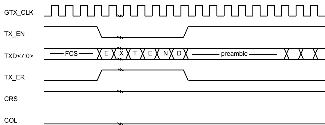
Figure 35–7—Burst transmission
