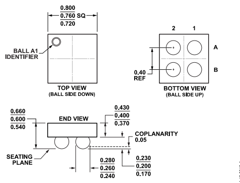
Figure 50. 4-Ball Wafer Level Chip Scale Package [WLCSP] (CB-4-3)
