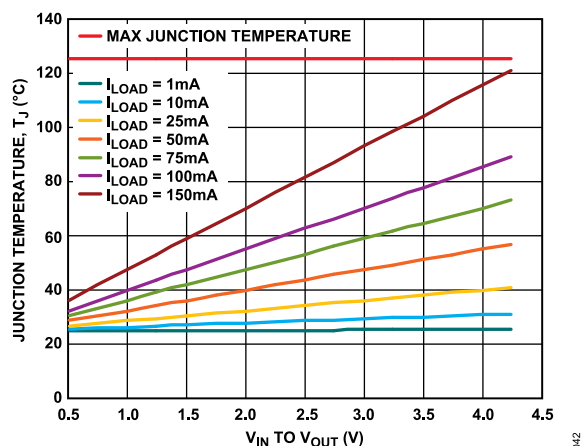
Figure 40. WLCSP, 500 mm² of PCB Copper, T_A = 25^\circ\text{C}
