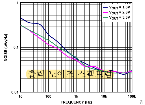
Figure 21. Output Noise Spectrum, V_{IN} = 5\text{ V} , I_{LOAD} = 10\text{ mA} , C_{OUT} = 1\text{ }\mu\text{F}
