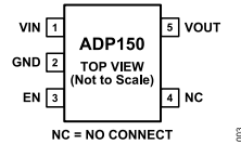
Figure 3. 5-Lead TSOT Pin Configuration
