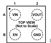
Figure 4. 4-Ball WLCSP Pin Configuration
