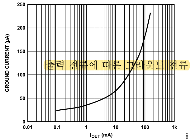
Figure 9. Ground Current vs. Load Current ( I_{OUT} )
