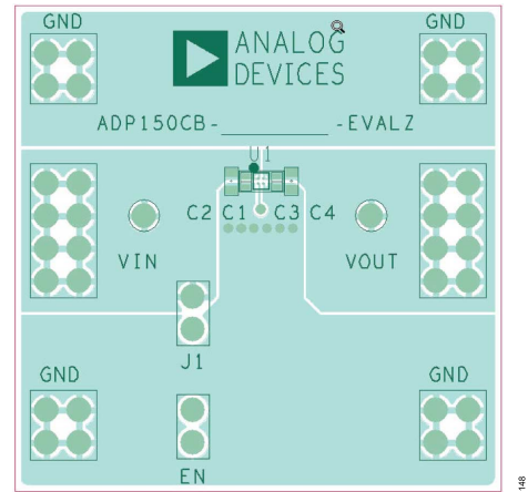
Figure 48. Example WLCSP PCB Layout
