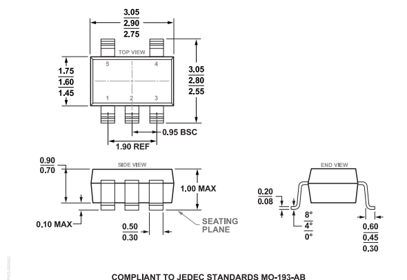
Figure 49. 5-Lead Thin Small Outline Transistor Package [TSOT] (UJ-5)
