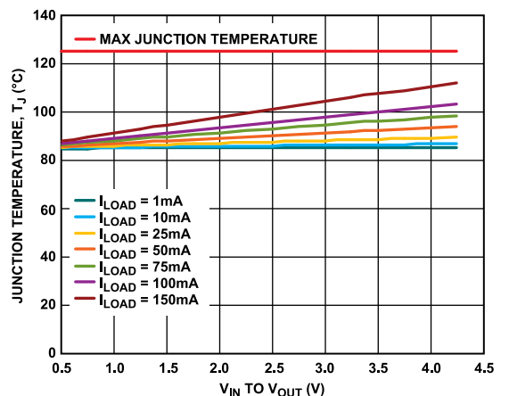
Figure 39. TSOT, 100 mm 2 of PCB Copper, Board Temperature = 85^\circ\text{C}
