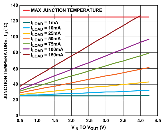
Figure 35. TSOT, 0 mm 2 of PCB Copper, T_A = 25^\circ\text{C}
