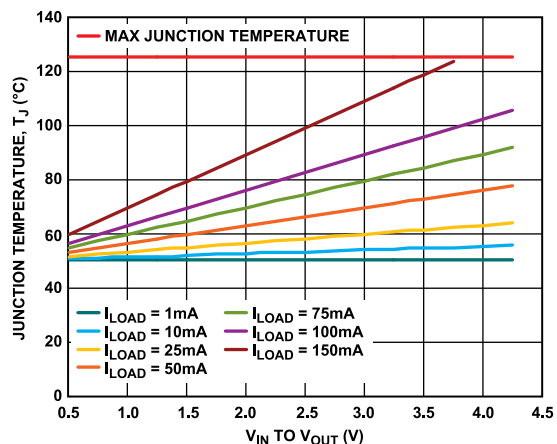
Figure 36. TSOT, 500 mm 2 of PCB Copper, T_A = 50^\circ\text{C}
