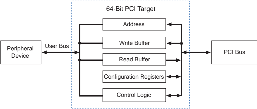
Figure 9. 64-Bit PCI Target Megafunction Block Diagram
