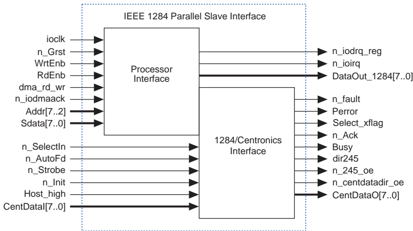
Figure 16. IEEE 1284 Parallel Slave Interface Megafunction Block Diagram
