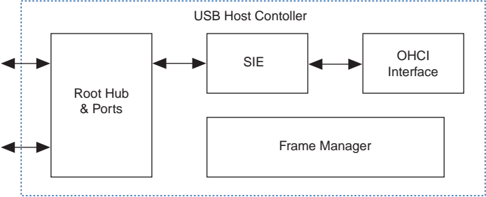
Figure 24. USB Host Controller Megafunction Block Diagram
