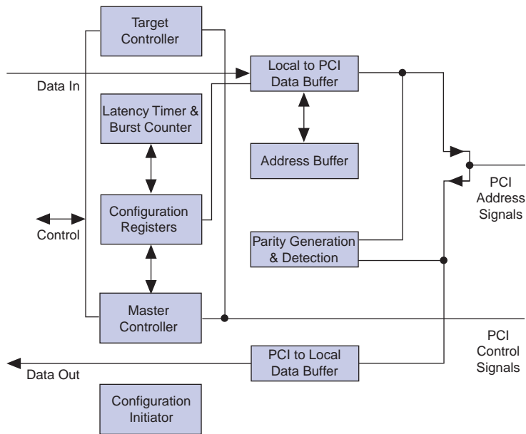
Figure 11. PCI Host Bridge Megafunction Block Diagram
