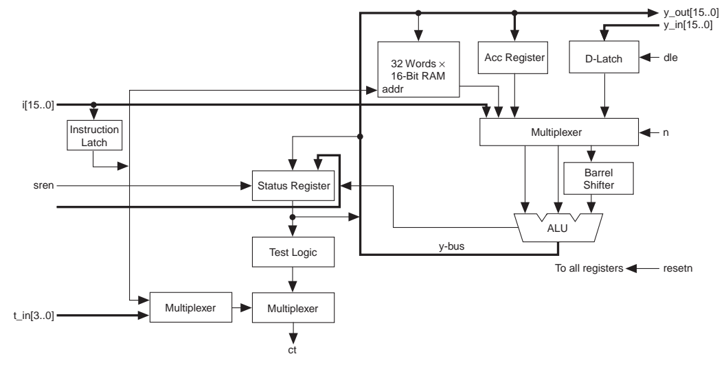
Figure 25. 29116A 16-Bit Microprocessor Block Diagram
