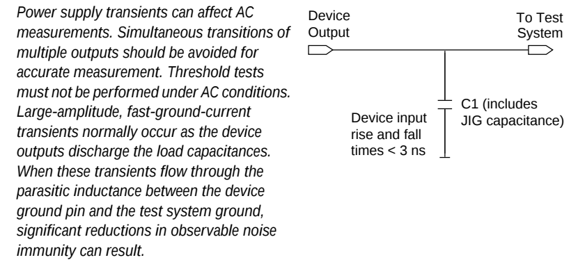
Figure 33. APEX 20K AC Test Conditions
