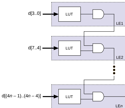
AND Cascade Chain
