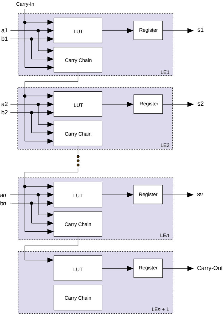
Figure 6. APEX 20K Carry Chain
