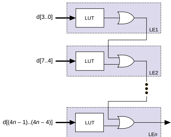
OR Cascade Chain
