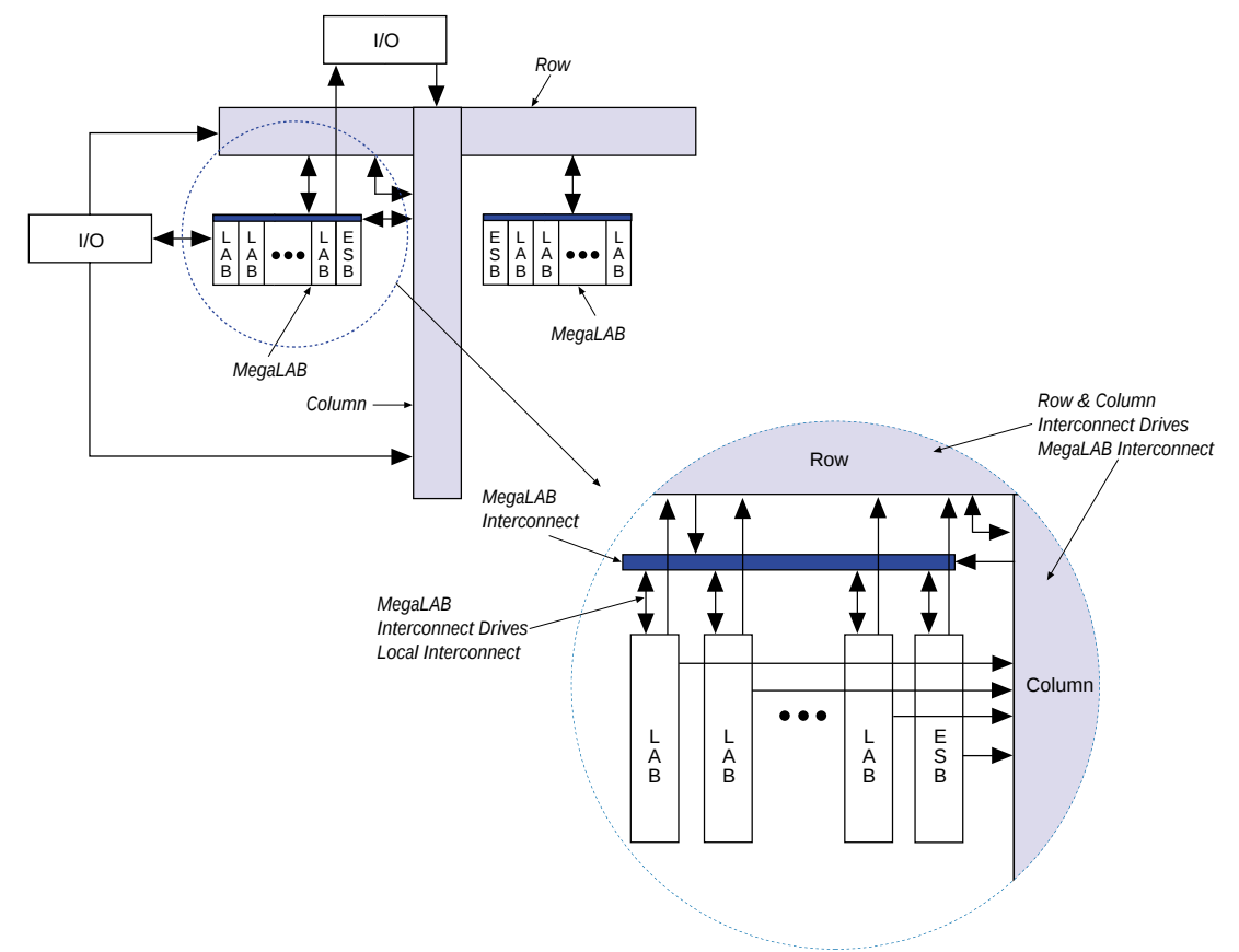
Figure 10. FastTrack Connection to Local Interconnect
