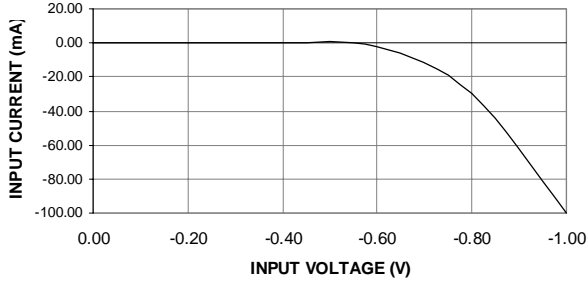
ATF22LV10C INPUT CLAMP CURRENT VS. INPUT VOLTAGE ( V_{CC} = 3.3V , T_A = 25C )
