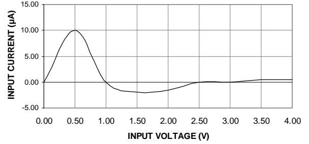
ATF22LV10C INPUT CURRENT VS. INPUT VOLTAGE ( V_{CC} = 3.3V , T_A = 25C )
