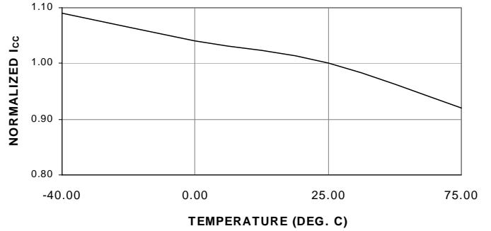
ATF22LV10C NORMALIZED I CC VS. TEMP.
