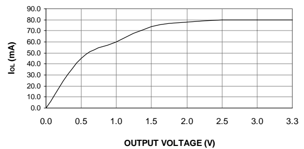
ATF22LV10C OUTPUT SINK CURRENT VS. OUTPUT VOLTAGE (V CC = 3.3V, TA = 25C)
