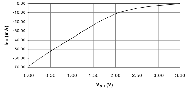
ATF22LV10C OUTPUT SOURCE CURRENT VS. OUTPUT VOLTAGE (V CC = 3.3V, TA = 25C)
