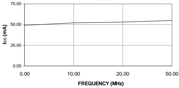
ATF22LV10C SUPPLY CURRENT VS. INPUT FREQUENCY (V CC = 3.3V, TA = 25C)
