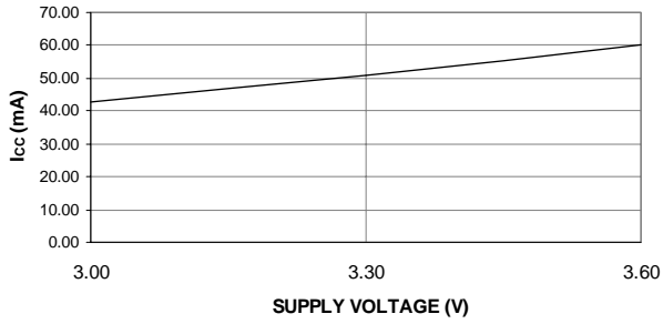
ATF22LV10C SUPPLY CURRENT VS. SUPPLY VOLTAGE (TA = 25C)
