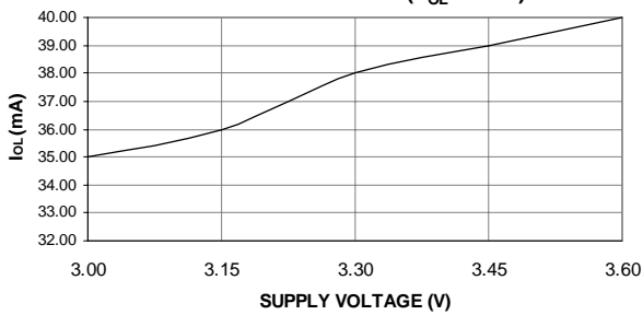
ATF22LV10C OUTPUT SINK CURRENT VS. SUPPLY VOLTAGE (V OL = 0.5V)
