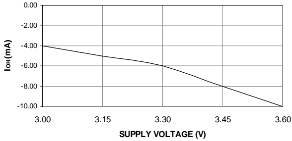
ATF22LV10C OUTPUT SOURCE CURRENT VS. SUPPLY VOLTAGE (V OH = 2.4V)
