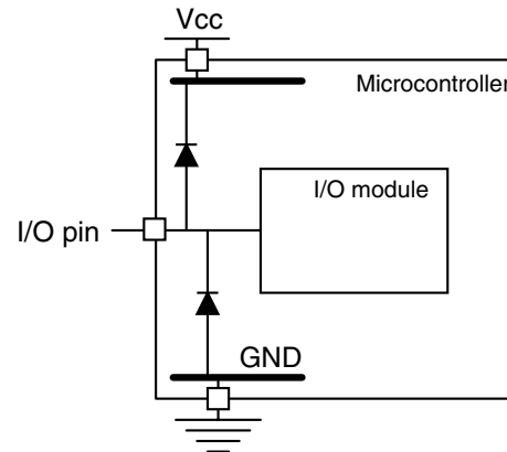
Figure 8. AVR I/O Pin Protection
