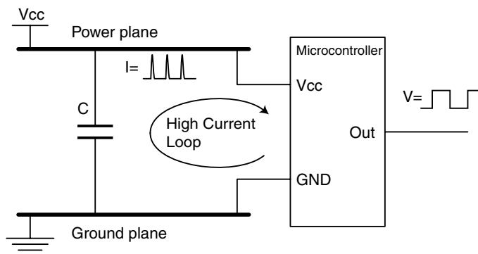
Figure 4. Incorrect Decoupling
