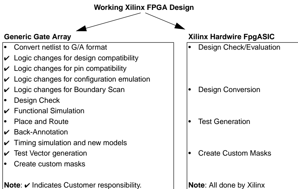
Figure 1: Steps Involved in Converting a PLD Design to a Gate Array as Compared to a HardWire FpgASIC
