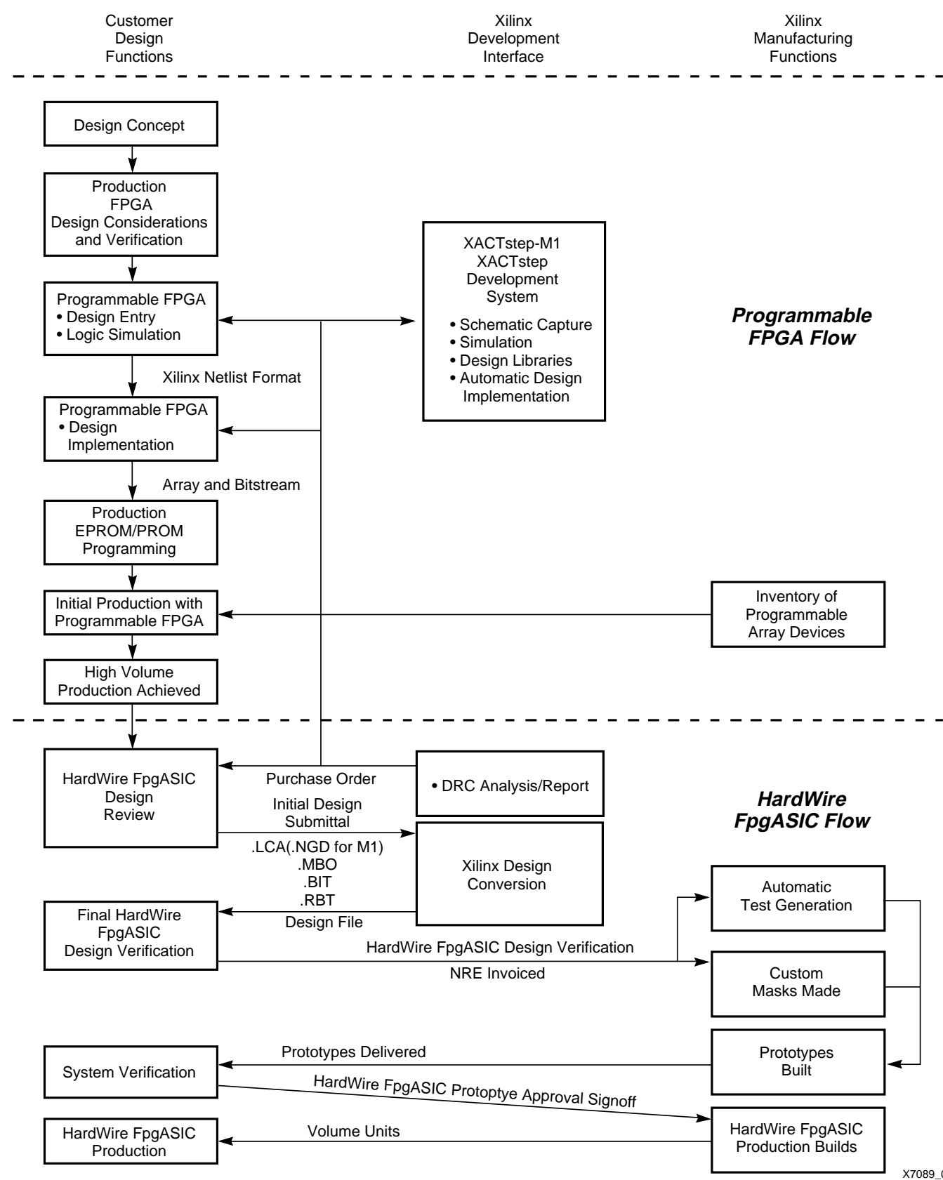
Figure 3: Programmable/HardWire Design/Production Interface
