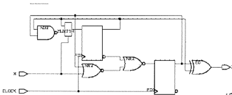
Figure A-2 Moore Machine Schematic
