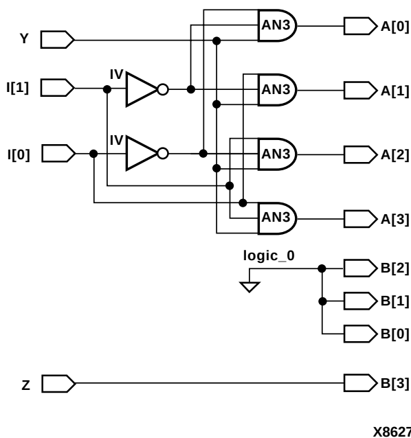
Figure 5-1 Design Illustrating Indexed Name Targets
