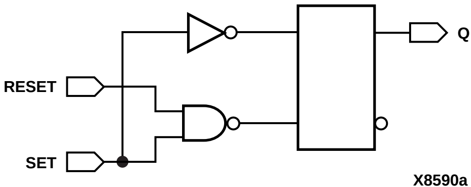
Figure 7-1 SR Latch
