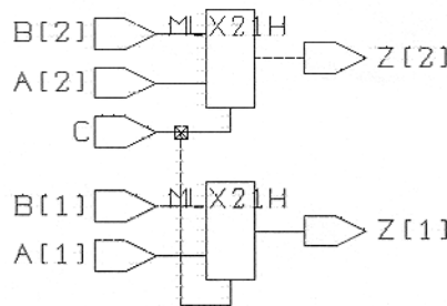
Figure 5-12 Circuit Design without Component Implication Directives
