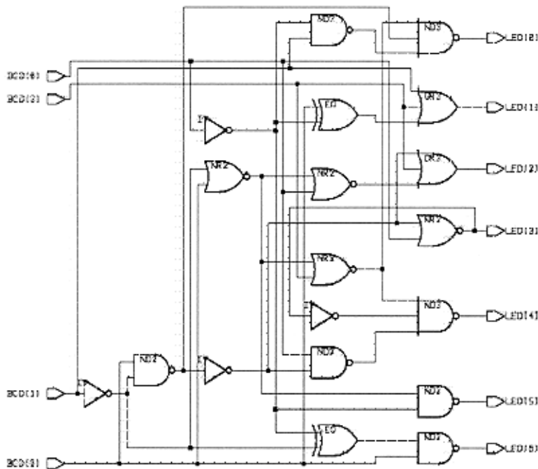
Figure 8-18 Seven-Segment LED Decoder with 0 LED Default
