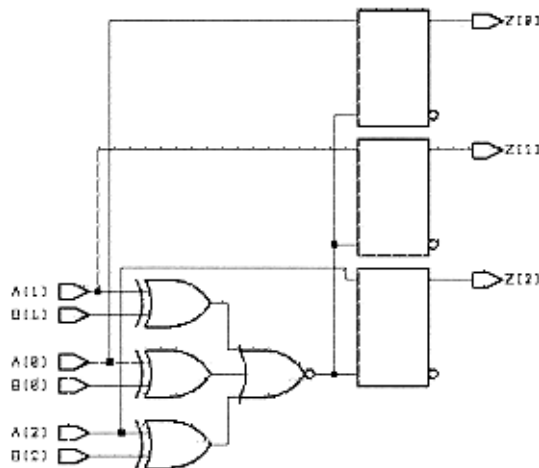
Figure 8-17 Schematic of Incorrect Asynchronous Design
