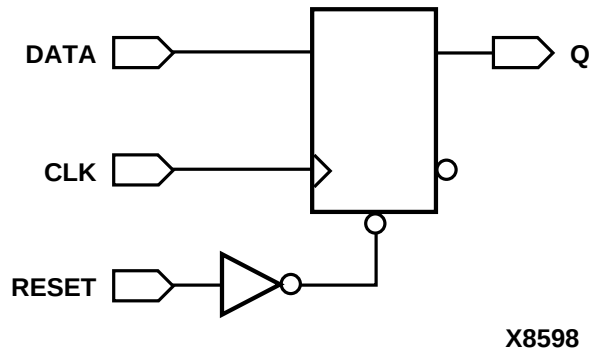
Figure 7-12 D Flip-Flop with Asynchronous Reset
