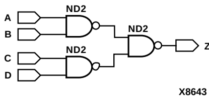
Figure 6-8 Simple Netlist Design
