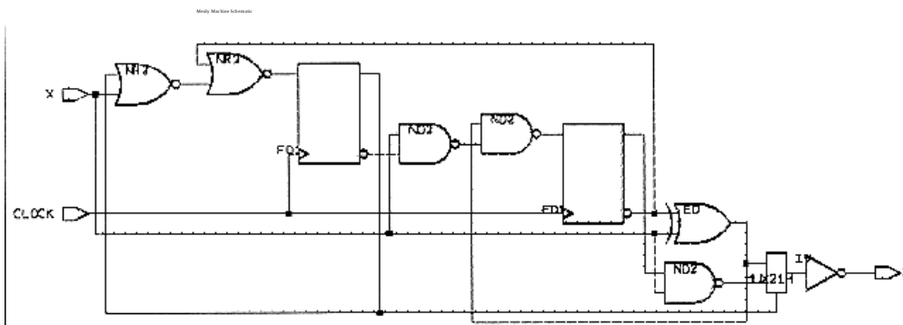
Figure A-5 Mealy Machine Schematic
