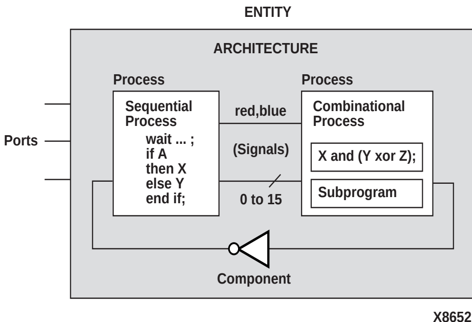
Figure 1-1 VHDL Hardware Model
