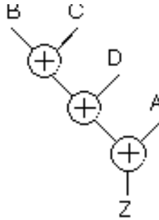
Figure 8-6 Expression Tree With Minimum Delay (Signal A Arrives Last)
