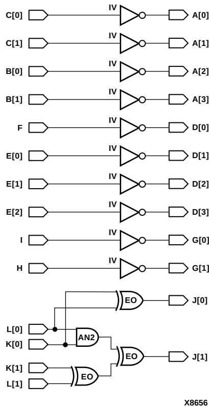
Figure 4-3 Circuits for Adding Operators
