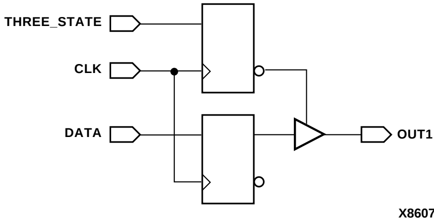
Figure 7-28 Three-State Driver with Registered Enable
