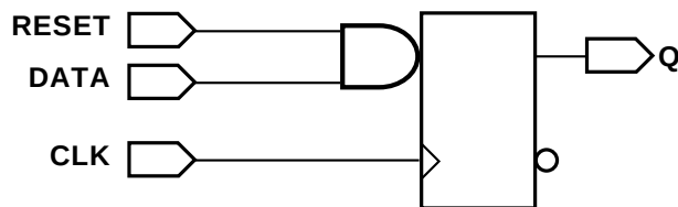
Figure 7-15 D Flip-Flop with Synchronous Reset
