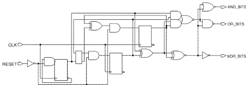
Figure 7-24 Circuit with Three Inferred Flip-Flops
