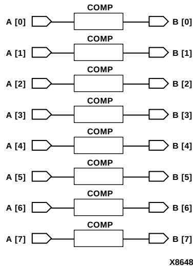
Figure 6-10 Design of COMP components Connecting Bit Vectors A and B
