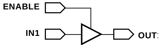
Figure 7-25 Simple Three-State Driver
