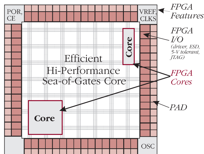
Figure 1: XH3 Architecture
