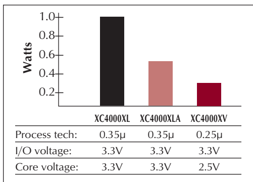
Figure 1: Relative Power Consumption
