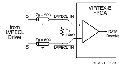
Figure 57: Receiving LVPECL Signal Circuit
