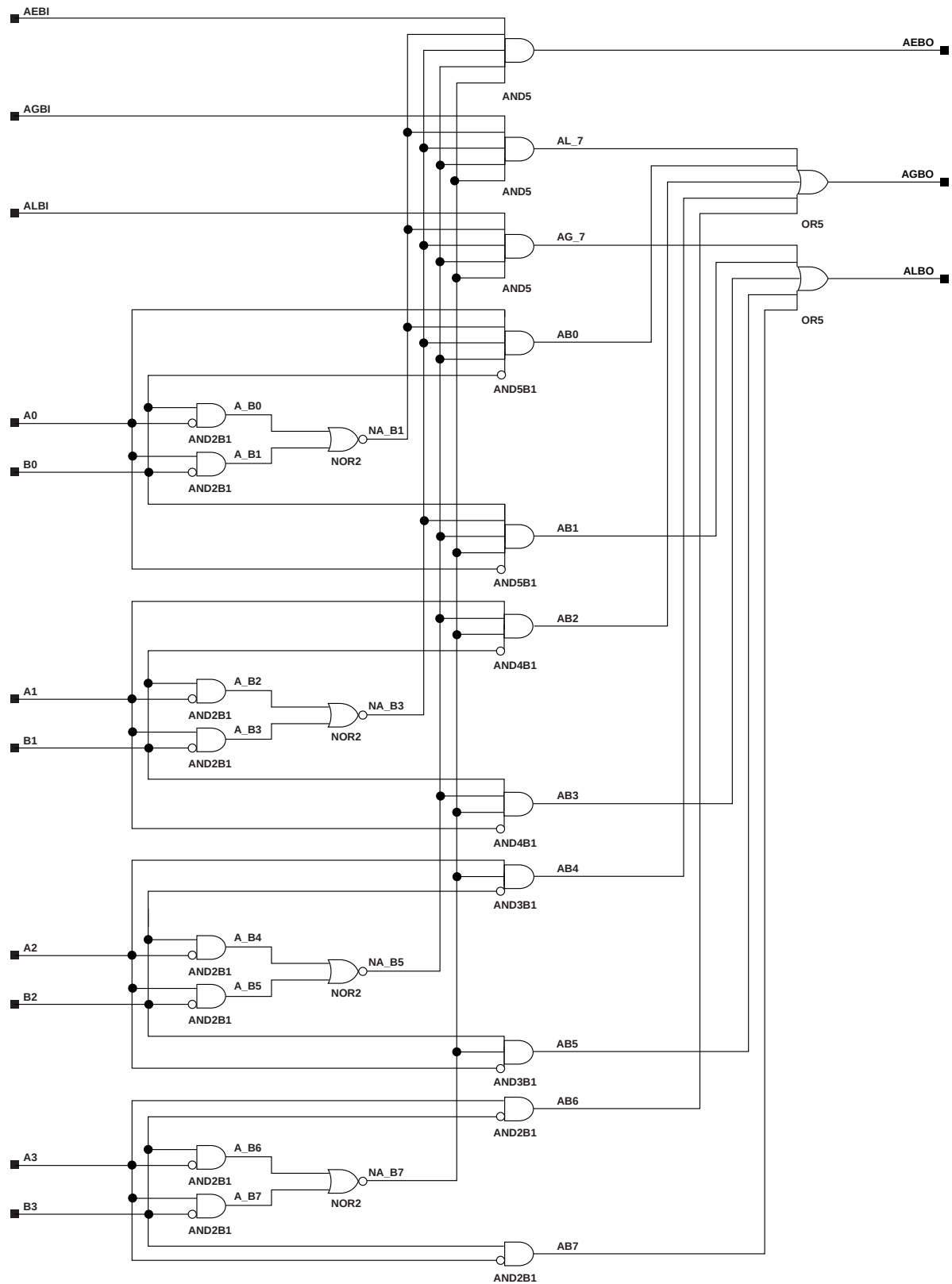
Figure 11-2 X74_L85 Implementation XC3000, XC4000E, XC4000X, XC5200, Spartan, SpartanXL
