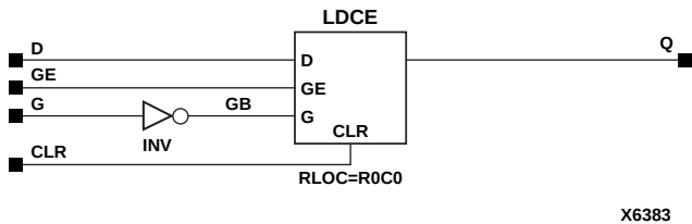
Figure 7-12 LDCE_1 Implementation XC5200
