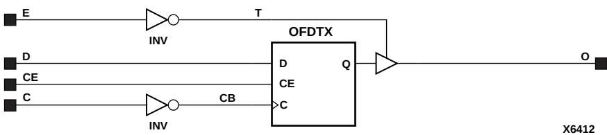
Figure 8-22 OFDEX_1 Implementation XC4000E, XC4000X, Spartan, SpartanXL
