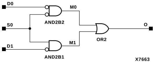
Figure 7-18 M2_1B2 Implementation XC3000, XC4000E, XC4000X, XC5200, XC9000, Spartan, SpartanXL, Spartan2, Virtex
