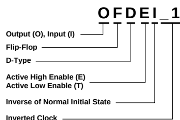
Figure 2-6 Input/Output Flip-Flop Naming Convention
