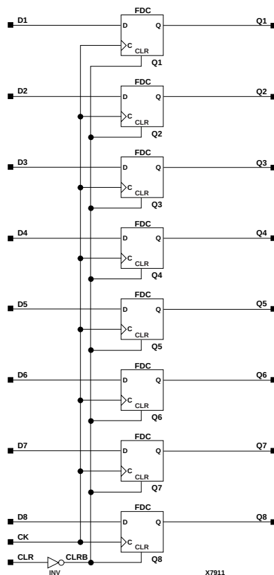
Figure 11-33 X74_273 Implementation XC3000, XC4000E, XC4000X, XC5200, XC9000, Spartan, SpartanXL
