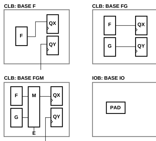
Figure 12-1 IOB and CLB Primitives for Base Configurations XC3000
