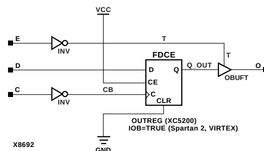
Figure 8-17 OFDE_1 Implementation XC5200, Spartan2, Virtex
