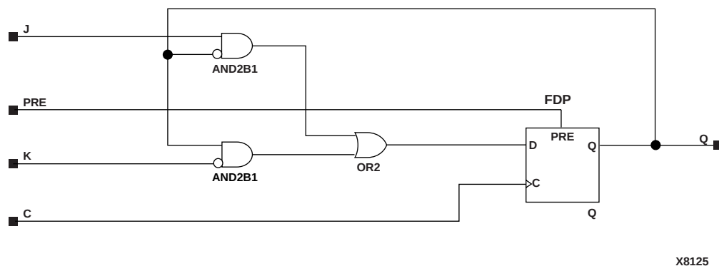
Figure 5-41 FJKP Implementation XC9000
