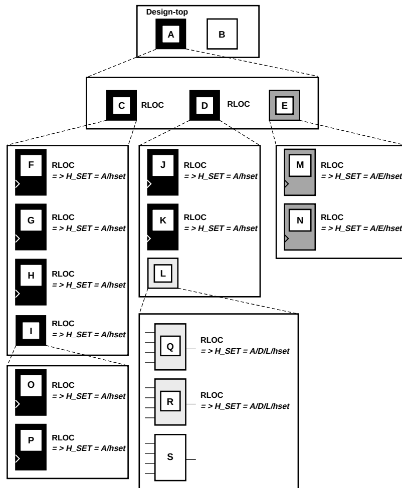
Figure 12-6 Three H_SET Sets
