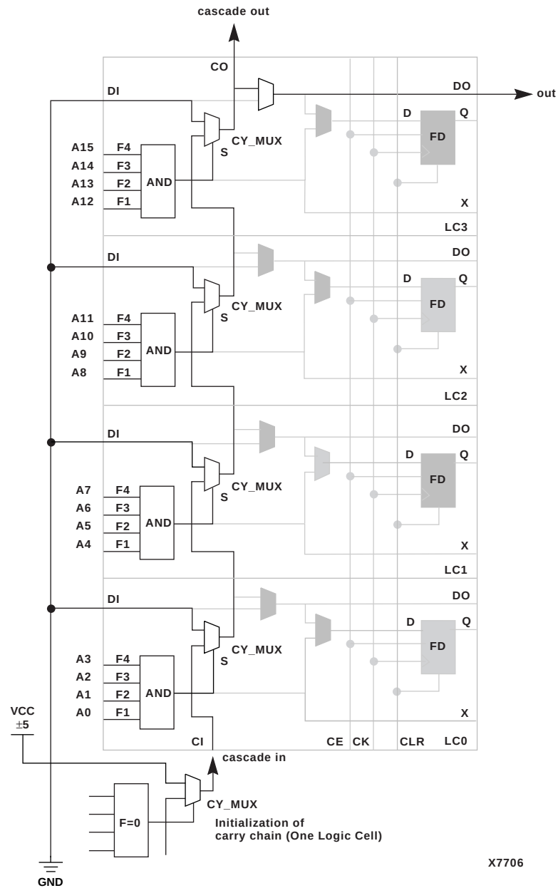
Figure 12-22 CY_MUX Used for Decoder Cascade Logic XC5200
