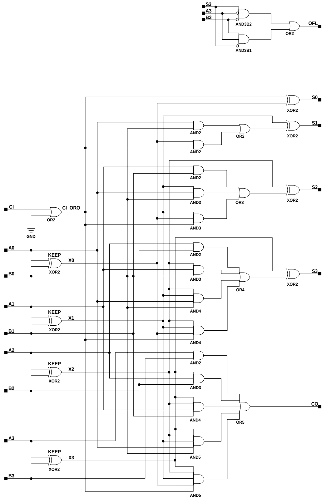
Figure 3-13 ADD4 Implementation XC9000
