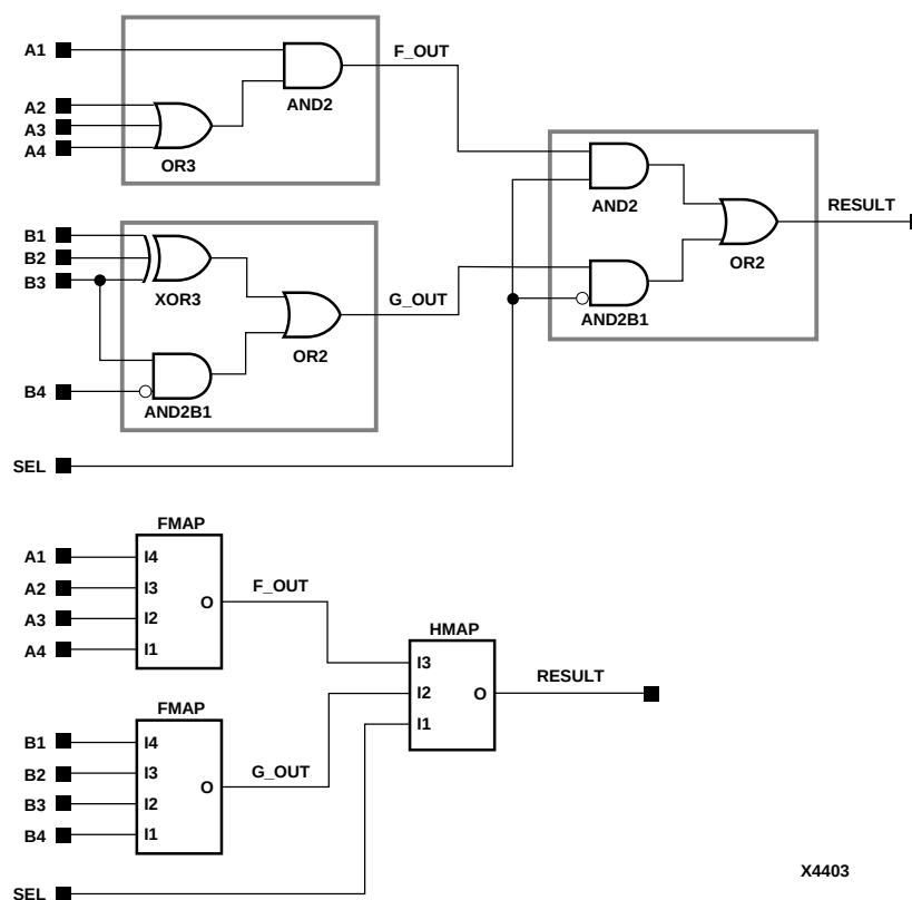
Figure 12-2 FMAP and HMAP Schematics
