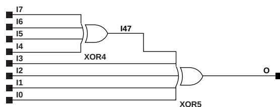
Figure 10-33 XOR8 Implementation XC3000
