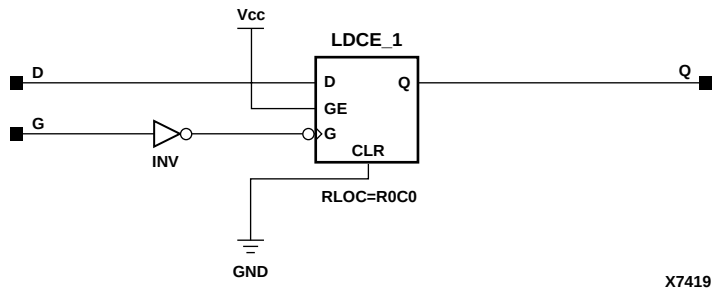
Figure 7-1 LD Implementation XC4000X, SpartanXL
