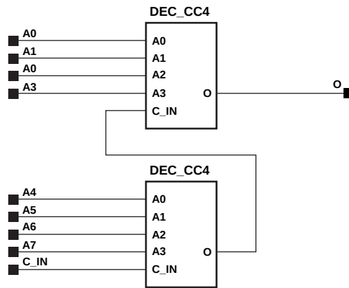
Figure 4-58 DEC_CC4 Implementation Spartan2, Virtex
