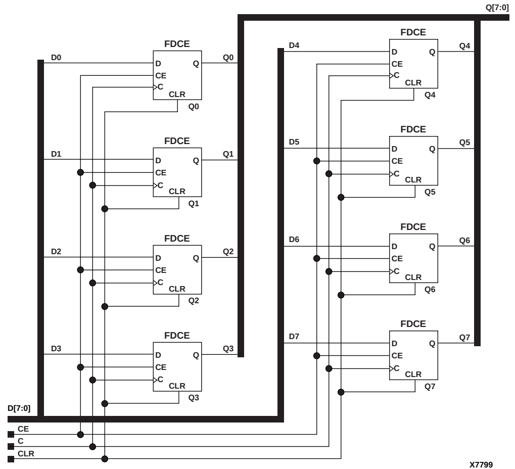
Figure 5-8 FD8CE Implementation XC3000, XC4000E, XC4000X, XC5200, XC9000, Spartan, SpartanXL, Spartan2, Virtex
