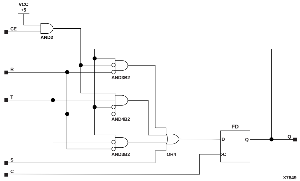
Figure 5-70 FTSRE Implementation XC9000
