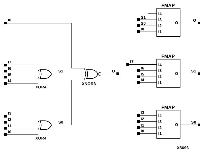
Figure 10-27 XNOR9 Implementation Spartan2, Virtex
