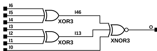
Figure 10-16 XNOR7 Implementation XC3000
