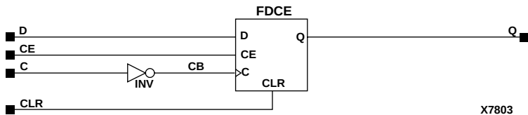
Figure 5-13 FDCE_1 Implementation XC3000, XC4000E, XC4000X, XC5200, Spartan, SpartanXL
