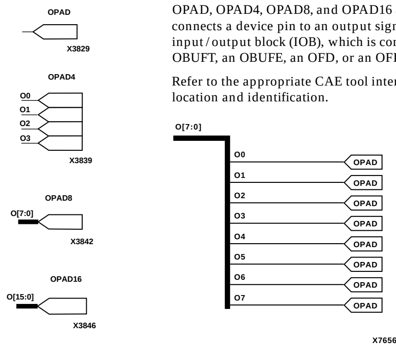
Figure 8-47 OPAD8 Implementation XC3000, XC4000E, XC4000X, XC5200, XC9000, Spartan, SpartanXL, Spartan2, Virtex
