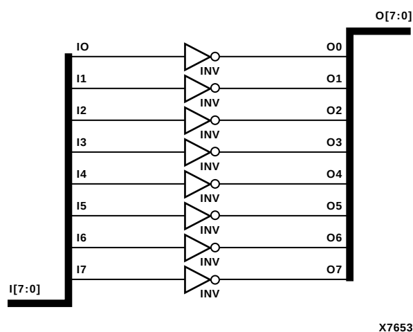
Figure 6-46 INV8 Implementation XC3000, XC4000E, XC4000X, XC5200, XC9000, Spartan, SpartanXL, Spartan2, Virtex
