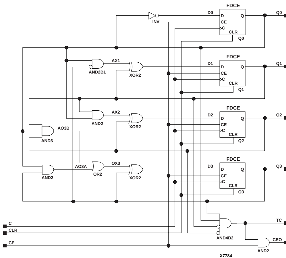
Figure 4-30 CD4CE Implementation XC3000, XC4000E, XC4000X, XC5200, Spartan, SpartanXL, Spartan2, Virtex
