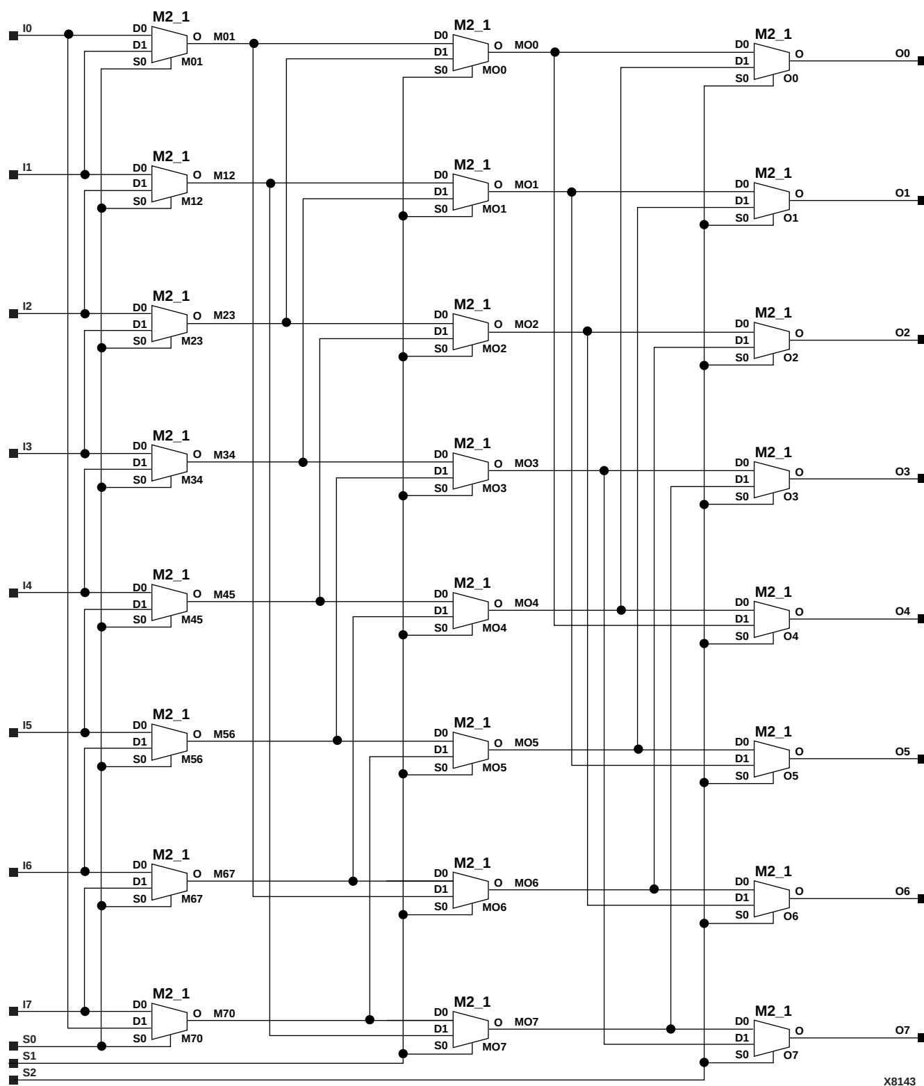
Figure 3-33 BRLSHFT8 Implementation XC3000, XC4000E, XC4000X, XC5200, XC9000, Spartan, SpartanXL, Spartan2, Virtex
