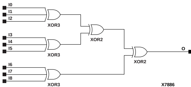
Figure 10-37 XOR9 Implementation XC9000
