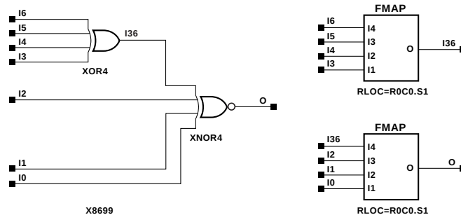
Figure 10-19 XNOR7 Implementation Spartan2, Virtex
