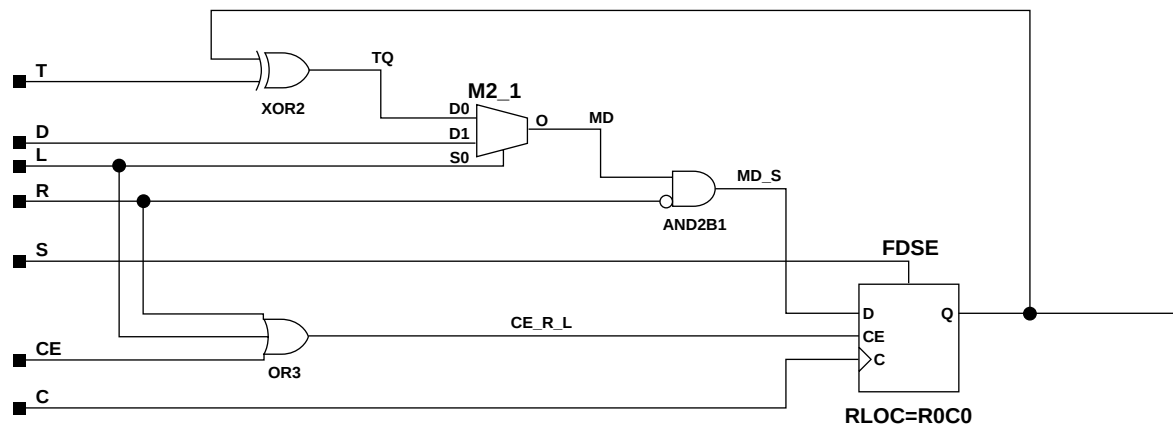
Figure 5-71 FTSRLE Implementation XC3000, XC4000E, XC4000X, XC5200, Spartan, SpartanXL, Spartan2, Virtex
