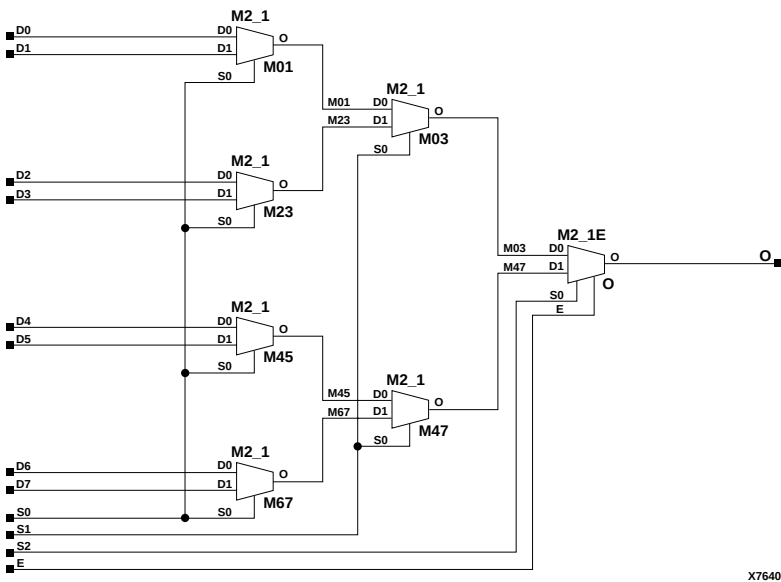
Figure 7-22 M8_1E Implementation XC3000, XC4000E, XC4000X, XC5200, XC9000, Spartan, SpartanXL
