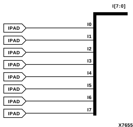
Figure 6-49 IPAD8 Implementation XC3000, XC4000E, XC4000X, XC5200, XC9000, Spartan, SpartanXL, Spartan2, Virtex
