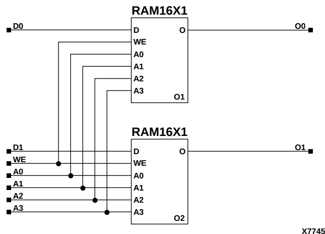
Figure 9-1 RAM16X2 Implementation XC4000E, XC4000X
