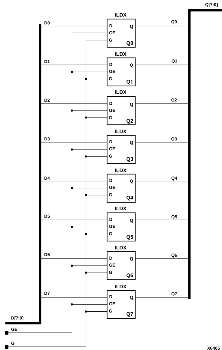
Figure 6-38 ILDX8 Implementation XC4000E, XC4000X, Spartan, SpartanXL, Spartan2, Virtex
