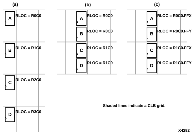
Figure 12-4 Different RLOC Specifications for Four Flip-flop Primitives for an XC4000, Spartan, or SpartanXL Design
