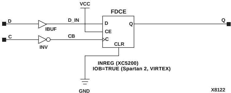
Figure 6-9 IFD_1 Implementation XC5200, Spartan2, Virtex
