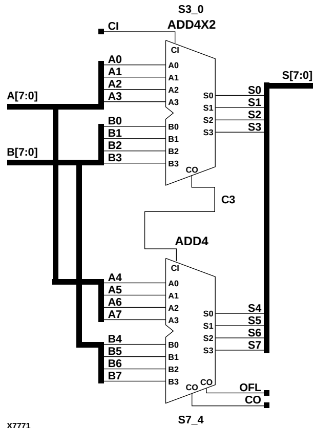
Figure 3-14 ADD8 Implementation XC9000
