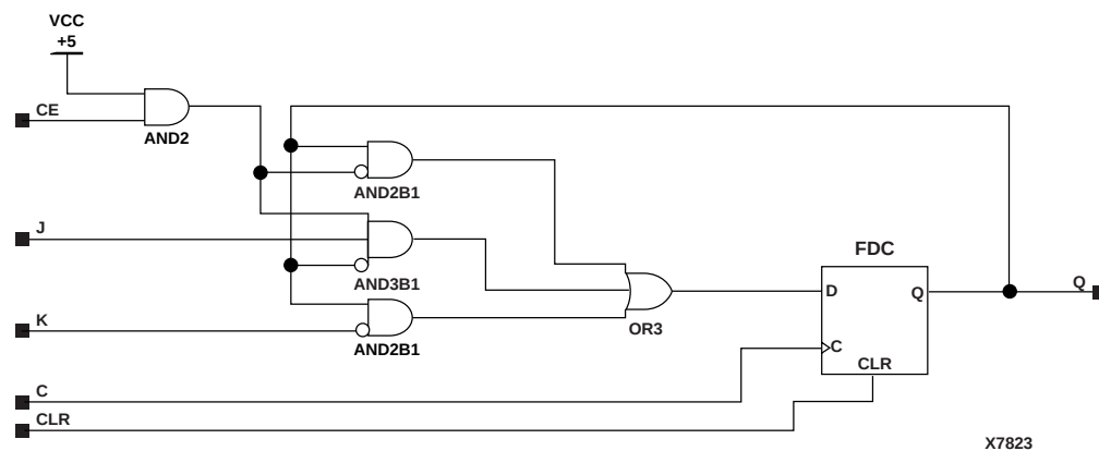
Figure 5-37 FJKCE Implementation XC9000
