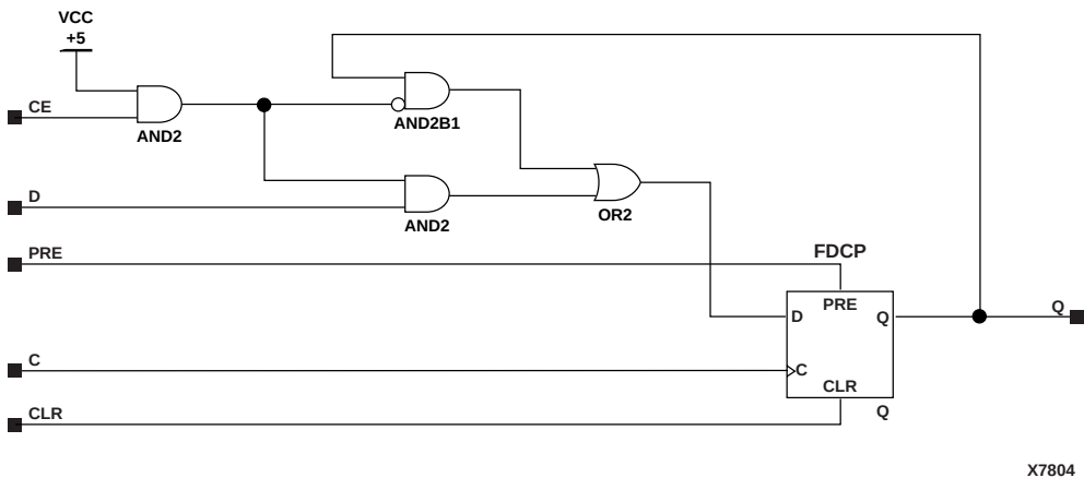
Figure 5-14 FDCPE Implementation XC9000
