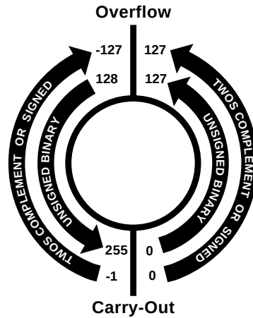
Figure 3-16 ADSU Carry-Out and Overflow Boundaries
