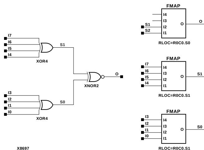
Figure 10-23 XNOR8 Implementation Spartan2, Virtex
