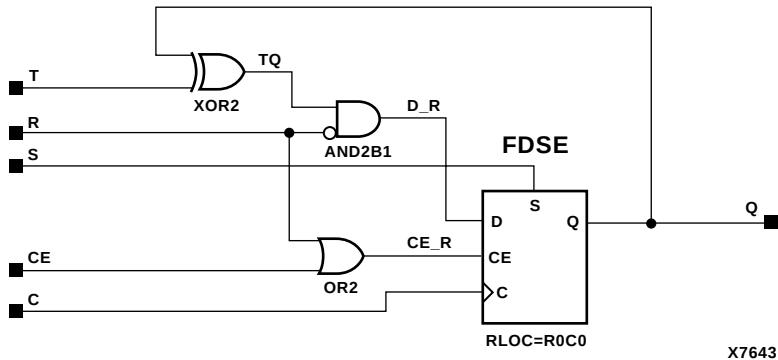
Figure 5-69 FTSRE Implementation XC3000, XC4000E, XC4000X, XC5200, Spartan, SpartanXL, Spartan2, Virtex
