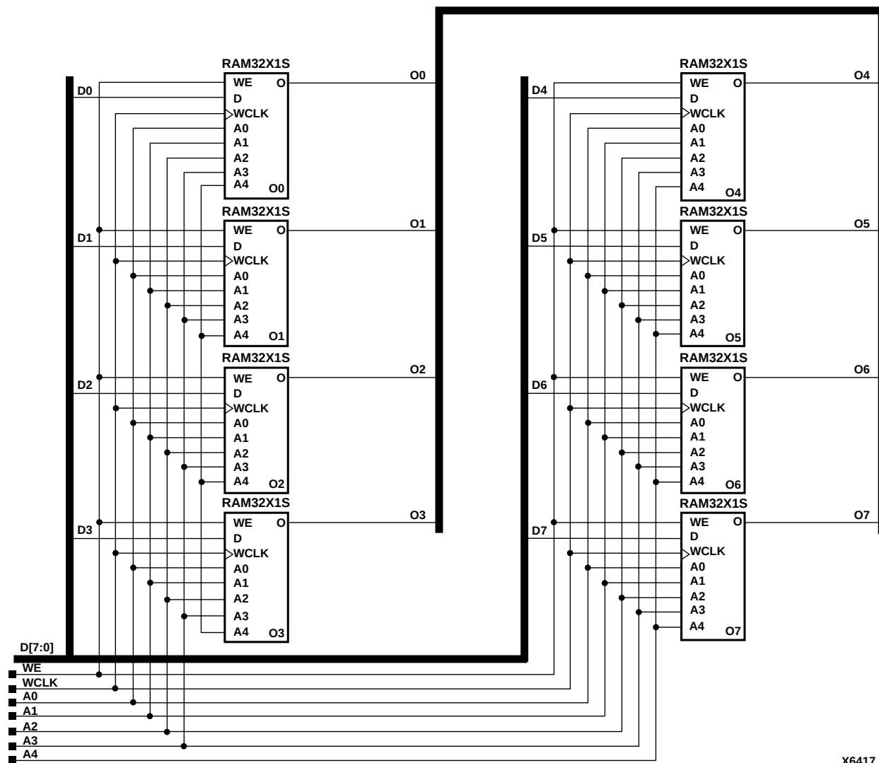
Figure 9-7 RAM32X8S Implementation XC4000E, XC4000X, Spartan, Spartan2, SpartanXL, Virtex
