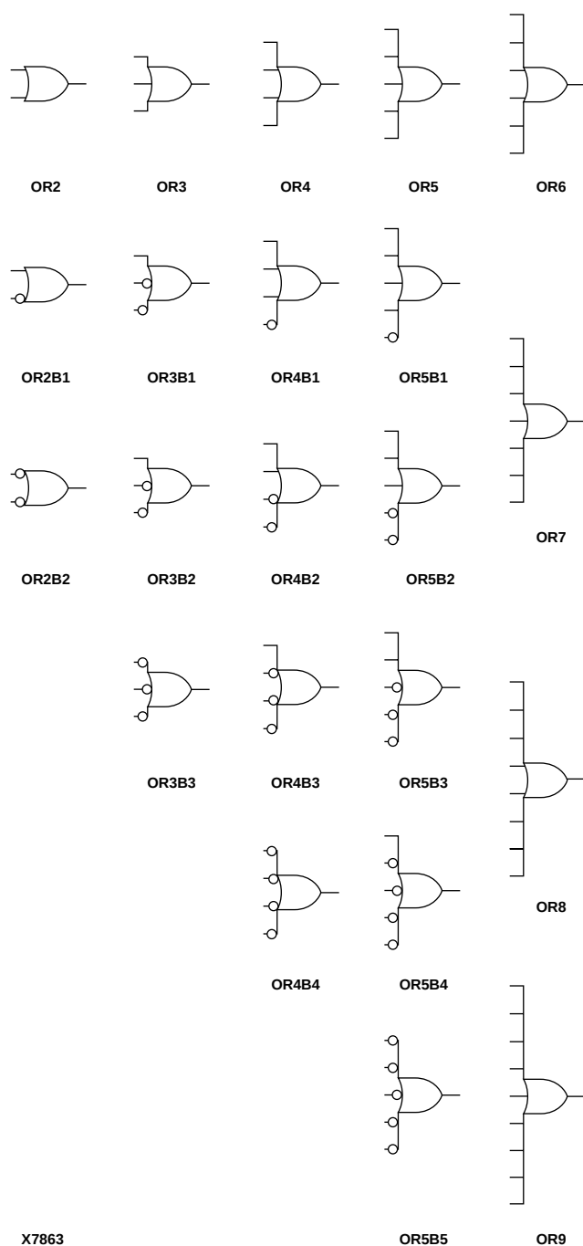
Figure 8-48 OR Gate Representations
