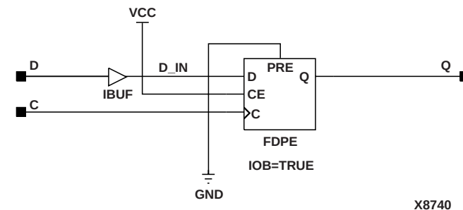
Figure 6-11 IFDI Implementation Spartan2, Virtex
