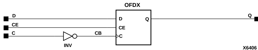
Figure 8-42 OFDX_1 Implementation XC4000E, XC4000X, Spartan, SpartanXL
