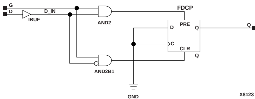
Figure 6-25 ILD Implementation XC9000
