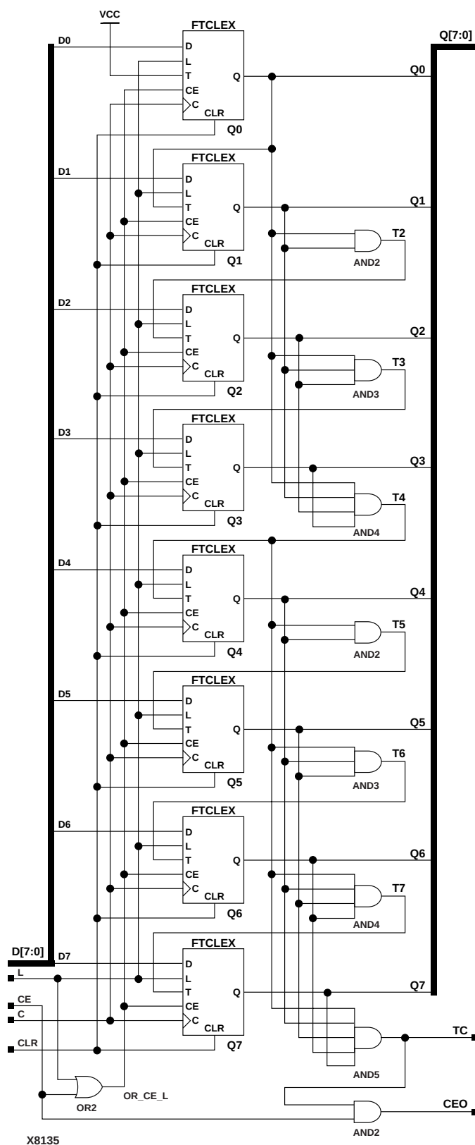
Figure 4-5 CB8CLE Implementation XC4000E, XC4000X, XC5200, Spartan, SpartanXL, Spartan2, Virtex
