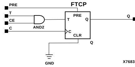
Figure 5-62 FTPE Implementation XC9000
