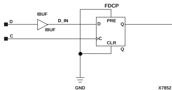
Figure 6-6 IFD Implementation XC9000
