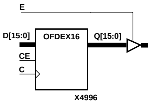
Figure 8-20 OFDEX Implementation XC4000E, XC4000X, Spartan, SpartanXL
