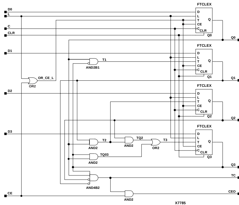
Figure 4-33 CD4CLE Implementation XC4000E, XC4000X, XC5200, Spartan, SpartanXL, Spartan2, Virtex
