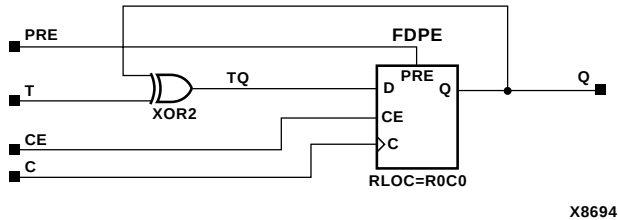
Figure 5-61 FTPE Implementation XC4000E, XC4000X, XC5200, Spartan, SpartanXL, Spartan2, Virtex
