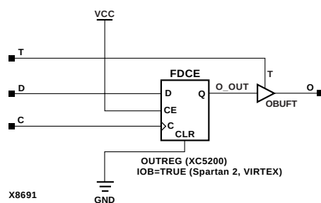
Figure 8-30 OFDT Implementation XC5200, Spartan2, Virtex
