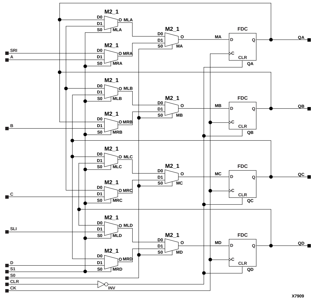
Figure 11-31 X74_194 Implementation XC3000, XC4000E, XC4000X, XC5200, XC9000, Spartan, SpartanXL
