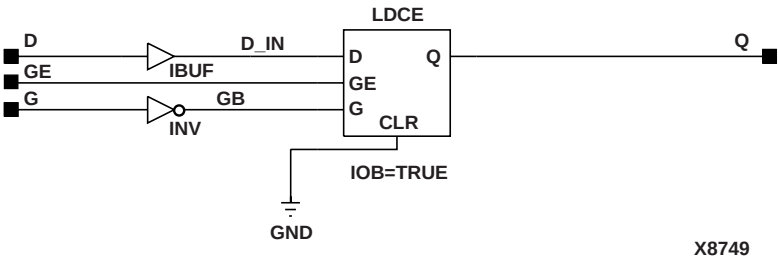
Figure 6-39 ILDX_1 Implementation Spartan2, Virtex
