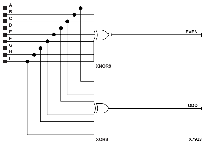
Figure 11-35 X74_280 Implementation XC9000
