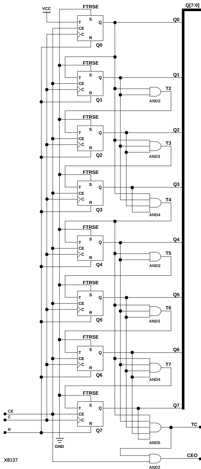
Figure 4-11 CB8RE Implementation XC3000, XC4000E, XC4000X, XC5200, Spartan, SpartanXL, Spartan2, Virtex
