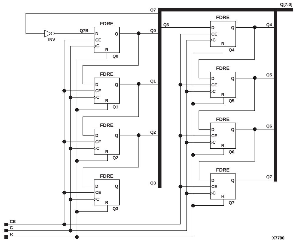
Figure 4-40 CJ8RE Implementation XC3000, XC4000E, XC4000X, XC5200, XC9000, Spartan, SpartanXL, Spartan2, Virtex
