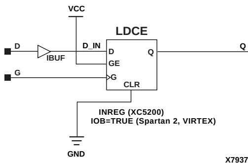
Figure 6-24 ILD Implementation XC5200, Spartan2, Virtex
