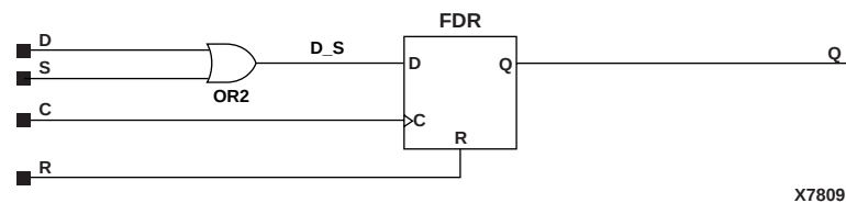
Figure 5-23 FDRS Implementation XC3000, XC4000E, XC4000X, XC5200, Spartan, SpartanXL
