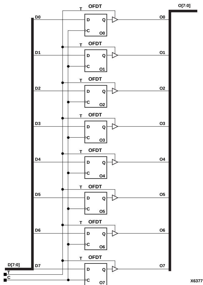
Figure 8-32 OFDT8 Implementation XC3000, XC4000E, XC4000X, XC5200, XC9000, Spartan, SpartanXL, Spartan2, Virtex
