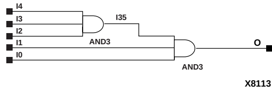
Figure 3-24 AND5 Implementation XC5200
