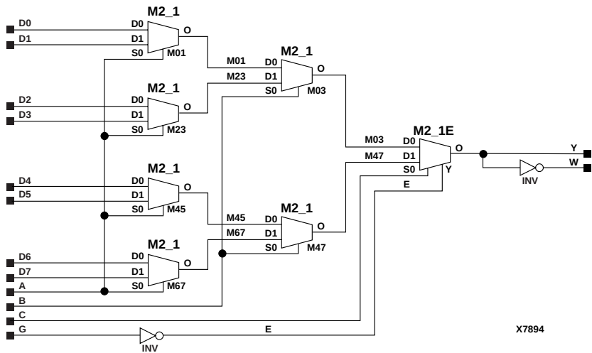
Figure 11-9 X74_151 Implementation XC3000, XC4000E, XC4000X, XC5200, XC9000, Spartan, SpartanXL
