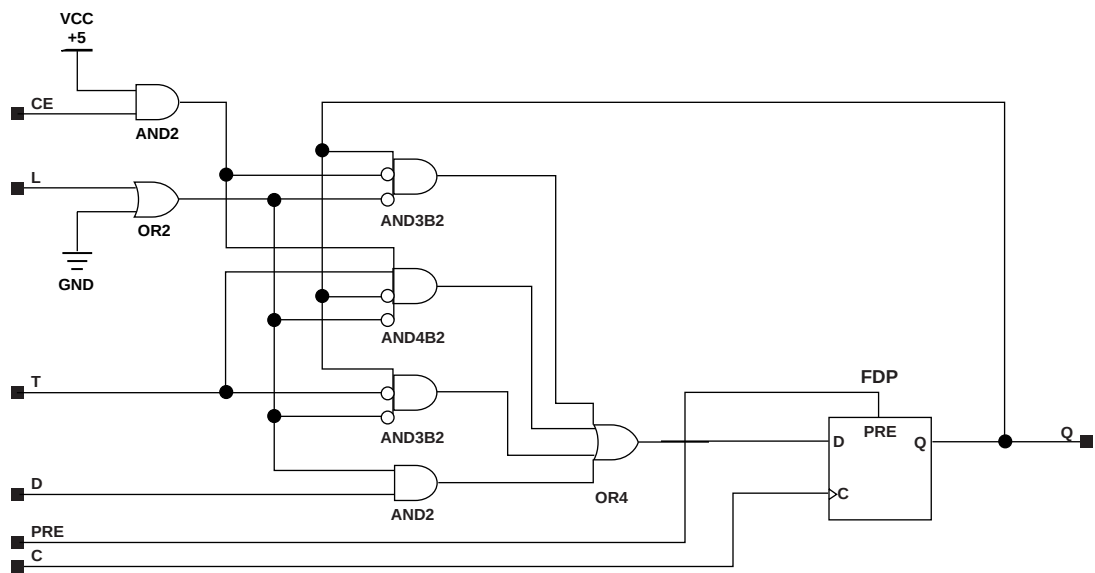
Figure 5-64 FTPLe Implementation XC9000
