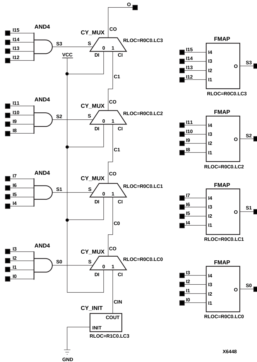
Figure 7-33 NAND16 Implementation XC5200
