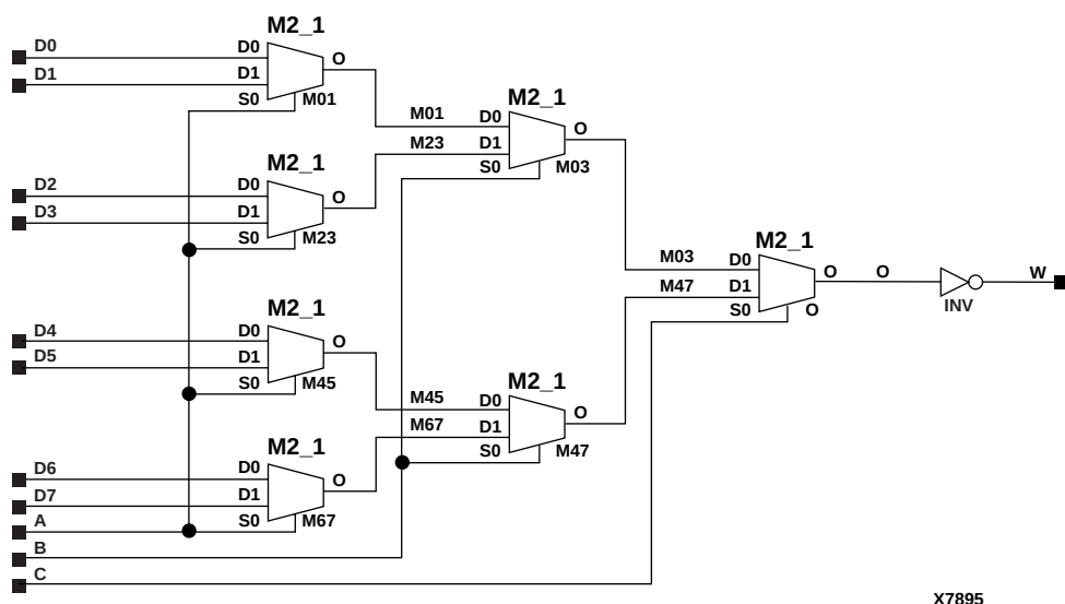
Figure 11-10 X74_152 Implementation XC3000, XC4000E, XC4000X, XC5200, XC9000, Spartan, SpartanXL
