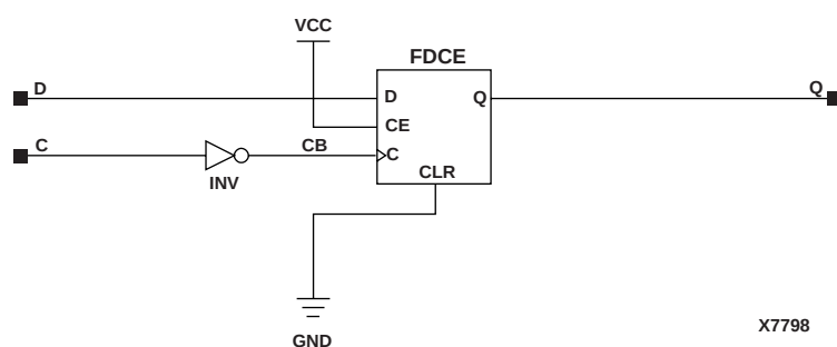
Figure 5-6 FD_1 Implementation XC3000, XC4000E, XC4000X, XC5200, Spartan, SpartanXL
