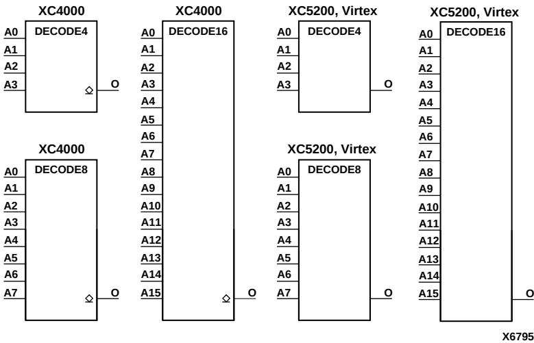
Figure 4-60 DECODE Representations
