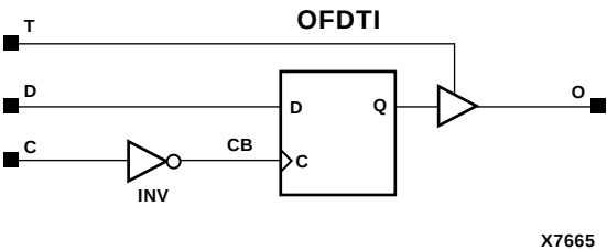
Figure 8-36 OFDTI_1 Implementation XC4000E, XC4000X, Spartan, SpartanXL
