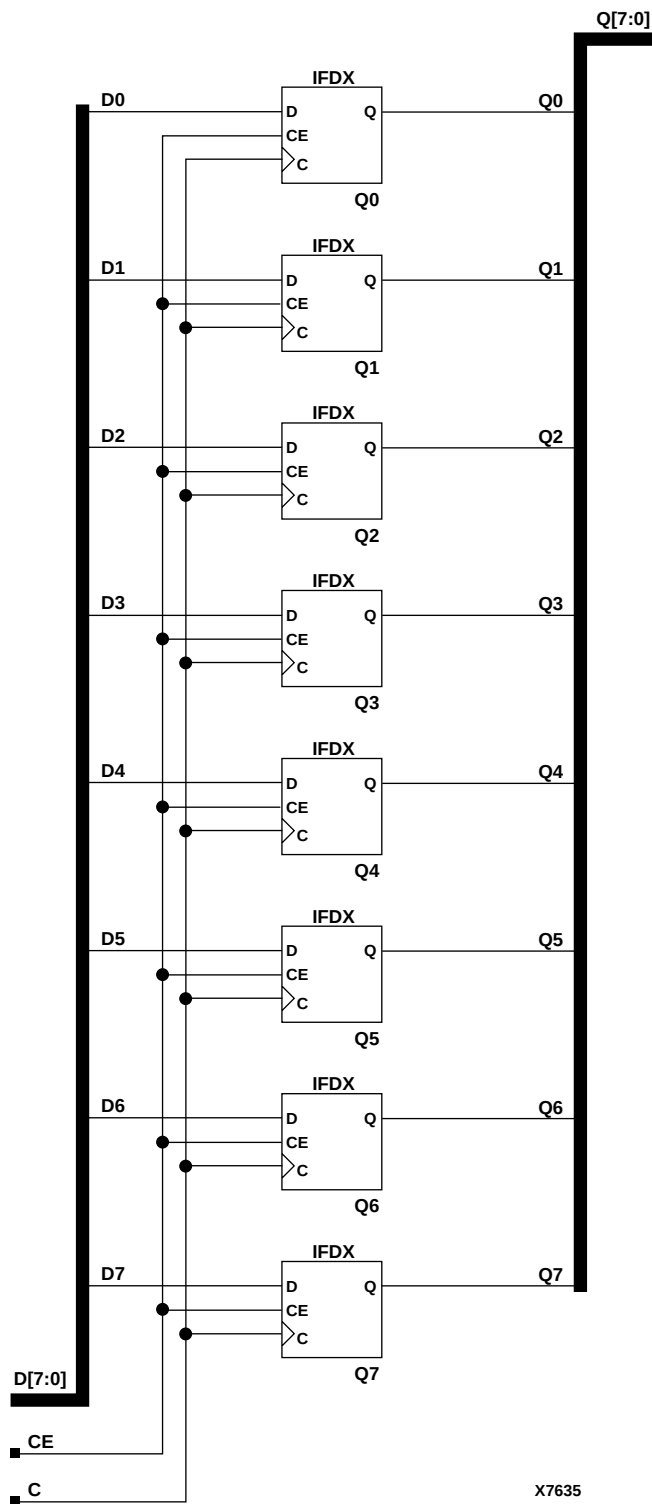
Figure 6-15 IFDX8 Implementation XC4000E, XC4000X, Spartan, SpartanXL, Spartan2, Virtex
