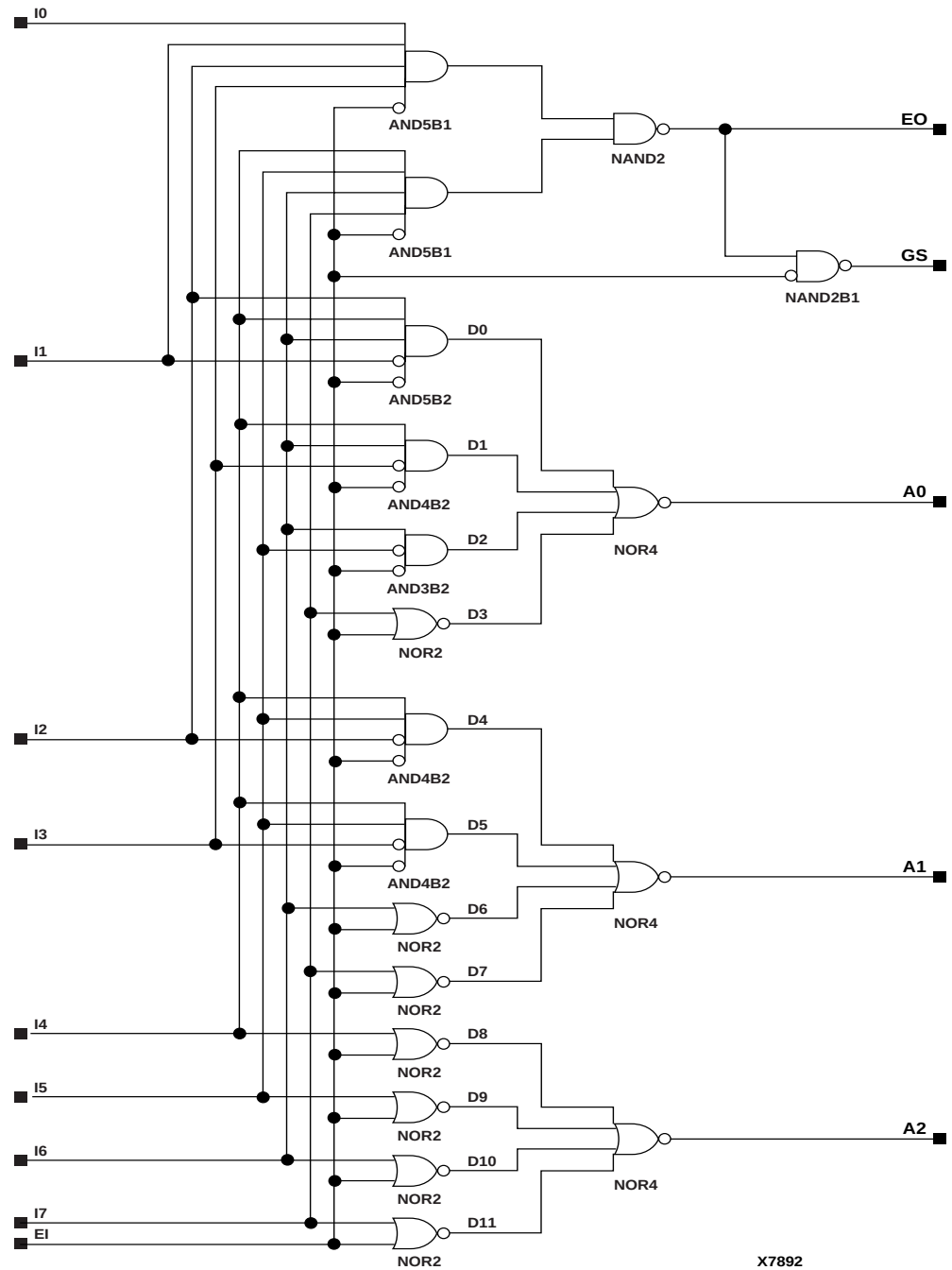
Figure 11-7 X74_148 Implementation XC3000, XC4000E, XC4000X, XC5200, XC9000, Spartan, SpartanXL
