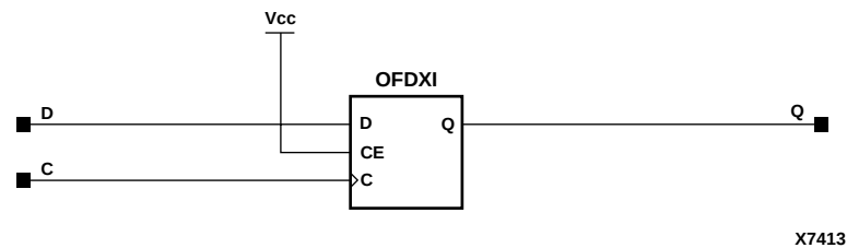
Figure 8-25 OFDI Implementation XC4000E, XC4000X, Spartan, SpartanXL
