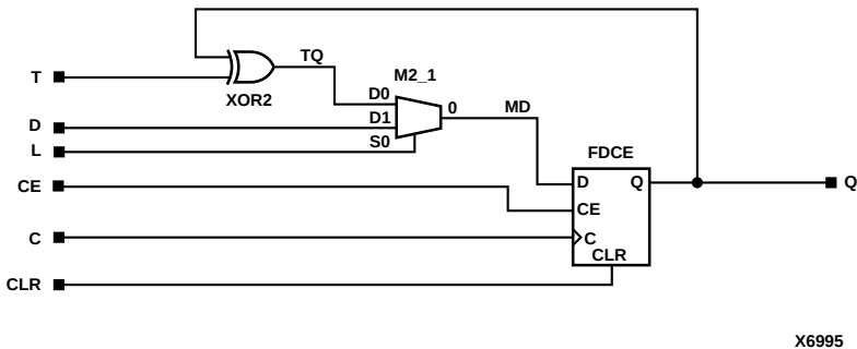
Figure 5-56 FTCLEX Implementation XC4000E, XC4000X, XC5200, Spartan, SpartanXL, Spartan2, Virtex
