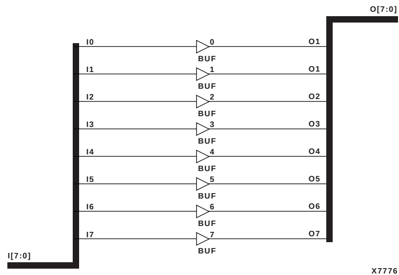
Figure 3-34 BUF8 Implementation XC9000
