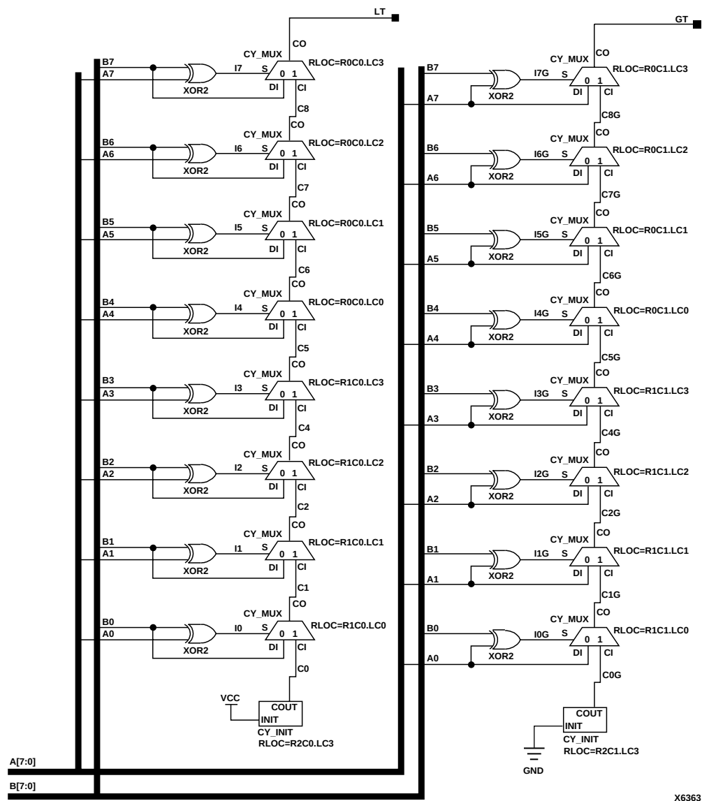
Figure 4-47 COMPMC8 Implementation XC5200
