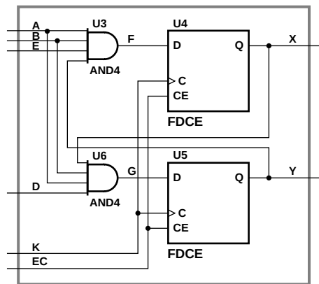
Figure 4-41 XC3000 CLB Primitive Example and Equivalent Circuit
