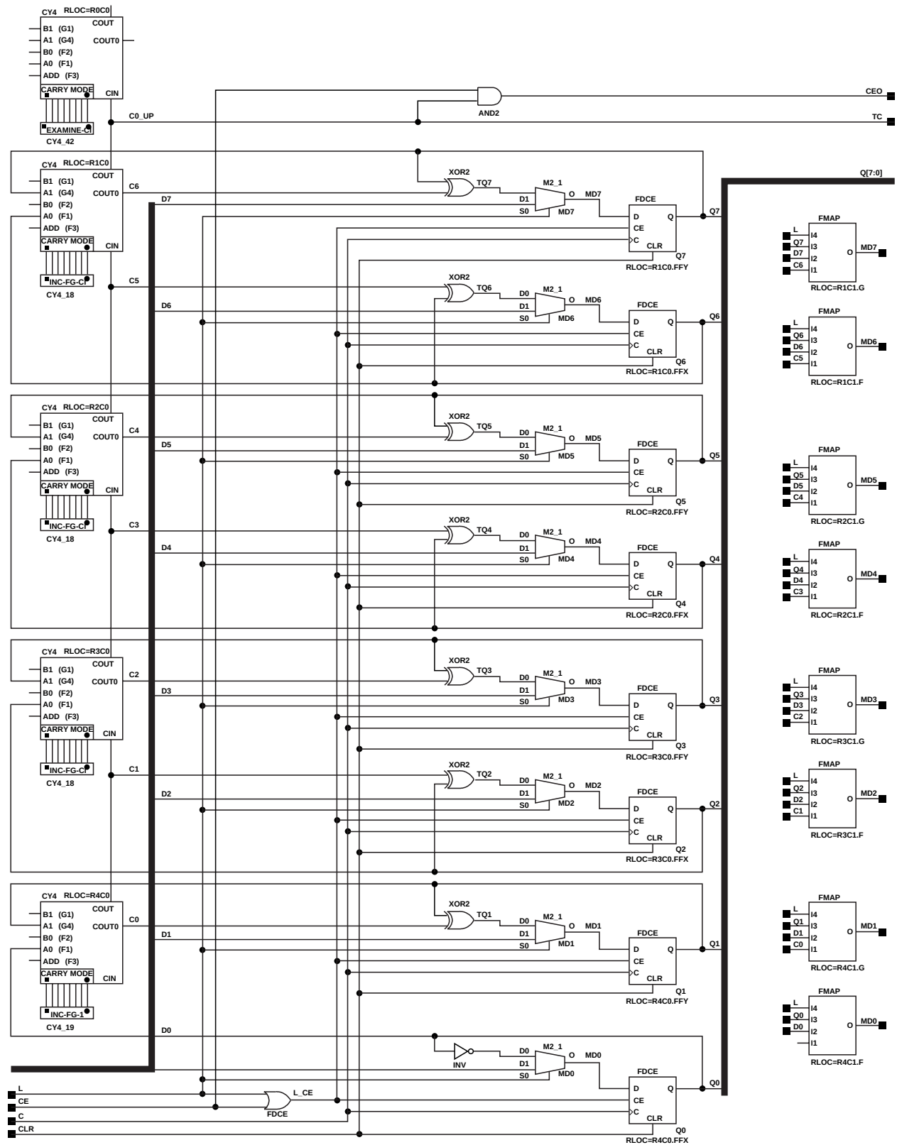
Figure 4-21 CC8CLE Implementation XC4000E, XC4000X, Spartan, SpartanXL
