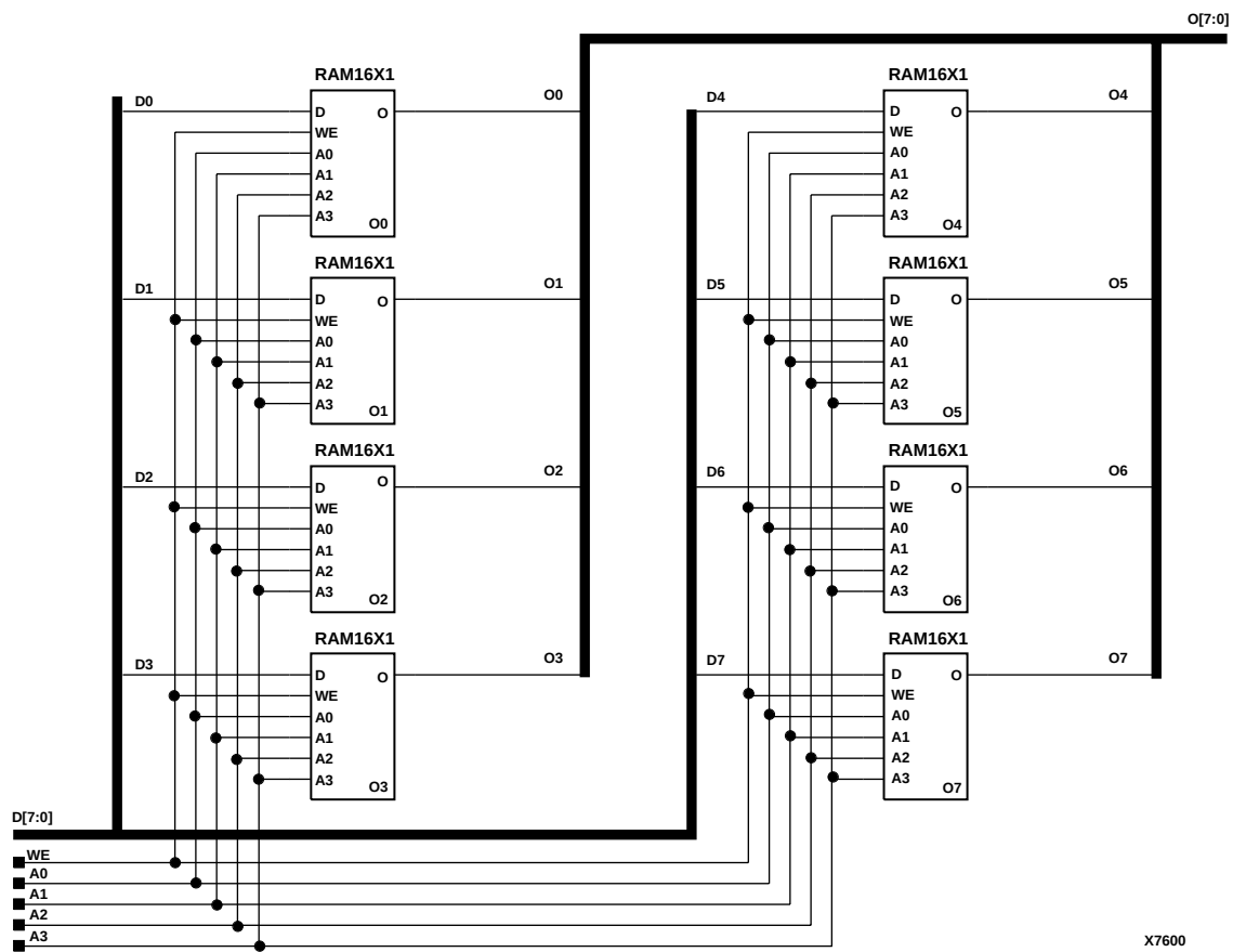
Figure 9-3 RAM16X8 Implementation XC4000E, XC4000X
