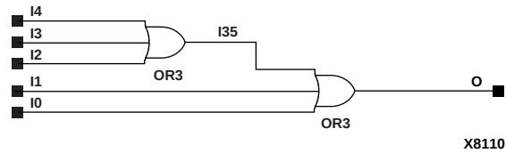
Figure 8-49 OR5 Implementation XC5200
