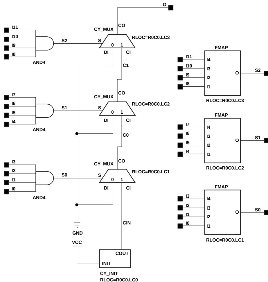
Figure 3-29 AND12 Implementation XC5200
