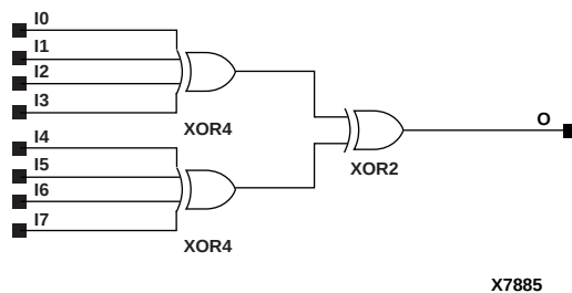
Figure 10-35 XOR8 Implementation XC9000
