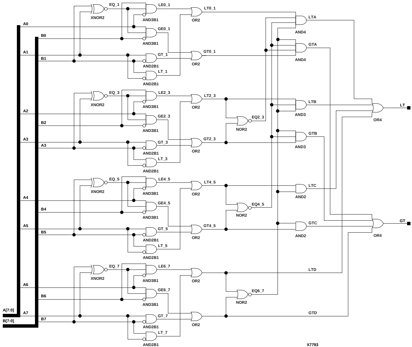
Figure 4-44 COMPM8 Implementation XC3000, XC4000E, XC4000X, XC5200, Spartan, SpartanXL, Spartan2, Virtex
