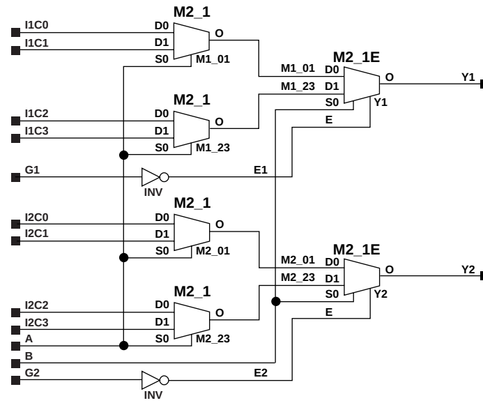
Figure 11-11 X74_153 Implementation XC3000, XC4000E, XC4000X, XC5200, XC9000, Spartan, SpartanXL
