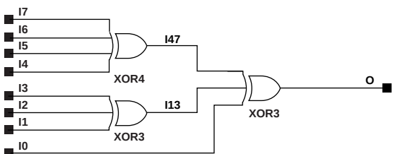
Figure 10-34 XOR8 Implementation XC4000E, XC4000X, XC5200, Spartan, SpartanXL
