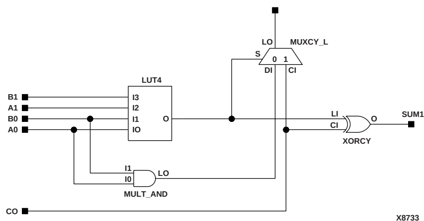
Figure 7-24 Example Multiplier Using MULT_AND
