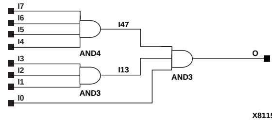
Figure 3-26 AND8 Implementation XC4000E, XC4000X, Spartan, SpartanXL
