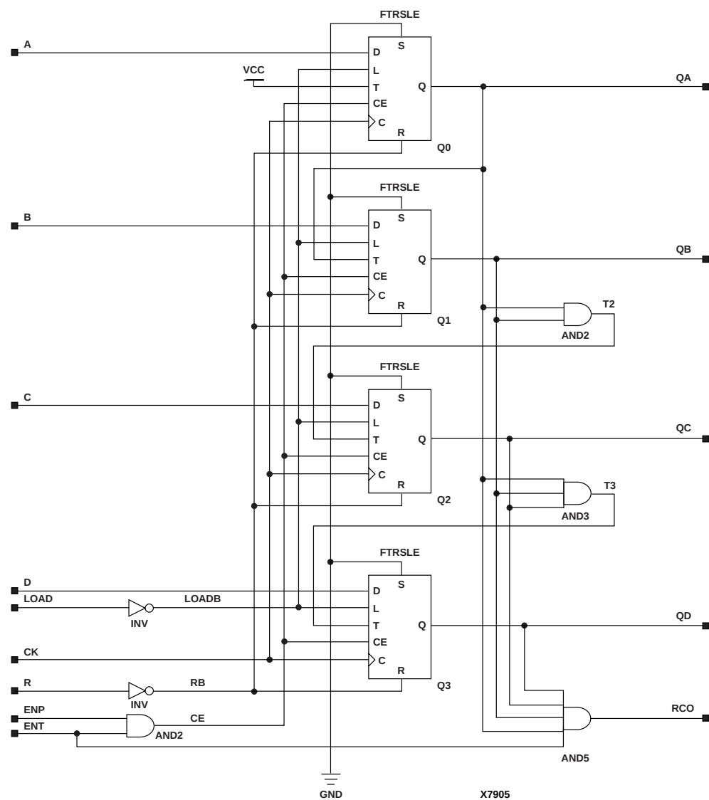
Figure 11-23 X74_163 Implementation XC3000, XC4000E, XC4000X, XC5200, Spartan, SpartanXL
