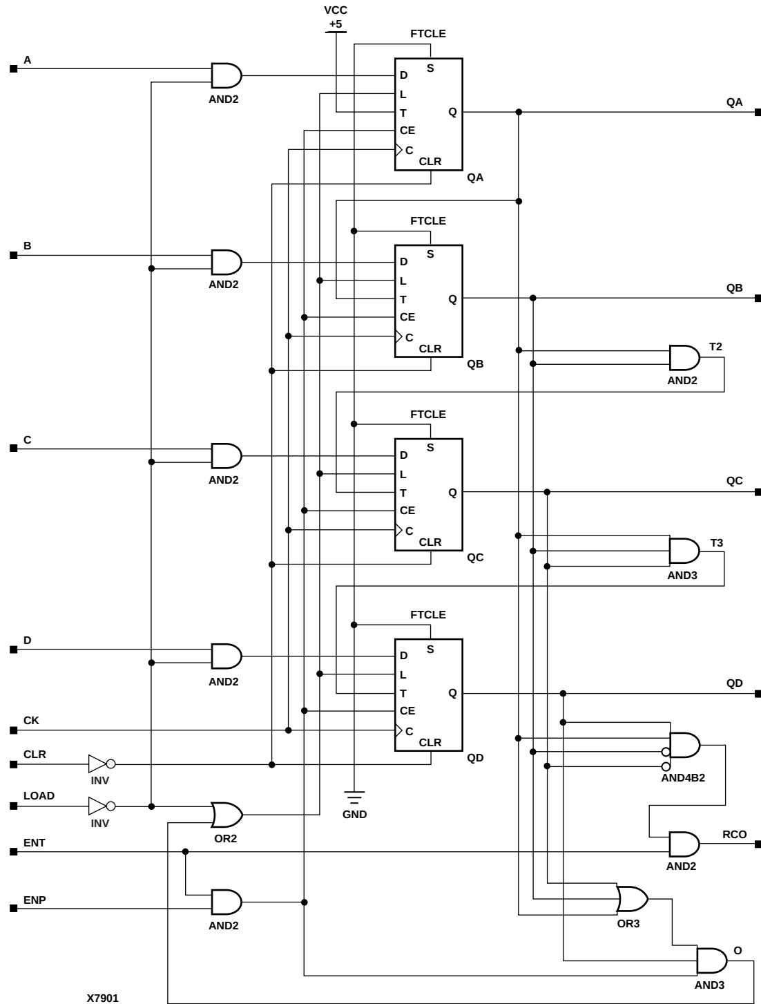
Figure 11-18 X74_160 Implementation XC9000
