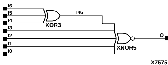
Figure 10-16 XNOR7 Implementation XC3000
