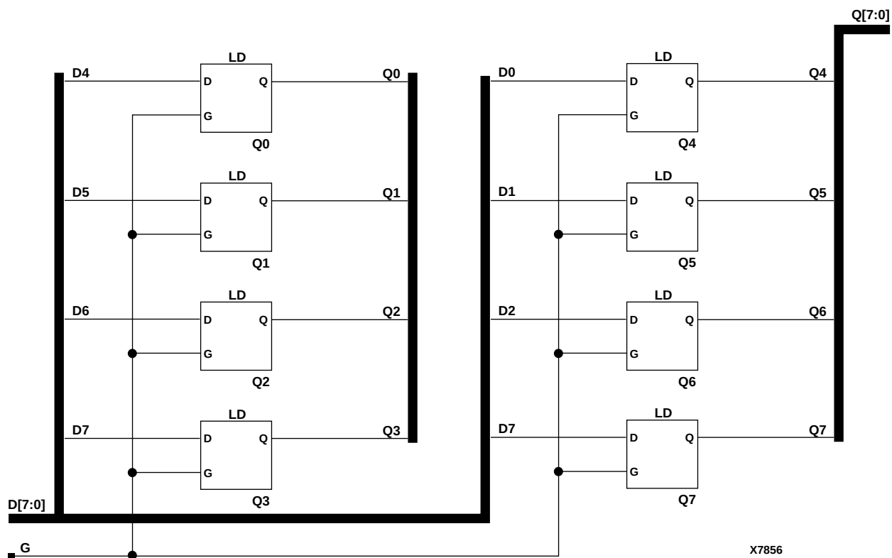
Figure 7-6 LD8 Implementation XC4000X, XC9000, SpartanXL, Spartan2, Virtex
