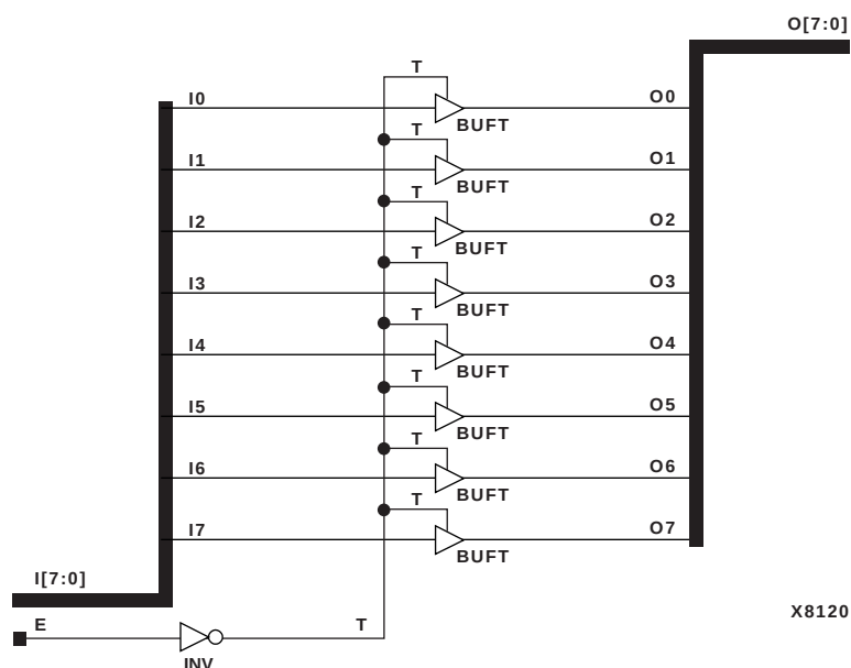
Figure 3-36 BUFE8 Implementation XC3000, XC4000E, XC4000X, XC5200, Spartan, SpartanXL
