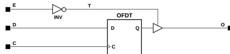
Figure 8-12 OFDE Implementation XC3000, XC4000E, XC4000X, Spartan, SpartanXL
