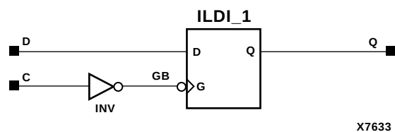
Figure 6-31 ILDI Implementation XC4000E, XC4000X, Spartan, SpartanXL
