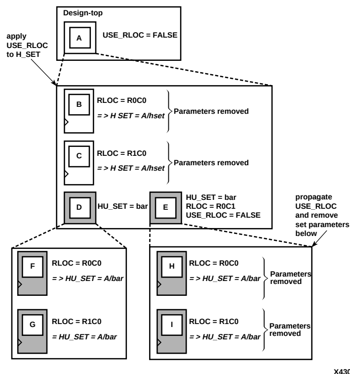
Figure 12-12 Using the USE_RLOC Constraint to Control RLOC Application on H_SET and HU_SET Sets
