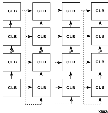
Figure 12-17 Available XC4000X, Spartan, and SpartanXL Carry Propagation Paths (dotted lines use general interconnect)
