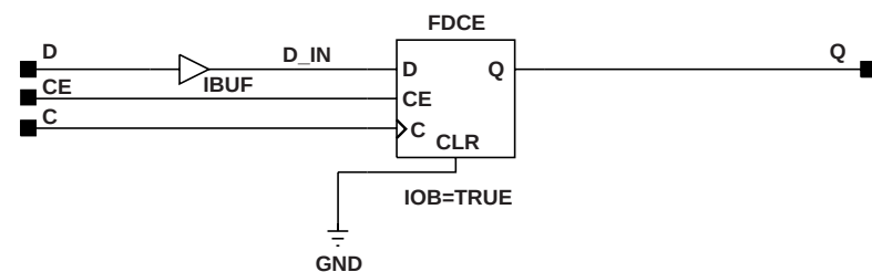
Figure 6-14 IFDX Implementation Spartan2, Virtex
