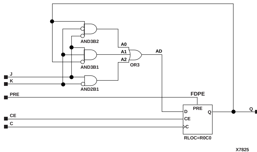
Figure 5-42 FJKPE Implementation XC4000E, XC4000X, XC5200, Spartan, SpartanXL, Spartan2, Virtex
