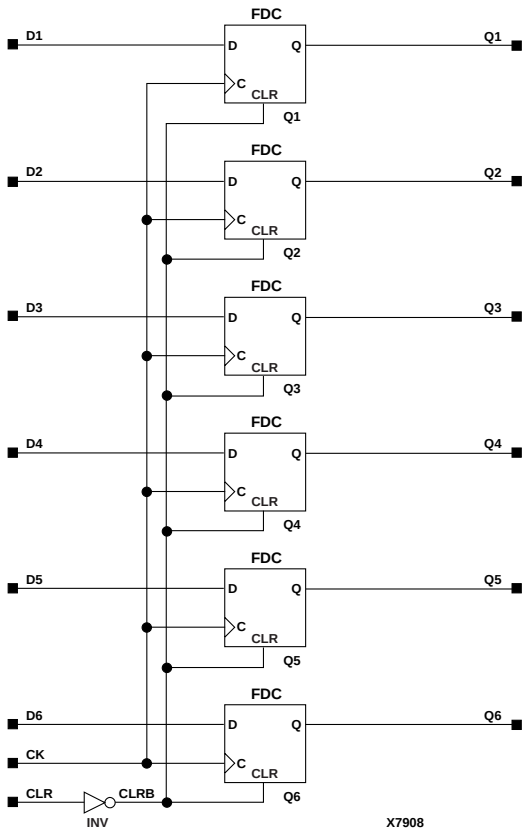
Figure 11-30 X74_174 Implementation XC3000, XC4000E, XC4000X, XC5200, XC9000, Spartan, SpartanXL
