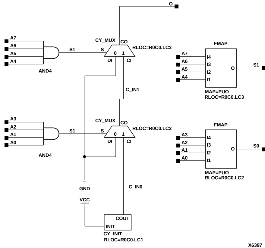
Figure 4-62 DECODE8 Implementation XC5200
