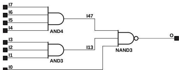
Figure 7-28 NAND8 Implementation XC4000E, XC4000X, Spartan, SpartanXL
