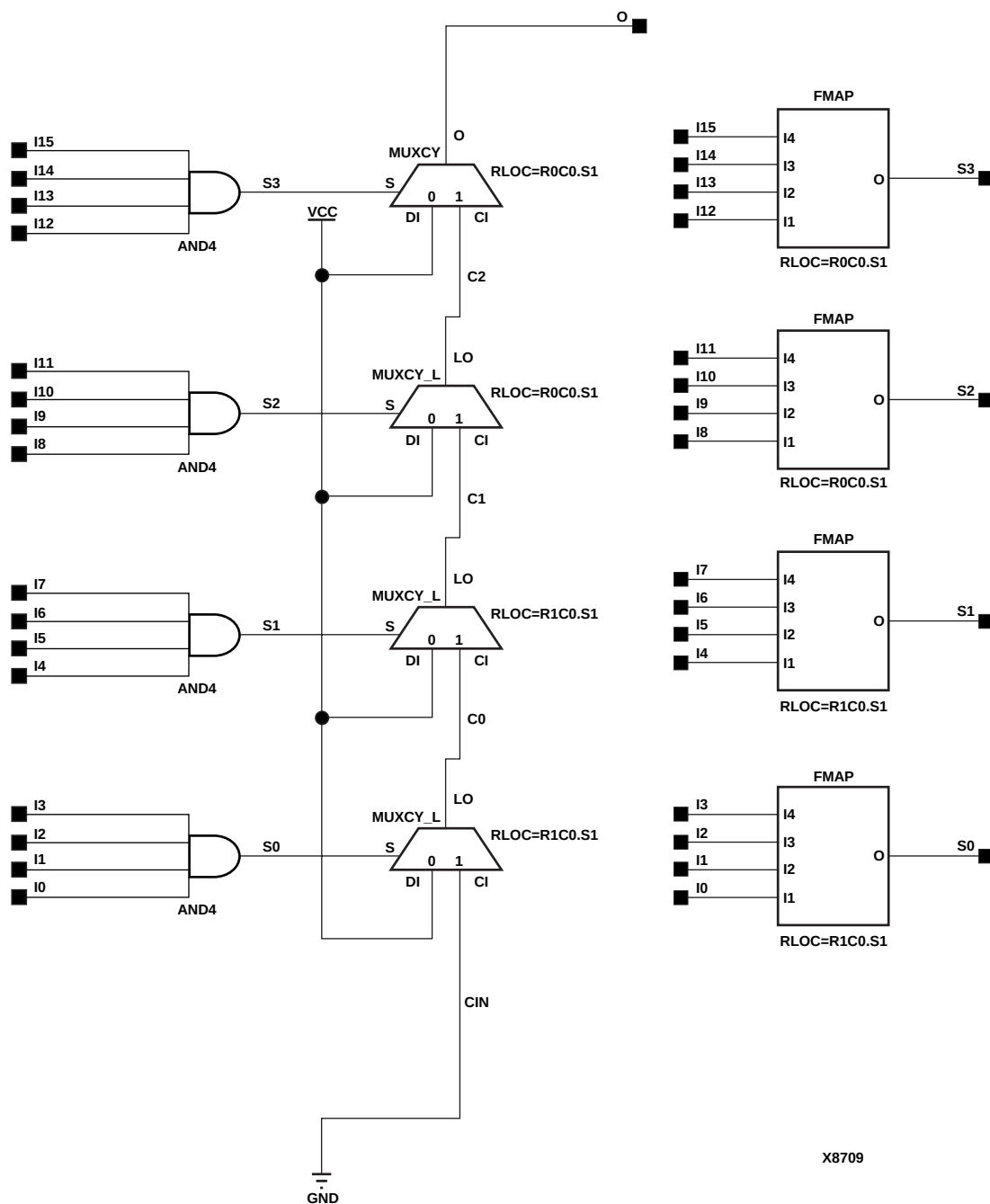
Figure 7-34 NAND16 Implementation Spartan2, Virtex
