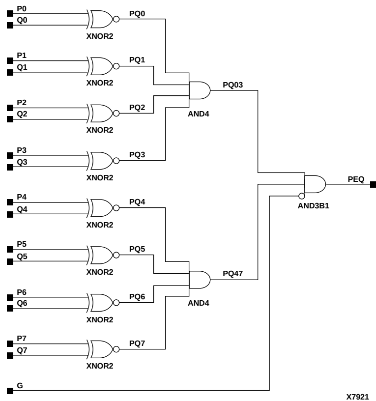
Figure 11-44 X74_518 Implementation XC3000, XC4000E, XC4000X, XC5200, XC9000, Spartan, SpartanXL
