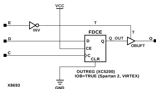
Figure 8-13 OFDE Implementation XC5200, Spartan2, Virtex
