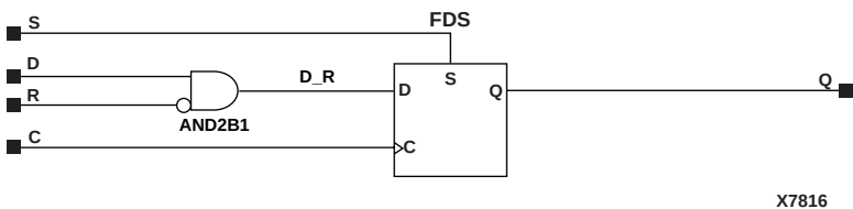
Figure 5-30 FDSR Implementation XC3000, XC4000E, XC4000X, XC5200, Spartan, SpartanXL
