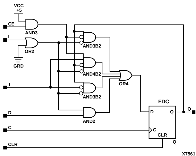
Figure 5-55 FTCLE Implementation XC9000
