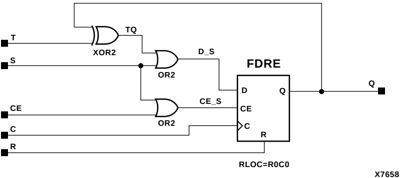
Figure 5-65 FTRSE Implementation XC3000, XC4000E, XC4000X, XC5200, Spartan, SpartanXL, Spartan2, Virtex
