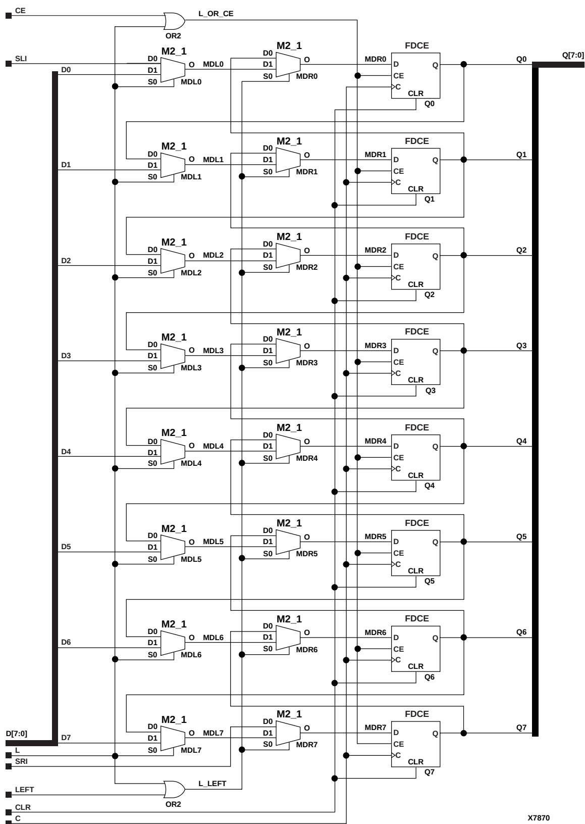
Figure 10-6 SR8CLED Implementation XC3000, XC4000E, XC4000X, XC5200, Spartan, SpartanXL, Spartan2, Virtex
