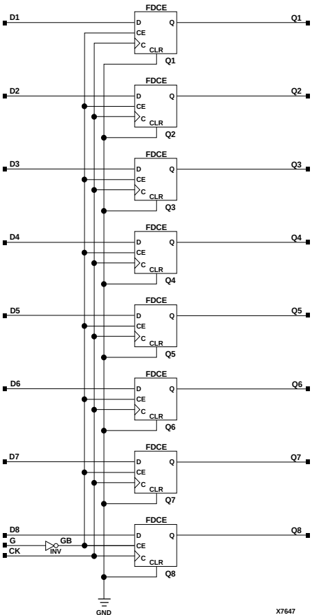
Figure 11-41 X74_377 Implementation XC3000, XC4000E, XC4000X, XC5200, XC9000, Spartan, SpartanXL
