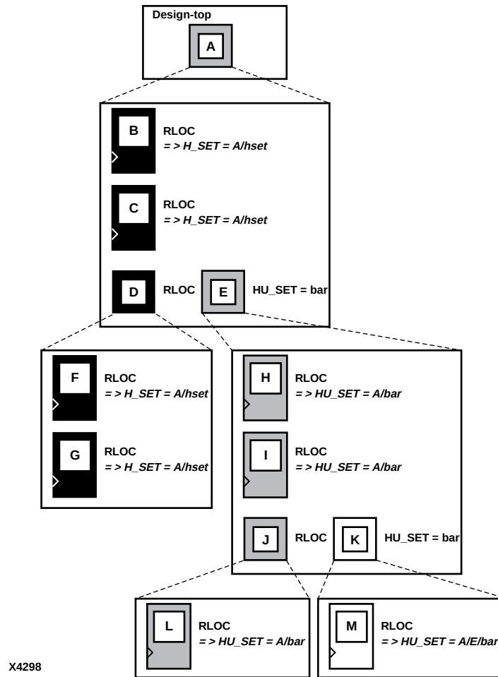
Figure 12-9 HU_SET Constraint Linking and Separating Elements from H_SET Sets
