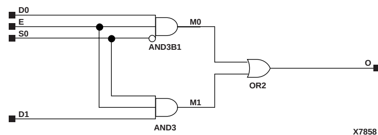
Figure 7-19 M2_1E Implementation XC3000, XC4000E, XC4000X, XC5200, XC9000, Spartan, SpartanXL, Spartan2, Virtex
