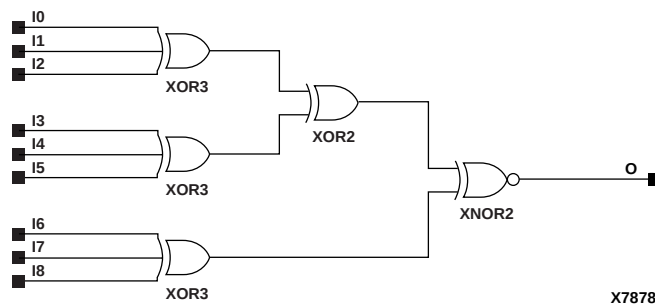
Figure 10-26 XNOR9 Implementation XC9000
