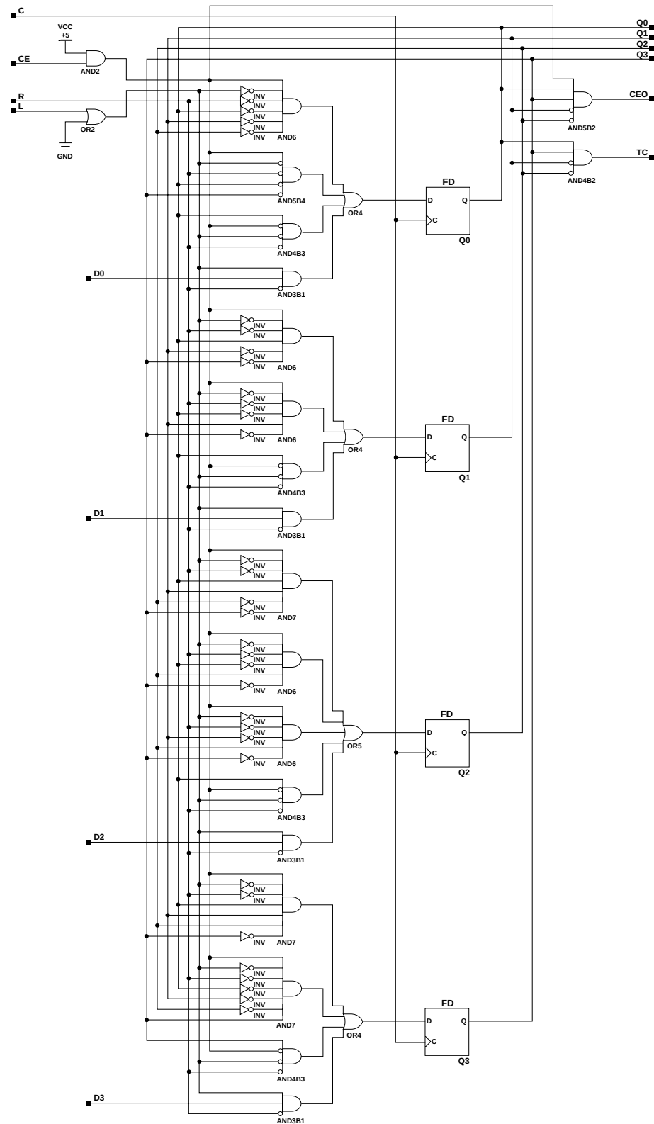
Figure 4-38 CD4RLE Implementation XC9000
