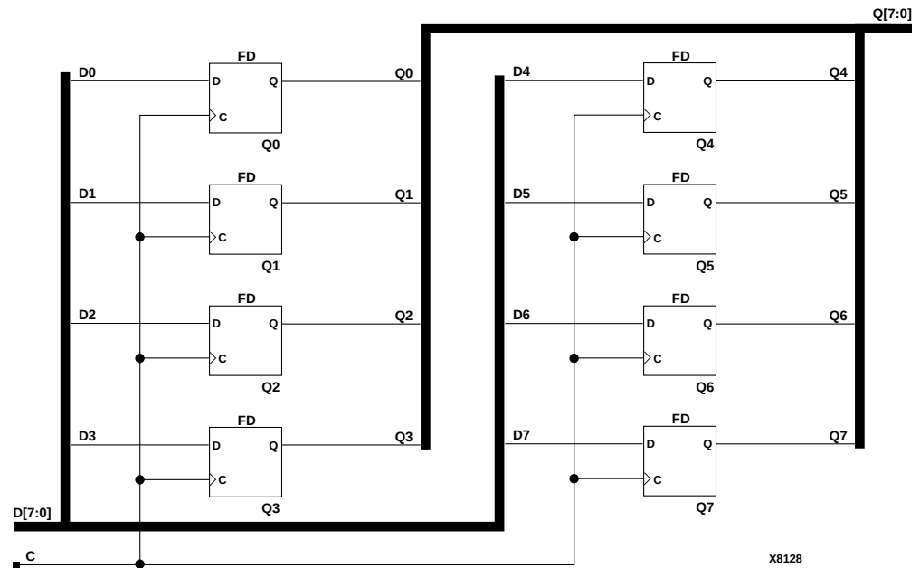
Figure 5-7 FD8 Implementation XC9000
