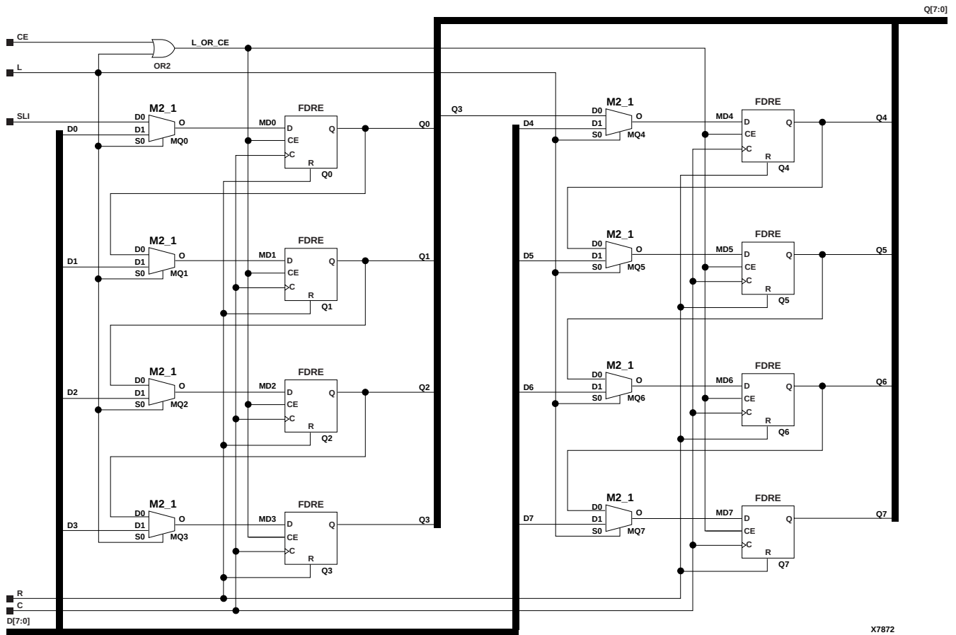
Figure 10-9 SR8RLE Implementation XC3000, XC4000E, XC4000X, XC5200, XC9000, Spartan, SpartanXL, Spartan2, Virtex
