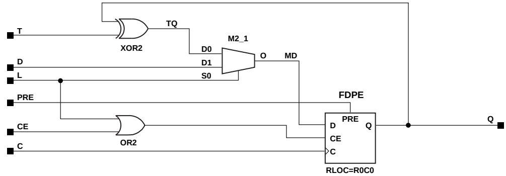
Figure 5-63 FTPLe Implementation XC4000E, XC4000X, XC5200, Spartan, SpartanXL, Spartan2, Virtex
