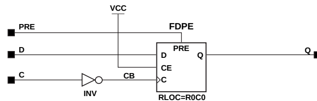
Figure 5-17 FDP_1 Implementation XC4000E, XC4000X, XC5200, Spartan, SpartanXL
