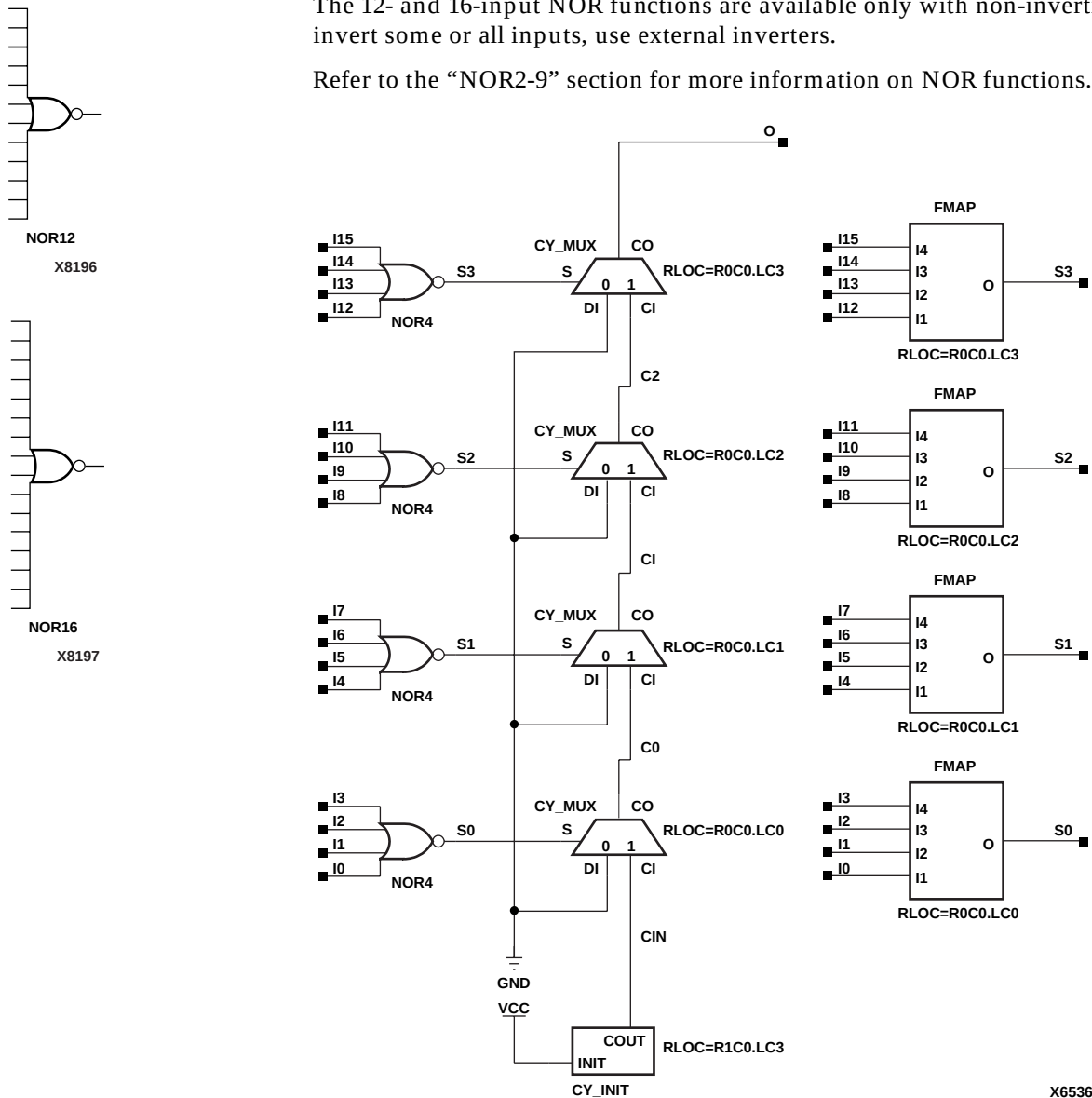
Figure 7-41 NOR16 Implementation XC5200
