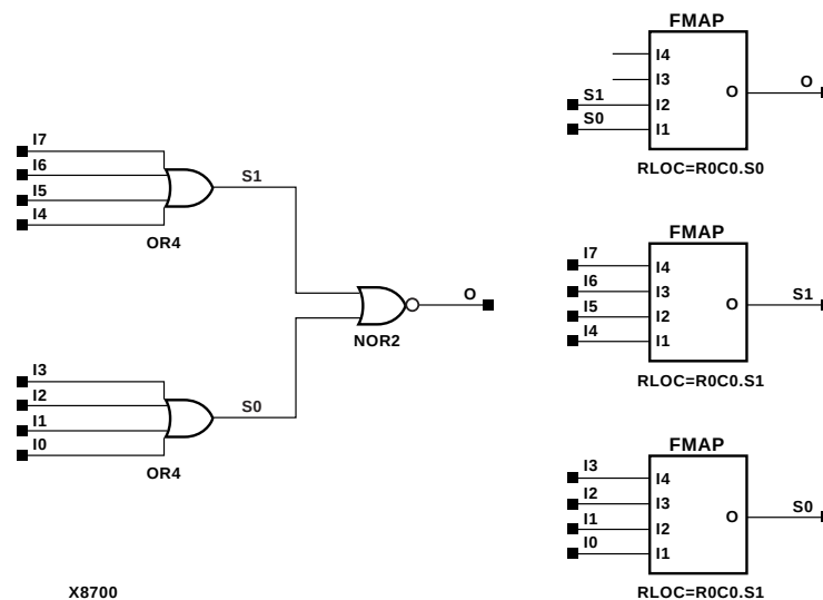
Figure 7-40 NOR8 Implementation Spartan2, Virtex
