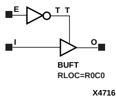
Figure 3-35 BUFE Implementation XC3000, XC4000E, XC4000X, XC5200, Spartan, SpartanXL
