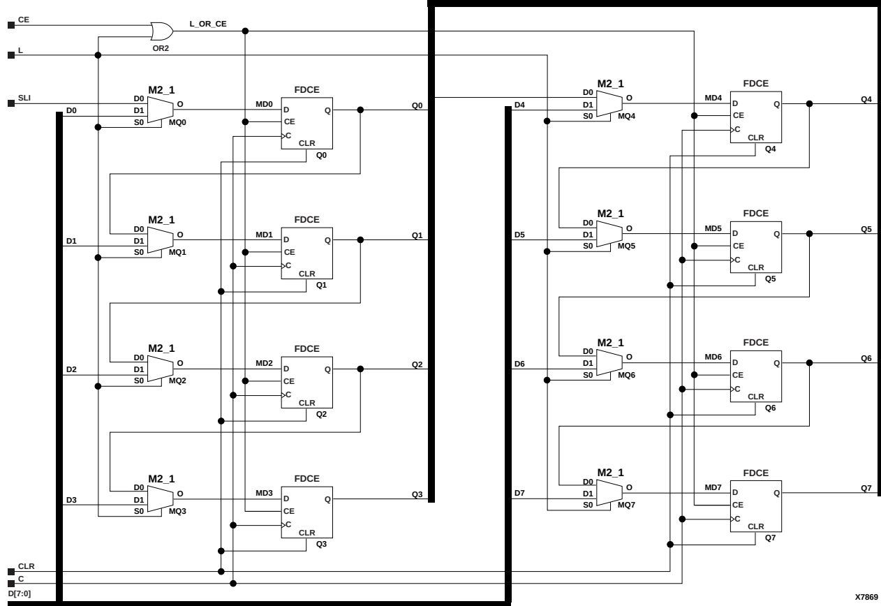
Figure 10-5 SR8CLE Implementation XC3000, XC4000E, XC4000X, XC5200, XC9000, Spartan, SpartanXL, Spartan2, Virtex
