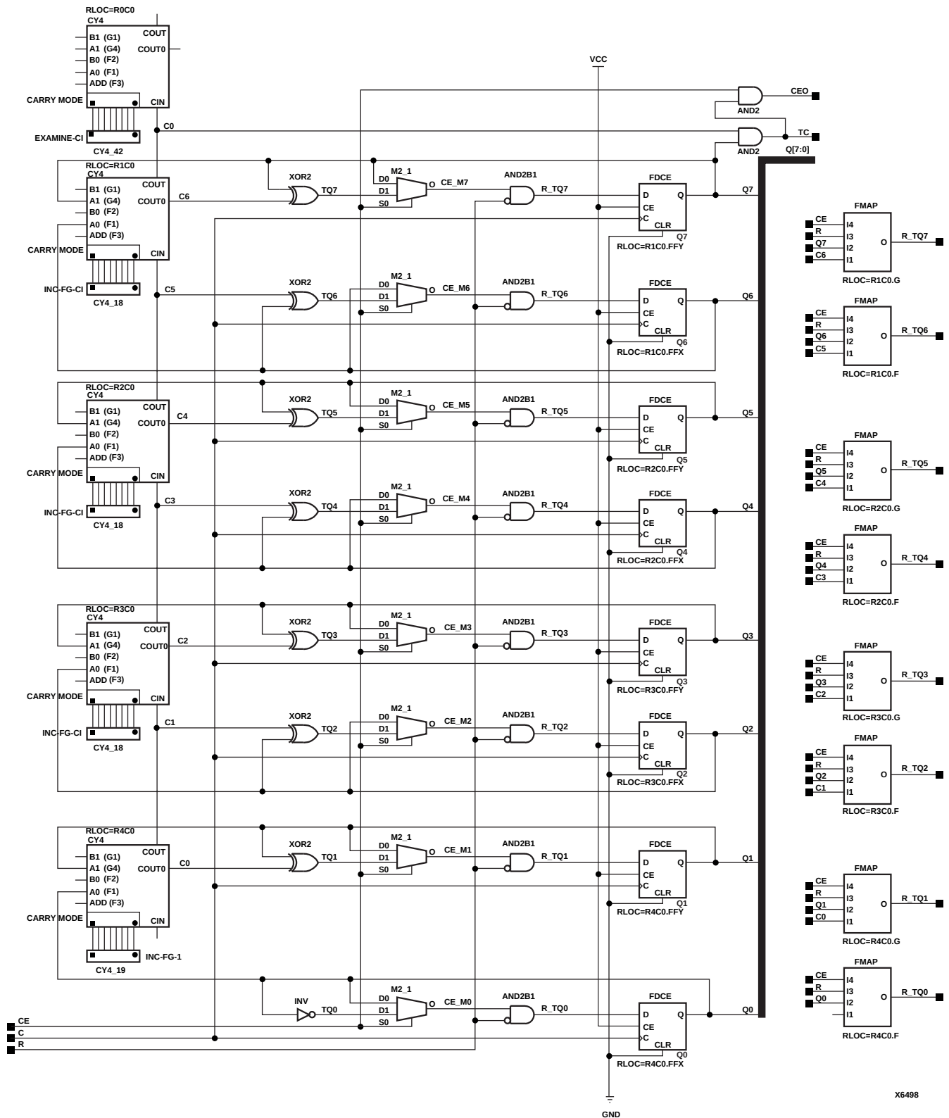
Figure 4-27 CC8RE Implementation XC4000E, XC4000X, Spartan, SpartanXL
