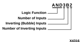
Figure 1-2 Combinatorial Naming Conventions
