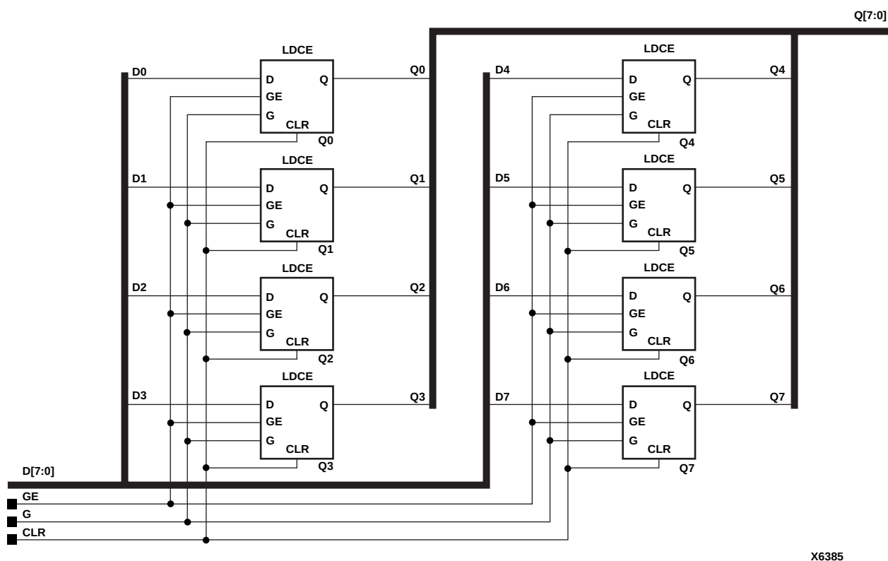
Figure 7-14 LD8CE Implementation XC4000X, XC5200, SpartanXL, Spartan2, Virtex
