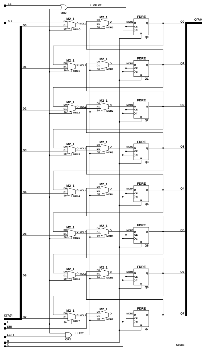
Figure 10-10 SR8LED Implementation XC3000, XC4000E, XC4000X, XC5200, XC9000, Spartan, SpartanXL, Spartan2, Virtex
