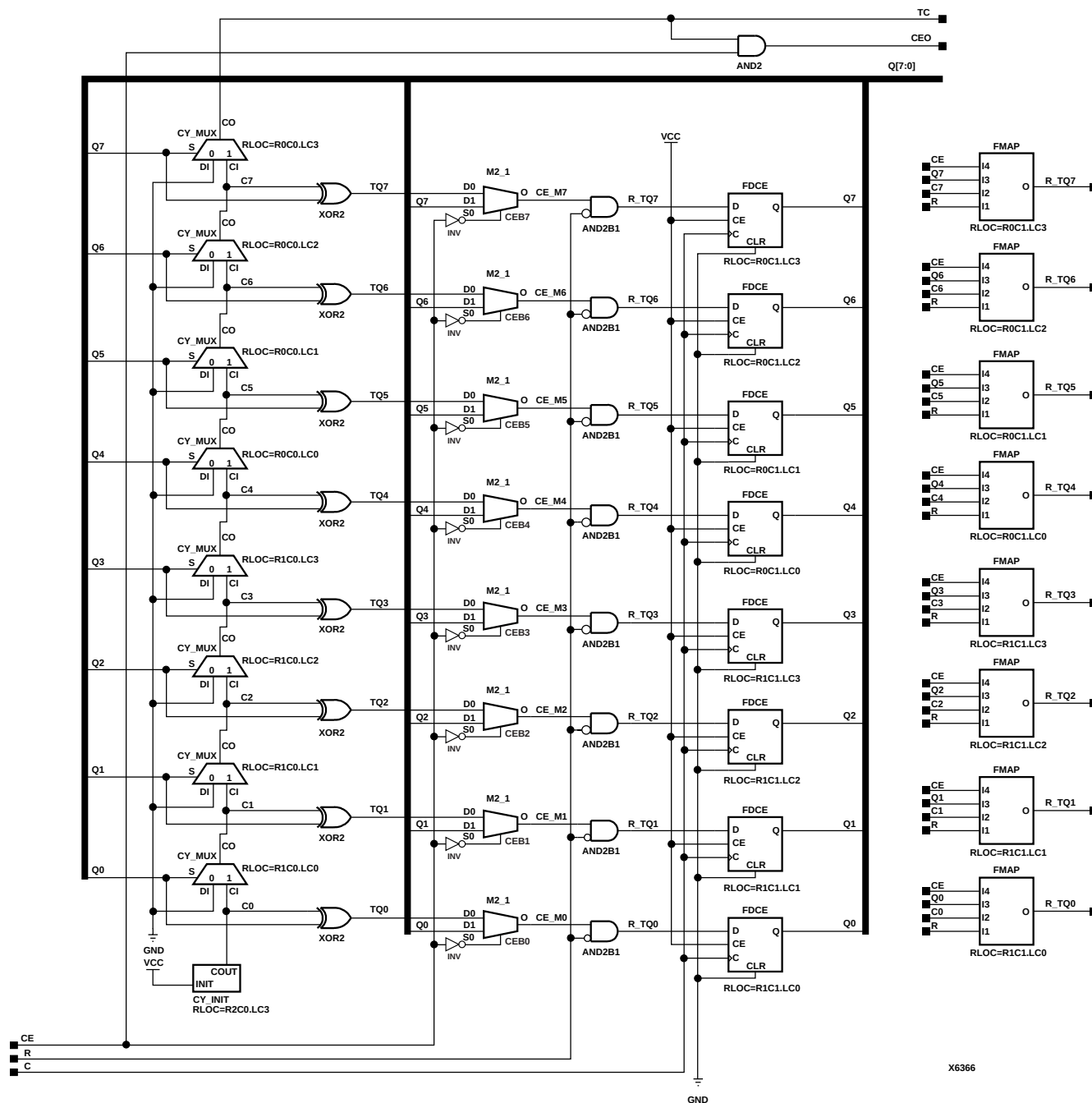
Figure 4-28 CC8RE Implementation XC5200
