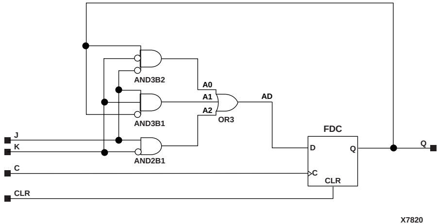
Figure 5-34 FJKC Implementation XC3000, XC4000E, XC4000X, XC5200, Spartan, SpartanXL, Spartan2, Virtex
