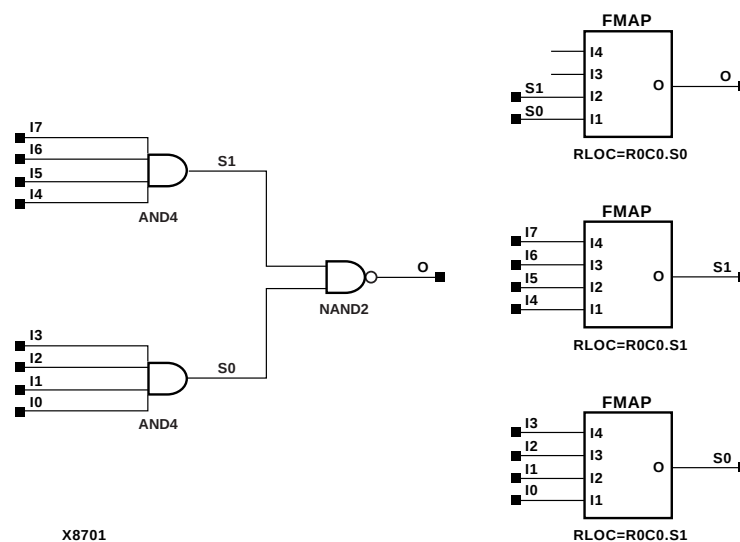
Figure 7-30 NAND8 Implementation Spartan2, Virtex
