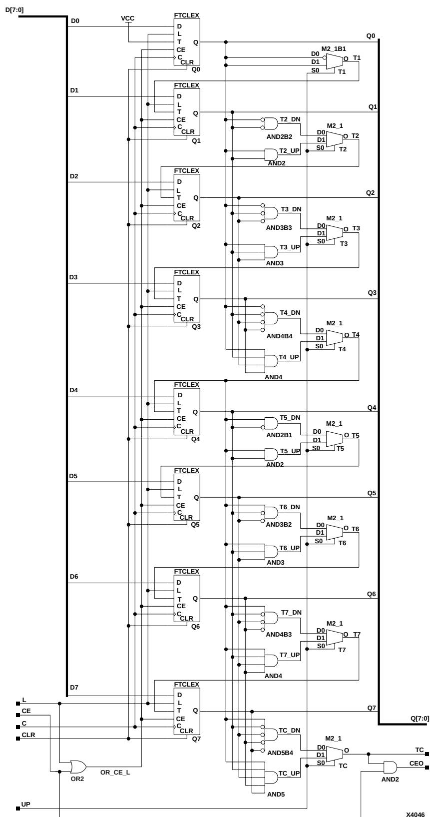
Figure 4-9 CB8CLED Implementation XC4000E, XC4000X, XC5200, Spartan, SpartanXL, Spartan2, Virtex
