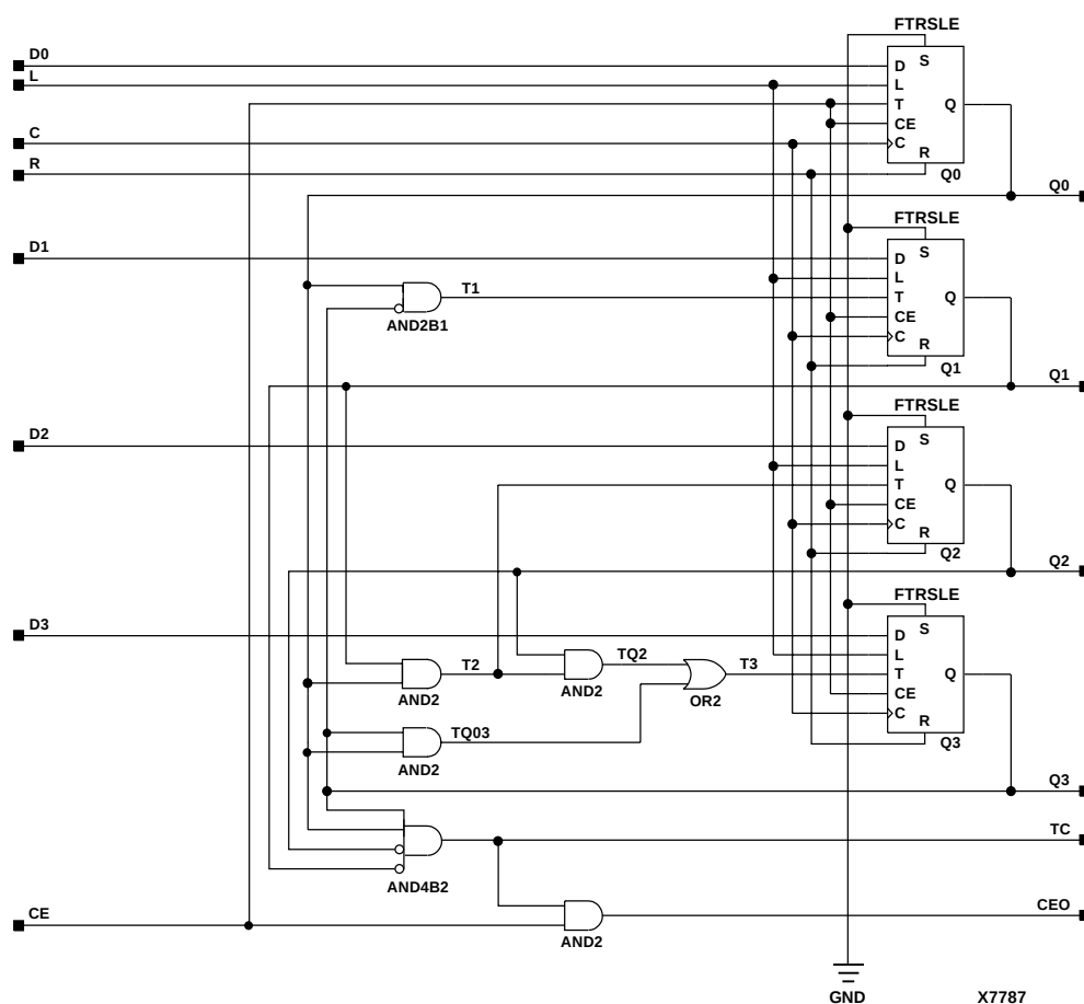
Figure 4-37 CD4RLE Implementation XC3000, XC4000E, XC4000X, XC5200, Spartan, SpartanXL, Spartan2, Virtex
