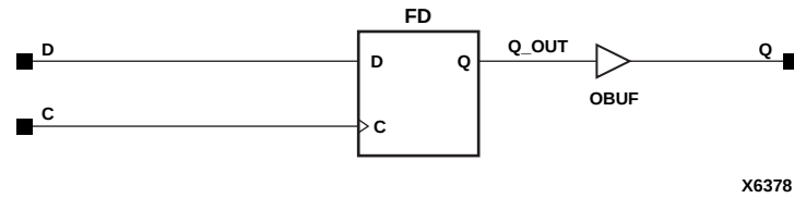
Figure 8-7 OFD Implementation XC9000
