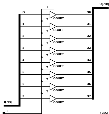
Figure 8-4 OBUFT8 Implementation XC3000, XC4000E, XC4000X, XC5200, XC9000, Spartan, SpartanXL, Spartan2, Virtex
