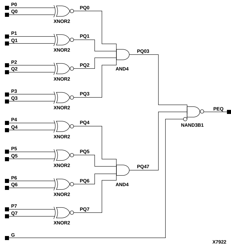
Figure 11-45 X74_521 Implementation XC3000, XC4000E, XC4000X, XC5200, XC9000, Spartan, SpartanXL
