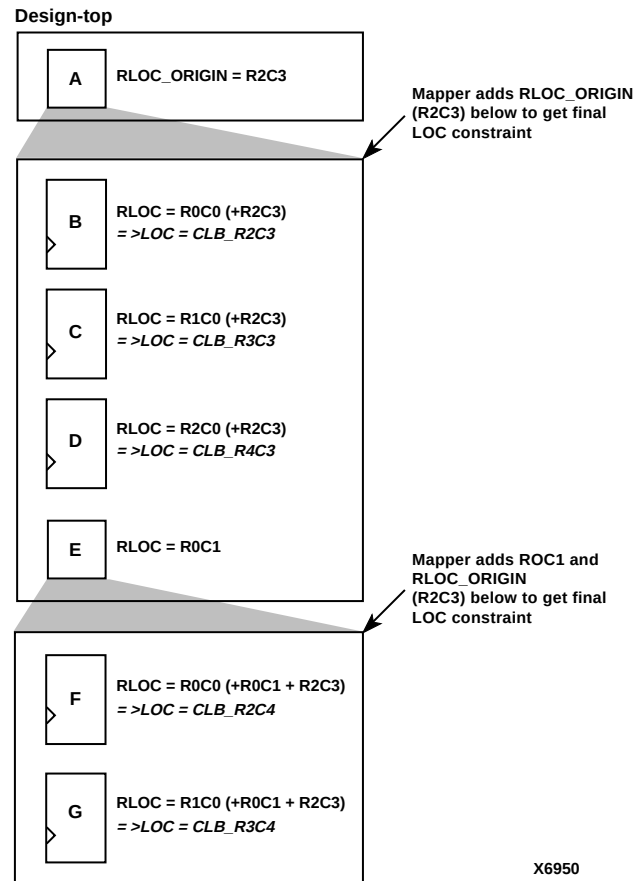
Figure 12-14 Using an RLOC_ORIGIN Constraint to Modify an H_SET Set
