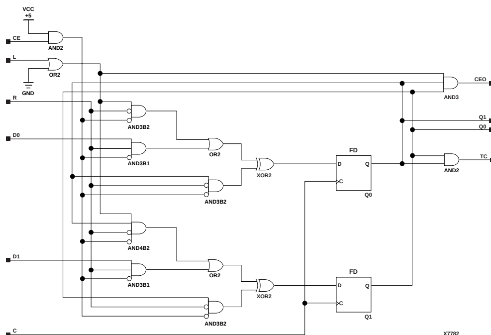
Figure 4-14 CB2RLE Implementation XC9000
