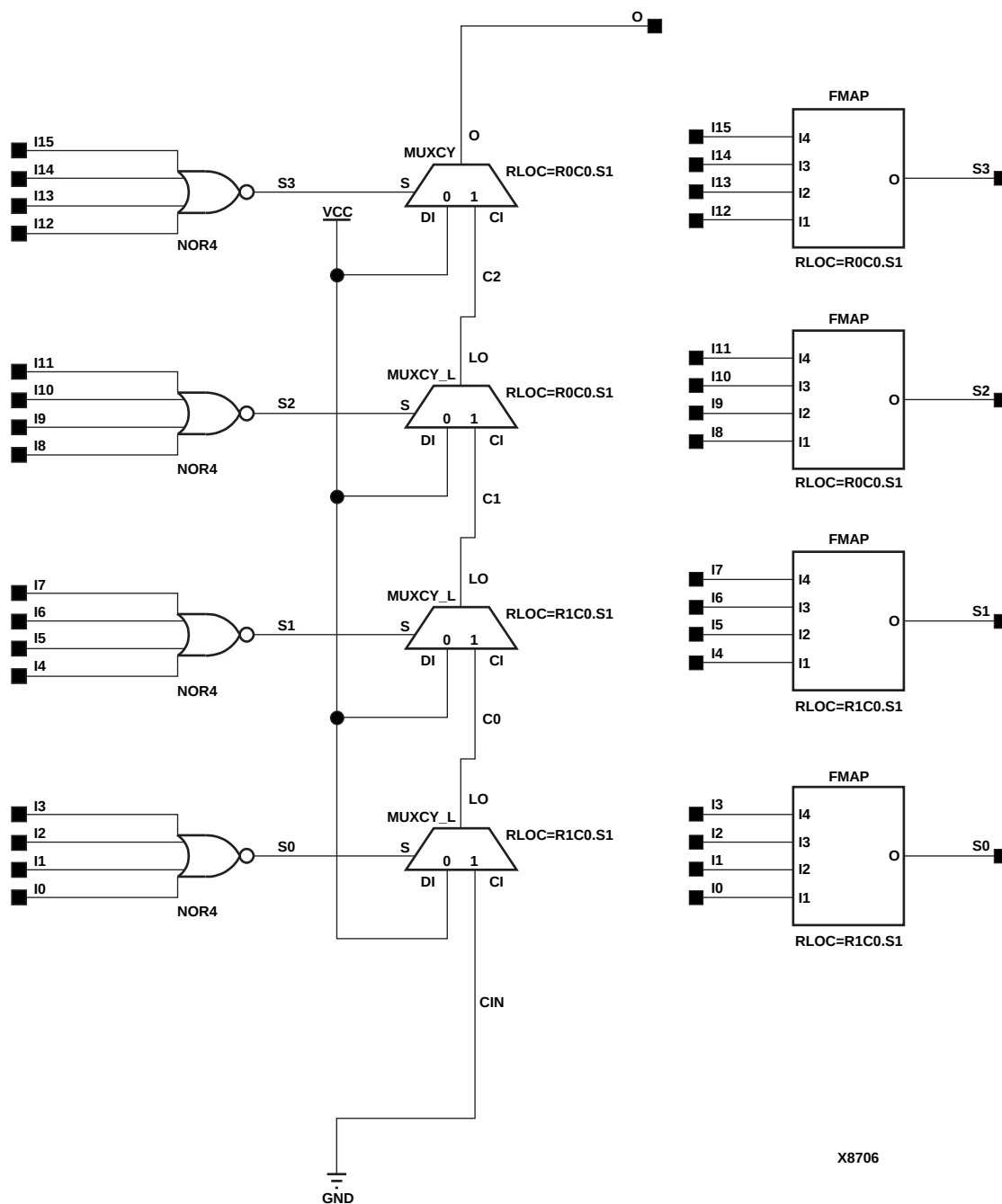
Figure 8-54 OR16 Implementation Spartan2, Virtex
