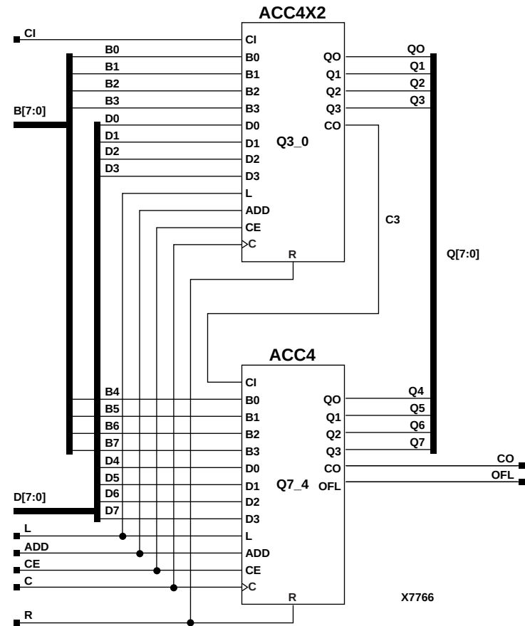
Figure 3-7 ACC8 Implementation XC9000
