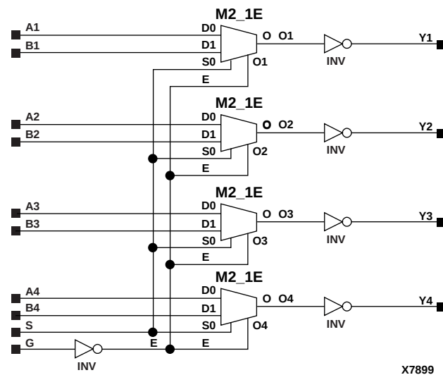
Figure 11-14 X74_158 Implementation XC3000, XC4000E, XC4000X, XC5200, XC9000, Spartan, SpartanXL
