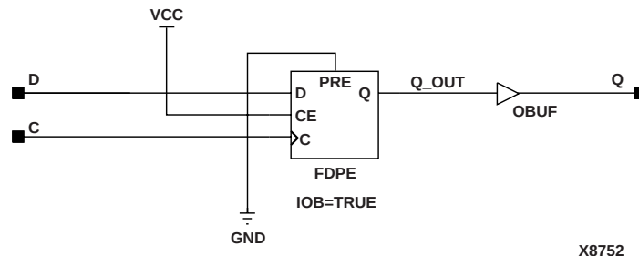
Figure 8-26 OFDI Implementation Spartan2, Virtex
