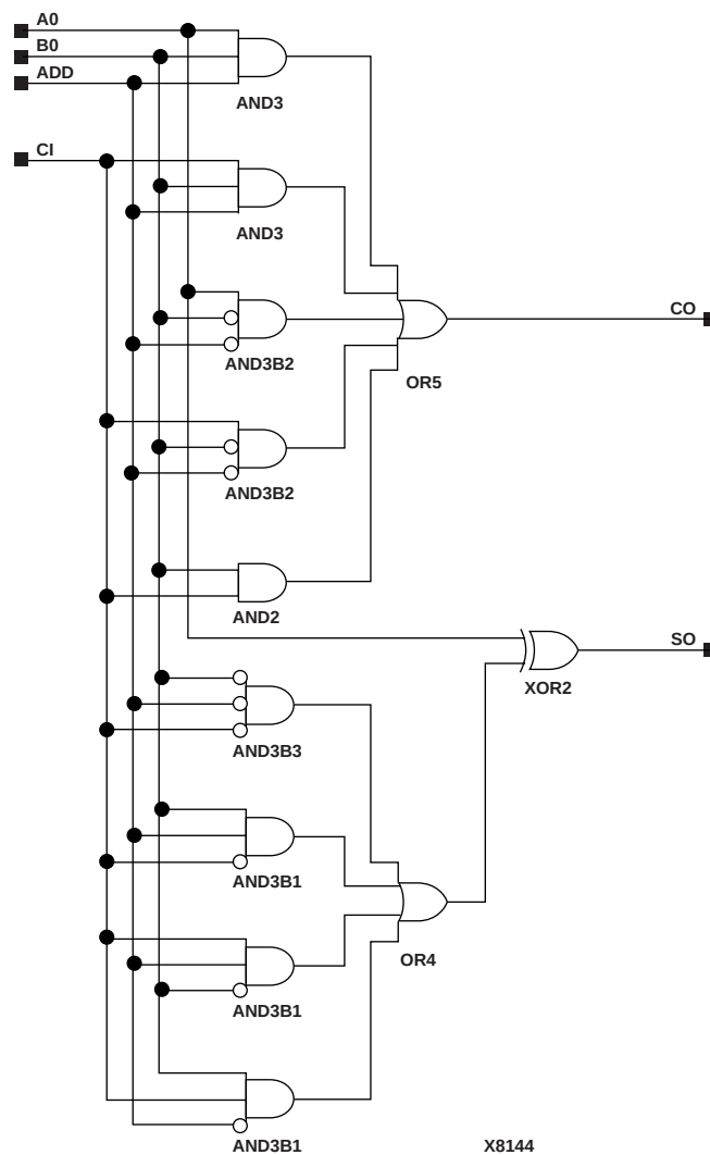
Figure 3-15 ADSU1 Implementation XC9000
