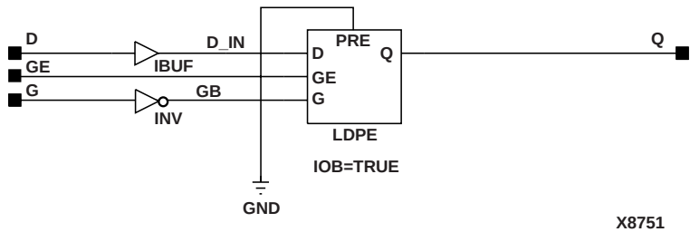
Figure 6-43 ILDXI_1 Implementation Spartan2, Virtex
