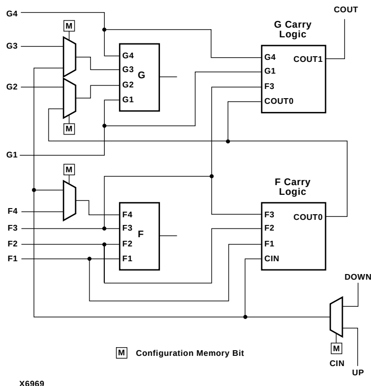
Figure 12-18 XC4000, Spartan, SpartanXL Carry Logic
