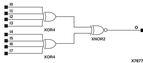
Figure 10-22 XNOR8 Implementation XC9000
