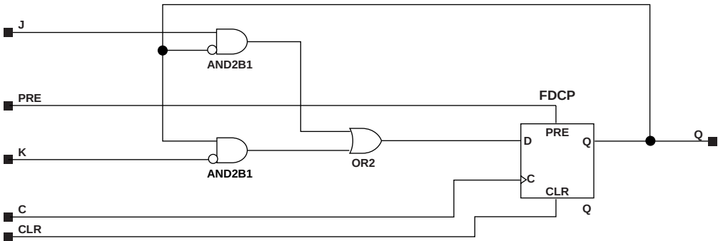
Figure 5-38 FJKCP Implementation XC9000
