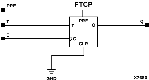
Figure 5-60 FTP Implementation XC9000
