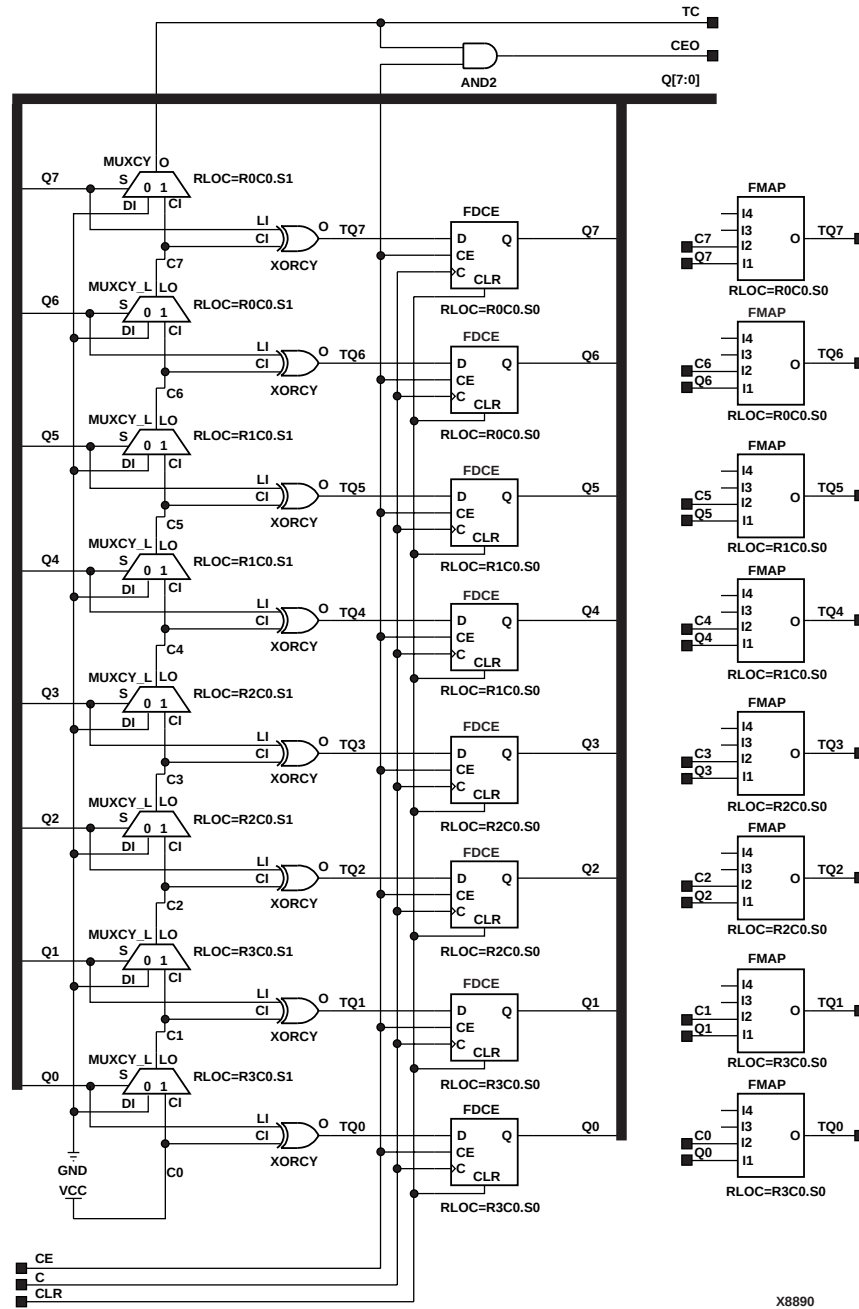
Figure 4-20 CC8CE Implementation Spartan2, Virtex
