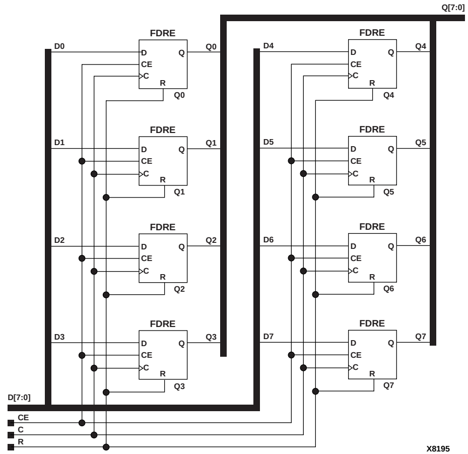
Figure 5-9 FD8RE Implementation XC3000, XC4000E, XC4000X, XC5200, XC9000, Spartan, SpartanXL, Spartan2, Virtex
