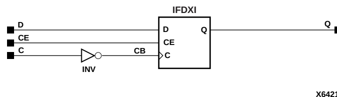
Figure 6-19 IFDXI_1 Implementation XC4000E, XC4000X, Spartan, SpartanXL
