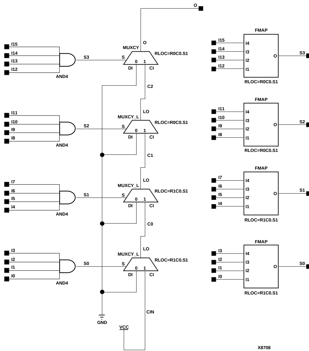
Figure 3-32 AND16 Implementation Spartan2, Virtex
