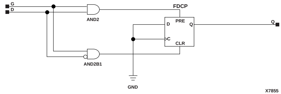
Figure 7-3 LD Implementation XC9000
