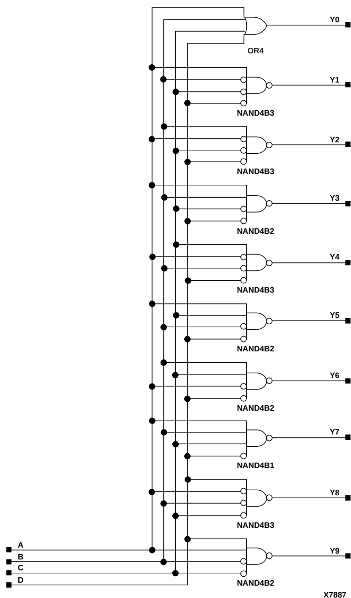
Figure 11-1 X74_42 Implementation XC3000, XC4000E, XC4000X, XC5200, XC9000, Spartan, SpartanXL
