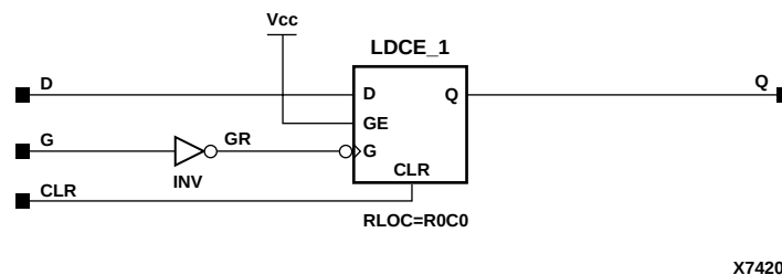
Figure 7-7 LDC Implementation XC4000X, SpartanXL
