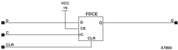
Figure 5-10 FDC Implementation XC3000, XC4000E, XC4000X, XC5200, Spartan, SpartanXL
