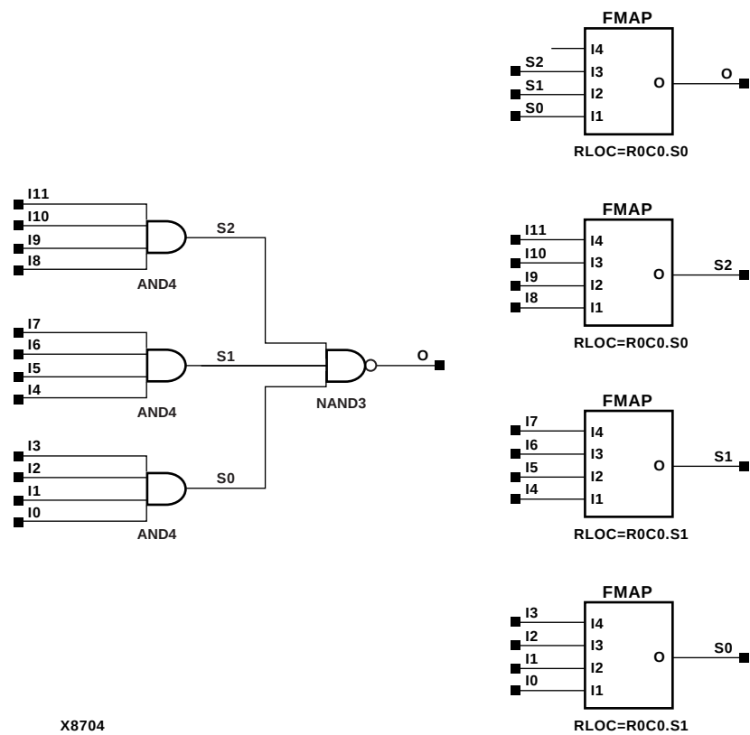
Figure 7-32 NAND12 Implementation Spartan2, Virtex
