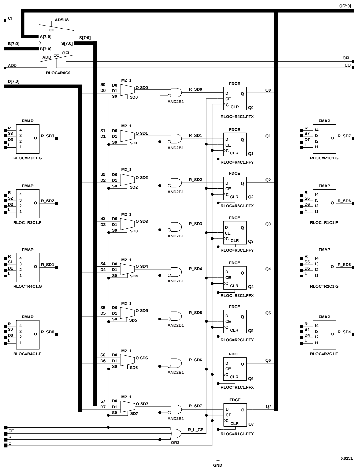
Figure 3-3 ACC8 Implementation XC4000E, XC4000X, Spartan, SpartanXL
