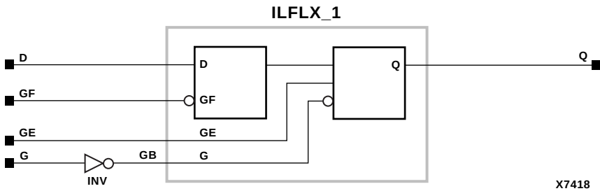
Figure 6-45 ILFLX Implementation XC4000X, SpartanXL
