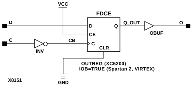
Figure 8-11 OFD_1 Implementation XC5200, Spartan2, Virtex
