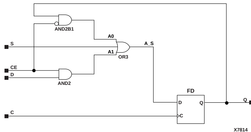
Figure 5-28 FDSE Implementation XC3000, XC4000E, XC4000X, XC5200, Spartan, SpartanXL
