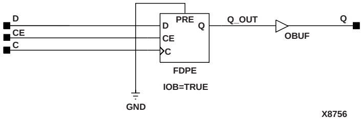
Figure 8-44 OFDXI Implementation Spartan2, Virtex
