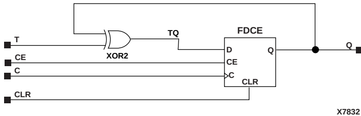
Figure 5-51 FTCE Implementation XC3000, XC4000E, XC4000X, XC5200, Spartan, SpartanXL, Spartan2, Virtex
