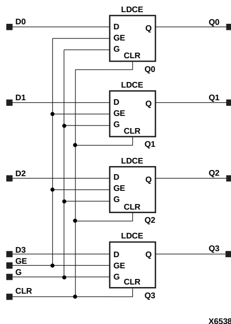
Figure 7-13 LD4CE Implementation XC4000X, XC5200, SpartanXL, Spartan2, Virtex
