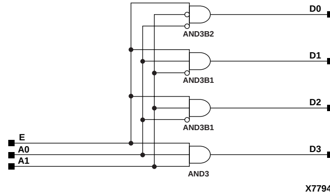
Figure 4-54 D2_4E Implementation XC3000, XC4000E, XC4000X, XC5200, XC9000, Spartan, SpartanXL, Spartan2, Virtex
