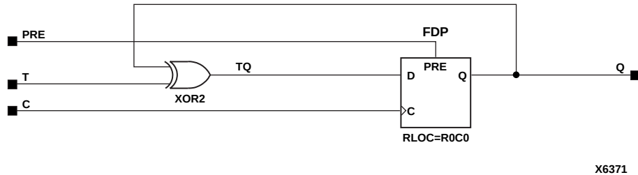
Figure 5-59 FTP Implementation XC4000E, XC4000X, XC5200, Spartan, SpartanXL, Spartan2, Virtex
