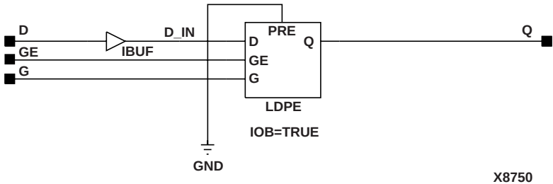
Figure 6-42 ILDXI Implementation Spartan2, Virtex
