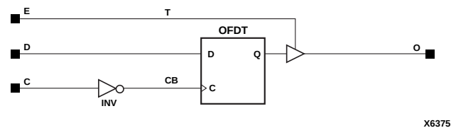
Figure 8-33 OFDT_1 Implementation XC3000, XC4000E, XC4000X, Spartan, SpartanXL
