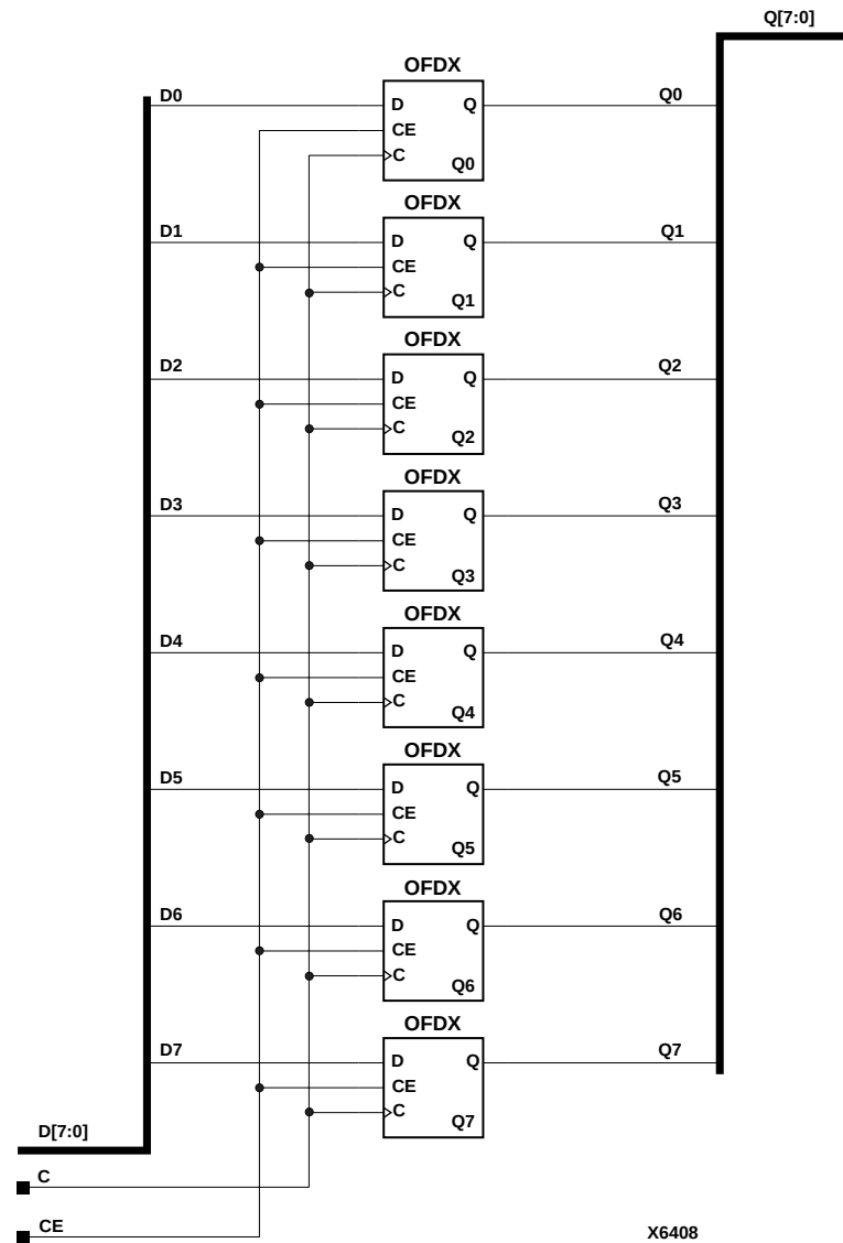
Figure 8-41 OFDX8 Implementation XC4000E, XC4000X, Spartan, SpartanXL, Spartan2, Virtex
