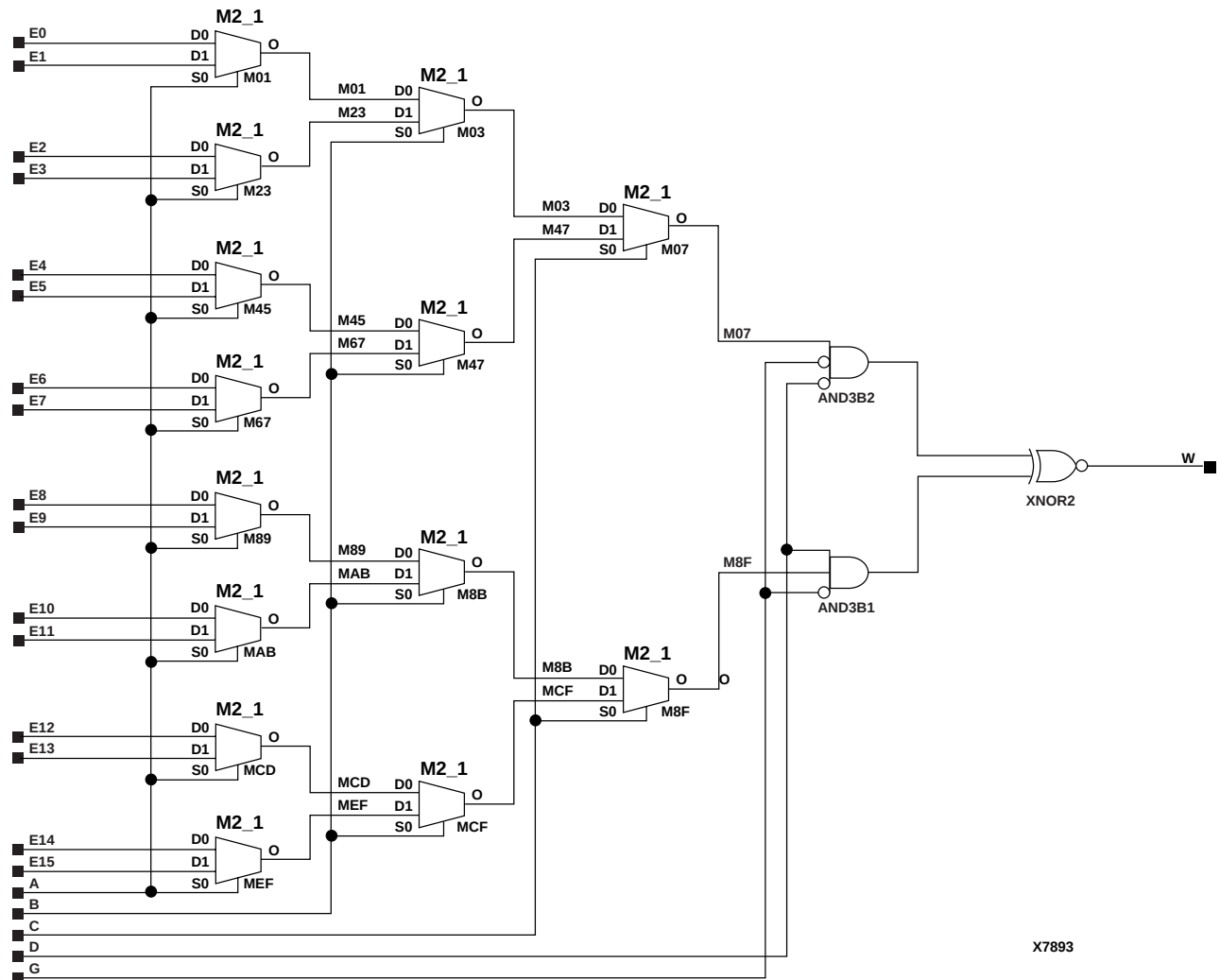
Figure 11-8 X74_150 Implementation XC3000, XC4000E, XC4000X, XC5200, XC9000, Spartan, SpartanXL
