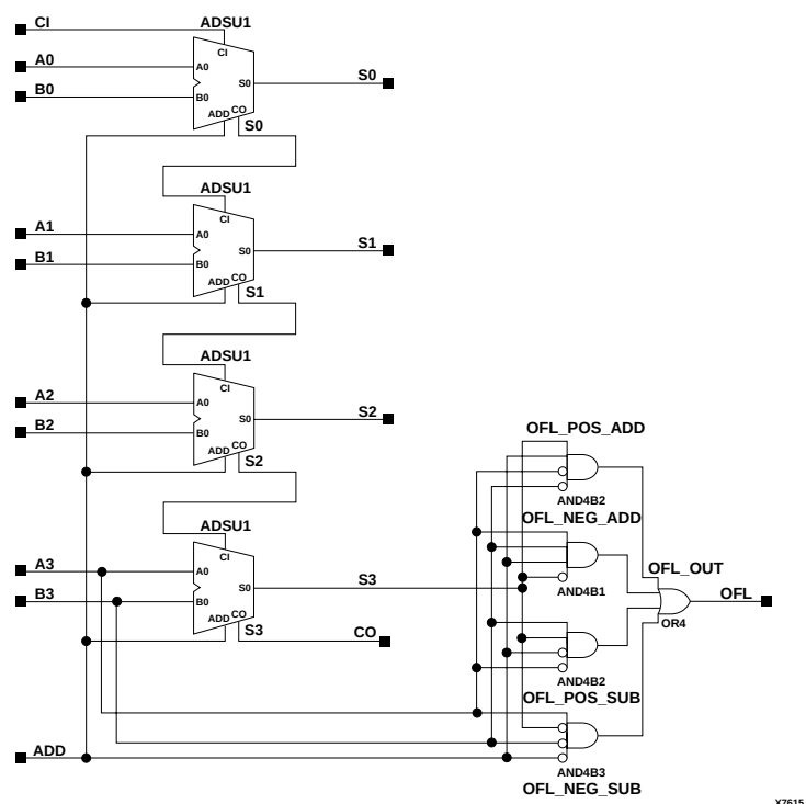
Figure 3-21 ADSU4 Implementation XC9000
