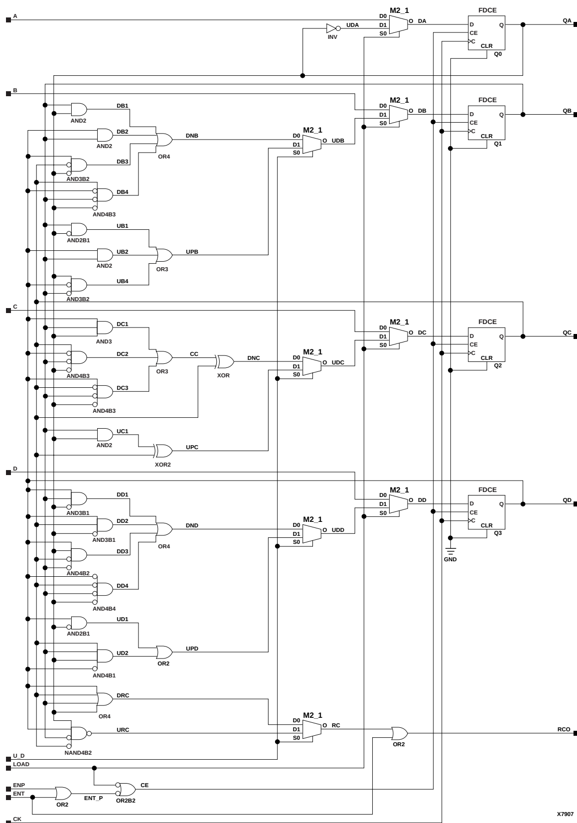
Figure 11-28 X74_168 Implementation XC3000, XC4000E, XC4000X, XC5200, Spartan, SpartanXL
