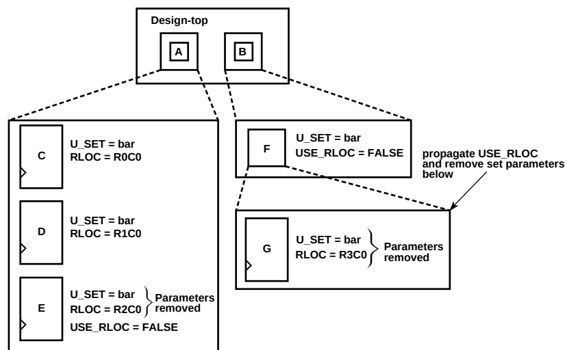
Figure 12-13 Using the USE_RLOC Constraint to Control RLOC Application on U_SET Sets
