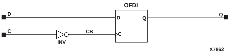
Figure 8-27 OFDI_1 Implementation XC4000E, XC4000X, Spartan, SpartanXL
