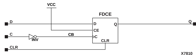
Figure 5-12 FDC_1 Implementation XC3000, XC4000E, XC4000X, XC5200, Spartan, SpartanXL
