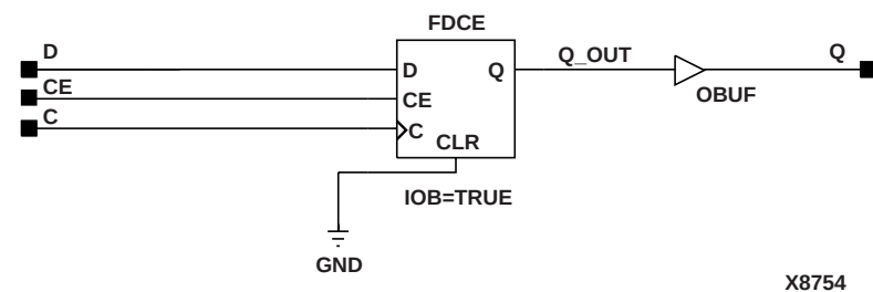
Figure 8-40 OFDX Implementation Spartan2, Virtex
