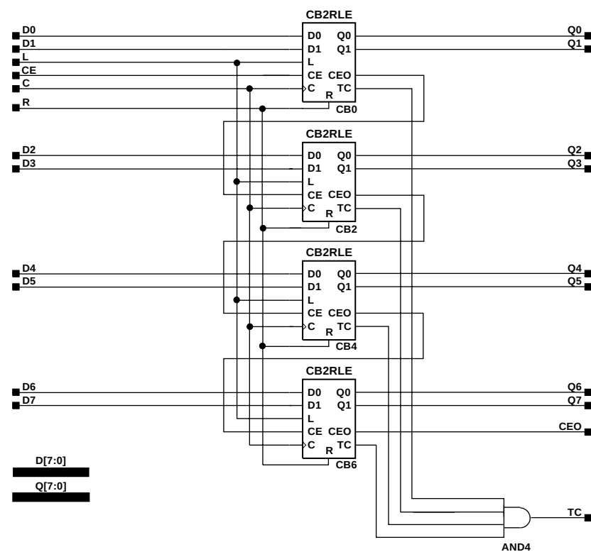
Figure 4-14 CB2RLE Implementation XC9000
