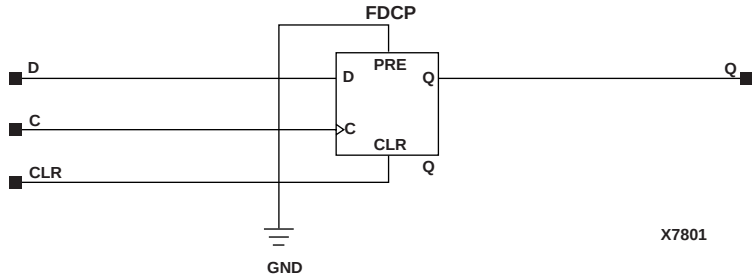
Figure 5-11 FDC Implementation XC9000
