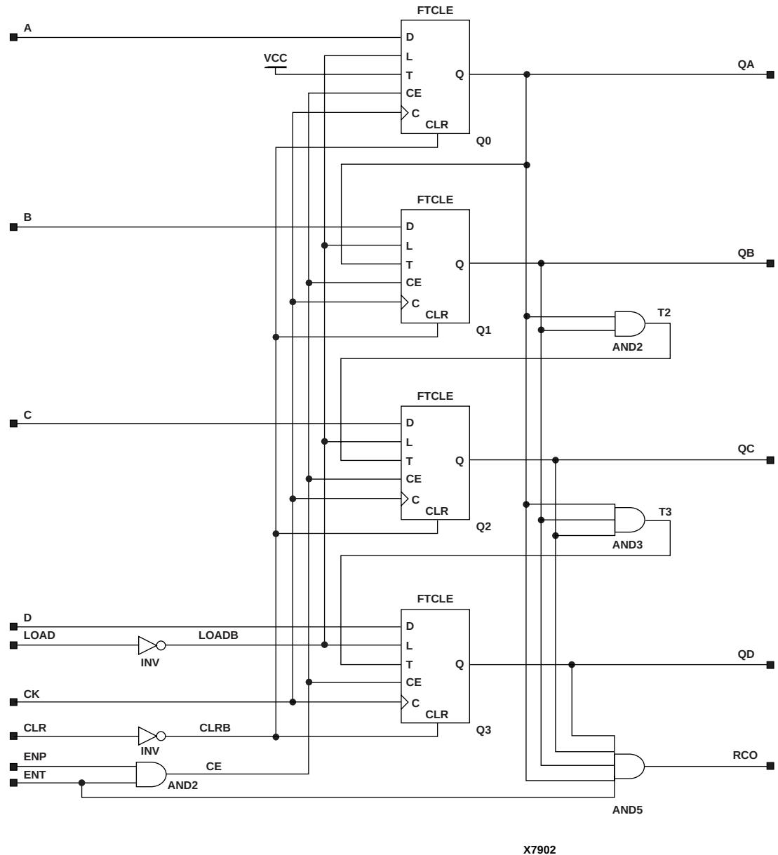
Figure 11-19 X74_161 Implementation XC3000, XC4000E, XC4000X, XC5200, Spartan, SpartanXL
