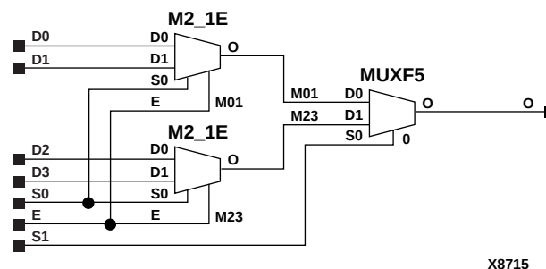
Figure 7-21 M4_1E Implementation Spartan2, Virtex
