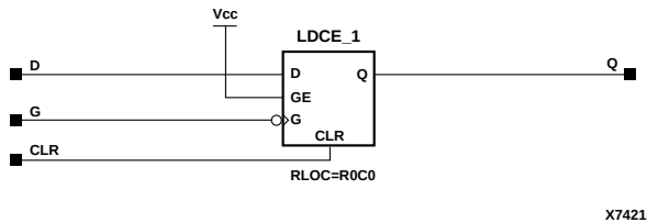
Figure 7-9 LDC_1 Implementation XC4000X, SpartanXL
