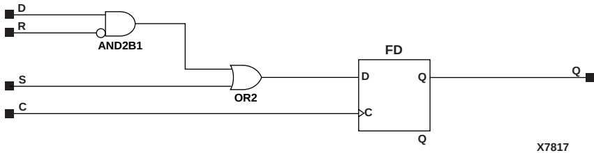
Figure 5-31 FDSR Implementation XC9000
