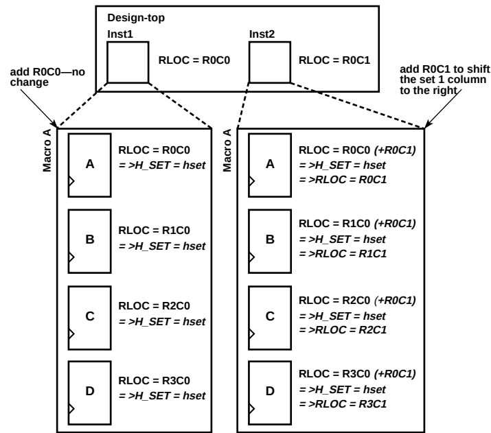
Figure 12-8 Modifying RLOC Values of Same Macro and Linking Together as One Set
