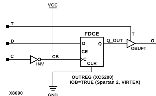
Figure 8-34 OFDT_1 Implementation XC5200, Spartan2, Virtex
