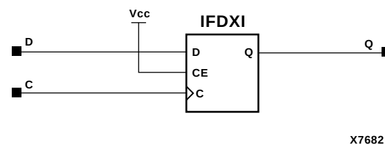
Figure 6-10 IFDI Implementation XC4000E, XC4000X, Spartan, SpartanXL
