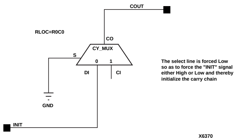
Figure 4-52 CY_INIT 4-Bit Adder Implementation XC5200
