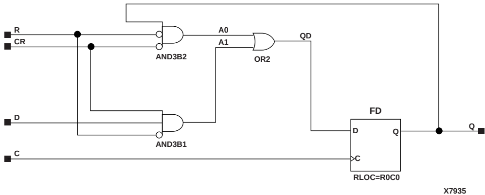
Figure 5-21 FDRE Implementation XC3000, XC4000E, XC4000X, XC5200, Spartan, SpartanXL
