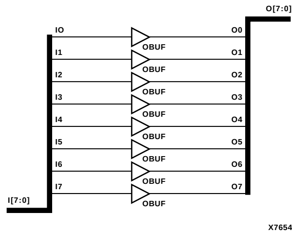
Figure 8-1 OBUF8 Implementation XC3000, XC4000E, XC4000X, XC5200, XC9000, Spartan, SpartanXL, Spartan2, Virtex
