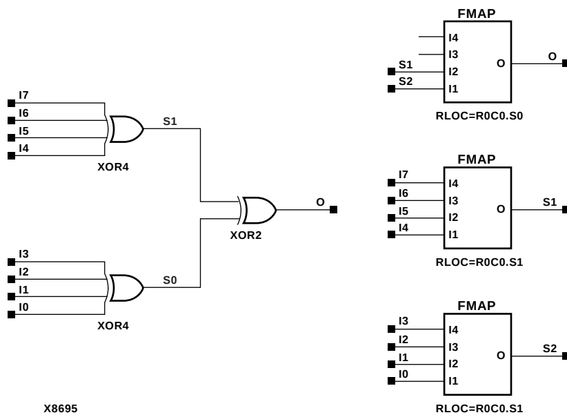
Figure 10-36 XOR8 Implementation Spartan2, Virtex
