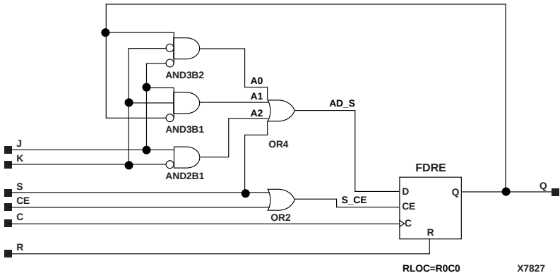
Figure 5-44 FJKRSE Implementation XC3000, XC4000E, XC4000X, XC5200, Spartan, SpartanXL, Spartan2, Virtex
