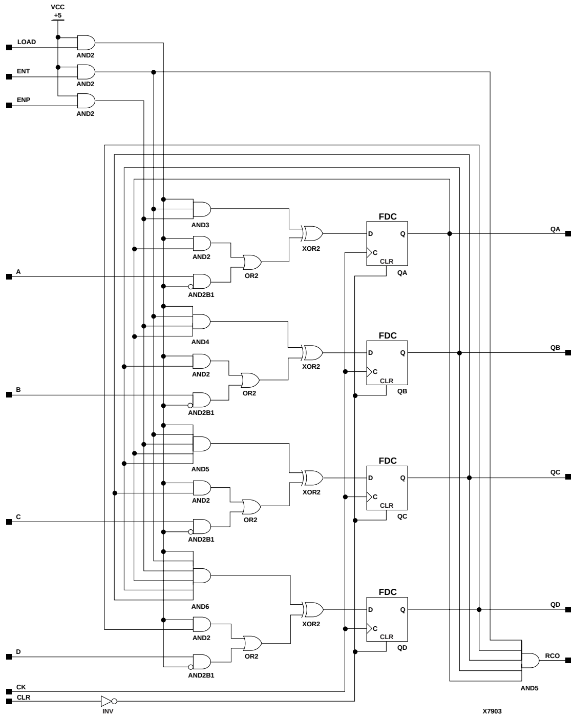
Figure 11-20 X74_161 Implementation XC9000
