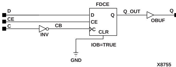
Figure 8-43 OFDX_1 Implementation Spartan2, Virtex
