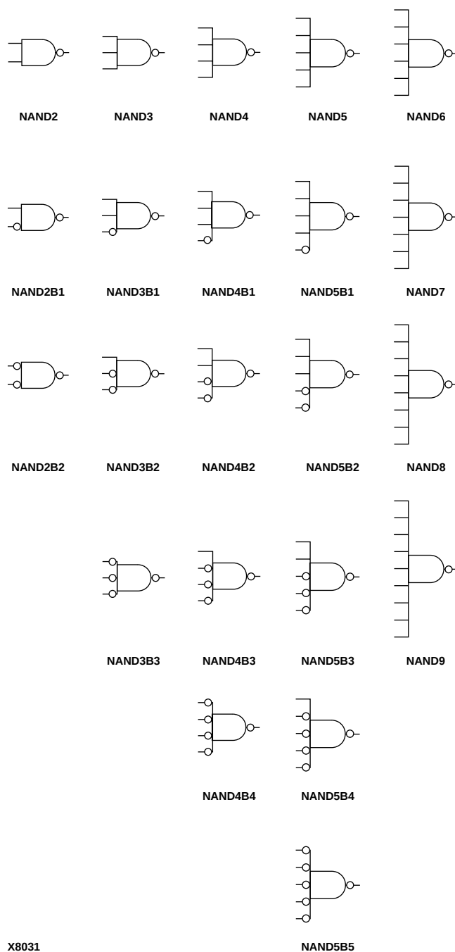
Figure 7-25 NAND Gate Representations
