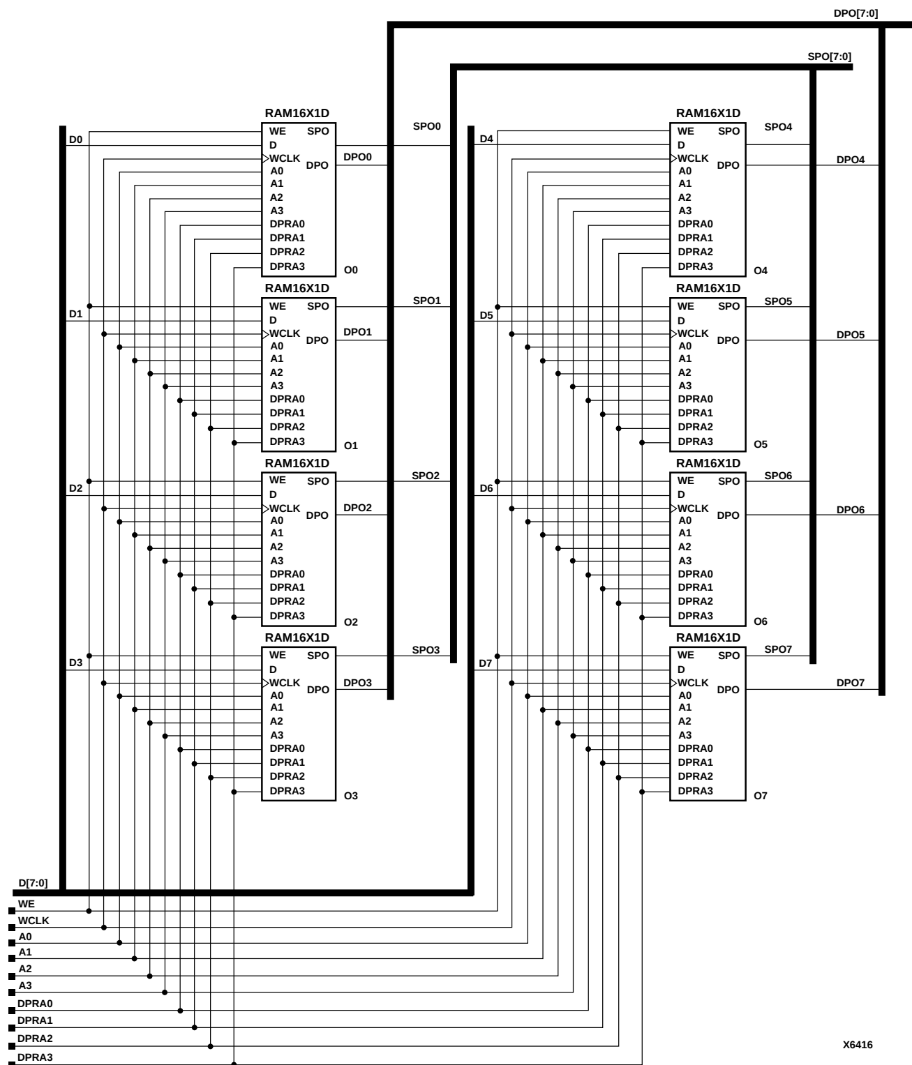
Figure 9-4 RAM16X8D Implementation XC4000E, XC4000X, Spartan, SpartanXL
