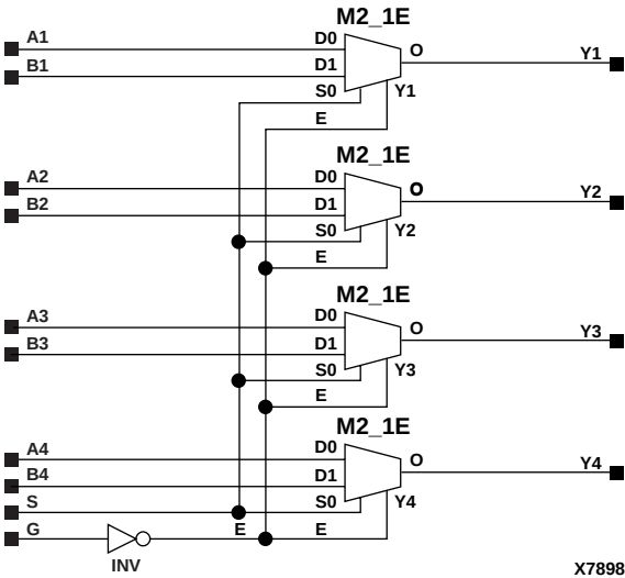
Figure 11-13 X74_157 Implementation XC3000, XC4000E, XC4000X, XC5200, XC9000, Spartan, SpartanXL
