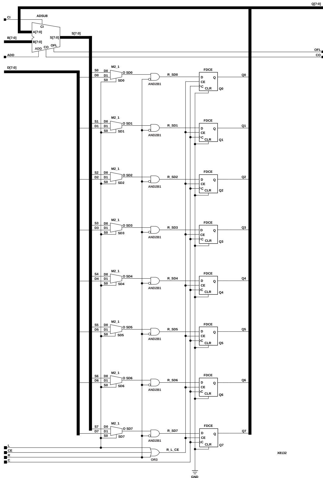
Figure 3-2 ACC8 Implementation XC3000
