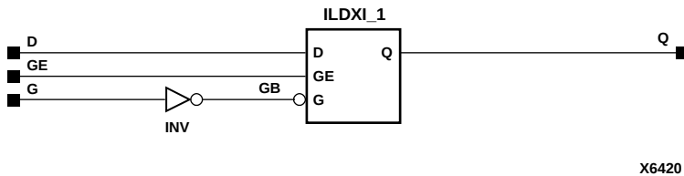
Figure 6-41 ILDXI Implementation XC4000E, XC4000X, Spartan, SpartanXL
