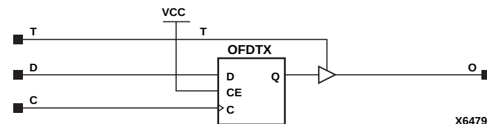
Figure 8-29 OFDT Implementation XC4000E, XC4000X, Spartan, SpartanXL
