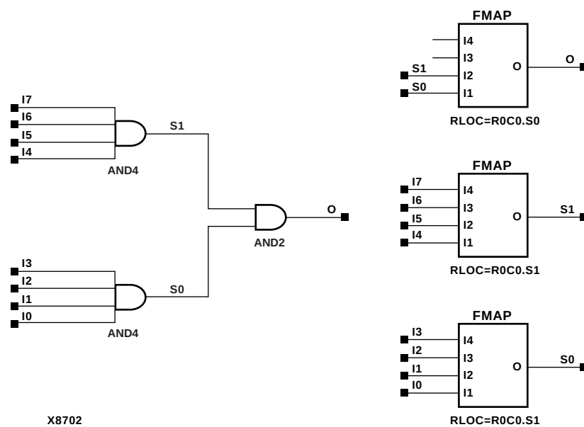
Figure 3-28 AND8 Implementation Spartan2, Virtex
