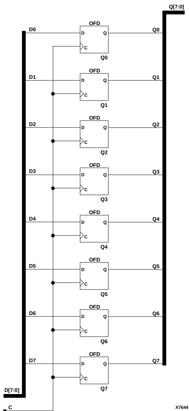
Figure 8-8 OFD8 Implementation XC3000, XC4000E, XC4000X, XC5200, Spartan, SpartanXL, Spartan2, Virtex
