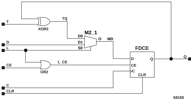
Figure 5-53 FTCLE Implementation XC3000
