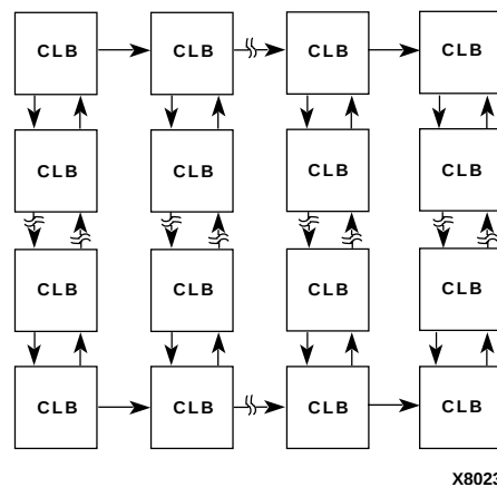
Figure 12-16 Available XC4000E Carry Propagation Paths
