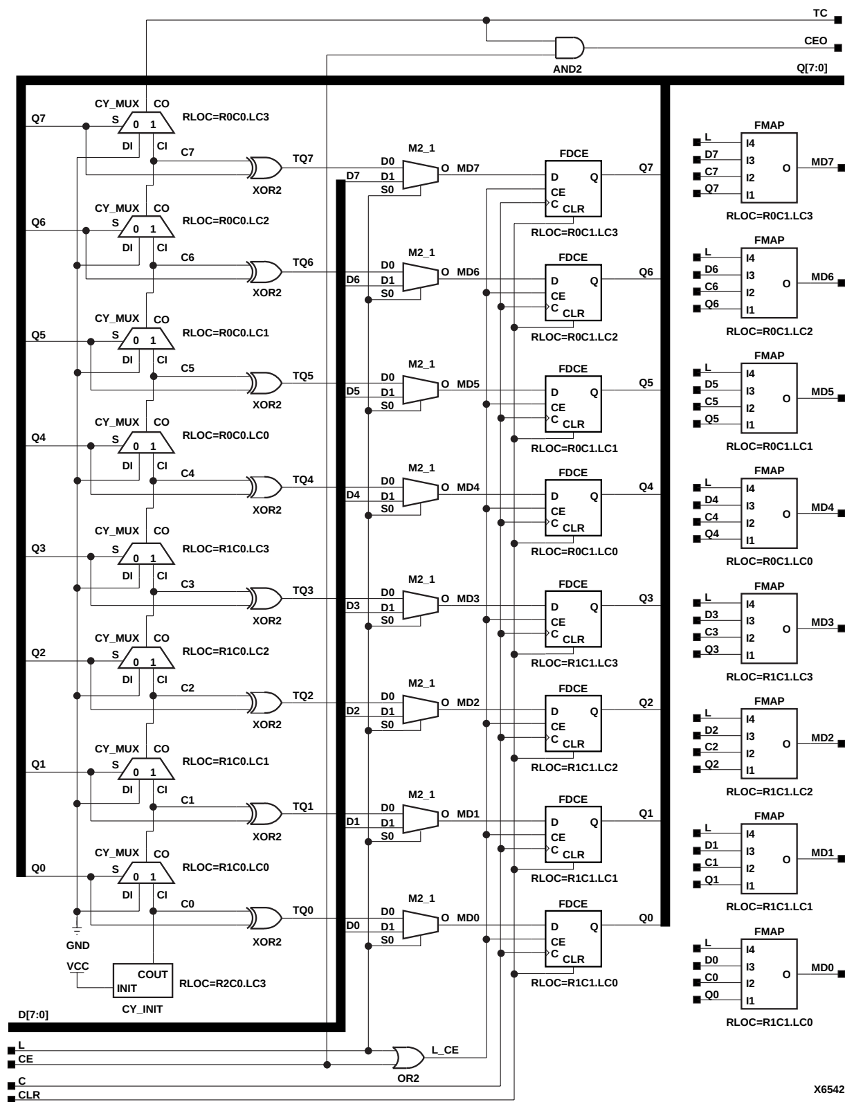
Figure 4-22 CC8CLE Implementation XC5200
