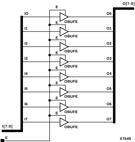
Figure 8-3 OBUFE8 Implementation XC3000, XC4000E, XC4000X, XC5200, XC9000, Spartan, SpartanXL, Spartan2, Virtex
