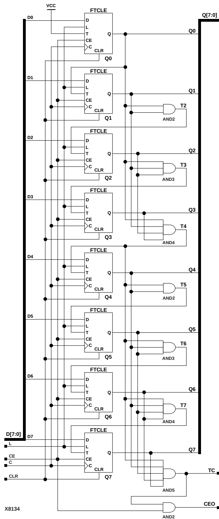
Figure 4-4 CB8CLE Implementation XC3000
