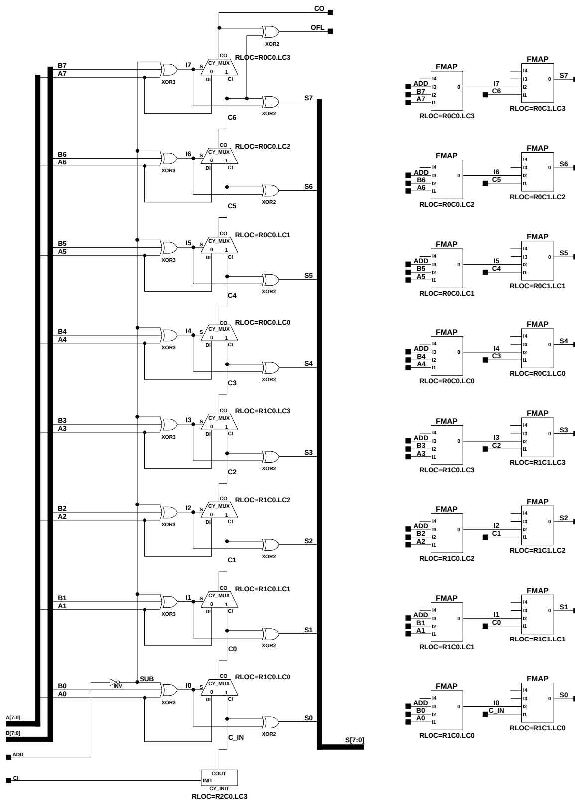
Figure 3-19 ADSU8 Implementation XC5200
