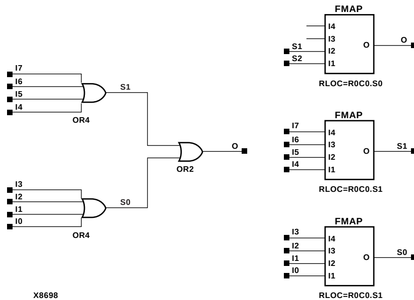
Figure 8-52 OR8 Implementation Spartan2, Virtex
