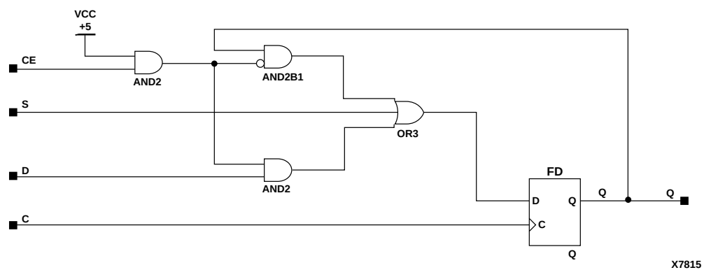
Figure 5-29 FDSE Implementation XC9000
