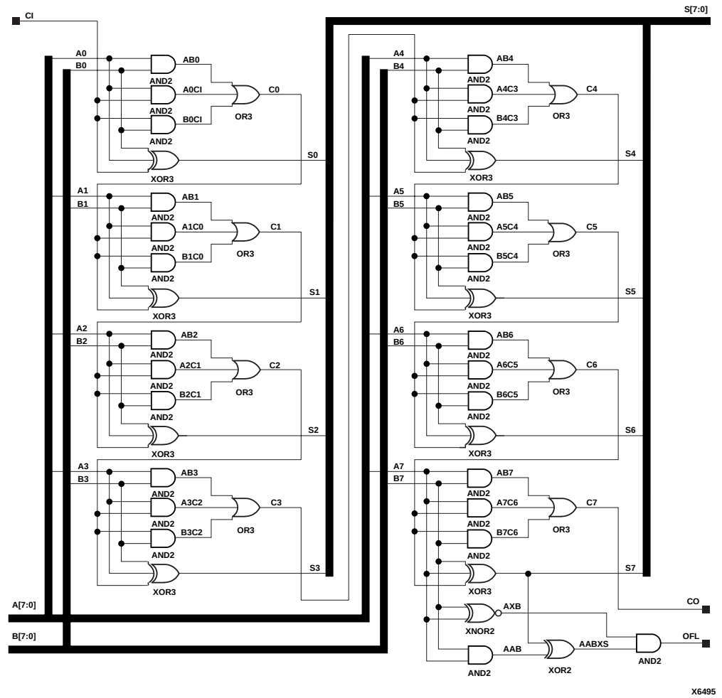
Figure 3-9 ADD8 Implementation XC3000
