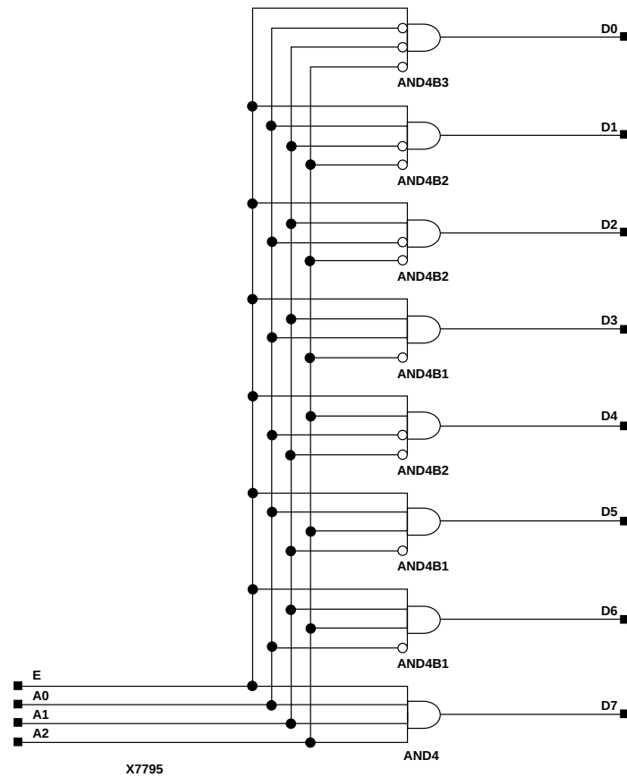
Figure 4-55 D3_8E Implementation XC3000, XC4000E, XC4000X, XC5200, XC9000, Spartan, SpartanXL, Spartan2, Virtex
