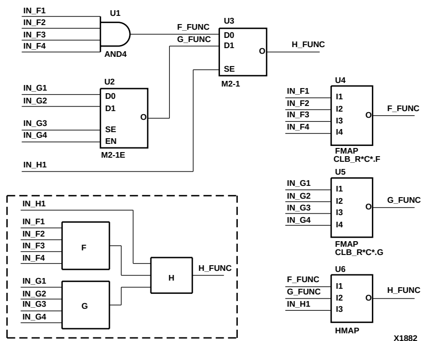
Figure 5-48 Partitioning Logic Using FMAP and HMAP Symbols
