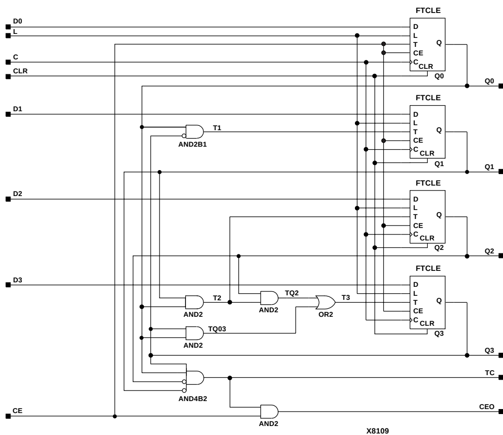
Figure 4-32 CD4CLE Implementation XC3000
