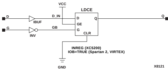
Figure 6-29 ILD_1 Implementation XC5200, Spartan2, Virtex
