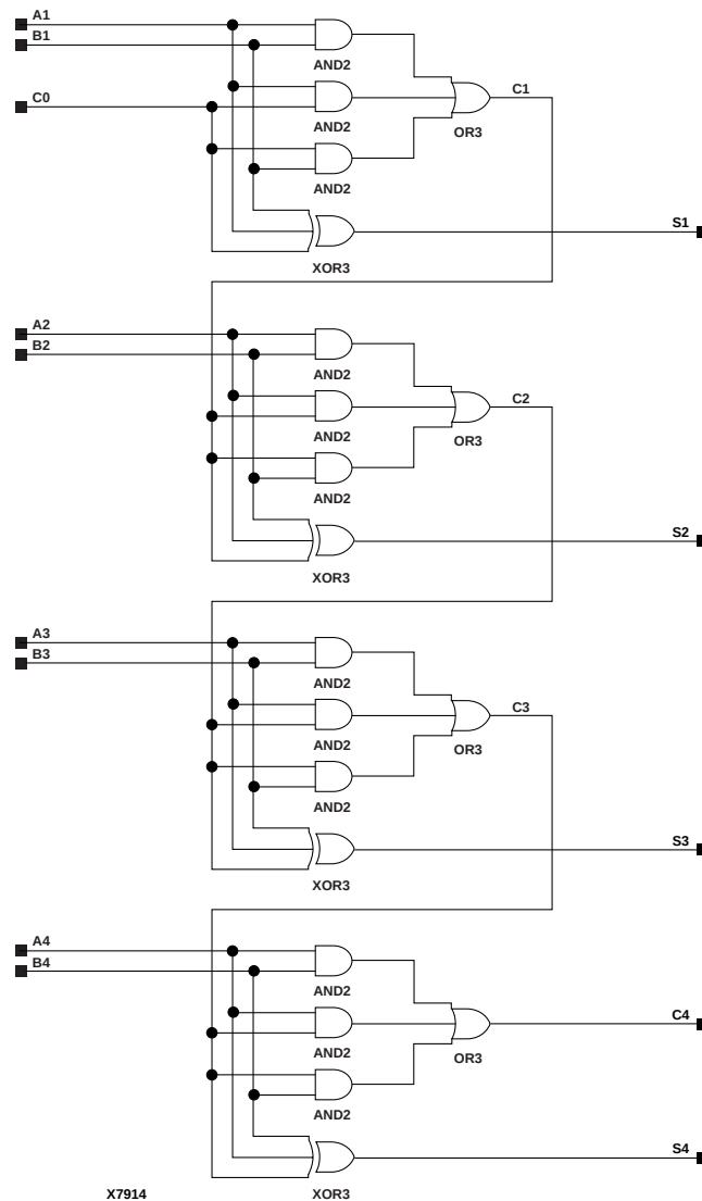
Figure 11-36 X74_283 Implementation XC3000, XC4000E, XC4000X, XC5200, Spartan, SpartanXL
