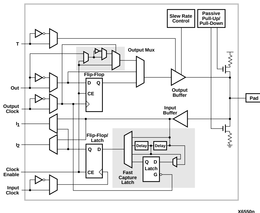
Figure 6-44 Block Diagram of XC4000X IOB
