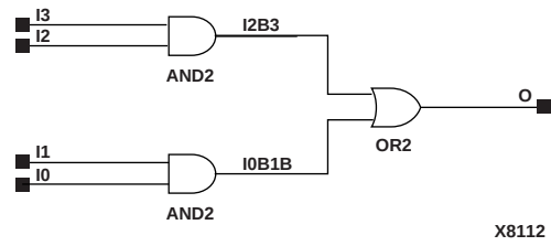
Figure 10-3 SOP4 Implementation XC3000, XC4000E, XC4000X, XC5200, XC9000, Spartan, SpartanXL, Spartan2, Virtex
