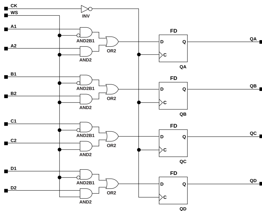
Figure 11-39 X74_298 Implementation XC9000
