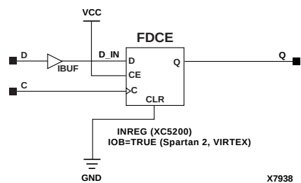
Figure 6-5 IFD Implementation XC5200, Spartan2, Virtex
