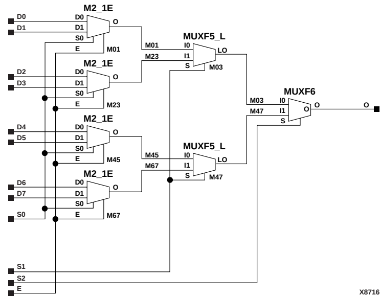
Figure 7-23 M8_1E Implementation Spartan2, Virtex
