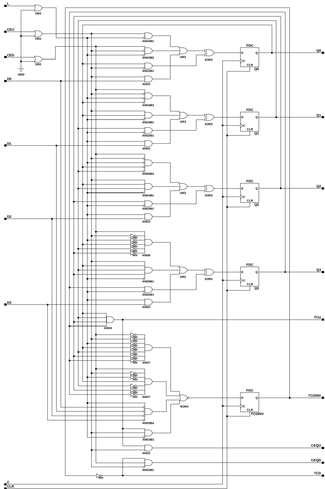
Figure 4-16 CB4X1 Implementation XC9000
