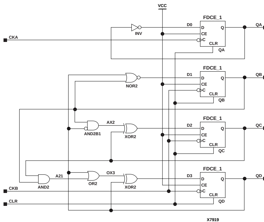
Figure 11-42 X74_390 Implementation XC3000, XC4000E, XC4000X, XC5200, Spartan, SpartanXL
