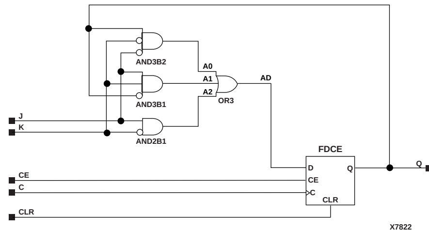
Figure 5-36 FJKCE Implementation XC3000, XC4000E, XC4000X, XC5200, Spartan, SpartanXL, Spartan2, Virtex
