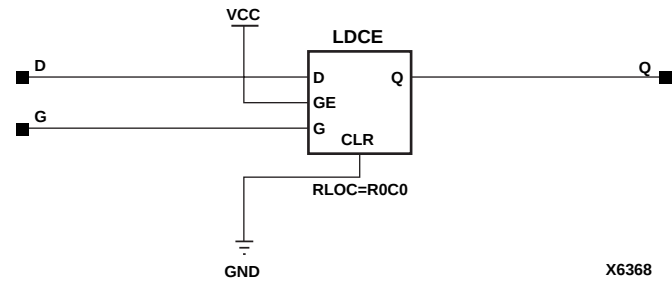
Figure 7-2 LD Implementation XC5200
