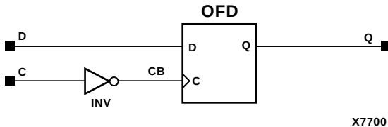
Figure 8-10 OFD_1 Implementation XC3000, XC4000E, XC4000X, Spartan, SpartanXL
