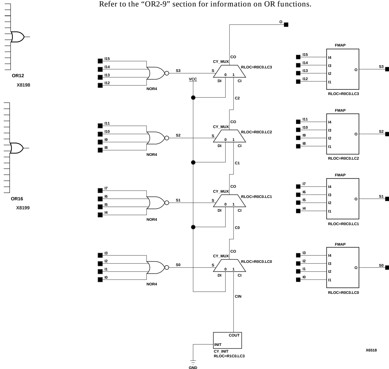
Figure 8-53 OR16 Implementation XC5200
