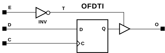
Figure 8-18 OFDEI Implementation XC4000E, XC4000X, Spartan, SpartanXL
