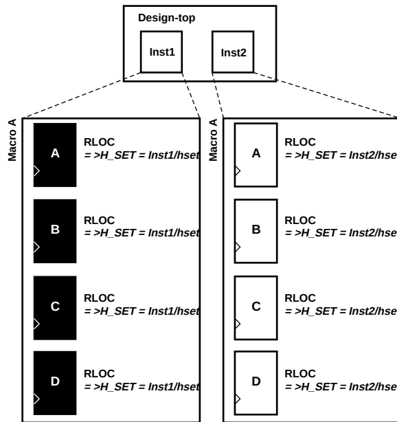
Figure 12-5 Macro A Instantiated Twice
