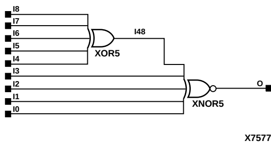
Figure 10-24 XNOR9 Implementation XC3000
