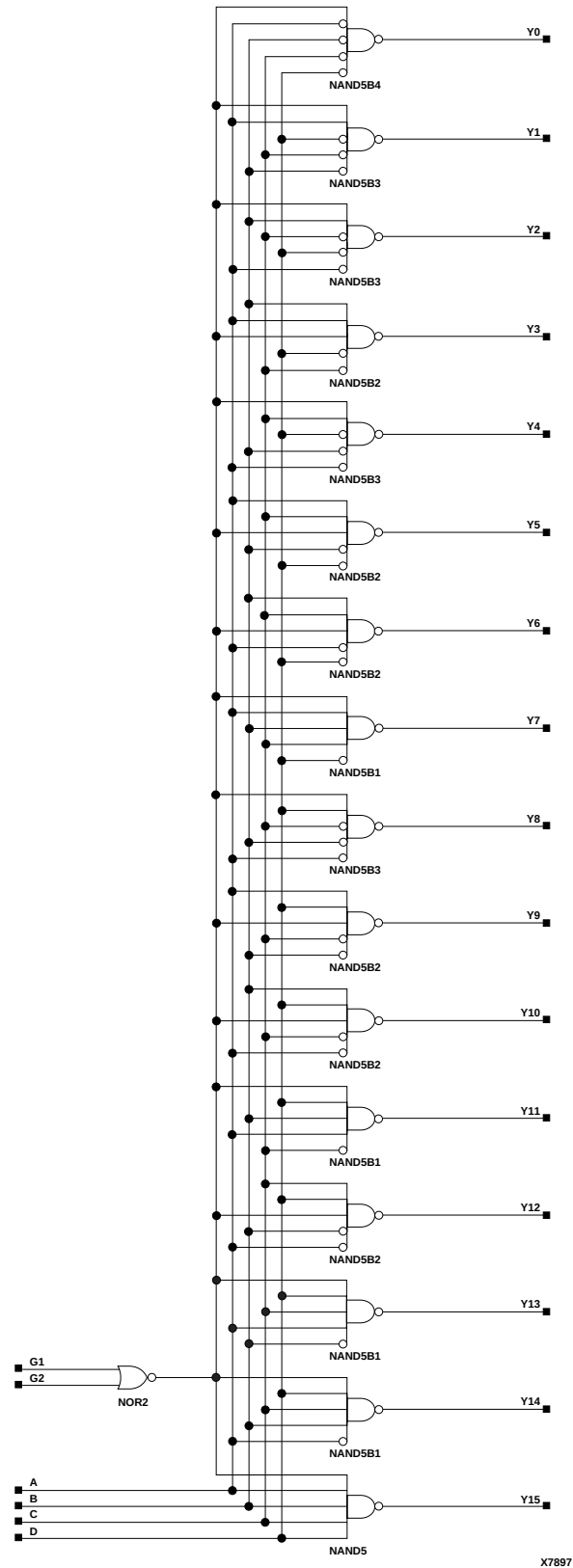
Figure 11-12 X74_154 Implementation XC3000, XC4000E, XC4000X, XC5200, XC9000, Spartan, SpartanXL
