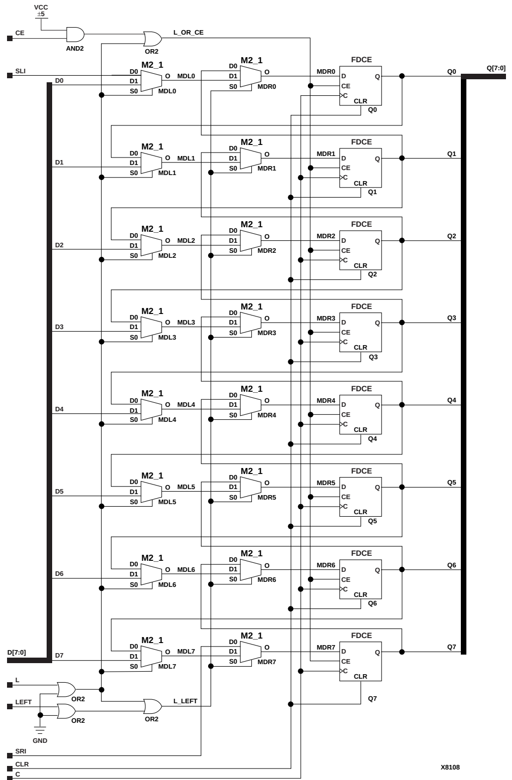
Figure 10-7 SR8CLED Implementation XC9000
