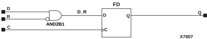
Figure 5-20 FDR Implementation XC3000, XC4000E, XC4000X, XC5200, XC9000, Spartan, SpartanXL
