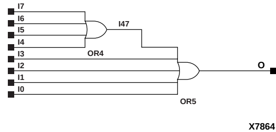
Figure 8-50 OR8 Implementation XC3000
