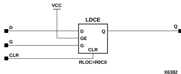
Figure 7-8 LDC Implementation XC5200
