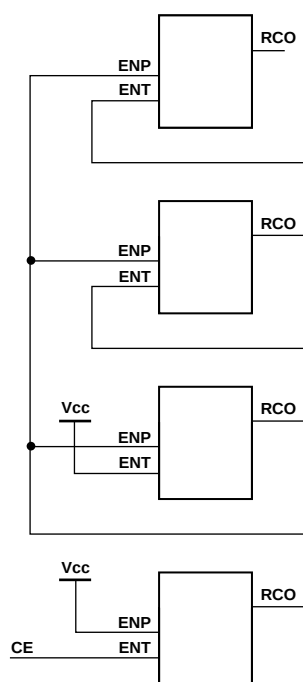
Figure 11-15 Carry-Lookahead Design
