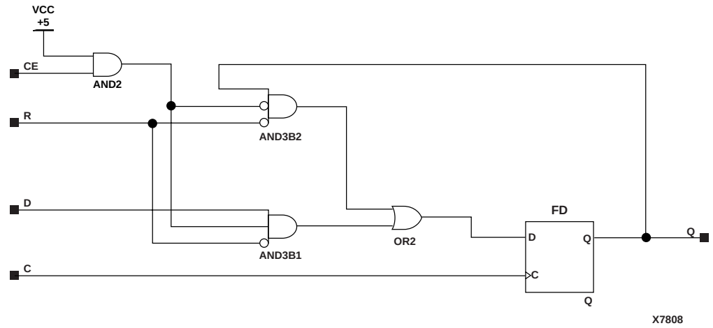
Figure 5-22 FDRE Implementation XC9000
