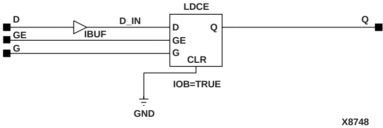
Figure 6-37 ILDX Implementation Spartan2, Virtex
