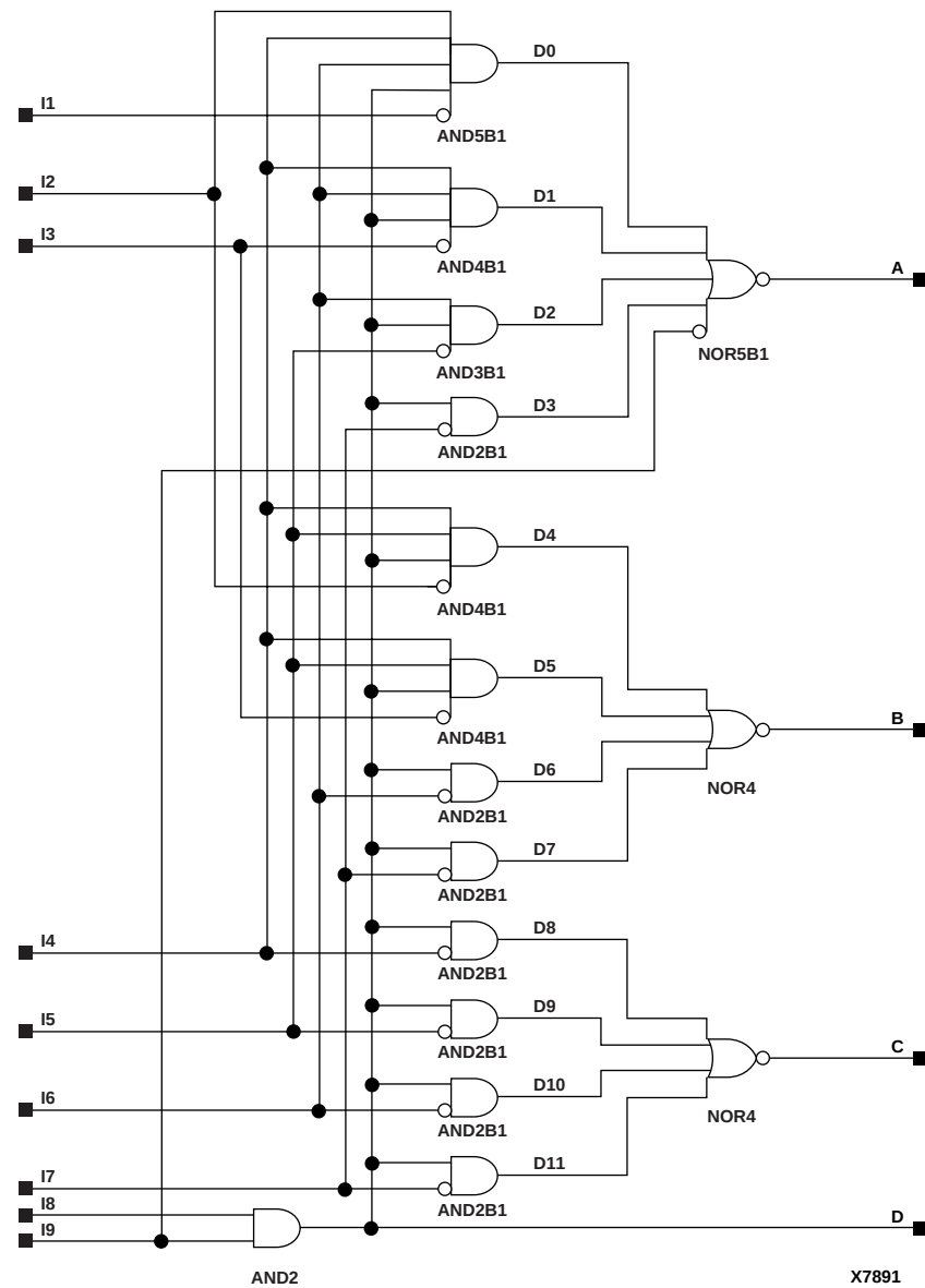
Figure 11-6 X74_147 Implementation XC3000, XC4000E, XC4000X, XC5200, XC9000, Spartan, SpartanXL
