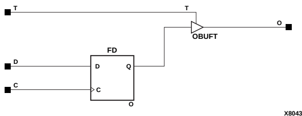
Figure 8-31 OFDT Implementation XC9000
