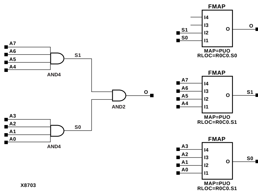
Figure 4-63 DECODE8 Implementation Spartan2, Virtex
