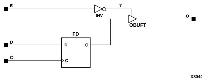
Figure 8-14 OFDE Implementation XC9000
