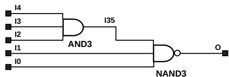
Figure 7-26 NAND5 Implementation XC5200
