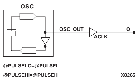
Figure 6-1 GXTL Implementation XC3000
