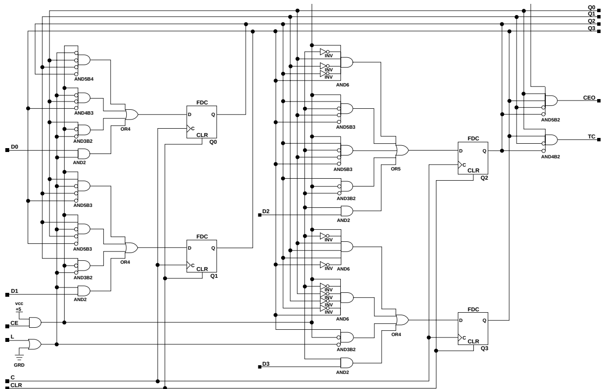
Figure 4-33 CD4CLE Implementation XC4000E, XC4000X, XC5200, Spartan, SpartanXL, Spartan2, Virtex
