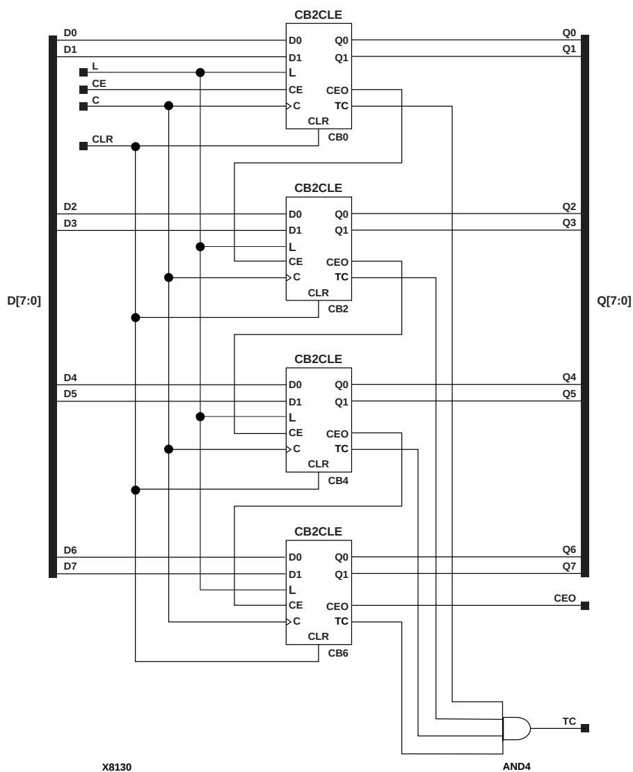
Figure 4-7 CB8CLE Implementation XC9000
