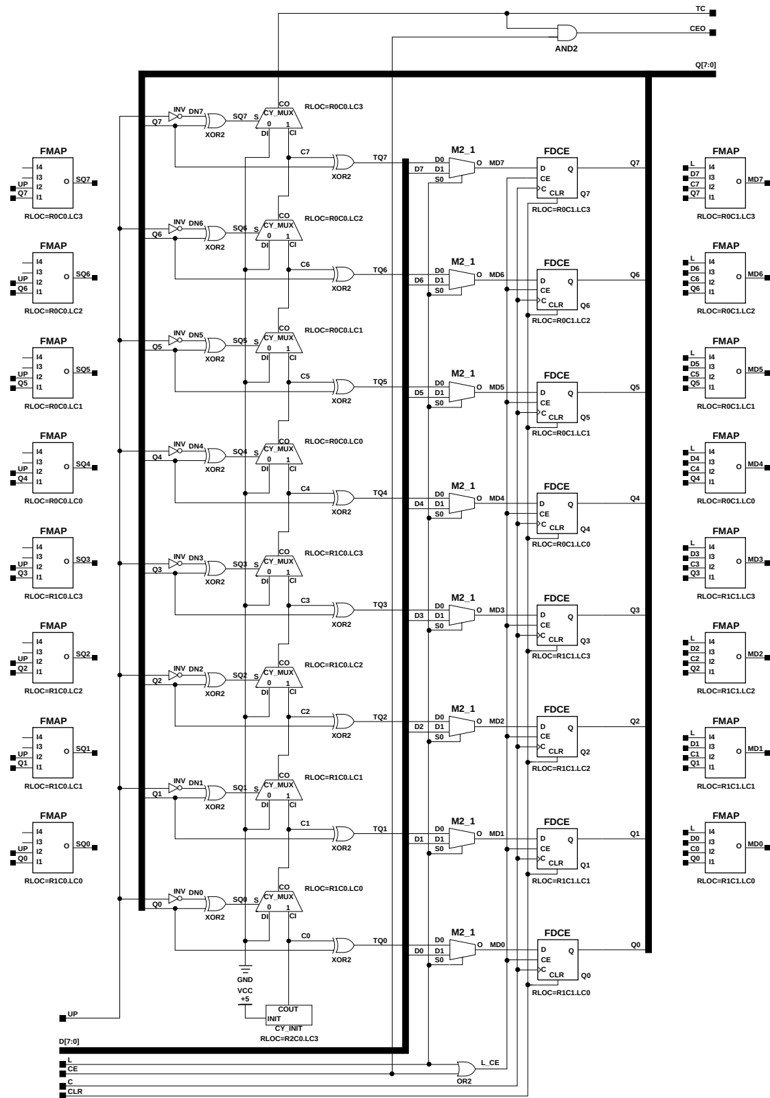
Figure 4-25 CC8CLED Implementation XC5200
