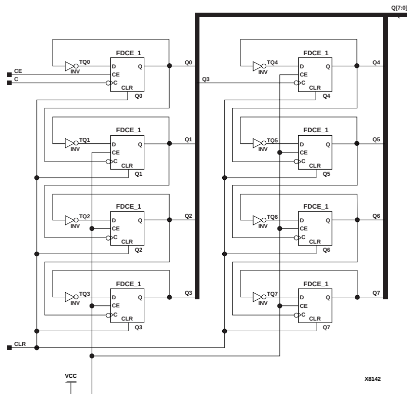
Figure 4-50 CR8CE Implementation XC4000E, XC4000X, XC5200, Spartan, SpartanXL, Spartan2, Virtex
