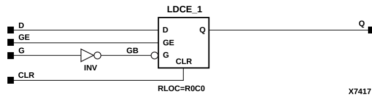
Figure 7-11 LDCE Implementation XC4000X, SpartanXL
