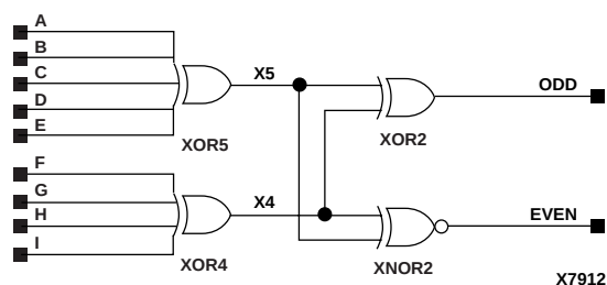
Figure 11-34 X74_280 Implementation XC3000, XC4000E, XC4000X, XC5200, Spartan, SpartanXL
