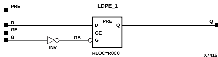
Figure 7-15 LDPE Implementation XC4000X, SpartanXL
