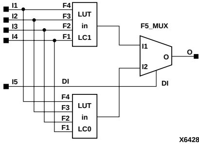
Figure 5-1 Two LUTs in Parallel Combined to Create a 5-Input Function
