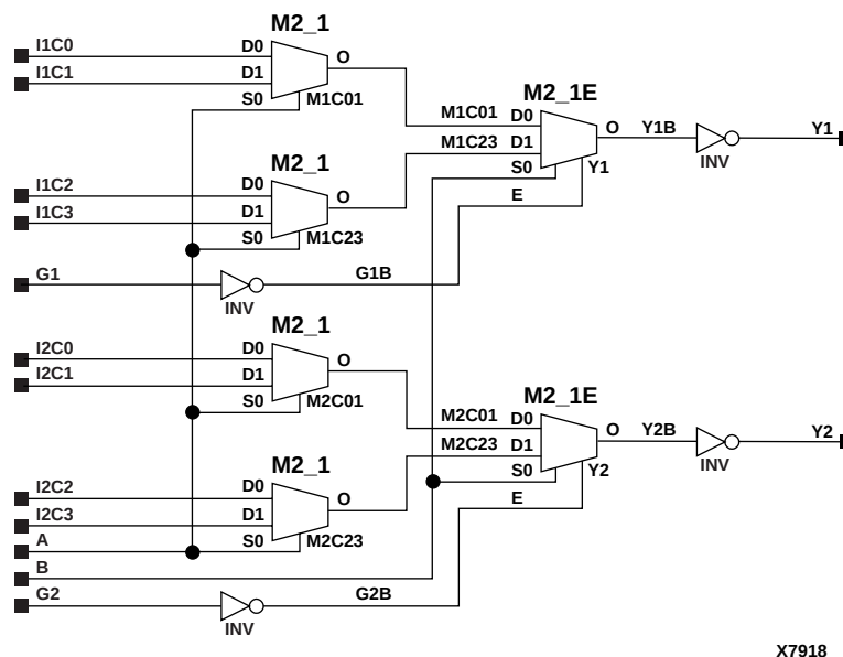
Figure 11-40 X74_352 Implementation XC3000, XC4000E, XC4000X, XC5200, XC9000, Spartan, SpartanXL
