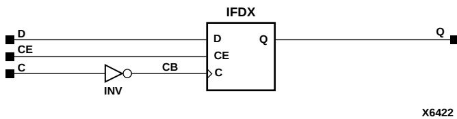
Figure 6-16 IFDX_1 Implementation XC4000E, XC4000X, Spartan, SpartanXL
