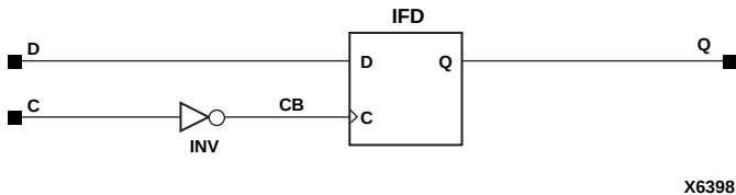
Figure 6-8 IFD_1 Implementation XC3000, XC4000E, XC4000X, Spartan, SpartanXL
