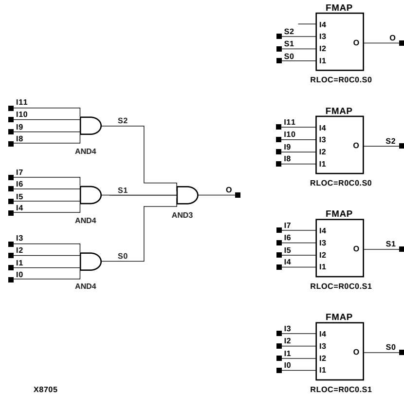
Figure 3-30 AND12 Implementation Spartan2, Virtex
