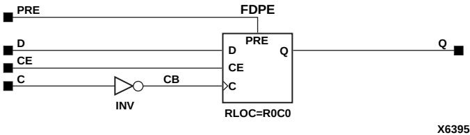
Figure 5-19 FDPE_1 Implementation XC4000E, XC4000X, XC5200, Spartan, SpartanXL
