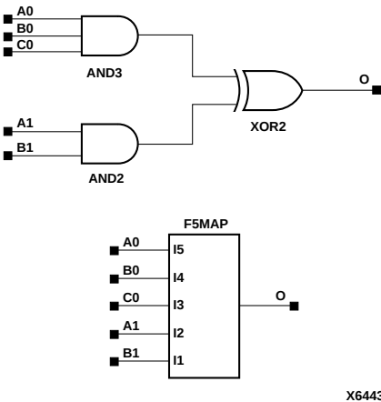
Figure 5-2 F5MAP Primitive Example
