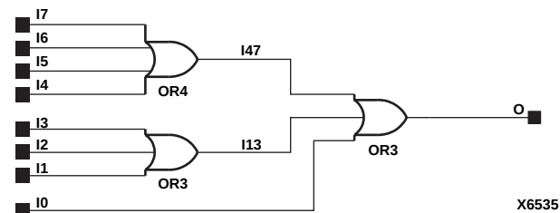
Figure 8-51 OR8 Implementation XC4000E, XC4000X, XC5200, Spartan, SpartanXL
