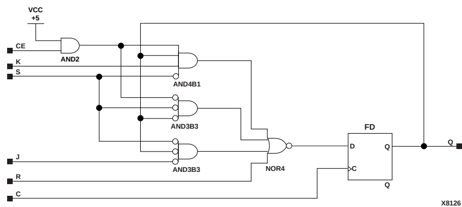
Figure 5-45 FJKRSE Implementation XC9000
