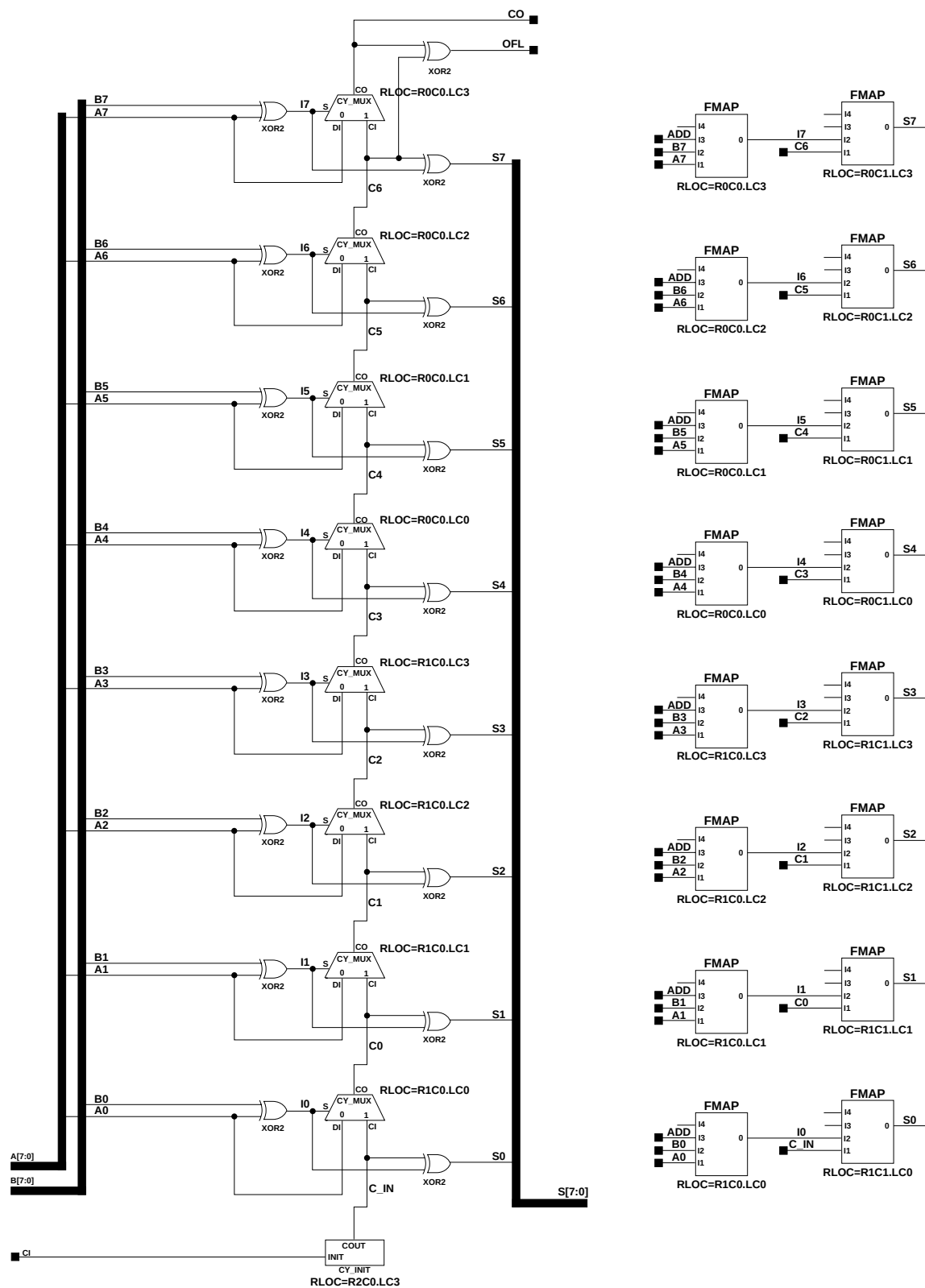
Figure 3-11 ADD8 Implementation XC5200
