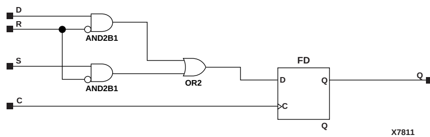
Figure 5-24 FDRS Implementation XC9000
