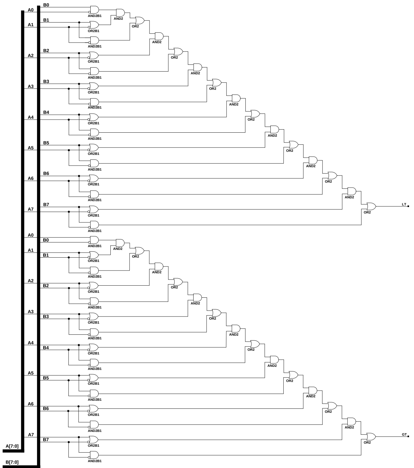
Figure 4-45 COMPM8 Implementation XC9000
