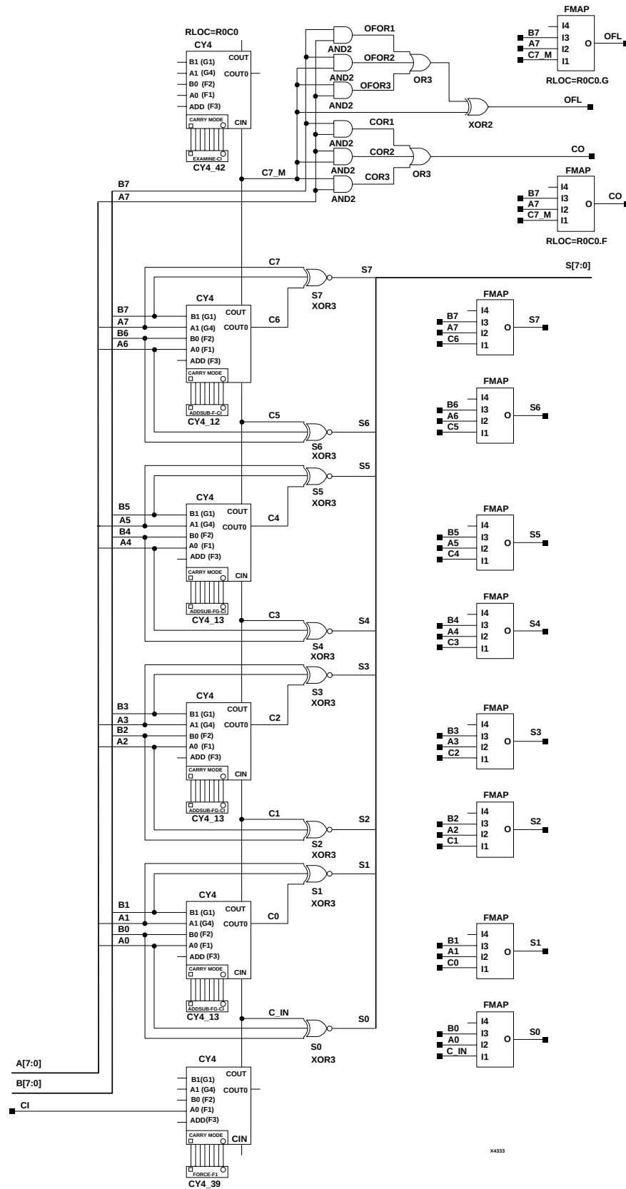
Figure 3-10 ADD8 Implementation XC4000E, XC4000X, Spartan, SpartanXL
