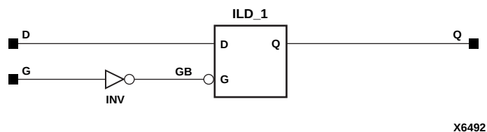
Figure 6-23 ILD Implementation XC4000E, XC4000X, Spartan, SpartanXL
