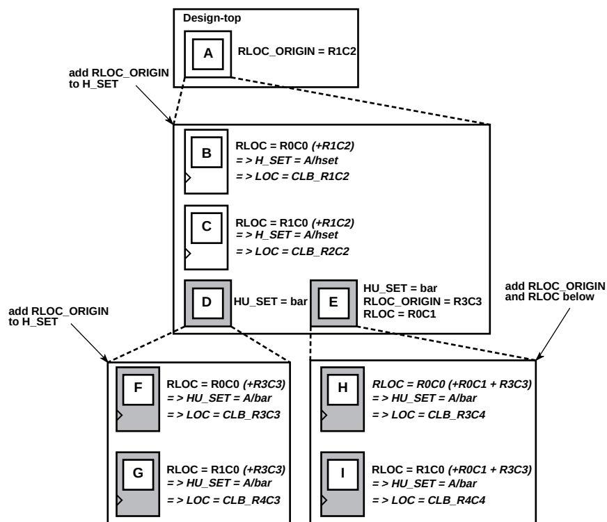
Figure 12-15 Using an RLOC_ORIGIN to Modify H_SET and HU_SET Sets
