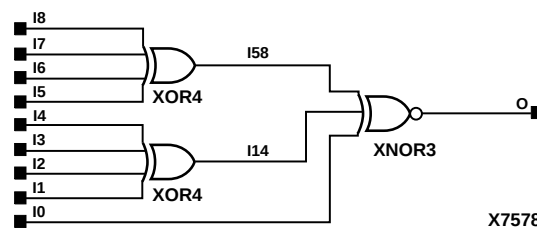
Figure 10-25 XNOR9 Implementation XC4000E, XC4000X, XC5200, Spartan, SpartanXL
