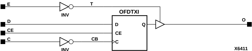
Figure 8-24 OFDEXI_1 Implementation XC4000E, XC4000X, Spartan, SpartanXL
