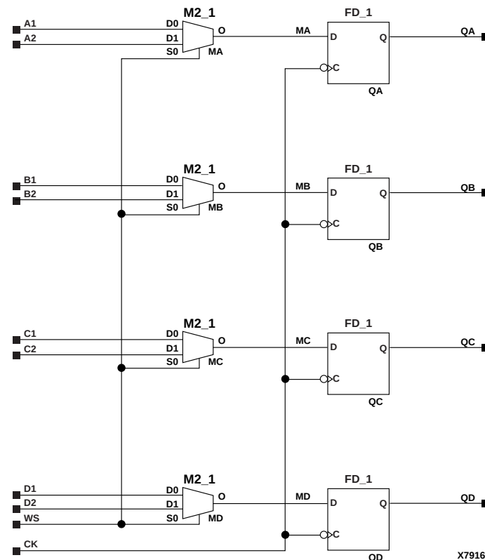
Figure 11-38 X74_298 Implementation XC3000, XC4000E, XC4000X, XC5200, Spartan, SpartanXL
