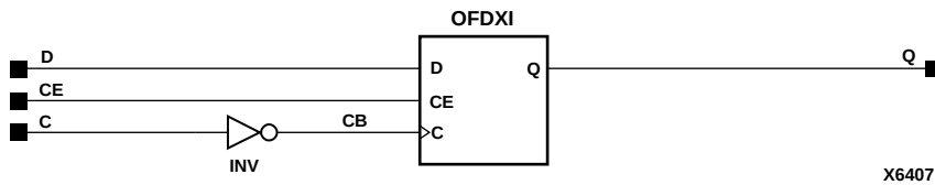
Figure 8-45 OFD XI_1 Implementation XC4000E, XC4000X, Spartan, SpartanXL
