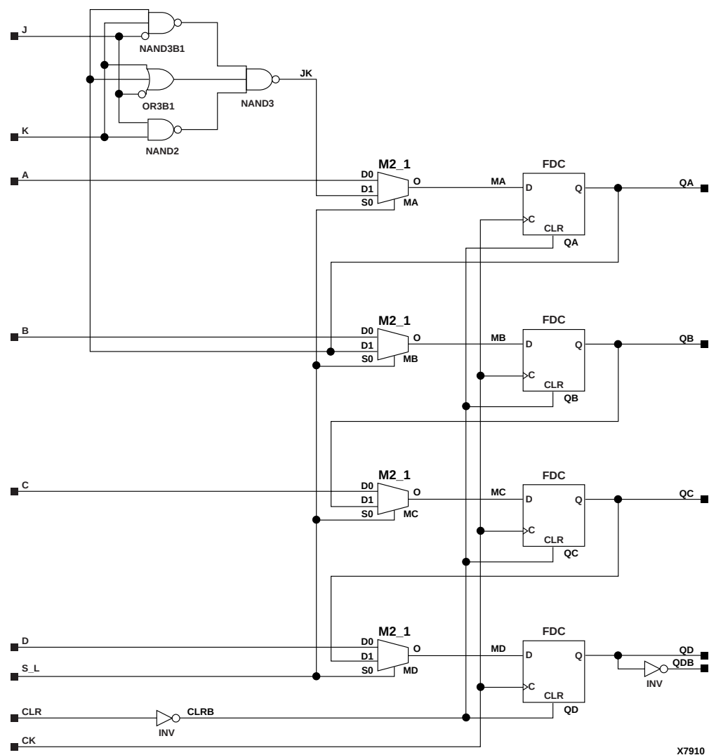
Figure 11-32 X74_195 Implementation XC3000, XC4000E, XC4000X, XC5200, XC9000, Spartan, SpartanXL
