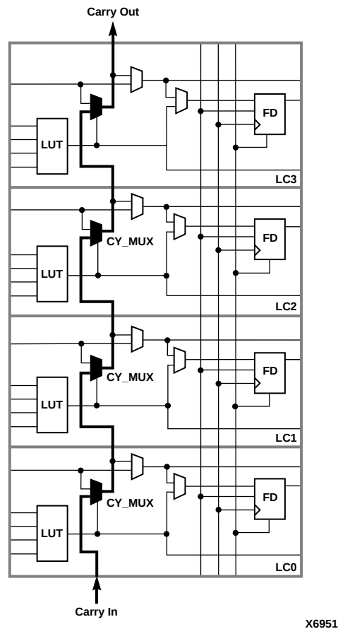
Figure 12-20 XC5200 Carry Logic
