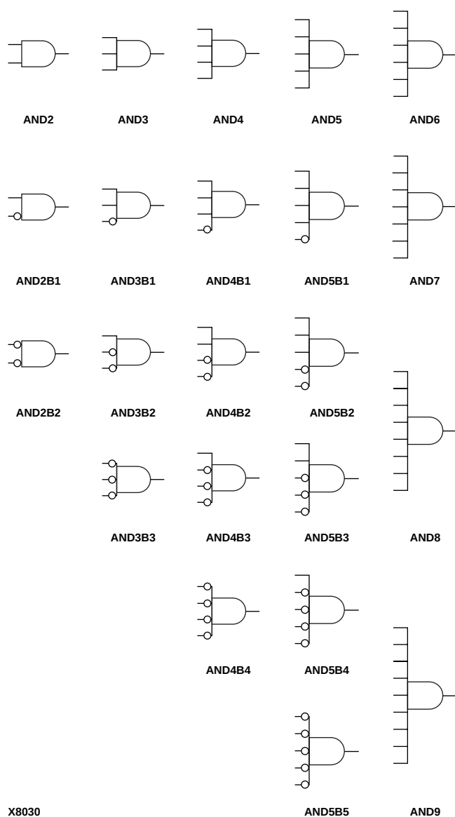
Figure 3-23 AND Gate Representations
