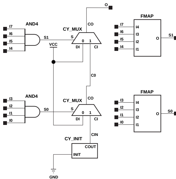
Figure 7-28 NAND8 Implementation XC4000E, XC4000X, Spartan, SpartanXL
