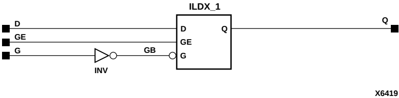
Figure 6-36 ILDX Implementation XC4000E, XC4000X, Spartan, SpartanXL
