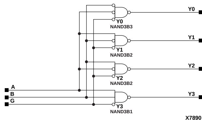
Figure 11-5 X74_139 Implementation XC3000, XC4000E, XC4000X, XC5200, XC9000, Spartan, SpartanXL
