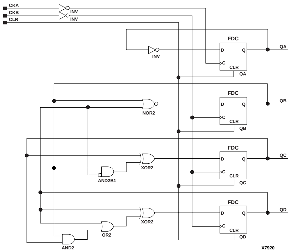
Figure 11-43 X74_390 Implementation XC9000
