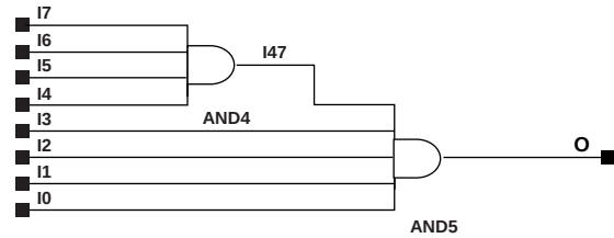
Figure 3-25 AND8 Implementation XC3000
