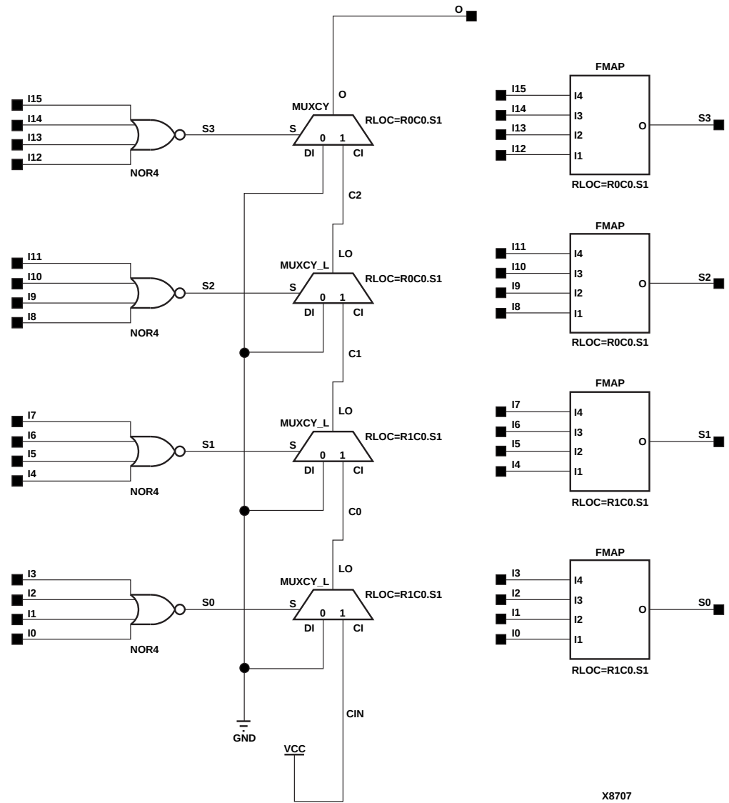
Figure 7-42 NOR16 Implementation Spartan2, Virtex
