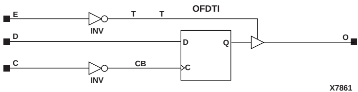
Figure 8-19 OFDEI_1 Implementation XC4000E, XC4000X, Spartan, SpartanXL
