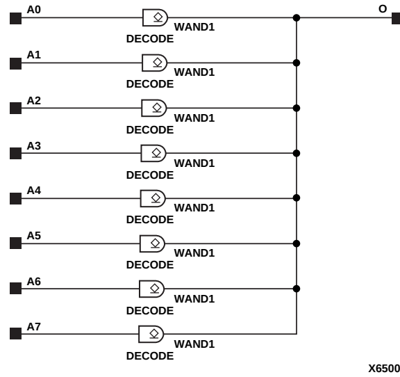
Figure 4-61 DECODE8 Implementation XC4000E, XC4000X
