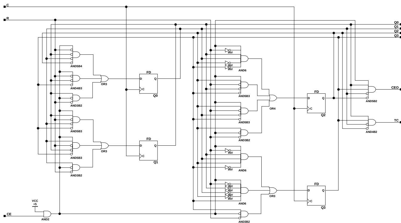
Figure 4-36 CD4RE Implementation XC9000
