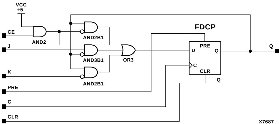
Figure 5-39 FJKCPE Implementation XC9000
