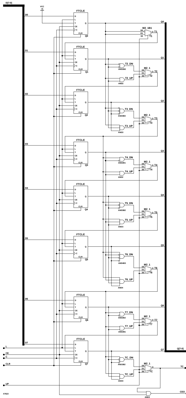
Figure 4-8 CB8CLED Implementation XC3000
