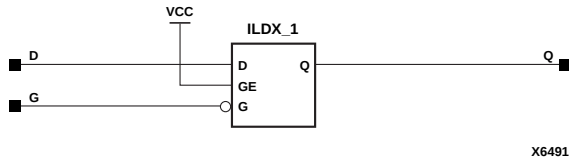
Figure 6-28 ILD_1 Implementation XC4000E, XC4000X, Spartan, SpartanXL
