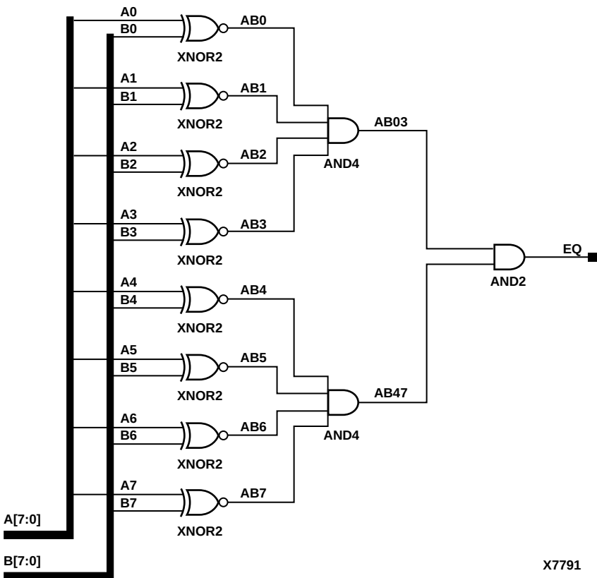
Figure 4-43 COMP8 Implementation XC3000, XC4000E, XC4000X, XC5200, XC9000, Spartan, SpartanXL, Spartan2, Virtex
