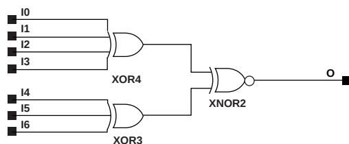
Figure 10-18 XNOR7 Implementation XC9000
