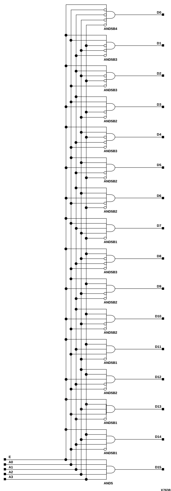
Figure 4-56 D4_16E Implementation XC3000, XC4000E, XC4000X, XC5200, XC9000, Spartan, SpartanXL, Spartan2, Virtex
