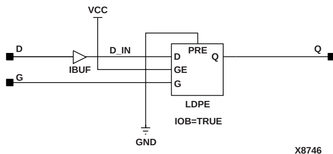
Figure 6-32 ILDI Implementation Spartan2, Virtex
