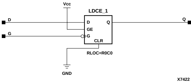
Figure 7-4 LD_1 Implementation XC4000X, SpartanXL
