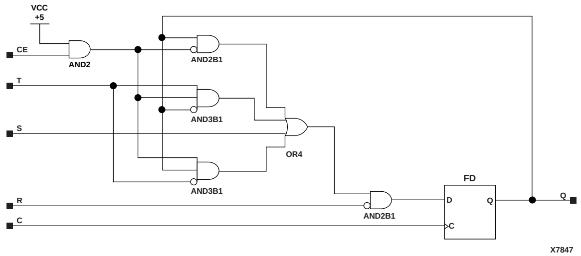
Figure 5-66 FTRSE Implementation XC9000
