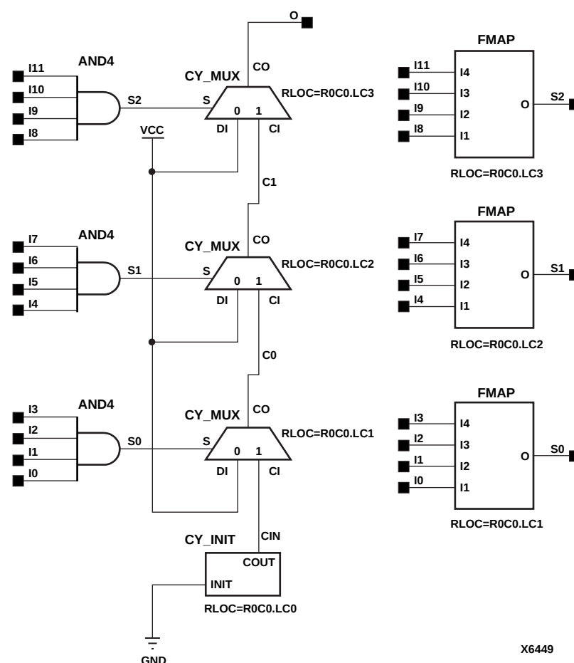
Figure 7-31 NAND12 Implementation XC5200
