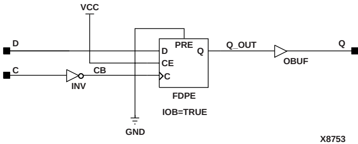
Figure 8-28 OFDI_1 Implementation Spartan2, Virtex
