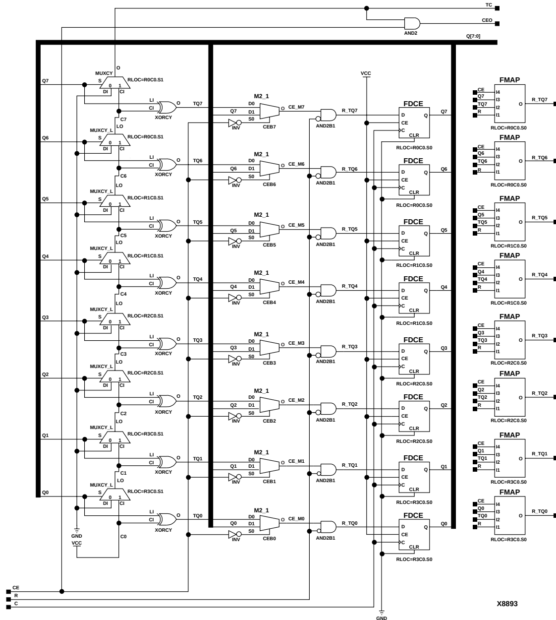
Figure 4-29 CC8RE Implementation Spartan2, Virtex
