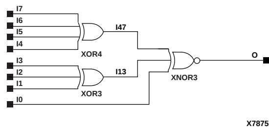
Figure 10-21 XNOR8 Implementation XC4000E, XC4000X, XC5200, Spartan, SpartanXL
