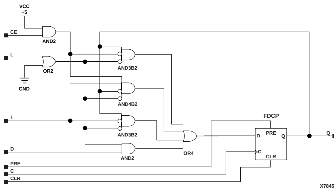
Figure 5-58 FTCPLE Implementation XC9000
