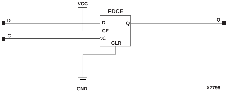
Figure 5-4 FD Implementation XC3000, XC4000E, XC4000X, XC5200, Spartan, SpartanXL
