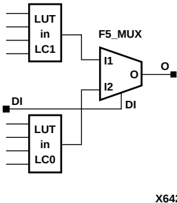
Figure 5-3 F5_MUX Representation
