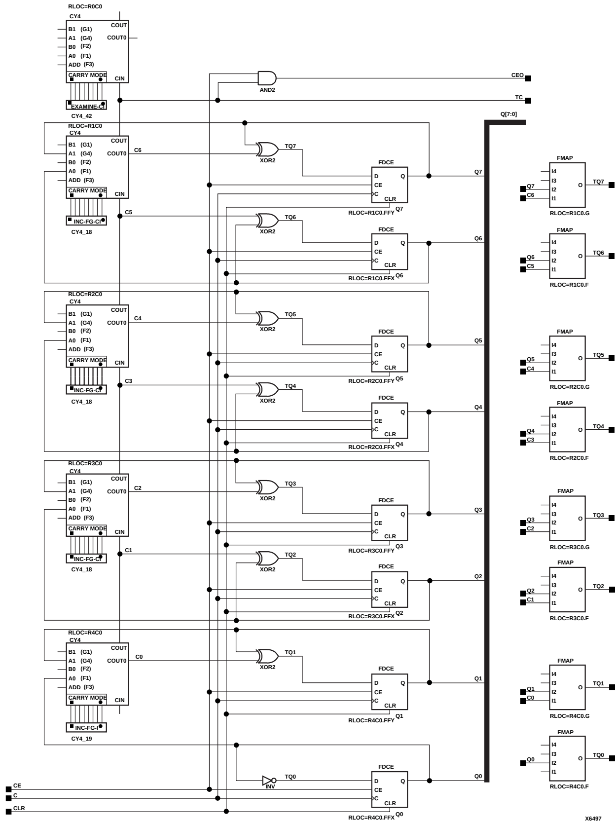
Figure 4-18 CC8CE Implementation XC4000E, XC4000X, Spartan, SpartanXL
