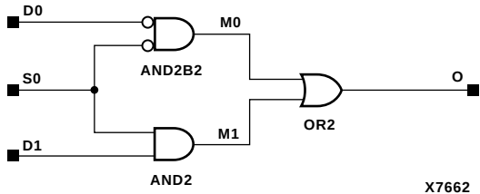
Figure 7-17 M2_1B1 Implementation XC3000, XC4000E, XC4000X, XC5200, XC9000, Spartan, SpartanXL, Spartan2, Virtex
