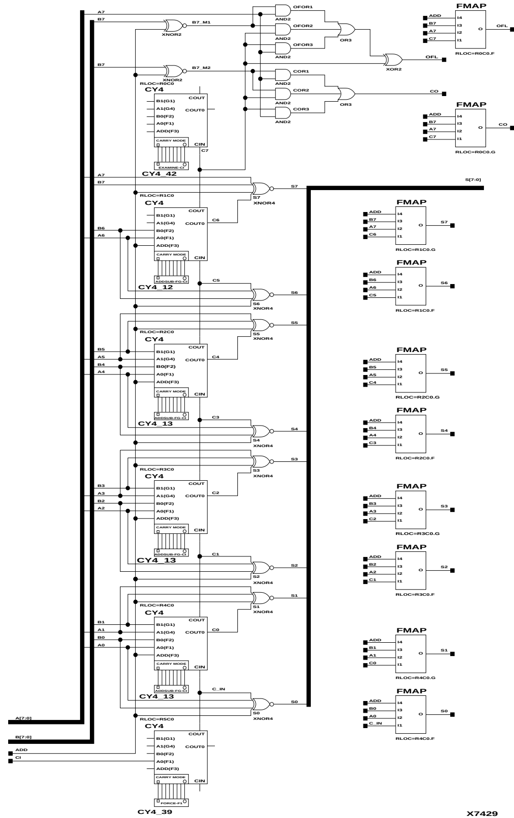
Figure 3-18 ADSU8 Implementation XC4000E, XC4000X, Spartan, SpartanXL
