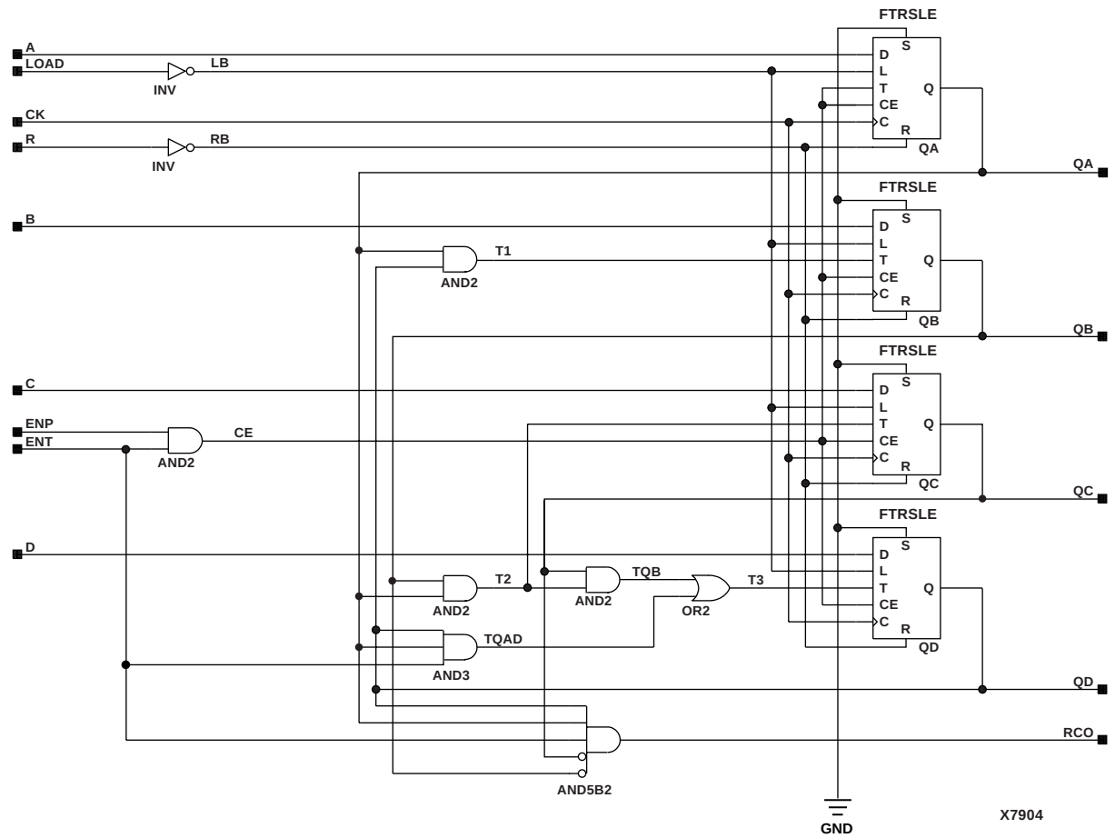
Figure 11-21 X74_162 Implementation XC3000, XC4000E, XC4000X, XC5200, Spartan, SpartanXL
