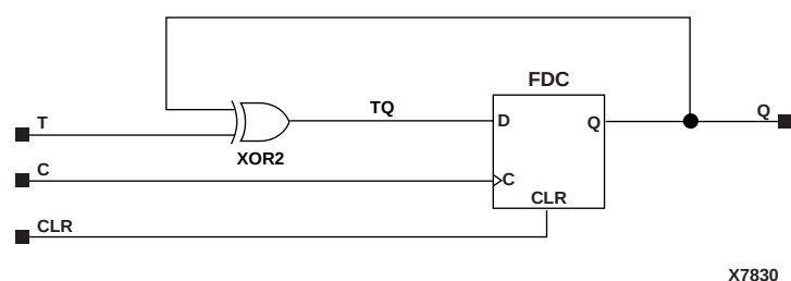
Figure 5-49 FTC Implementation XC3000, XC4000E, XC4000X, XC5200, Spartan, SpartanXL, Spartan2, Virtex
