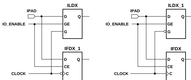
Figure 6-35 Legal Combinations of IFDX and ILDX for a Single IOB in XC4000E, XC4000X, Spartan, or SpartanXL
