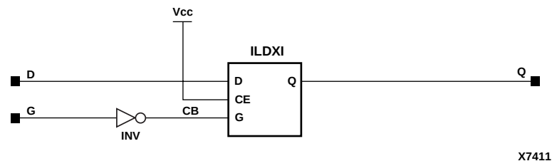
Figure 6-33 ILDI_1 Implementation XC4000E, XC4000X, Spartan, SpartanXL
