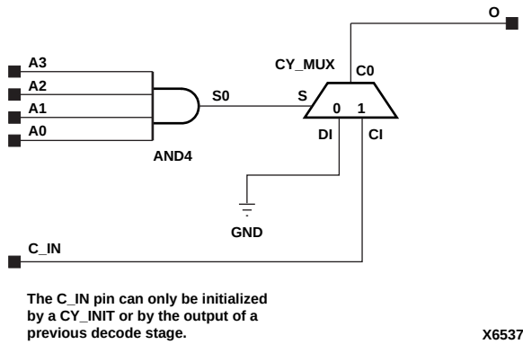
Figure 4-57 DEC_CC4 Implementation XC5200
