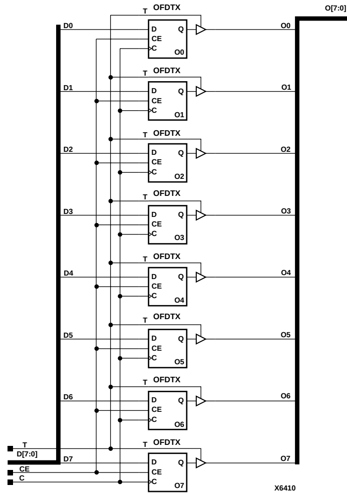
Figure 8-37 OFDTX8 Implementation XC4000E, XC4000X, Spartan, SpartanXL
