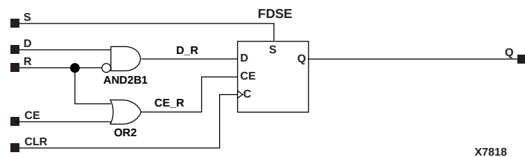
Figure 5-32 FDSRE Implementation XC3000, XC4000E, XC4000X, XC5200, Spartan, SpartanXL
