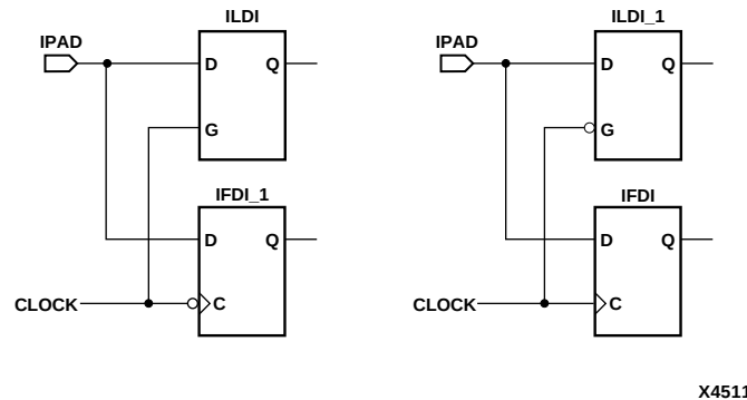
Figure 6-30 Legal Combinations of IFDI and ILDI for a Single IOB in XC4000E, XC4000X, Spartan, or SpartanXL
