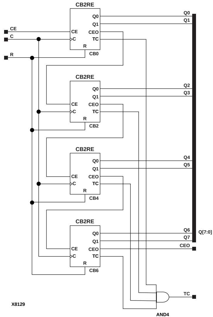
Figure 4-13 CB8RE Implementation XC9000
