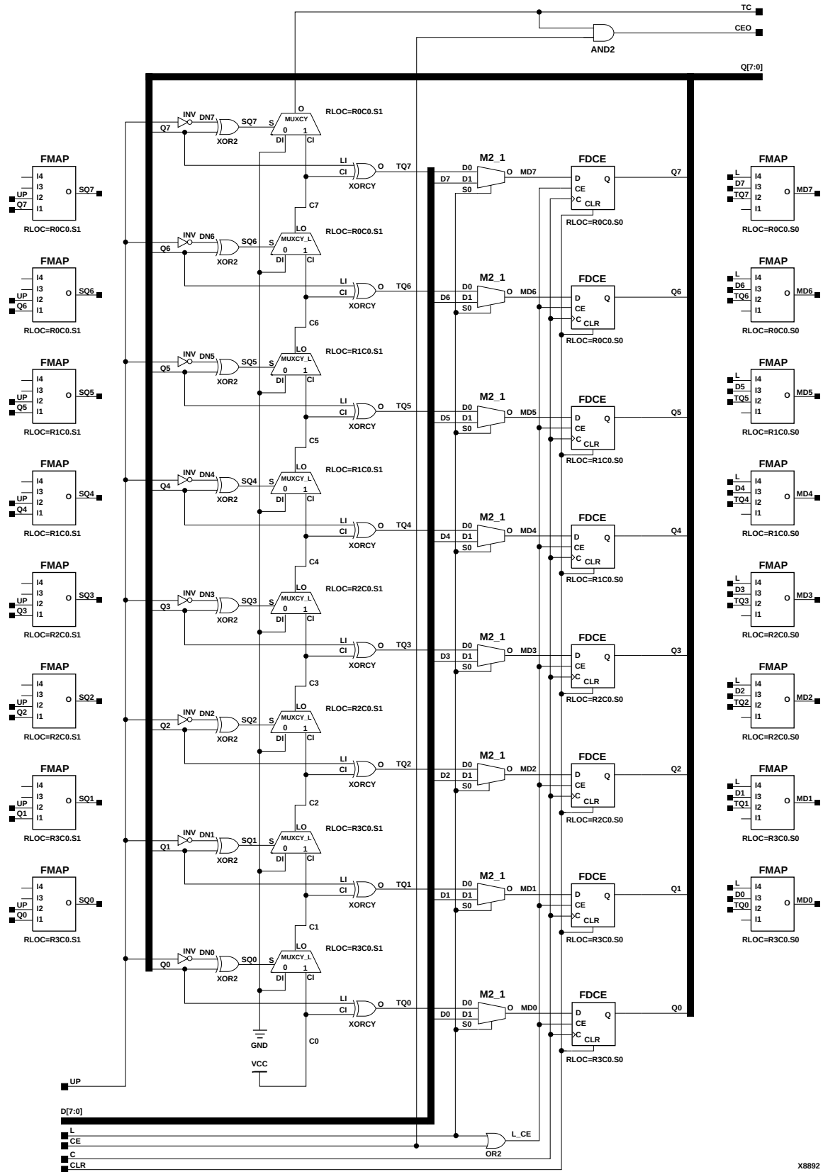
Figure 4-26 CC8CLED Implementation Spartan2, Virtex
