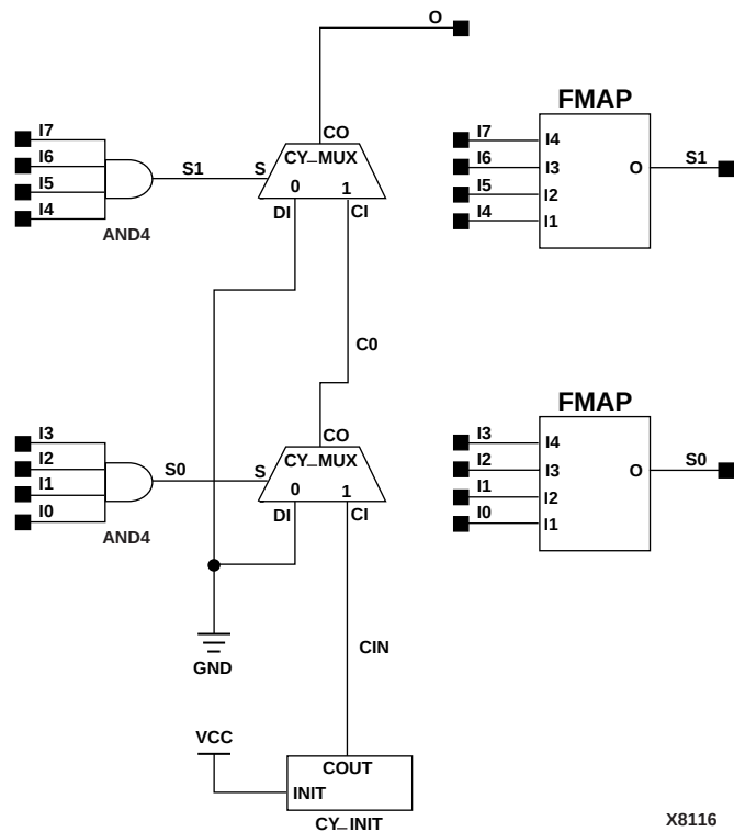
Figure 3-27 AND8 Implementation XC5200
