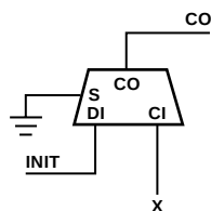
Figure 12-21 Carry Initialize Function XC5200
