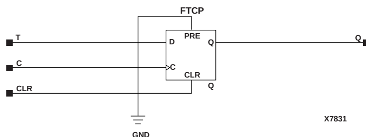
Figure 5-50 FTC Implementation XC9000
