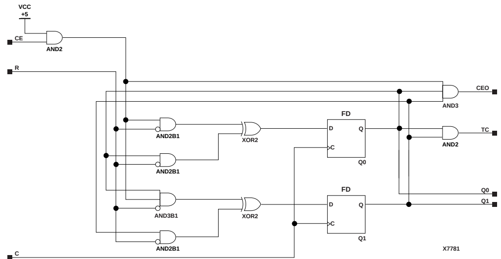
Figure 4-12 CB2RE Implementation XC9000
