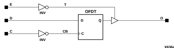
Figure 8-16 OFDE_1 Implementation XC3000, XC4000E, XC4000X, Spartan, SpartanXL
