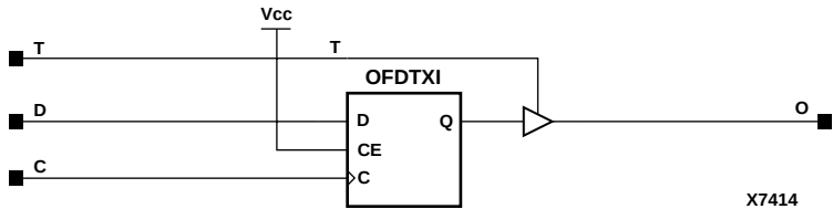
Figure 8-35 OFDTI Implementation XC4000E, XC4000X, Spartan, SpartanXL
