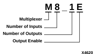
Figure 2-7 Multiplexer Naming Convention
