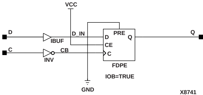
Figure 6-13 IFDI_1 Implementation Spartan2, Virtex
