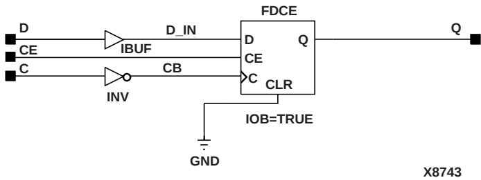
Figure 6-17 IFDX_1 Implementation Spartan2, Virtex
