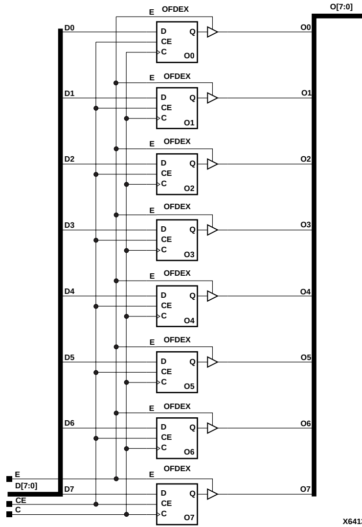
Figure 8-21 OFDEX8 Implementation XC4000E, XC4000X, Spartan, SpartanXL
