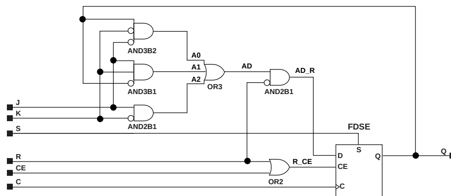
Figure 5-46 FJKSRE Implementation XC3000, XC4000E, XC4000X, XC5200, Spartan, SpartanXL, Spartan2, Virtex
