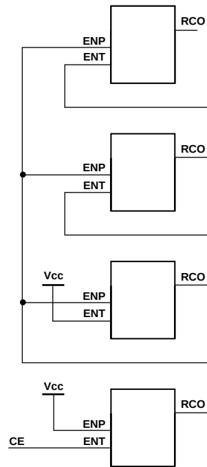
Figure 11-27 Carry-Lookahead Design
