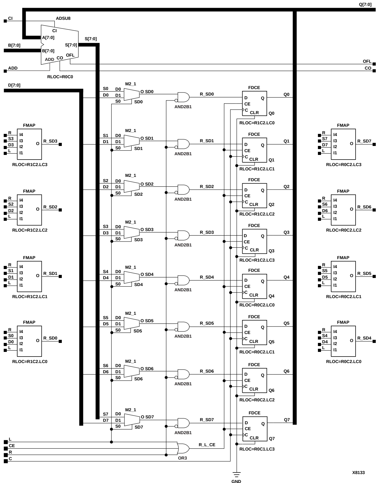
Figure 3-4 ACC8 Implementation XC5200
