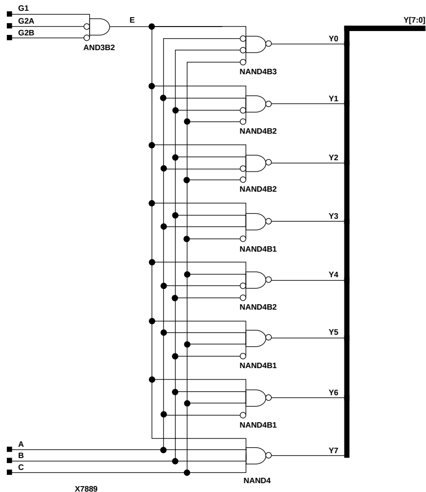
Figure 11-4 X74_138 Implementation XC3000, XC4000E, XC4000X, XC5200, XC9000, Spartan, SpartanXL
