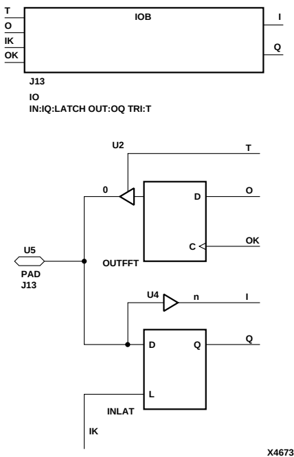
Figure 6-47 XC3000 IOB Primitive Example and Equivalent Circuit
