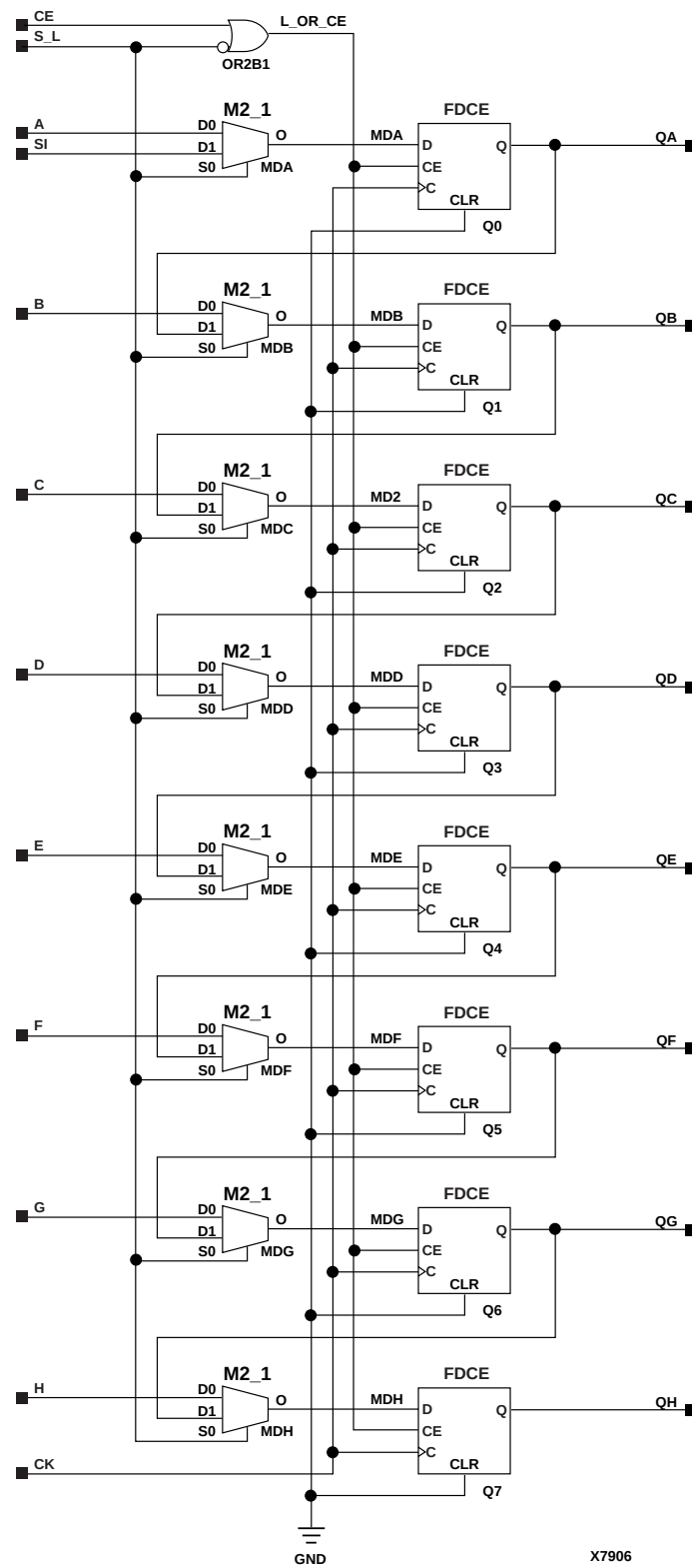
Figure 11-26 X74_165S Implementation XC3000, XC4000E, XC4000X, XC5200, XC9000, Spartan, SpartanXL
