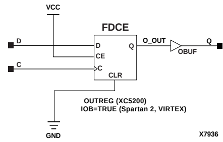
Figure 8-6 OFD Implementation XC5200, Spartan2, Virtex
