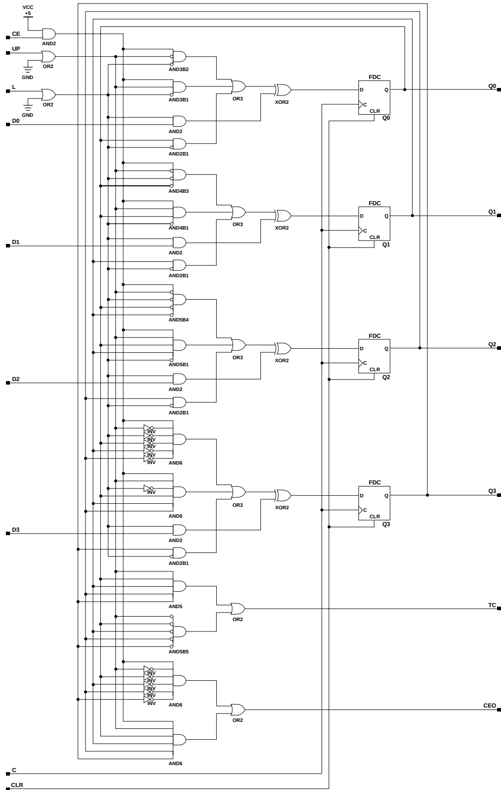
Figure 4-10 CB4CLED Implementation XC9000
