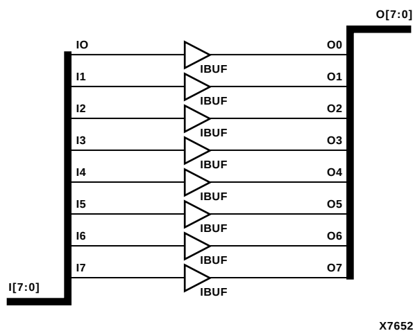
Figure 6-3 IBUF8 Implementation XC3000, XC4000E, XC4000X, XC5200, XC9000, Spartan, SpartanXL, Spartan2, Virtex
