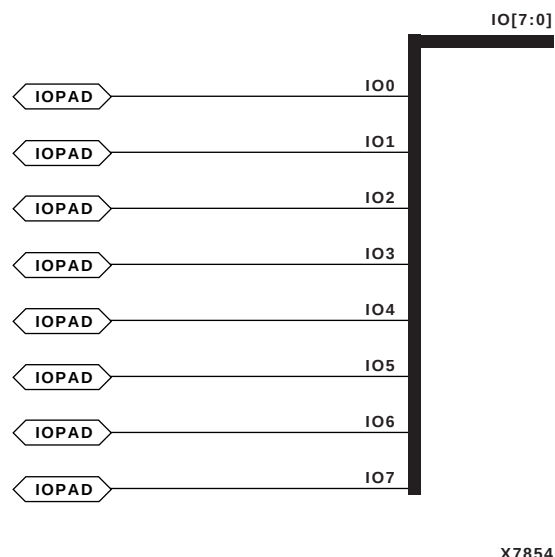
Figure 6-48 IOPAD8 Implementation XC3000, XC4000E, XC4000X, XC5200, XC9000, Spartan, SpartanXL, Spartan2, Virtex
