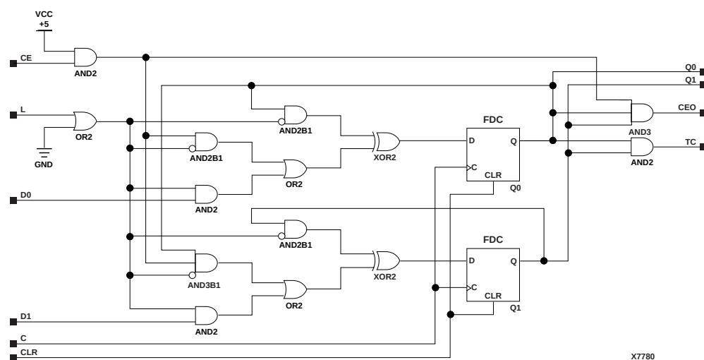
Figure 4-6 CB2CLE Implementation XC9000
