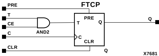
Figure 5-57 FTCPE Implementation XC9000
