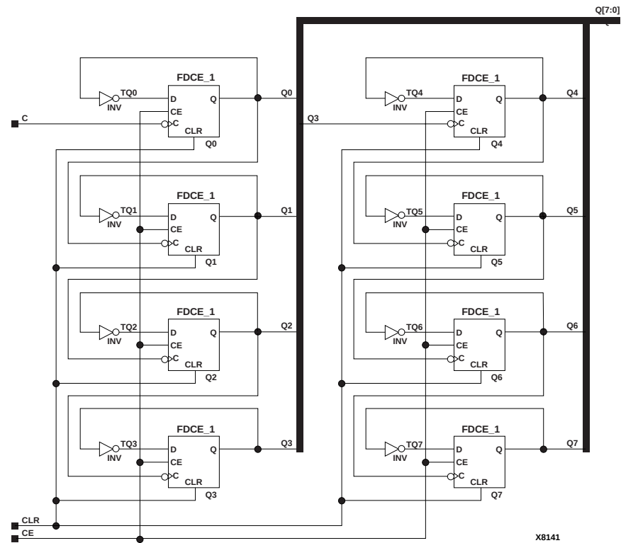
Figure 4-49 CR8CE Implementation XC3000
