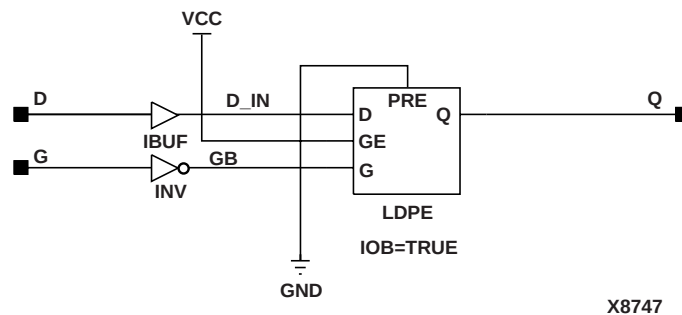
Figure 6-34 ILDI_1 Implementation Spartan2, Virtex
