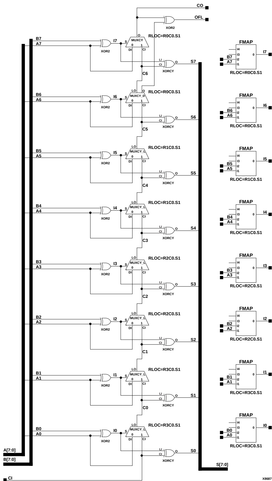
Figure 3-12 ADD8 Implementation Spartan2, Virtex
