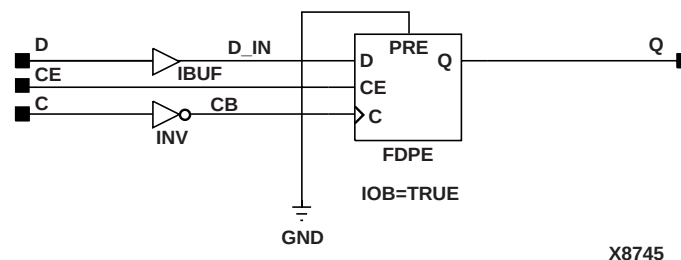
Figure 6-20 IFDXI_1 Implementation Spartan2, Virtex
