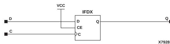
Figure 6-4 IFD Implementation XC4000E, XC4000X, Spartan, SpartanXL
