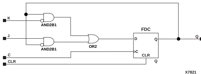
Figure 5-35 FJKC Implementation XC9000
