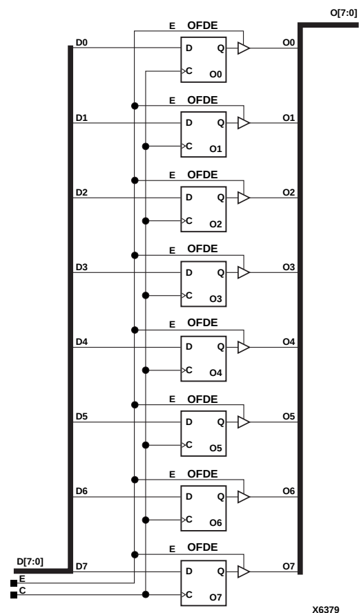
Figure 8-15 OFDE8 Implementation XC3000, XC4000E, XC4000X, XC5200, XC9000, Spartan, SpartanXL, Spartan2, Virtex
