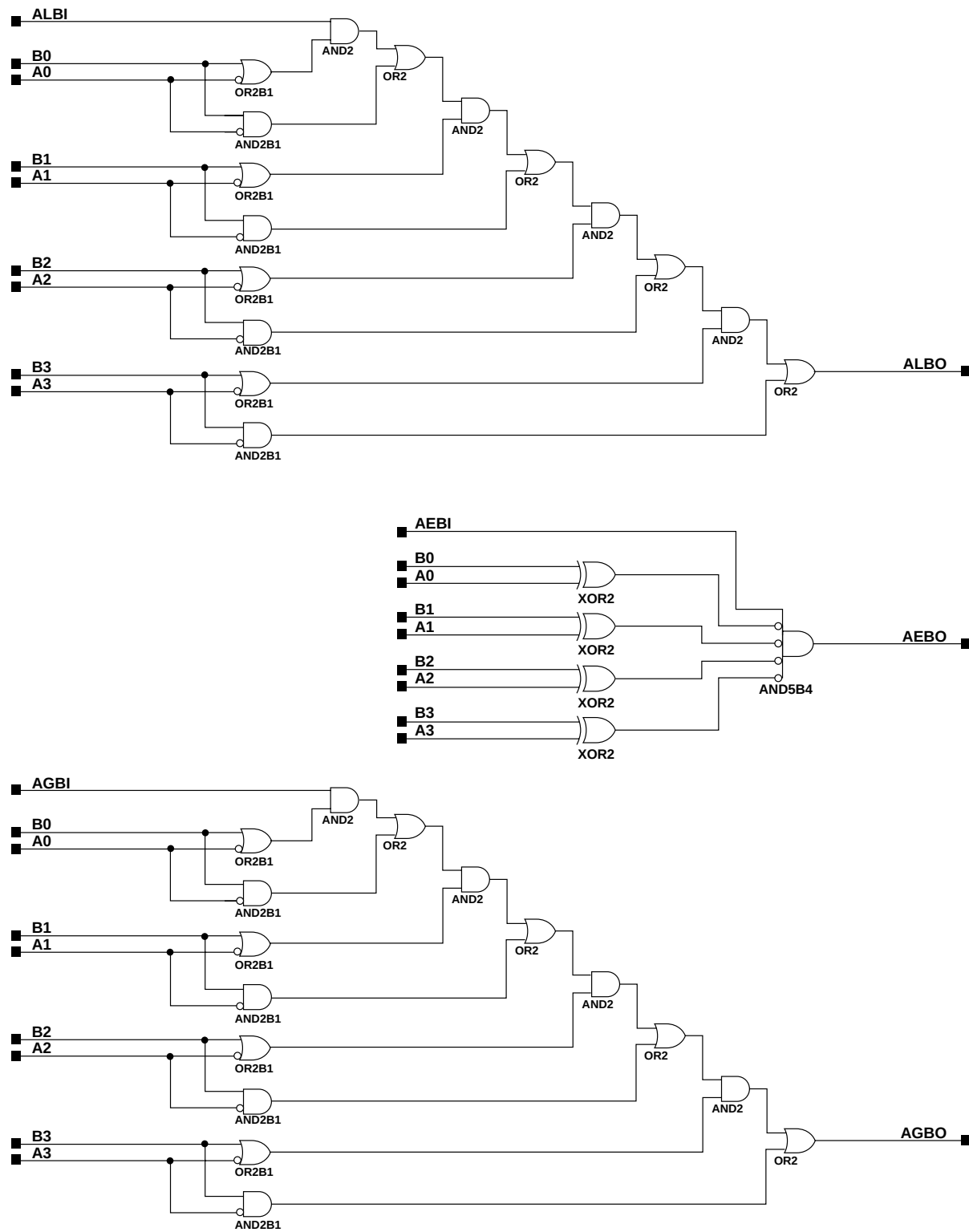
Figure 11-3 X74_L85 Implementation XC9000
