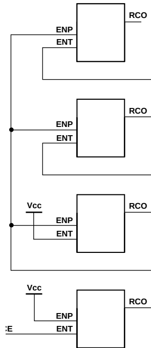
Figure 2-3 Carry-Lookahead Design
