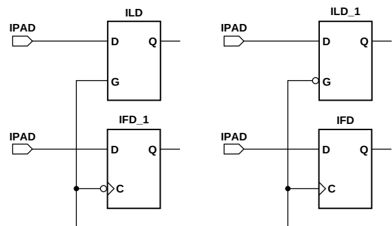
Figure 6-21 Legal Combinations of IFD and ILD for a Single Device Edge of an XC3000 IOB
