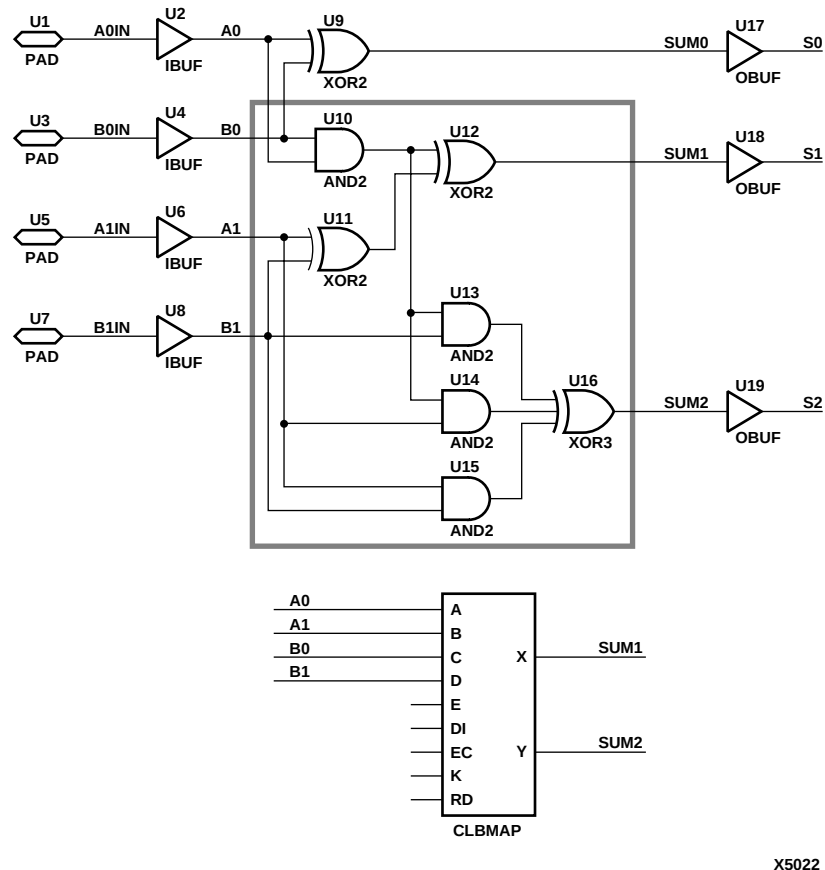
Figure 4-42 XC3000 CLBMAP Primitive Example and Equivalent
