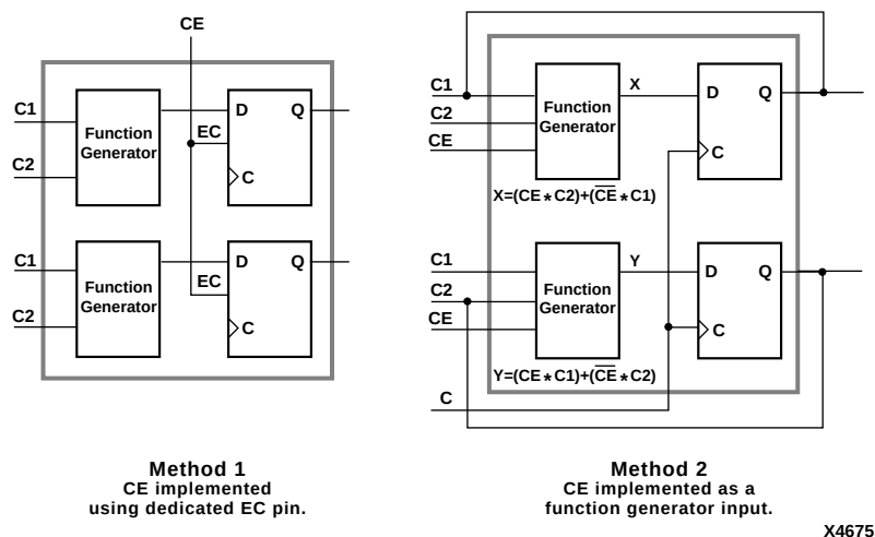
Figure 1-3 Clock Enable Implementation Methods
