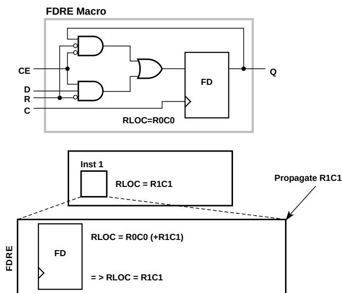
Figure 12-11 Typical Use of a Xilinx Macro
