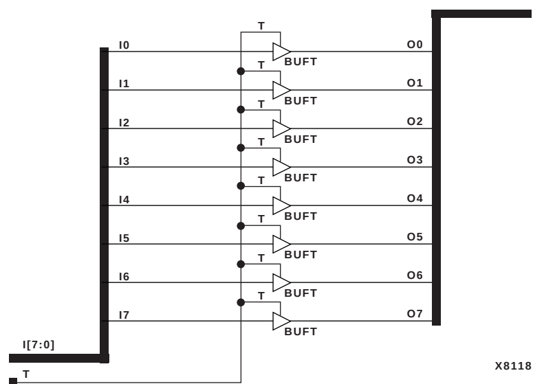
Figure 3-41 BUFT8 Implementation XC3000, XC4000E, XC4000X, XC5200, XC9000, Spartan, SpartanXL, Spartan2, Virtex
