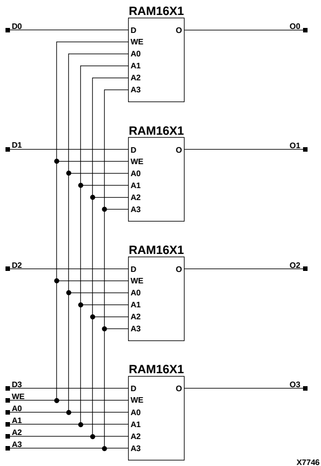
Figure 9-2 RAM16X4 Implementation XC4000E, XC4000X
