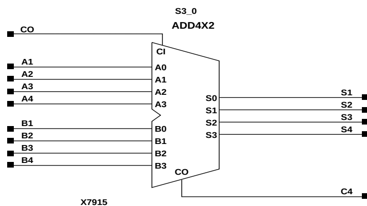
Figure 11-37 X74_283 Implementation XC9000
