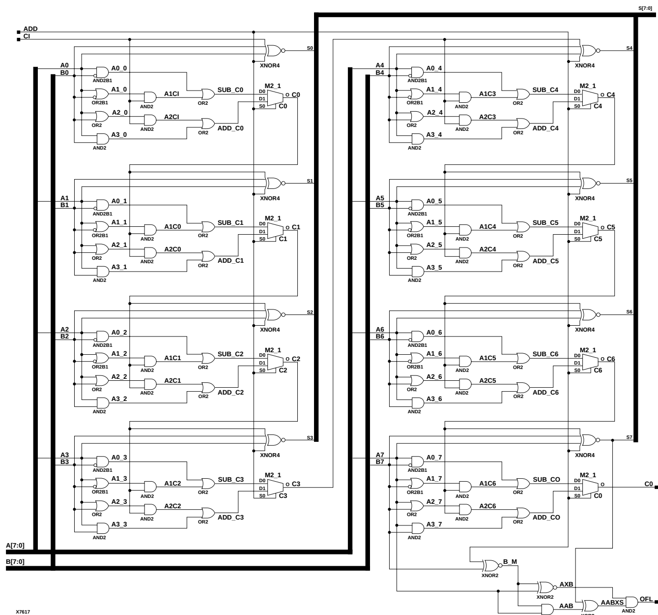
Figure 3-17 ADSU8 Implementation XC3000
