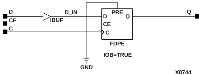
Figure 6-18 IFDXI Implementation Spartan2, Virtex
