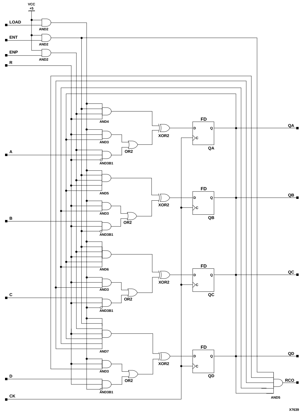
Figure 11-24 X74_163 Implementation XC9000
