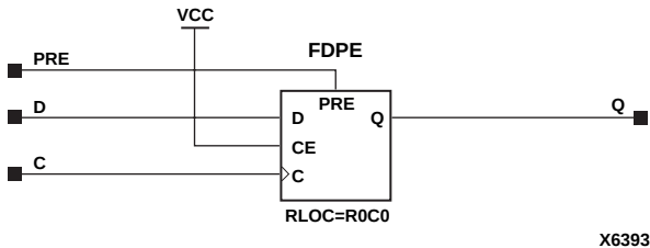
Figure 5-15 FDP Implementation XC4000E, XC4000X, XC5200, Spartan, SpartanXL
