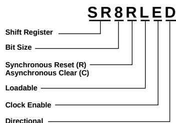
Figure 2-8 Shift Register Naming Convention
