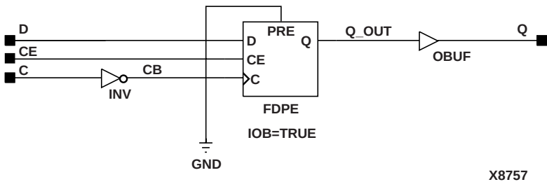
Figure 8-46 OFD XI_1 Implementation Spartan2, Virtex
