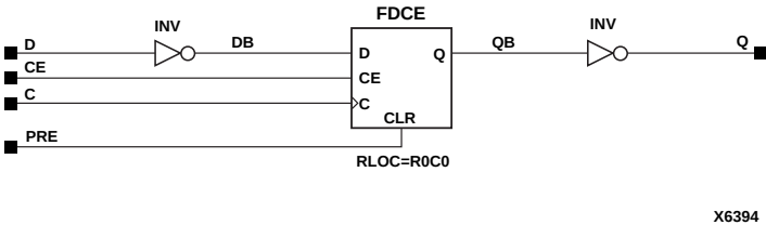
Figure 5-18 FDPE Implementation XC5200
