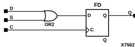
Figure 5-27 FDS Implementation XC3000, XC4000E, XC4000X, XC5200, XC9000, Spartan, SpartanXL
