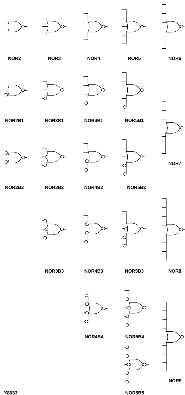
Figure 7-35 NOR Gate Representations
