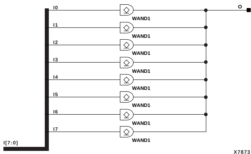
Figure 10-11 WAND8 Implementation XC4000E, XC4000X
