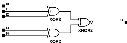
Figure 10-14 XNOR5 Implementation XC9000
