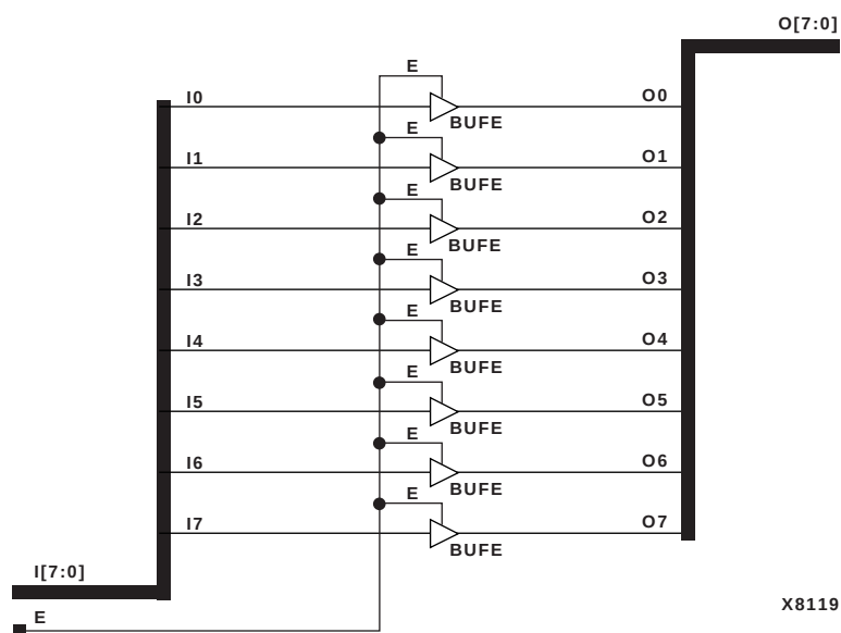
Figure 3-37 BUFE8 Implementation XC9000, Spartan2, Virtex
