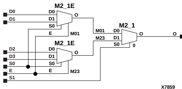
Figure 7-20 M4_1E Implementation XC3000, XC4000E, XC4000X, XC5200, XC9000, Spartan, SpartanXL
