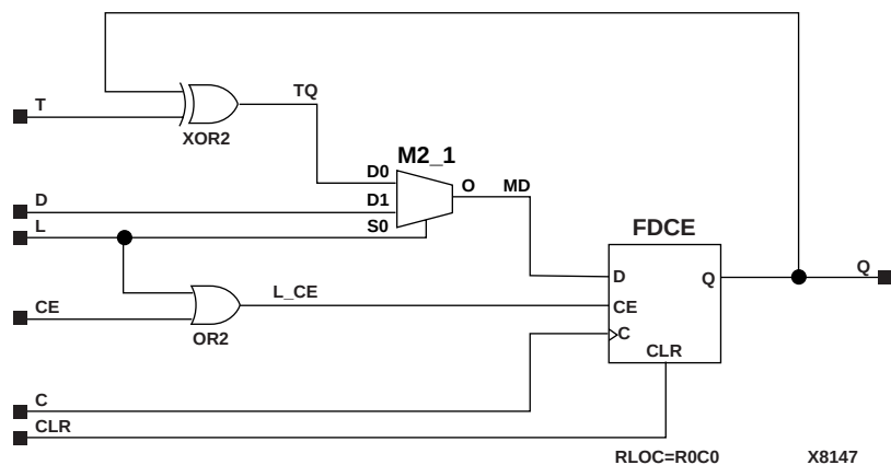
Figure 5-54 FTCLE Implementation XC4000E, XC4000X, XC5200, Spartan, SpartanXL, Spartan2, Virtex
