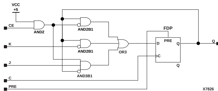
Figure 5-43 FJKPE Implementation XC9000
