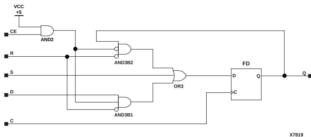
Figure 5-33 FDSRE Implementation XC9000
