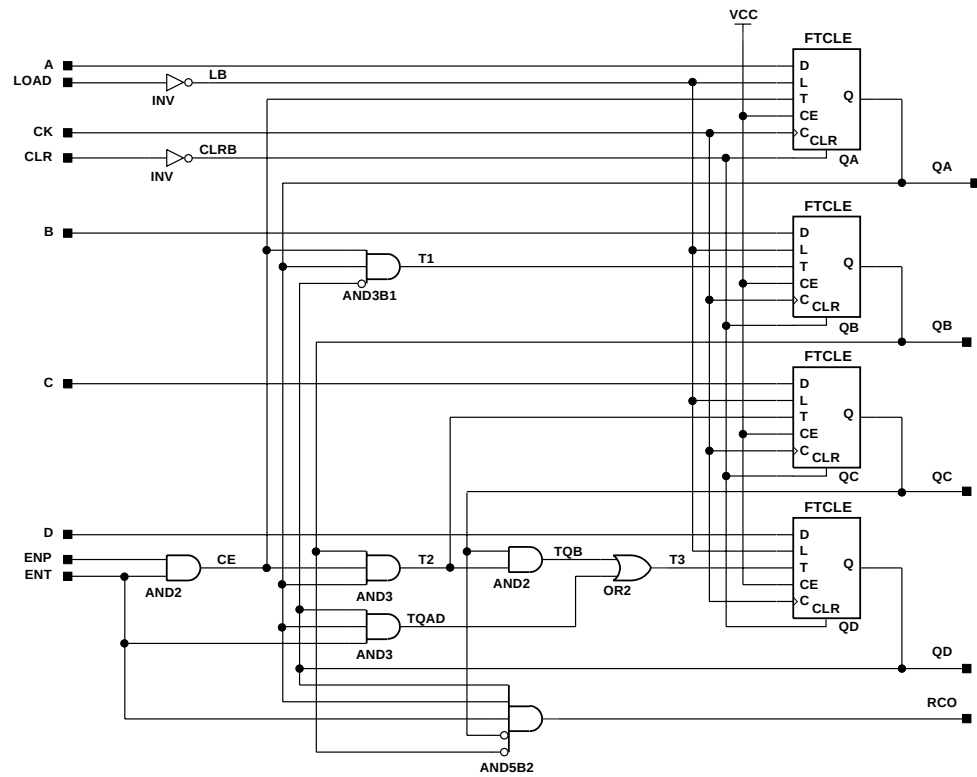
Figure 11-17 X74_160 Implementation XC4000E, XC4000X, XC5200, Spartan, SpartanXL
