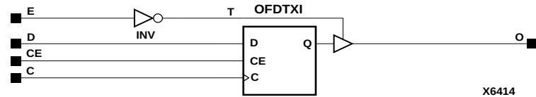
Figure 8-23 OFDEXI Implementation XC4000E, XC4000X, Spartan, SpartanXL
