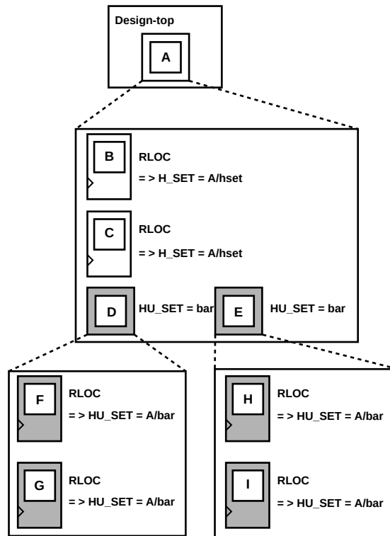
Figure 12-10 Linking Two HU_SET Sets
