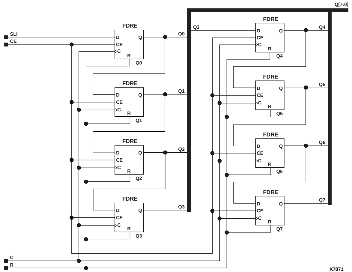
Figure 10-8 SR8RE Implementation XC3000, XC4000E, XC4000X, XC5200, XC9000, Spartan, SpartanXL, Spartan2, Virtex
