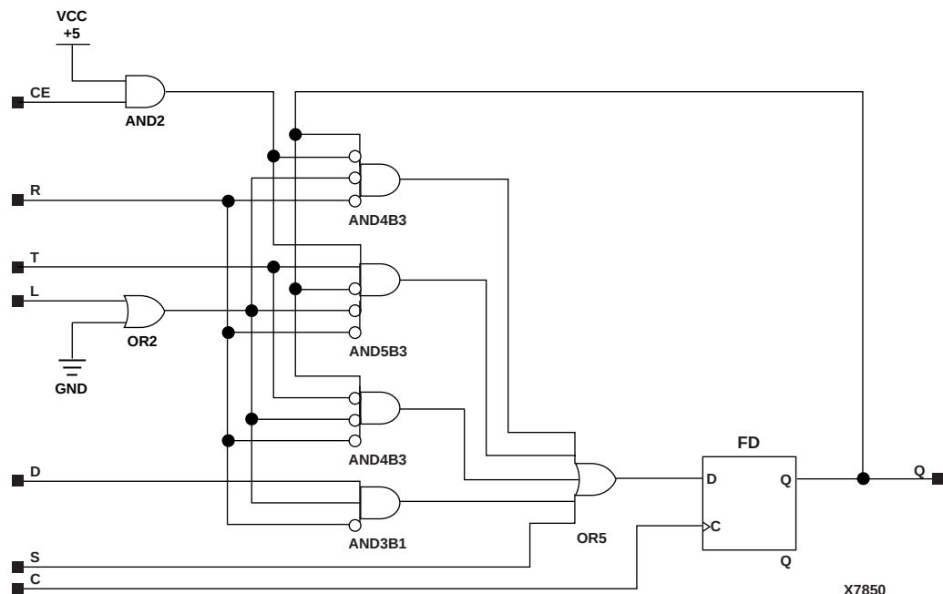
Figure 5-72 FTSRLE Implementation XC9000
