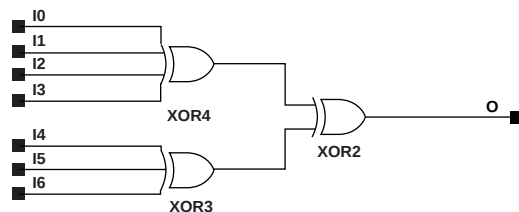
Figure 10-32 XOR7 Implementation XC9000
