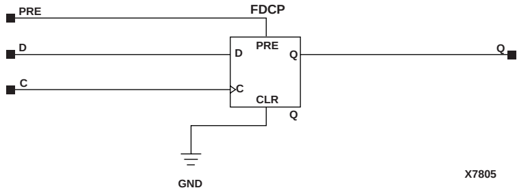
Figure 5-16 FDP Implementation XC9000
