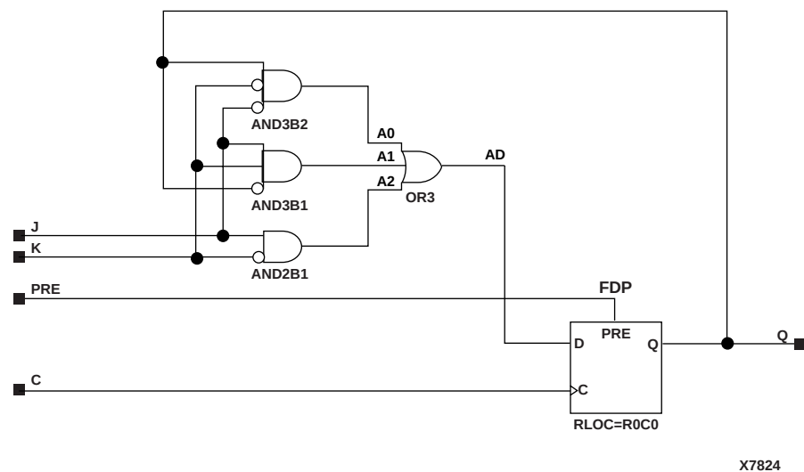
Figure 5-40 FJKP Implementation XC4000E, XC4000X, XC5200, Spartan, SpartanXL, Spartan2, Virtex
