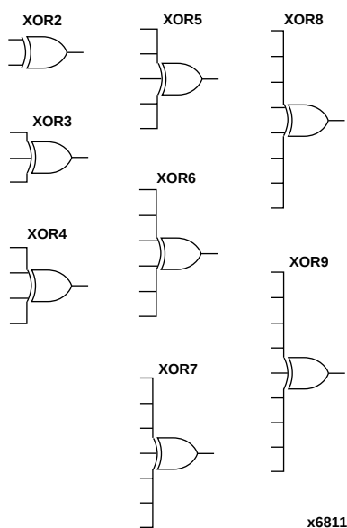
Figure 10-28 XOR Gate Representations
