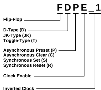
Figure 2-5 Flip-Flop Naming Convention
