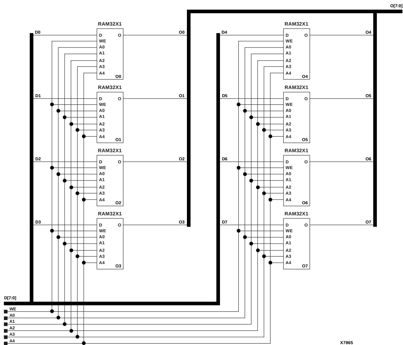
Figure 9-6 RAM32X8 Implementation XC4000E, XC4000X
