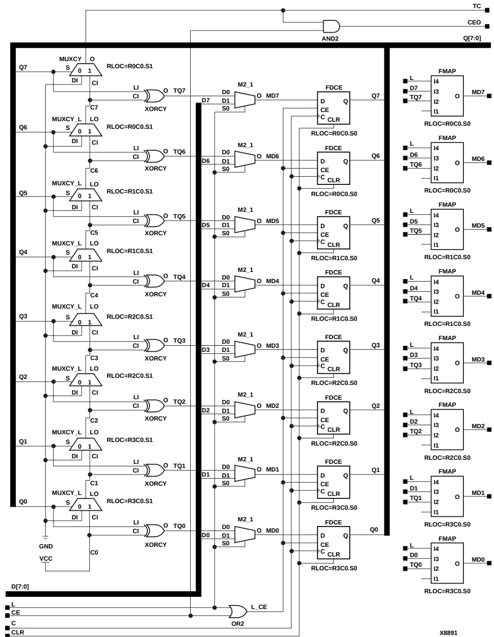
Figure 4-23 CC8CLE Implementation Spartan2, Virtex
