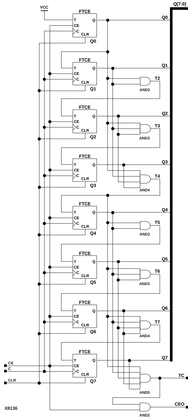
Figure 4-1 CB8CE Implementation XC3000, XC4000E, XC4000X, XC5200, Spartan, SpartanXL, Spartan2, Virtex
