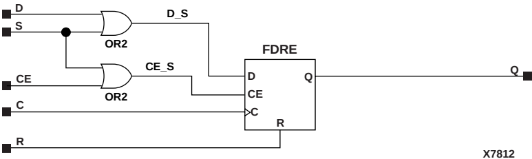
Figure 5-25 FDRSE Implementation XC3000, XC4000E, XC4000X, XC5200, Spartan, SpartanXL
