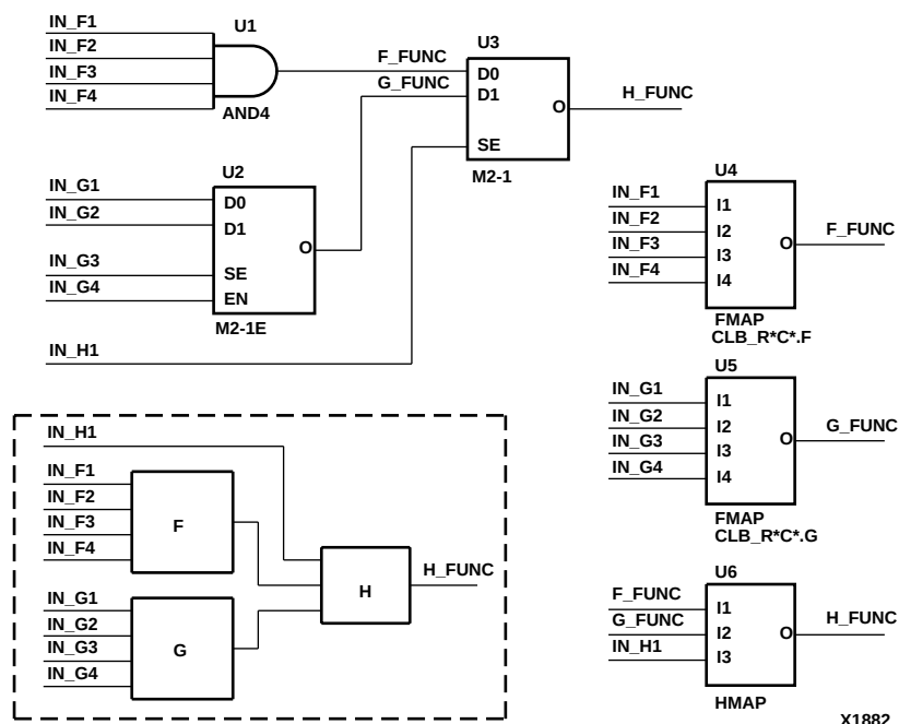
Figure 6-2 Partitioning Logic Using FMAP and HMAP Symbols
