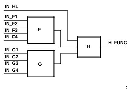
Figure 12-3 Implementation of FMAP and HMAP
