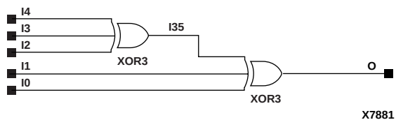
Figure 10-29 XOR5 Implementation XC5200
