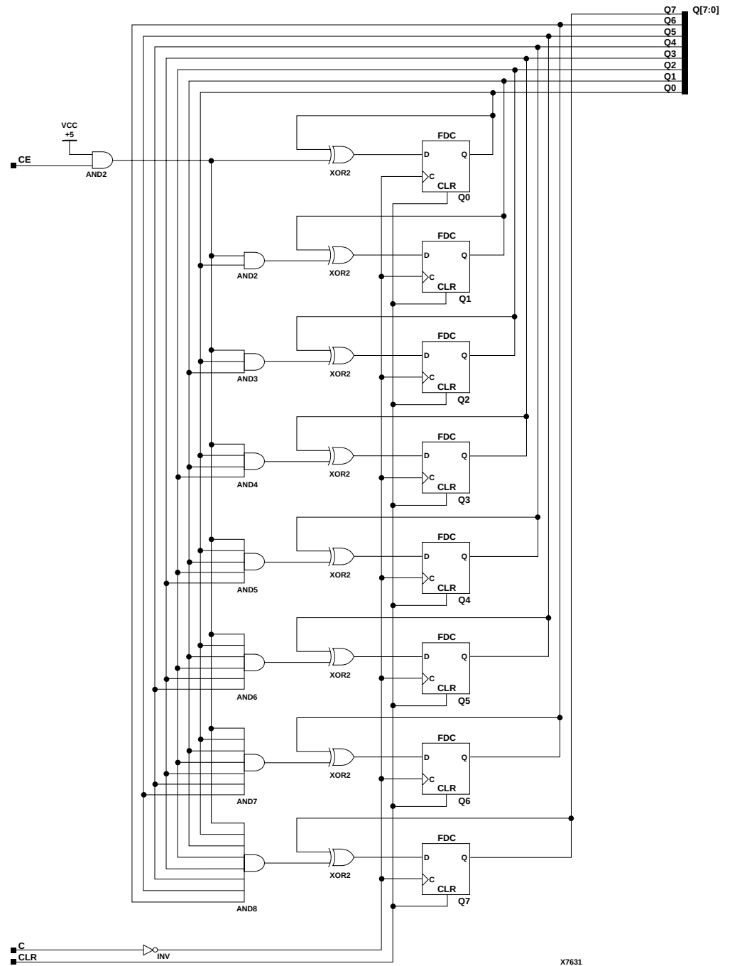
Figure 4-51 CR8CE Implementation XC9000
