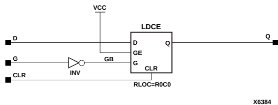
Figure 7-10 LDC_1 Implementation XC5200
