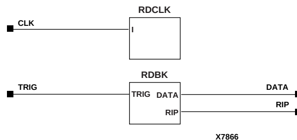
Figure 9-9 READBACK Implementation XC4000E, XC4000X, XC5200, Spartan, SpartanXL
