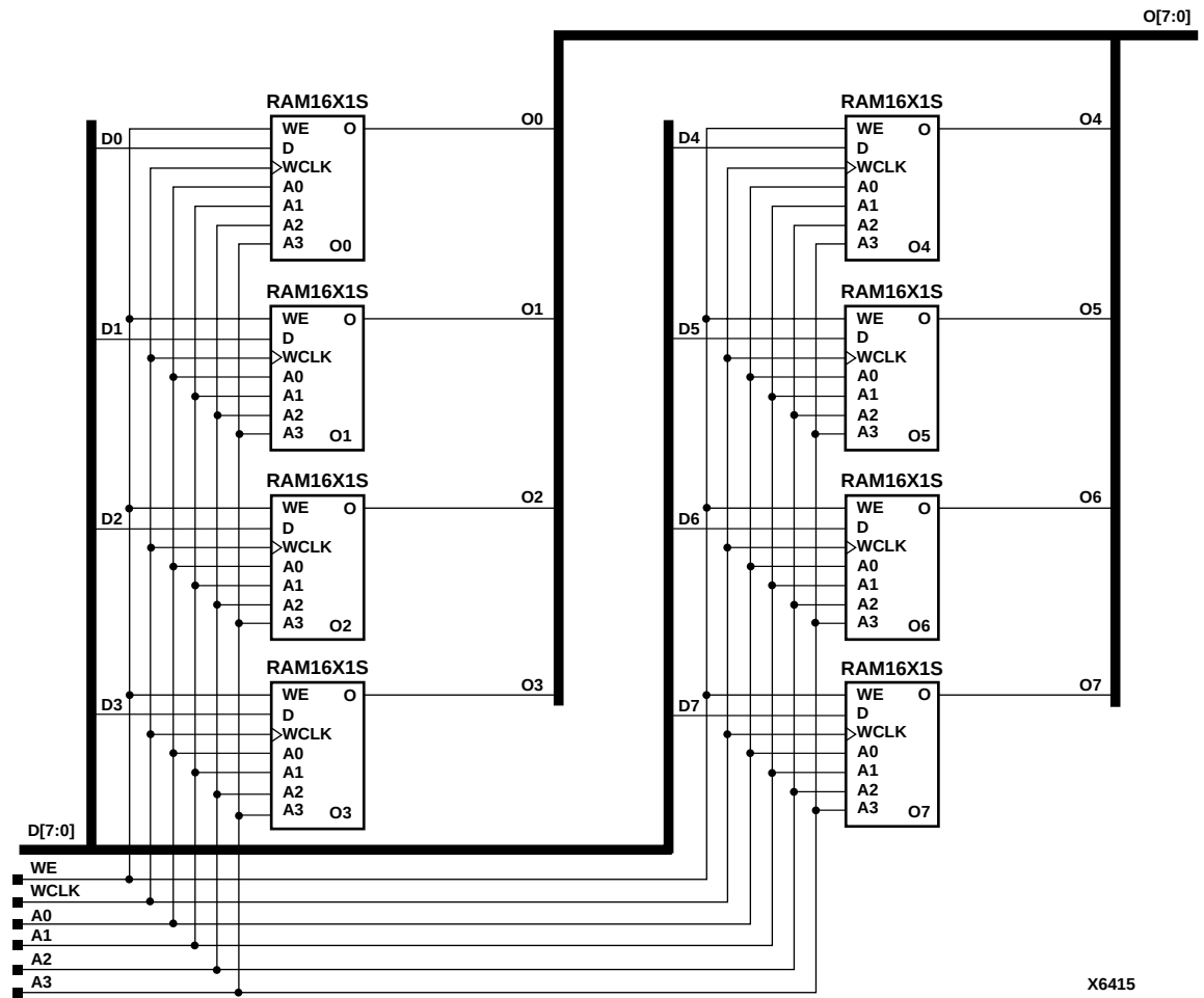
Figure 9-5 RAM16X8S Implementation XC4000E, XC4000X, Spartan, SpartanXL
