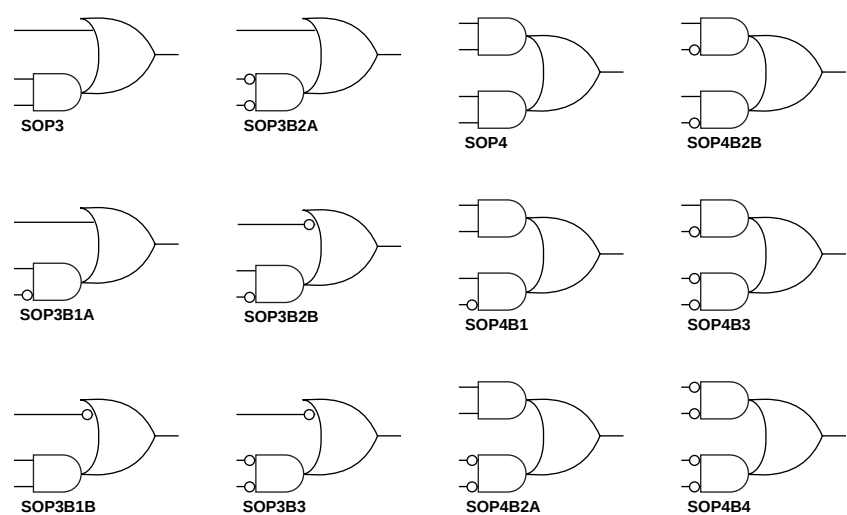
Figure 10-1 SOP Gate Representations
