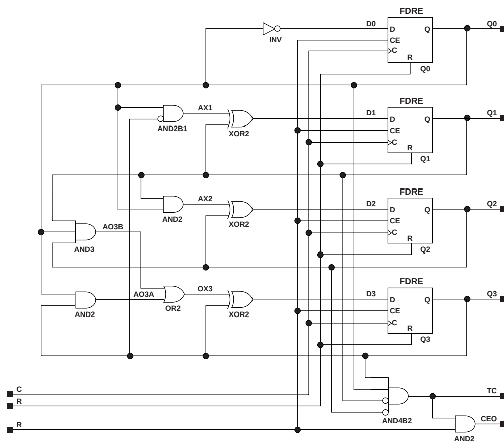
Figure 4-35 CD4RE Implementation XC3000, XC4000E, XC4000X, XC5200, Spartan, SpartanXL, Spartan2, Virtex
