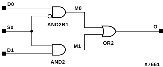
Figure 7-16 M2_1 Implementation XC3000, XC4000E, XC4000X, XC5200, XC9000, Spartan, SpartanXL, Spartan2, Virtex
