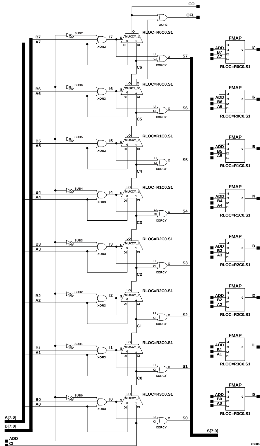
Figure 3-20 ADSU8 Implementation Spartan2, Virtex
