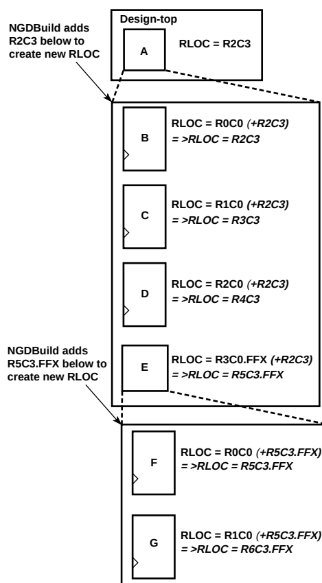
Figure 12-7 Adding RLOC Values Down the Hierarchy
