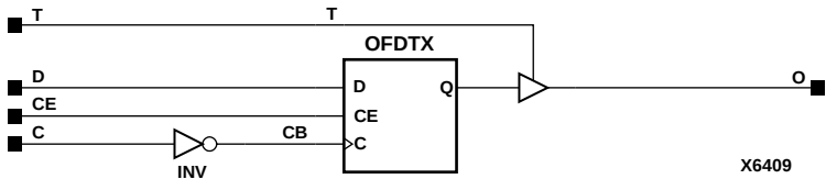
Figure 8-38 OFDTX_1 Implementation XC4000E, XC4000X, Spartan, SpartanXL
