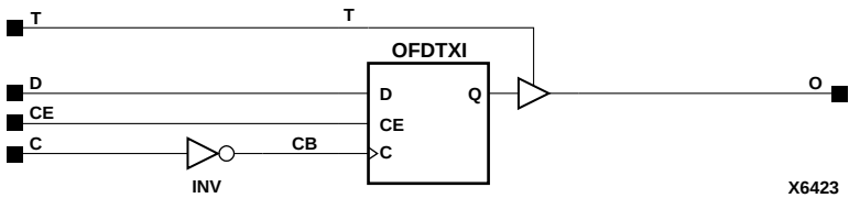
Figure 8-39 OFDTXI_1 Implementation XC4000E, XC4000X, Spartan, SpartanXL
