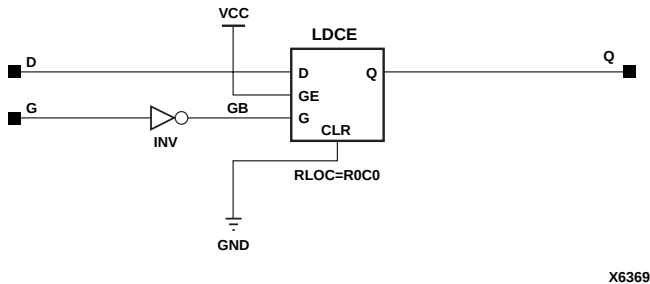
Figure 7-5 LD_1 Implementation XC5200
