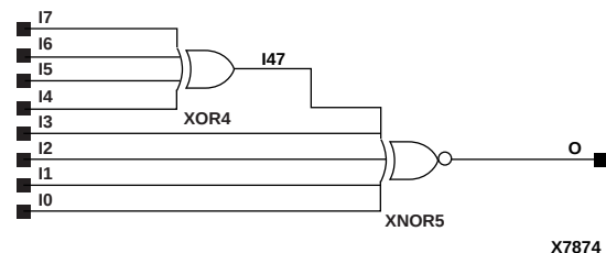
Figure 10-20 XNOR8 Implementation XC3000
