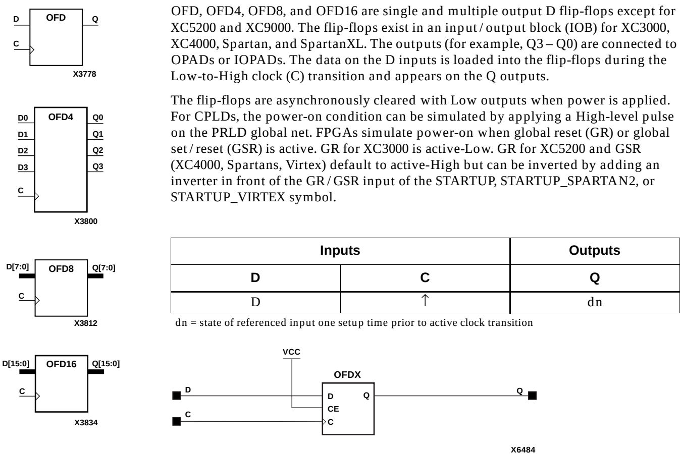
Figure 8-5 OFD Implementation XC4000E, XC4000X, Spartan, SpartanXL
