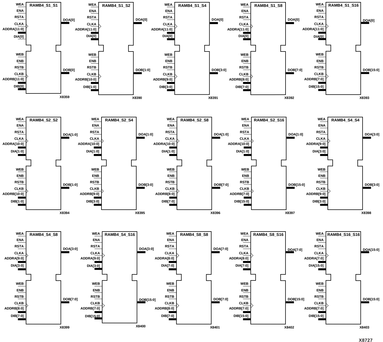
Figure 9-8 RAMB4_Sn_Sn Representations
