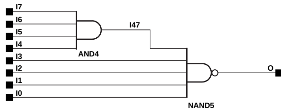
Figure 7-27 NAND8 Implementation XC3000
