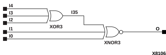
Figure 10-13 XNOR5 Implementation XC5200
