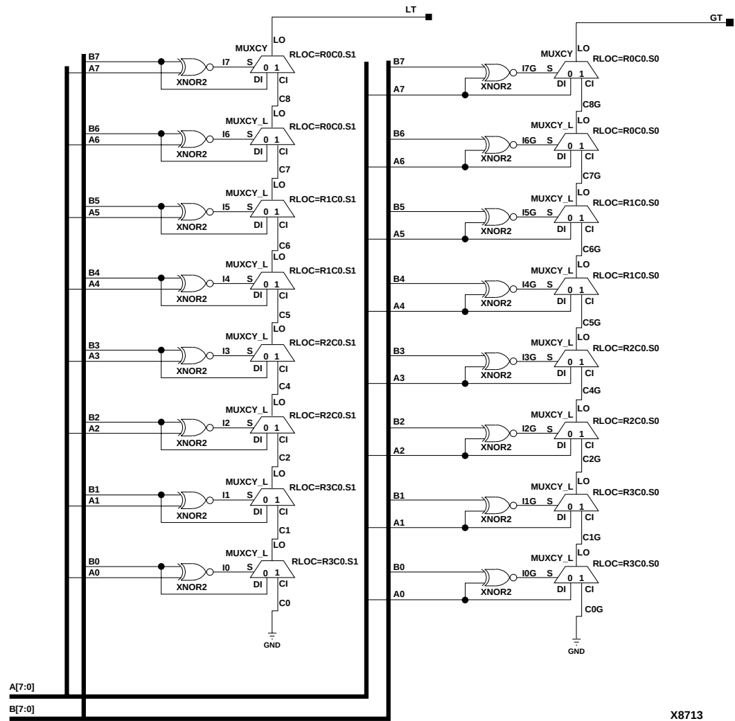
Figure 4-48 COMP8 Implementation Spartan2, Virtex
