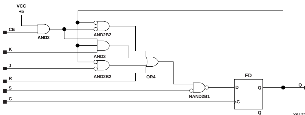
Figure 5-47 FJKSRE Implementation XC9000
