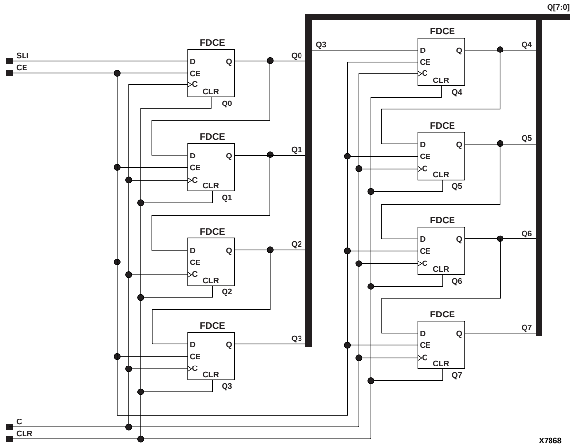
Figure 10-4 SR8CE Implementation XC3000, XC4000E, XC4000X, XC5200, XC9000, Spartan, SpartanXL, Spartan2, Virtex
