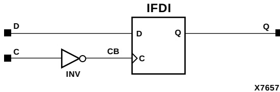
Figure 6-12 IFDI_1 Implementation XC4000E, XC4000X, Spartan, SpartanXL
