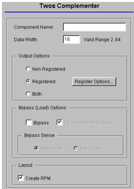
Figure 1: Main Twos Complementer Parameterization Screen
