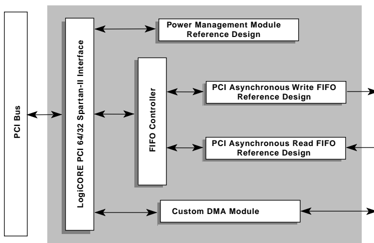
Figure 1: LogiCORE PCI Interface Block Diagram
