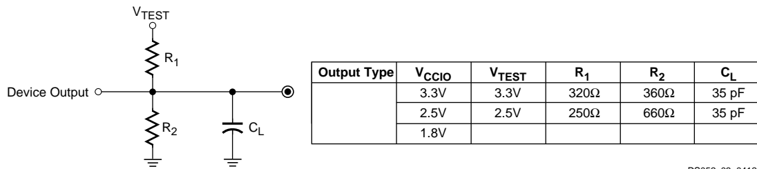
Figure 3: AC Load Circuit
