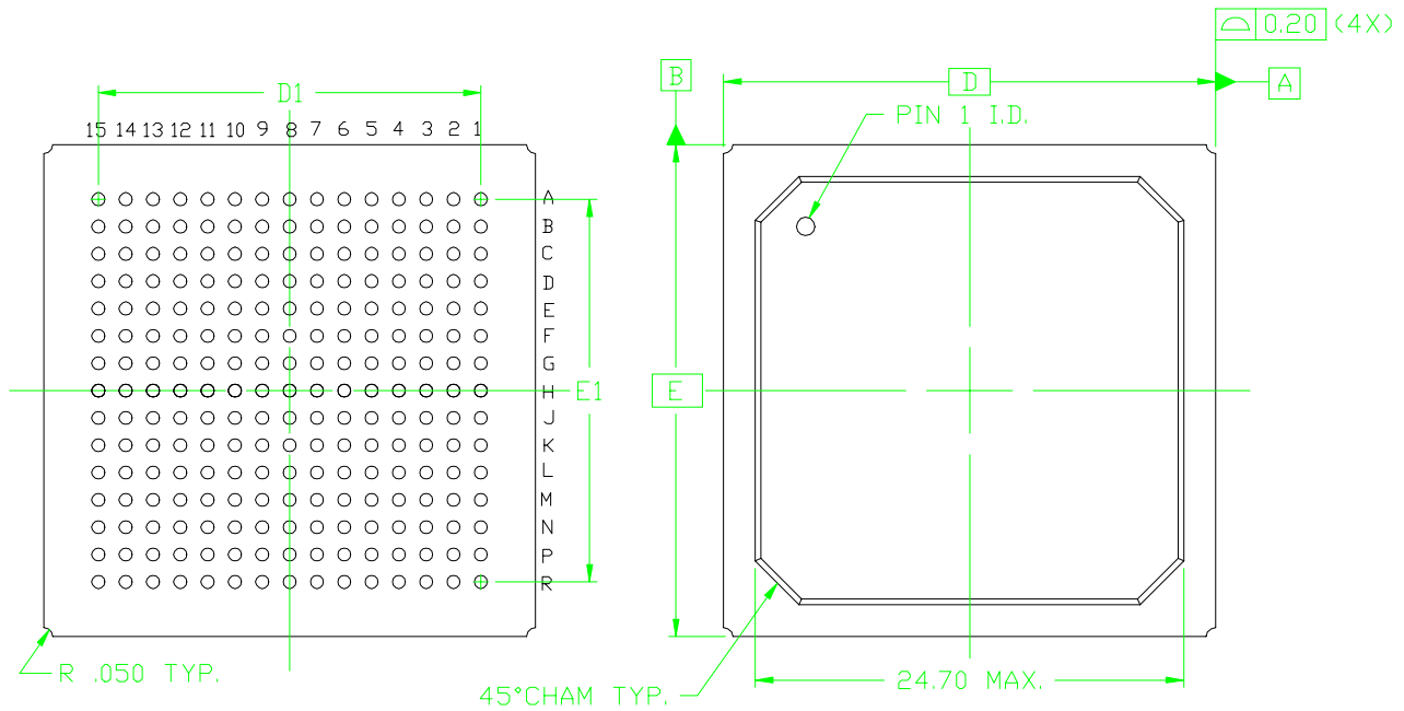
BOTTOM VIEW
