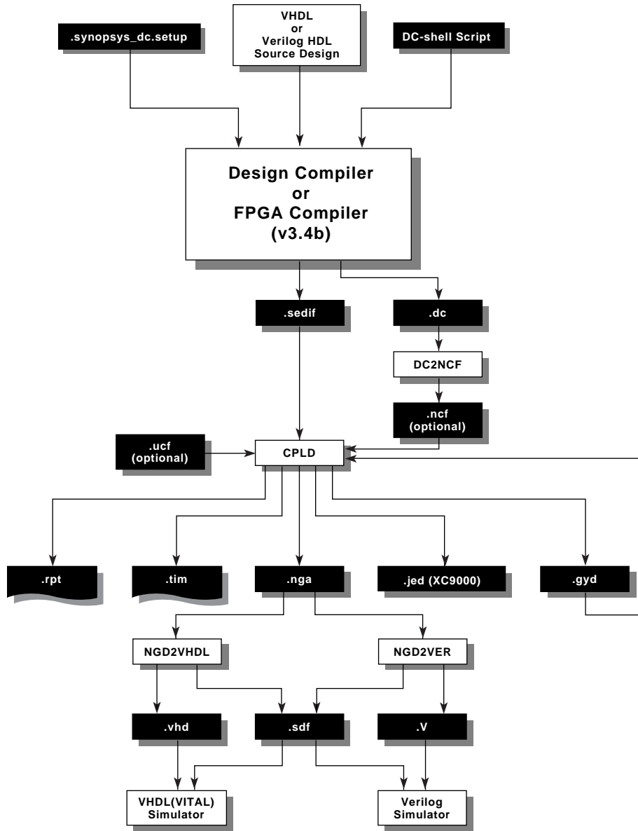
Figure 1-1 Basic CPLD Design Flow
