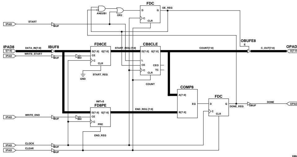
Figure 1-2 Schematic Representation - SCAN Design
